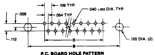
MOUNTING STYLE C FLUSH INSERT
