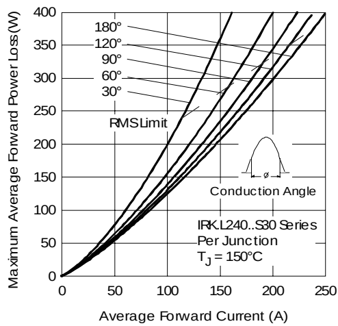
Fig. 9 - Forward Power Loss Characteristics
