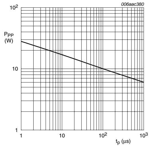
T_{amb} = 25\text{ }^{\circ}C (1) PESD9V0V4UK
