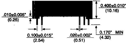
SIDEVIEW - "A" Package Option
