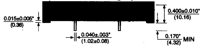
SIDEVIEW - "B" Package Option
