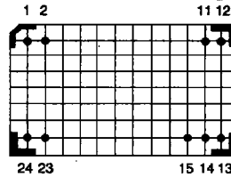
BOTTOMVIEW - "A" Package Option
