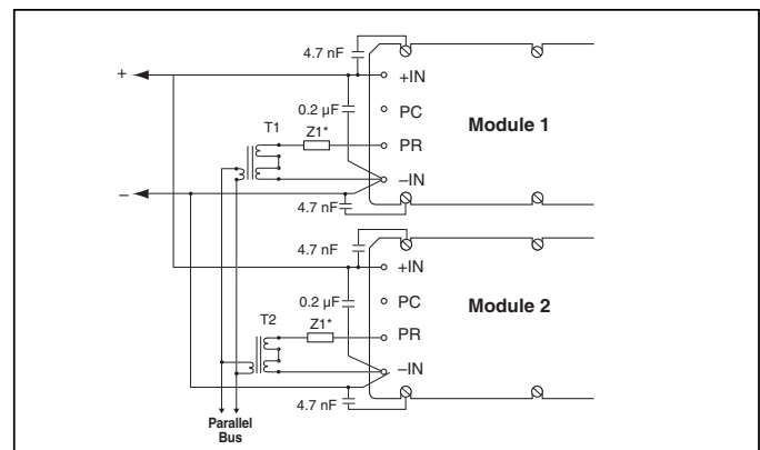
Figure 10 — Transformer-coupled interface.
