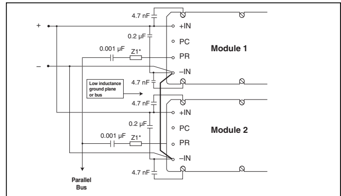
Figure 9 — AC coupled single-wire interface.
