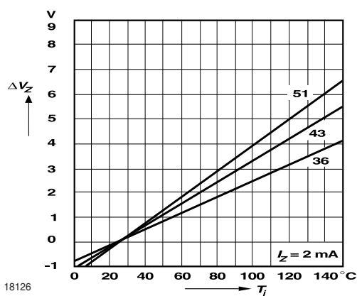
Figure 9. Change of Zener voltage versus junction temperature
