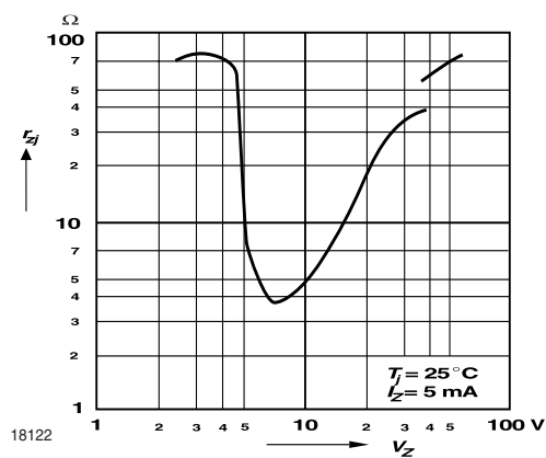
Figure 5. Dynamic resistance versus Zener voltage
