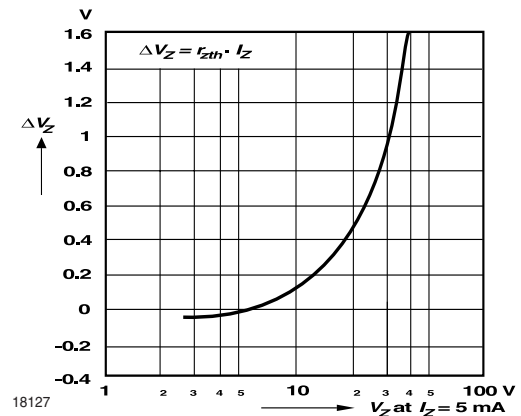
Figure 10. Change of Zener voltage from turn-on up to the point of thermal equilibrium versus Zener voltage
