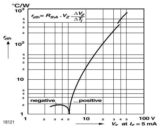
Figure 4. Thermal differential resistance versus Zener voltage
