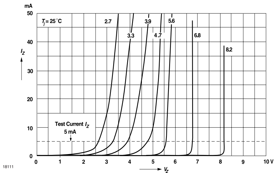
Figure 12. Breakdown Characteristics
