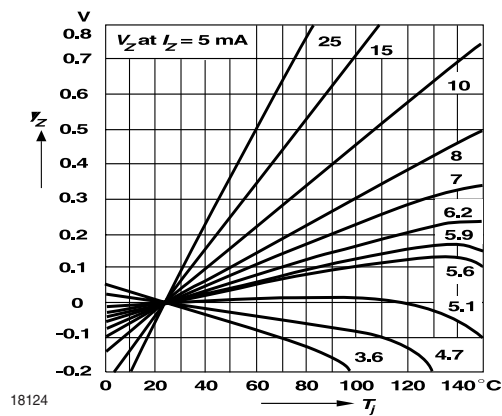
Figure 7. Change of Zener voltage versus junction temperature
