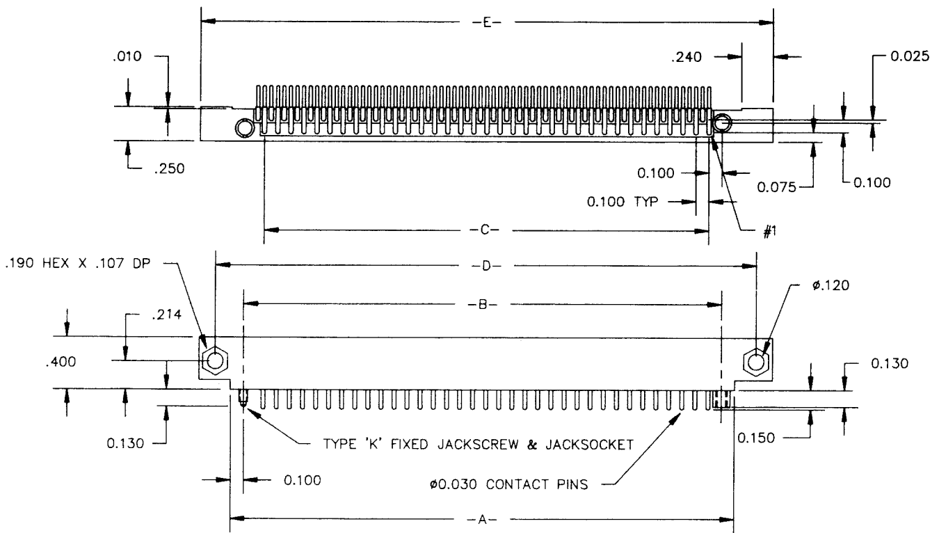
DIMENSIONS - 2 ROW CONNECTORS
