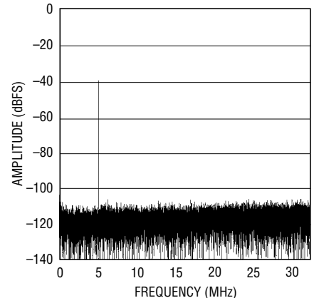
LTC2205: 32K Point FFT, f_{IN} = 5.1\text{MHz} , -40\text{dB} , 65\text{Mps} , \text{PGA} = 1 , \text{DITH} = 1
