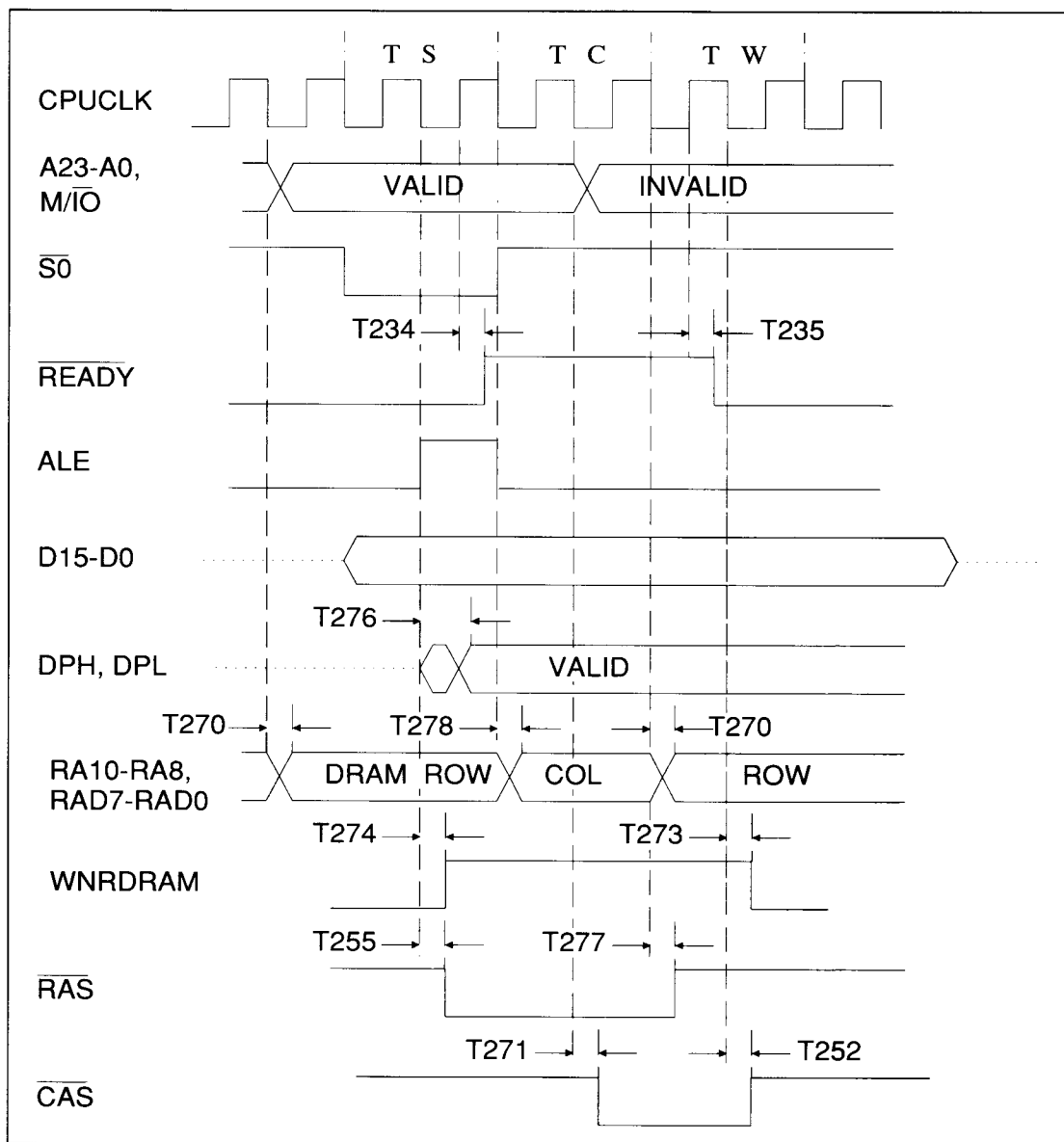
FIGURE 11-7. 80286 - NON-PAGE MODE 00, 1 WAIT STATE WRITE (4072H = 0001)
