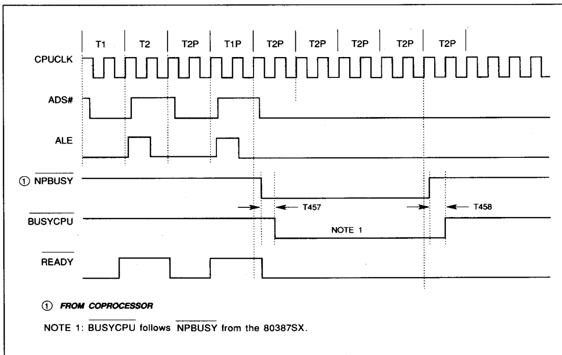
FIGURE 11-58. 80386SX - BUSYCPU ASSERTION DURING COPROCESSOR ACCESS
