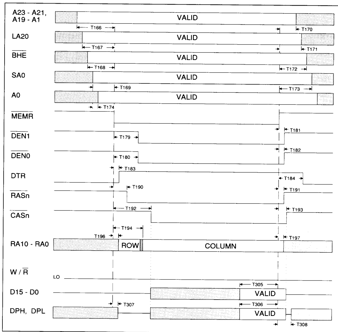
FIGURE 11-47. AT BUS MASTER, READ FROM ON-BOARD MEMORY
