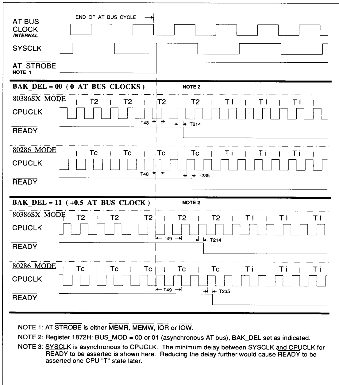
FIGURE 11-41. ASYNCHRONOUS AT BUS CYCLE COMPLETION, BAK_DEL = 0 OR +0.5 AT BUS CLOCKS
