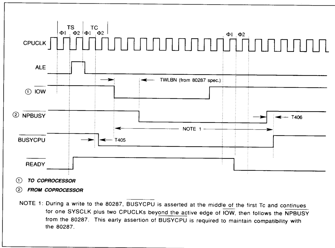
FIGURE 11-52. 80286 - BUSYCPU ASSERTED DURING COPROCESSOR ACCESS
