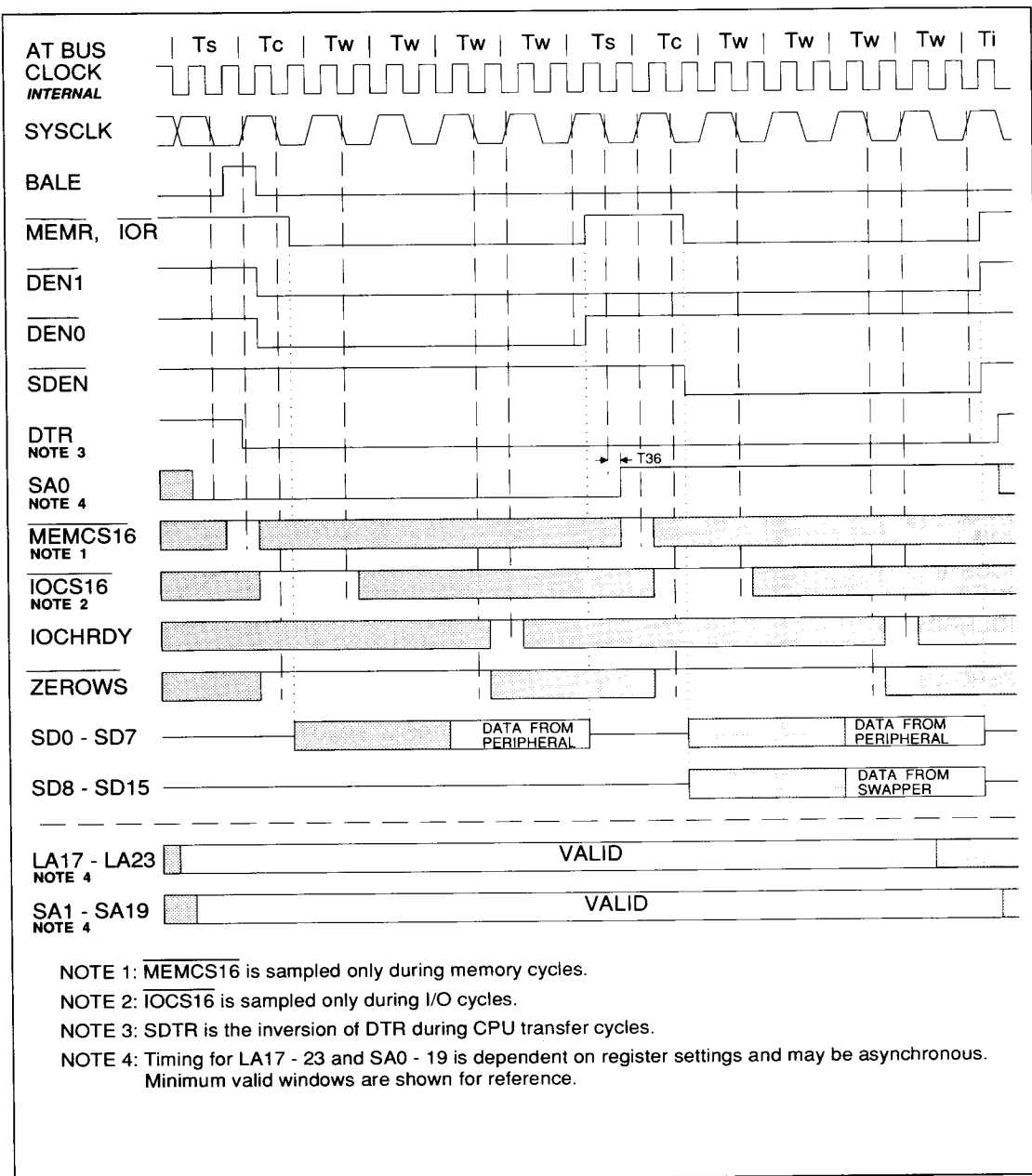
FIGURE 11-27. AT BUS I/O OR MEMORY READ: 8-BIT, WORD TO BYTE CONVERSION, DEFAULT TIMING
