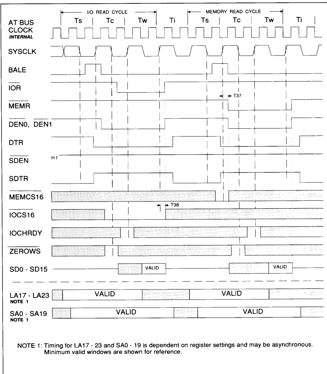
FIGURE 11-29. AT BUS I/O OR MEMORY READ: 16-BIT, DEFAULT TIMING
