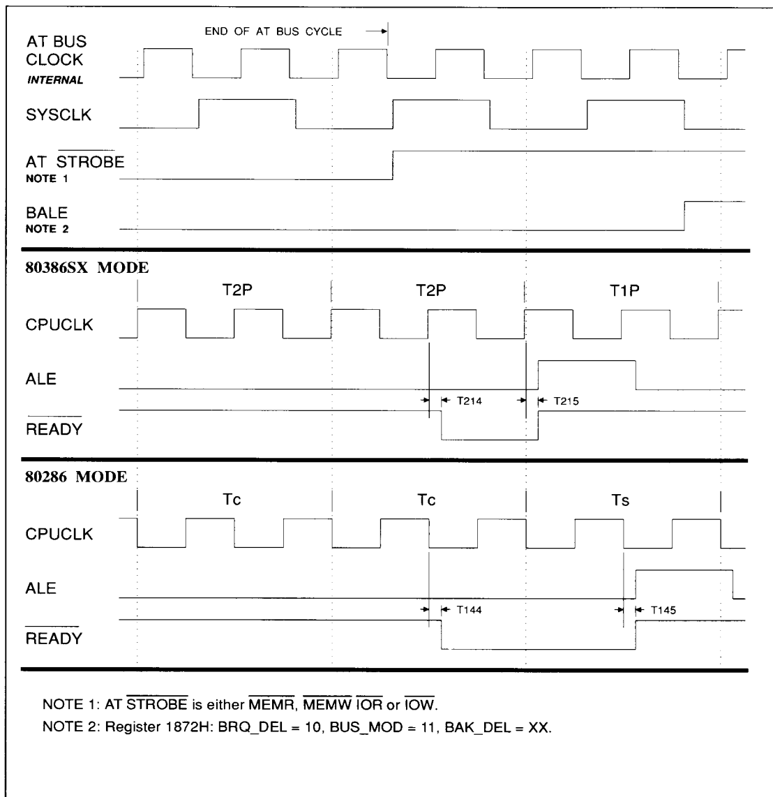
FIGURE 11-39. SYNCHRONOUS AT BUS CYCLE COMPLETION, AT BUS CLOCK = CPUCLK ÷ 1
