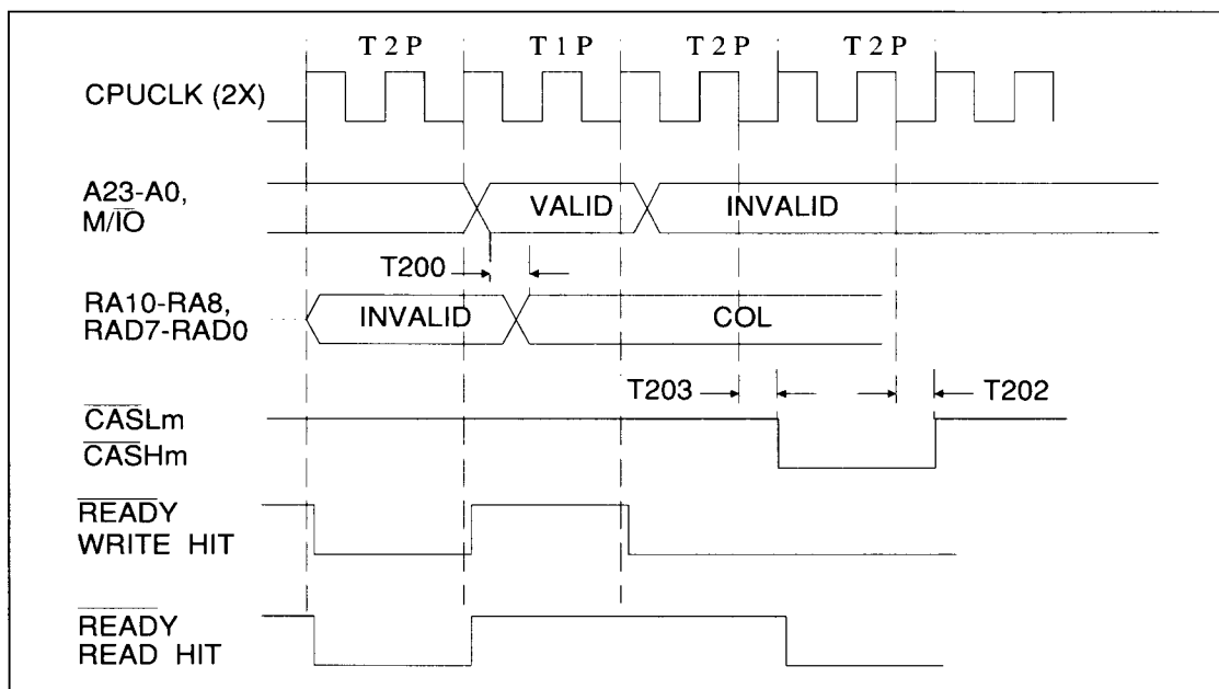
FIGURE 11-14. 80386SX - PAGE MODE, READ CYCLE FOLLOWED BY A PAGE HIT
