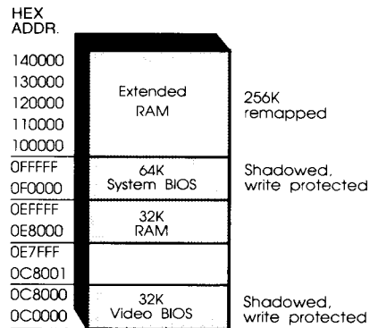
FIGURE 6-3. X_MEM = 1
