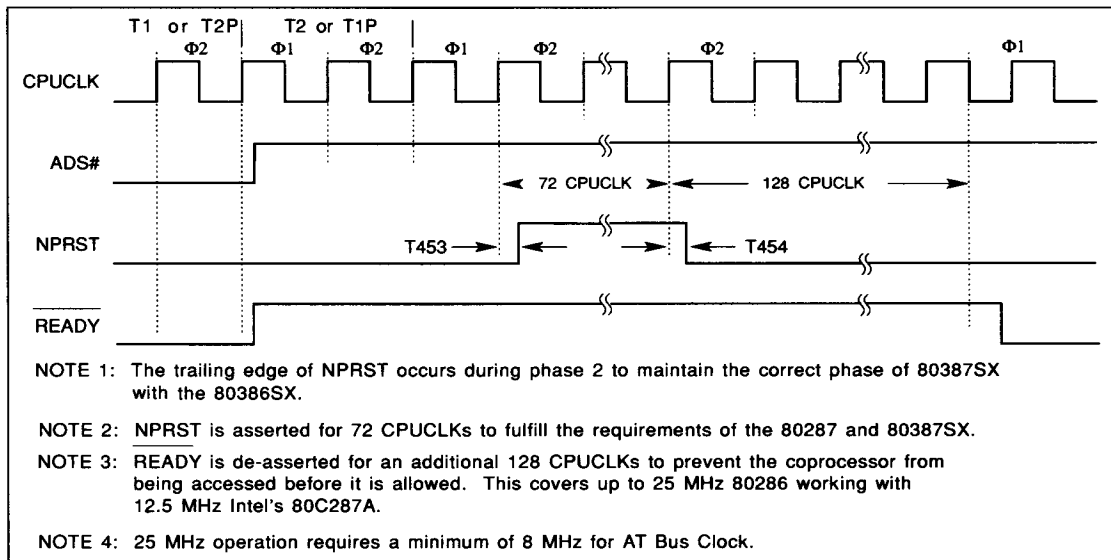
FIGURE 11-56. 80386SX - COPROCESSOR RESET (NPRST) INITIATED BY IOW TO PORT F1
