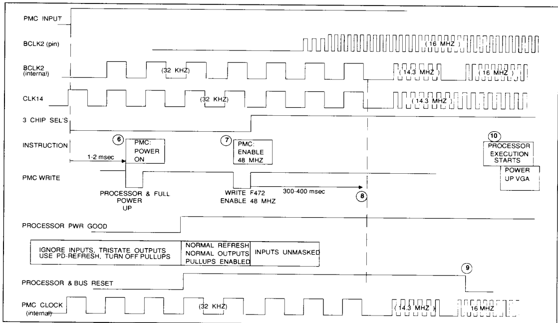
FIGURE 8-3. POWER UP
