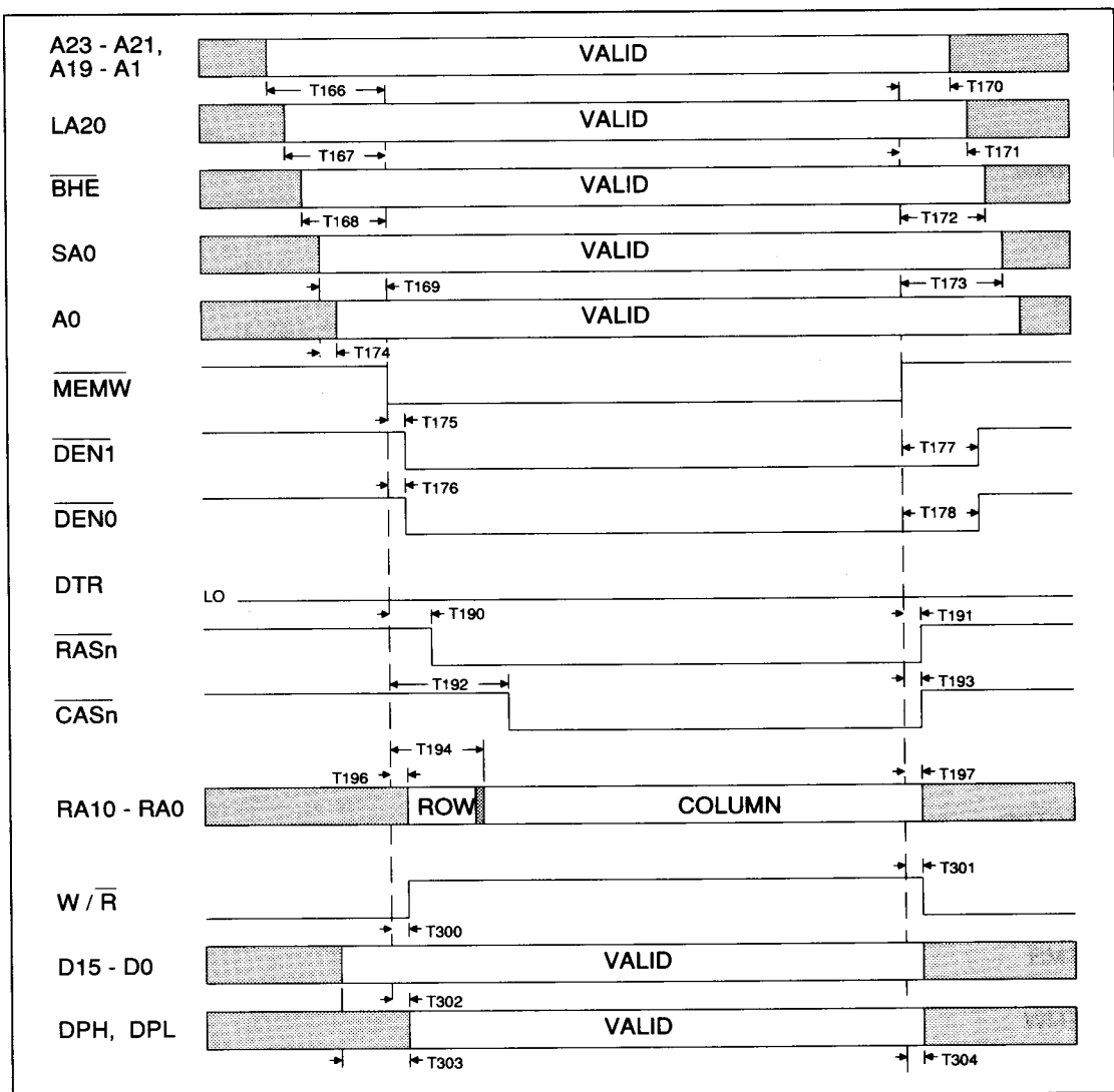
FIGURE 11-46. AT BUS MASTER, WRITE TO ON-BOARD MEMORY
