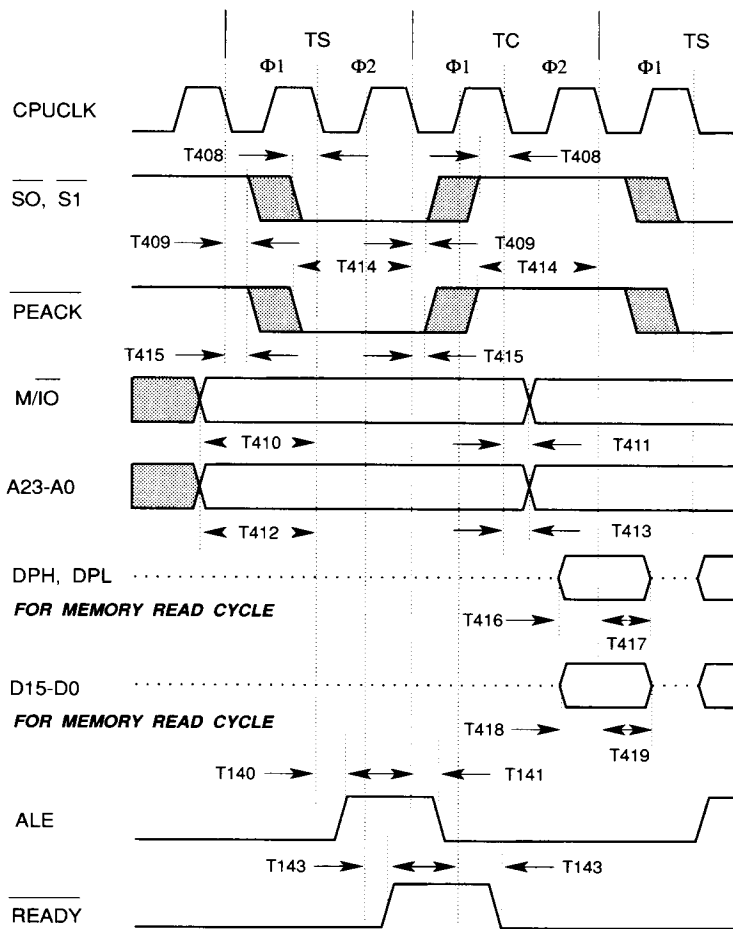
FIGURE 11-54. 80286 - MISCELLANEOUS TIMING
