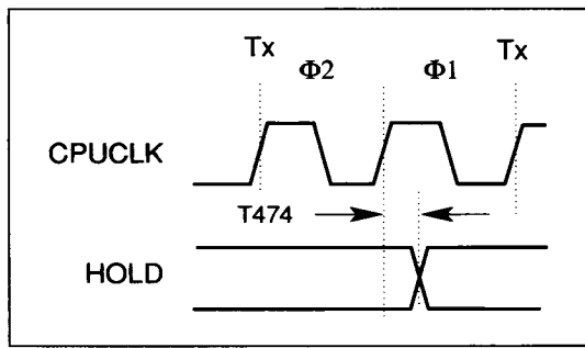
FIGURE 11-62. 80386SX - OUTPUT DELAY TIMING
