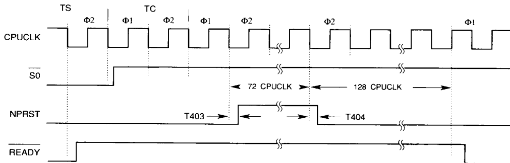
FIGURE 11-49. 80286 - CPURES AND NPRST DURING POWER UP
