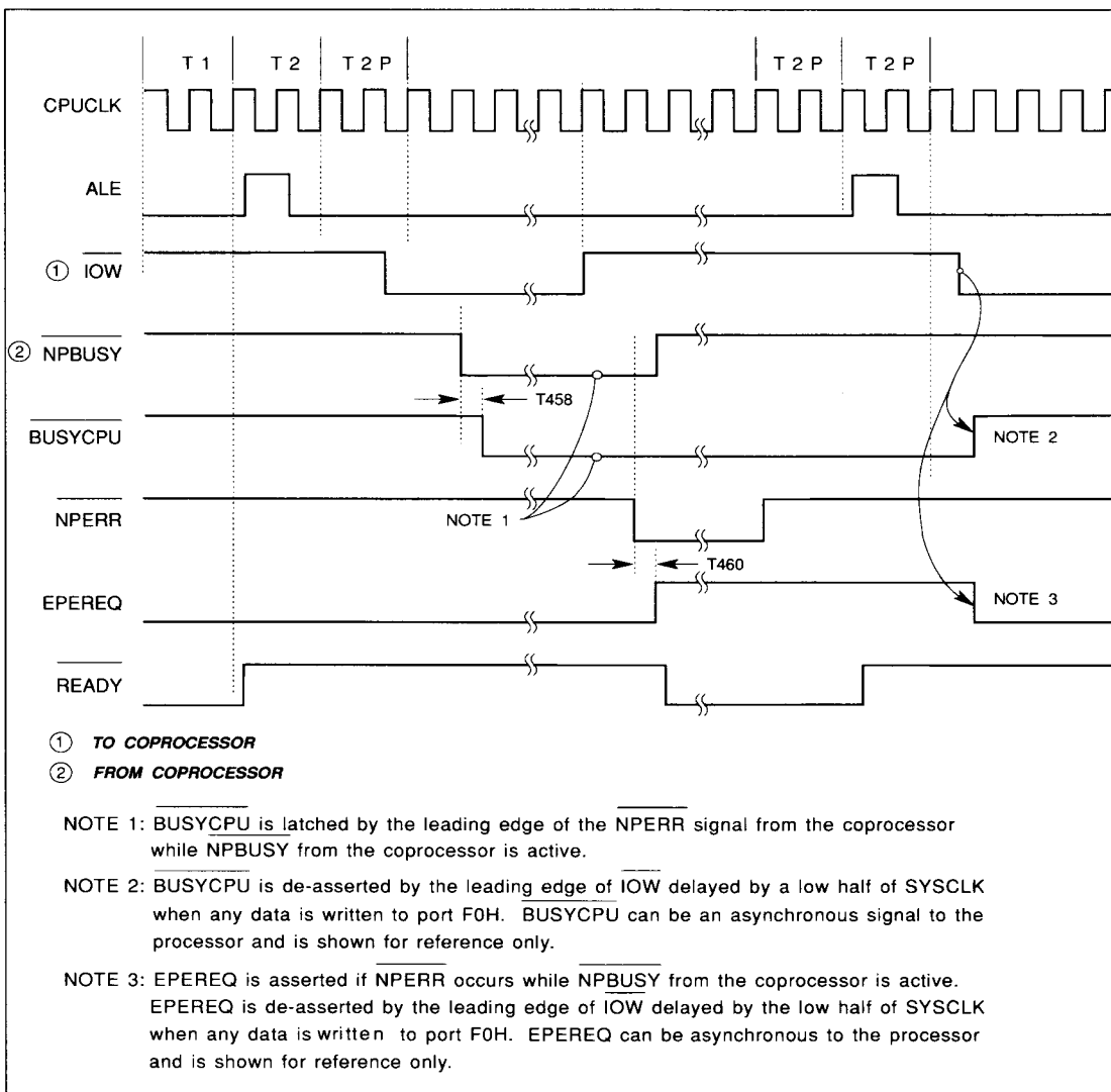
FIGURE 11-59. 80386SX - LATCHING BUSYCPU WHEN AN ERROR OCCURS AND CLEARING IT WITH A WRITE TO PORT F0
