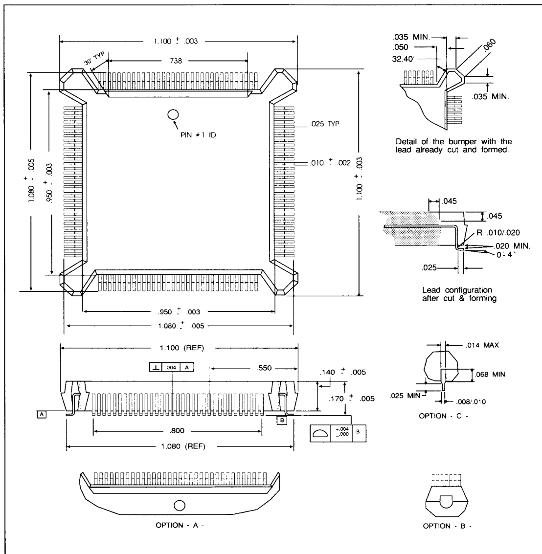
FIGURE 13-1. 132-PIN PQFP PACKAGE
