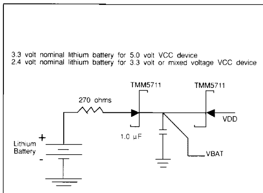
FIGURE 7-2. VBAT EXTERNAL SUPPORT
