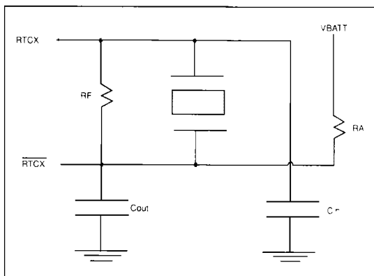
FIGURE 7-3. RTC CRYSTAL EXTERNAL CIRCUITRY
