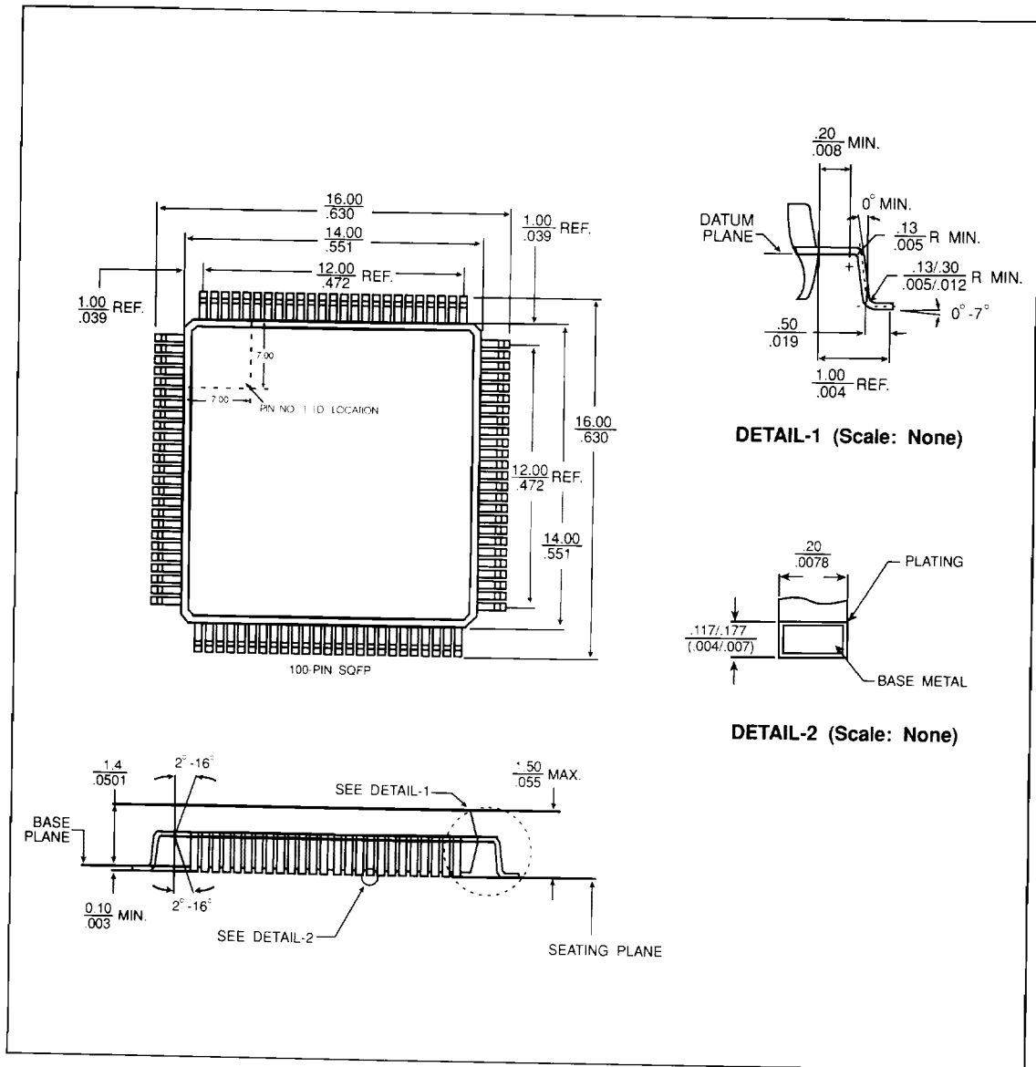
FIGURE 11-2. 100-PIN SQFP PACKAGE DIMENSIONS
