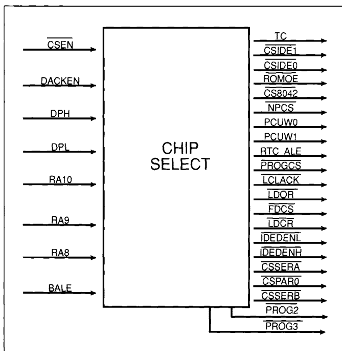
FIGURE 4-1. CHIP SELECT BLOCK DIAGRAM
