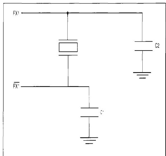
FIGURE 5-1. 16 MHz CRYSTAL
