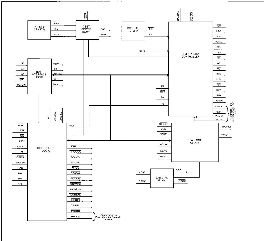
FIGURE 2-1. WD76C20ALV FUNCTIONAL BLOCK DIAGRAM
