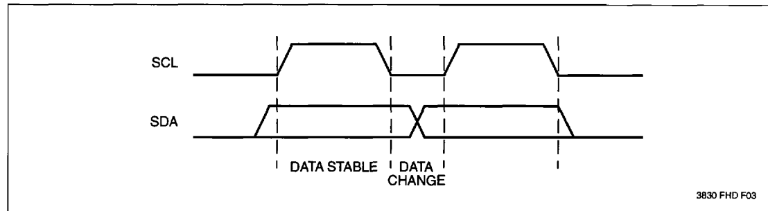
Figure 1. Data Validity
