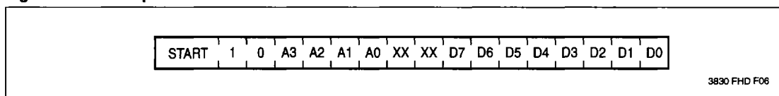
Figure 4. Read Sequence
