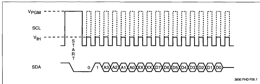
Figure 3. Programming Sequence
