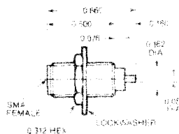
Bulkhead Feedthrough Female
