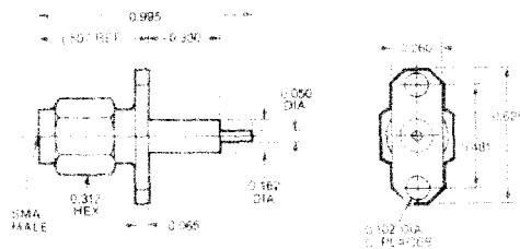
Two Hole Flange Mount Male
