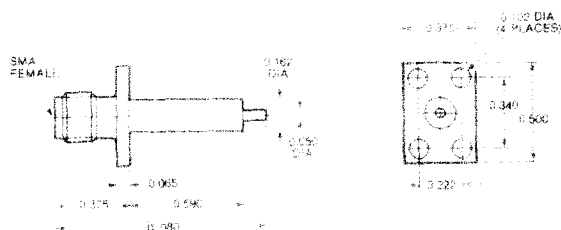
Flange Mount Female
