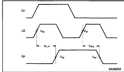
Waveform 2. Propagation Delay, Latch Enable to Output
