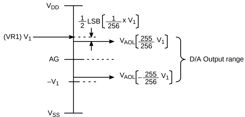
Fig. 3 – EXTERNAL REFERENCE VOLTAGE MODE
