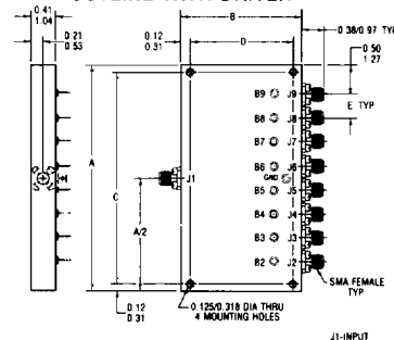
CONFIGURATION S OUTLINE WITHOUT DRIVER
