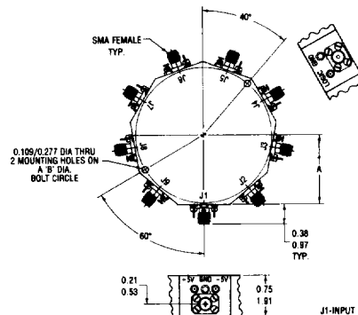
CONFIGURATION S OUTLINE WITHOUT DRIVER
