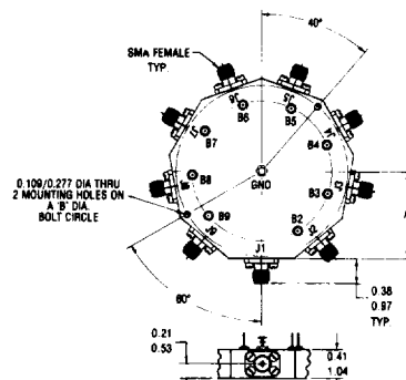
CONFIGURATION R OUTLINE WITHOUT DRIVER
