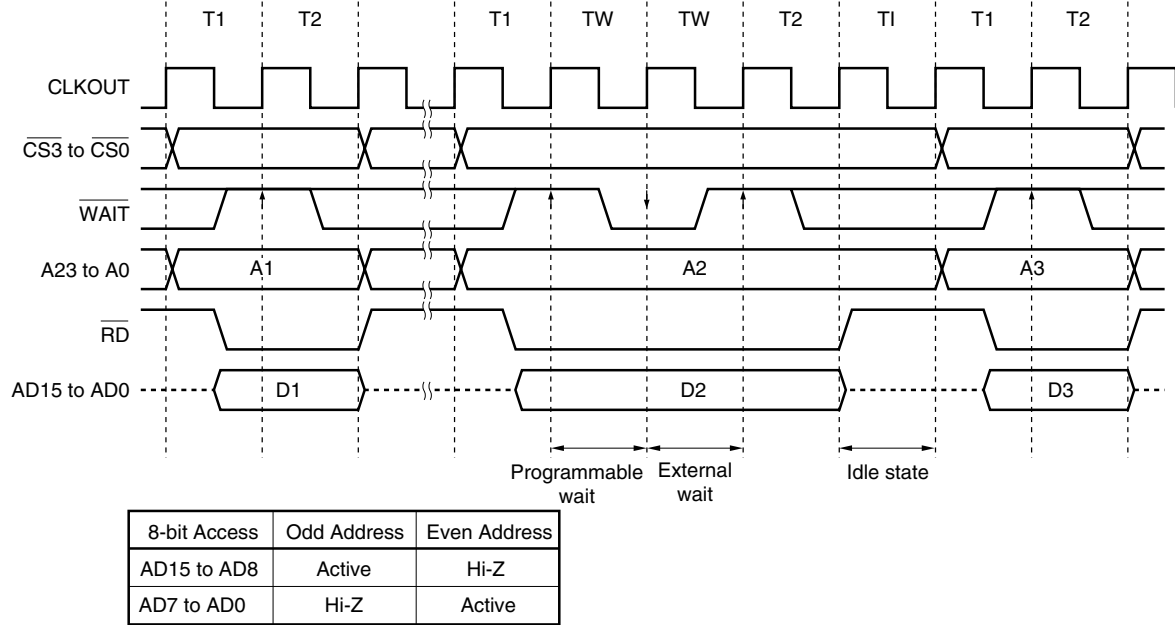
Figure 5-9. Separate Bus Read Timing (Bus Size: 16 Bits, 16-Bit Access)
