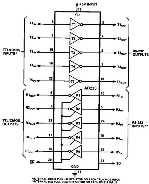
Figure 12. AD235 Typical Operating Circuit
