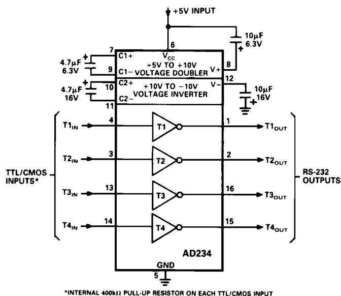
Figure 10. AD234 Typical Operating Circuit
