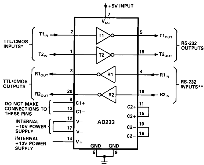
Figure 8. AD233 Typical Operating Circuit
