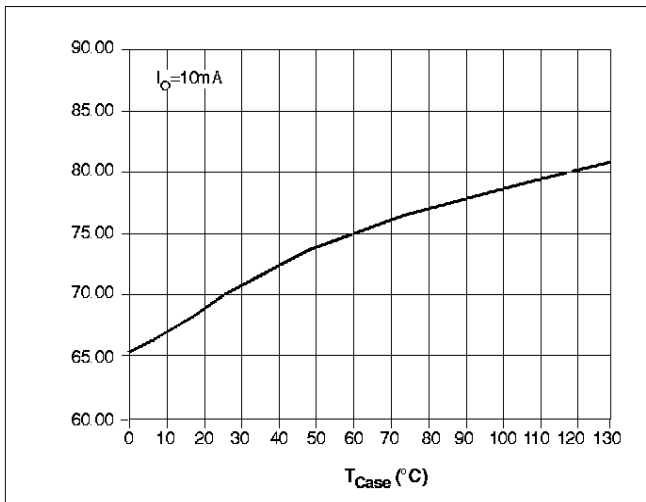
Adjust Pin Current vs. Temperature
