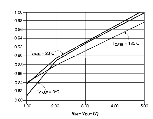
Minimum Load Current vs. V_{IN} - V_{OUT}
