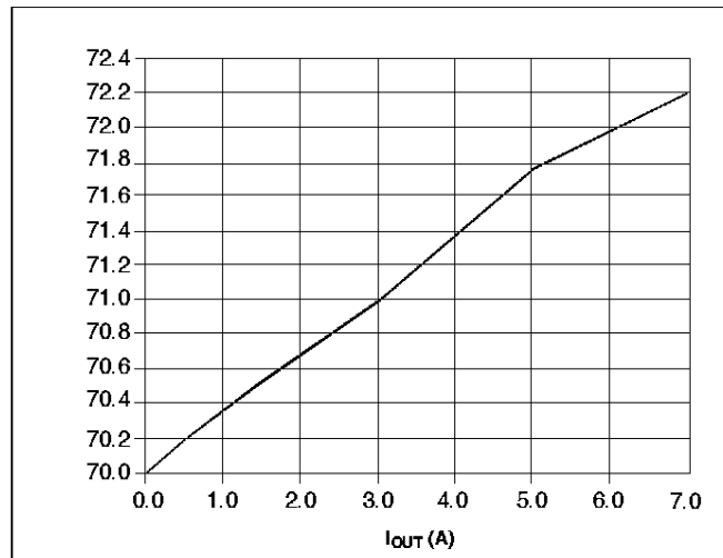
Adjust Pin Current vs. I_{OUT}
