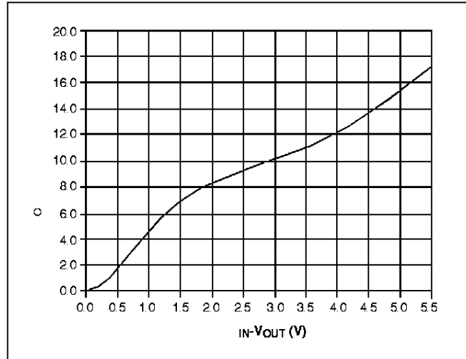
Short Circuit Current vs. V_{IN} - V_{OUT}
