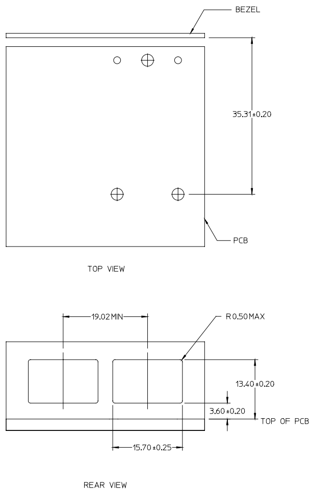
Figure 19. Host Frontplate Layout (dimensions in mm)
