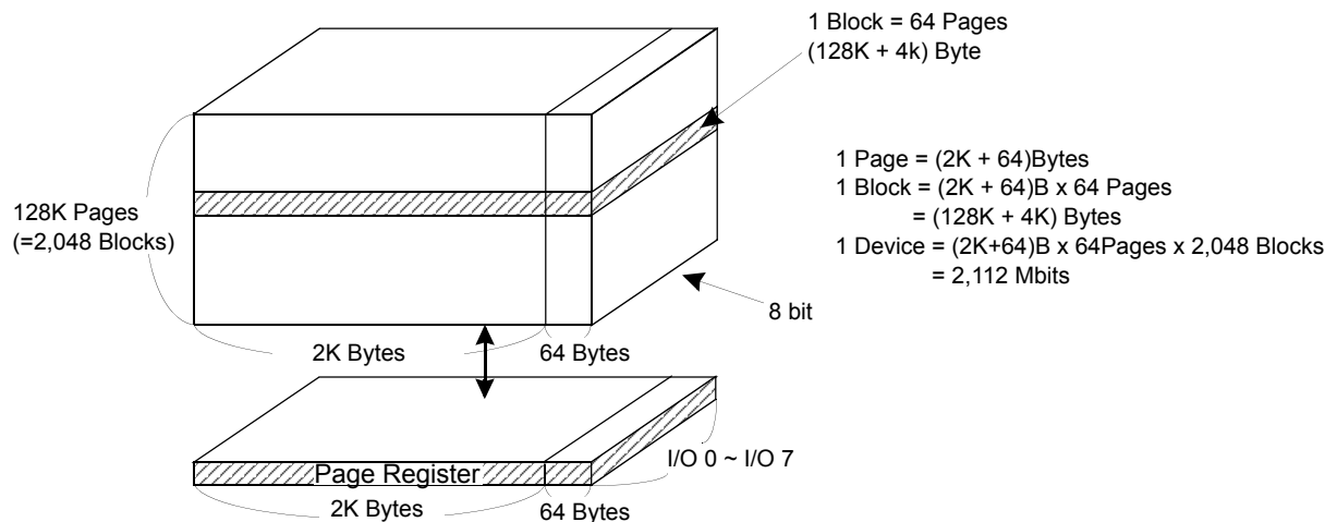
Figure 2. K9F2G08X0A Array Organization
