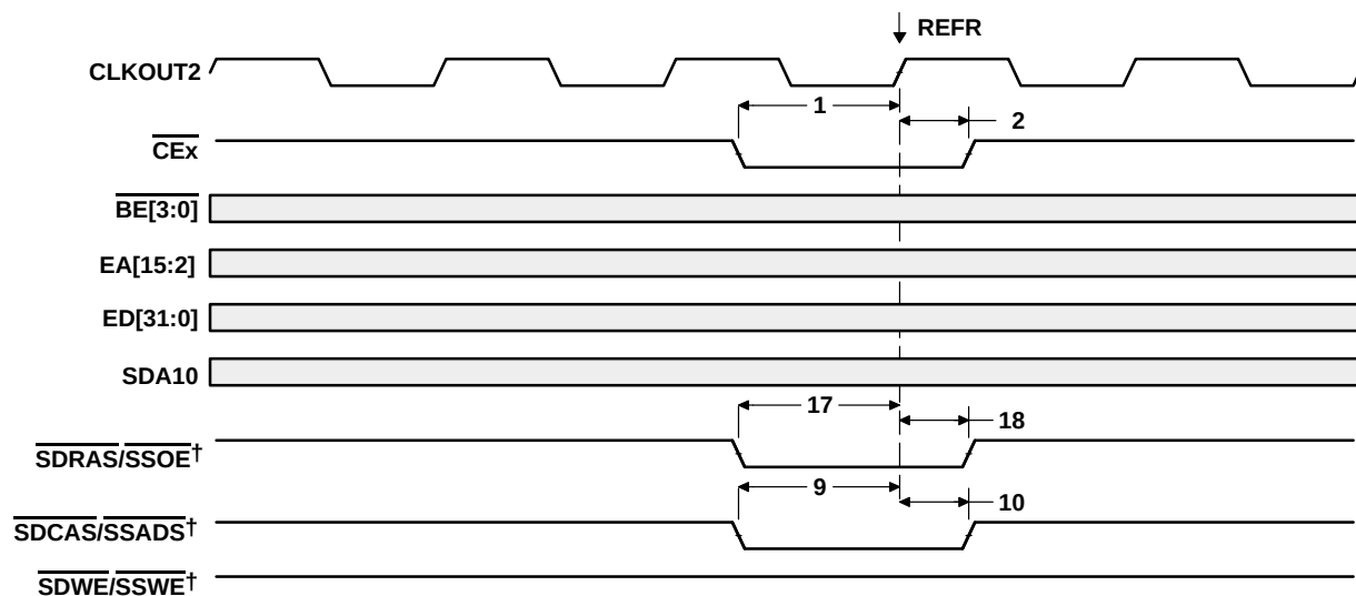
Figure 26. SDRAM REFR Command
