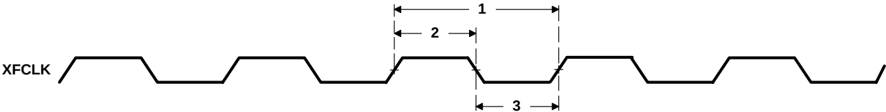
Figure 15. XFCLK Timings
