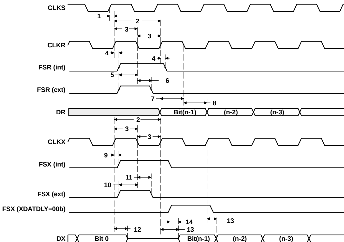
Figure 47. McBSP Timings
