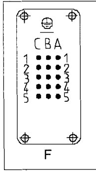
View from cable side
