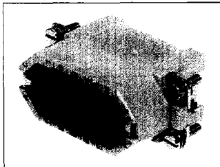
Male insert crimp termination
