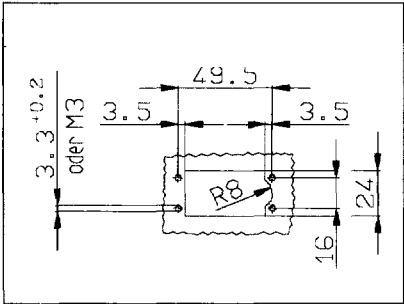
Panel cut out for application, without Housing
