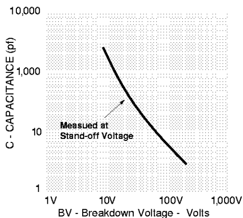
Figure 2 - Typical Capacitance vs. Breakdown Voltage
