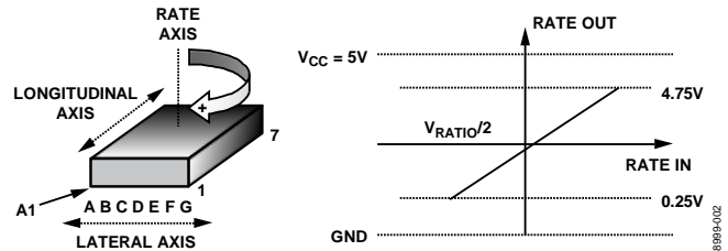
Figure 2. RATEOUT Signal Increases with Clockwise Rotation
