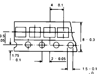
SOT-23 and SOT-143 TAPE DIMENSIONS
