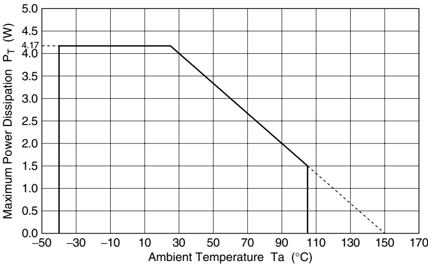
Figure 1 Derating Curve
