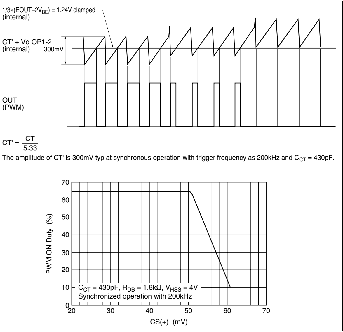
Timing Chart 7 (Current Limiting)
