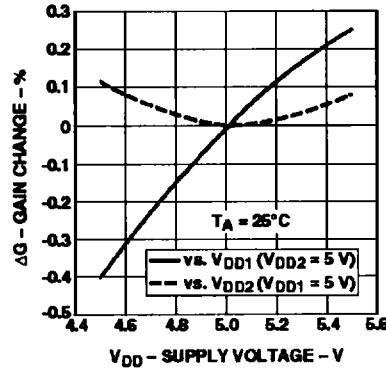
Figure 7. Gain Change vs. V_{DD1} and V_{DD2} .
