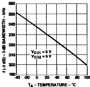
Figure 20. 3 dB Bandwidth vs. Temperature.
