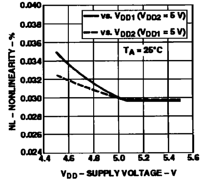
Figure 11. 100 mV Nonlinearity vs. V_{DD1} and V_{DD2} .
