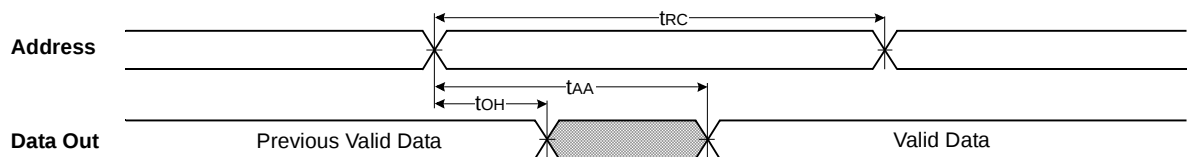
TIMING WAVEFORM OF READ CYCLE(2) ( \overline{\text{WE}}=\text{V}_{\text{IH}} )
