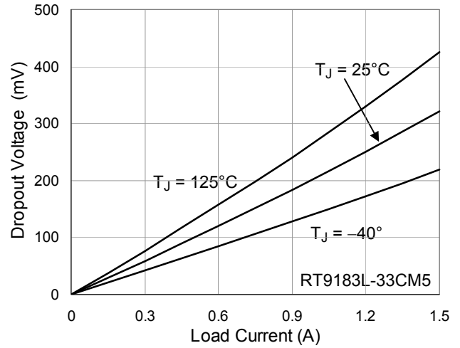
Dropout Voltage
