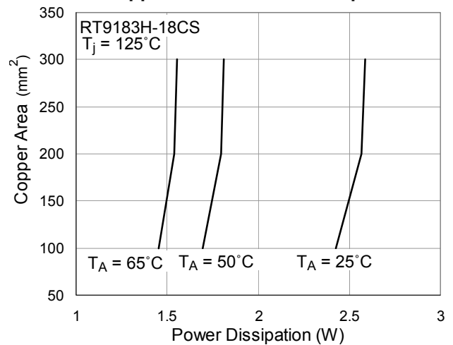
Copper Area vs. Power Dissipation
