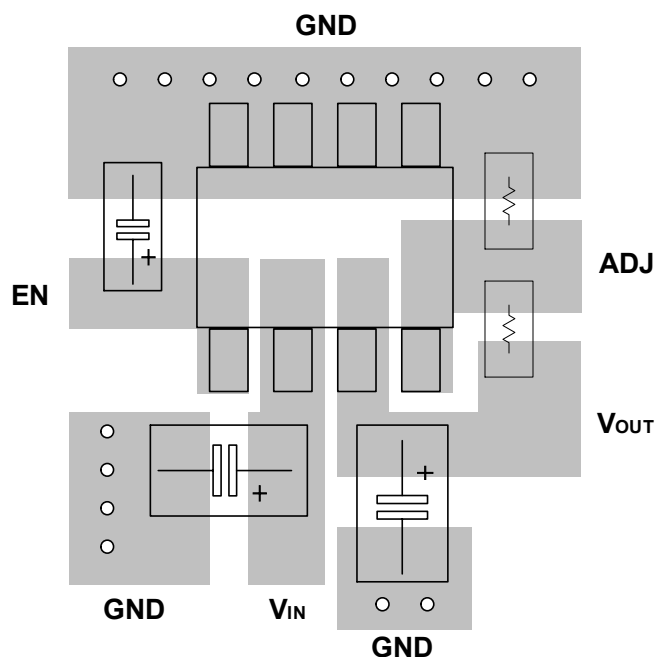
SOP-8 Board Layout
