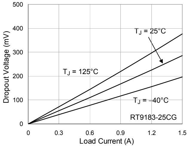
Dropout Voltage
