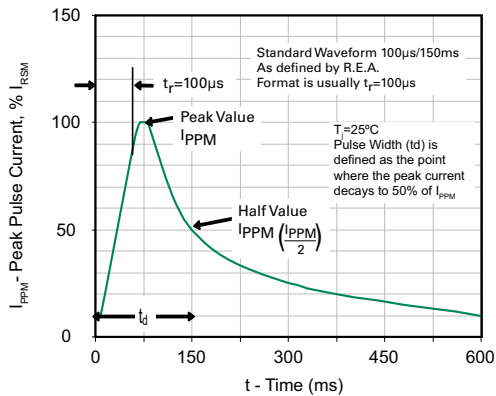
Figure 3 - Pulse Waveform
