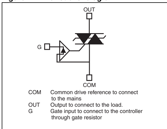
Figure 1. Functional diagram
