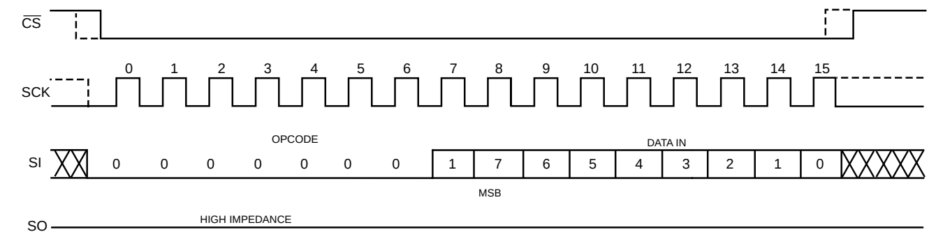
Figure 7. WRSR Timing
