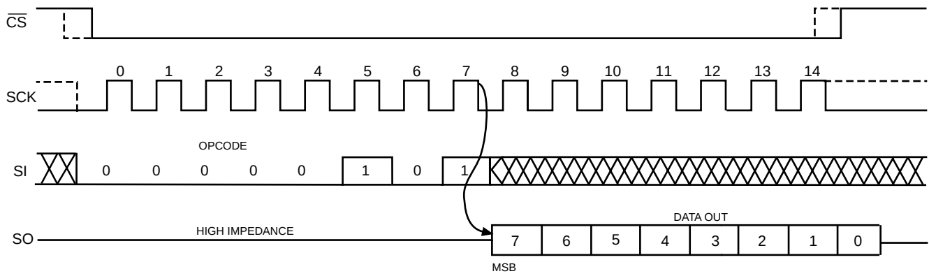
Figure 5. RDSR Timing
