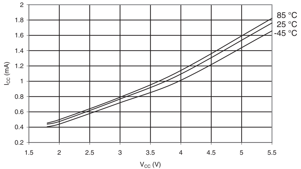
Figure 30-555. ATmega6490P: Idle Supply Current vs. V_{CC} (Internal RC Oscillator, 8MHz)
