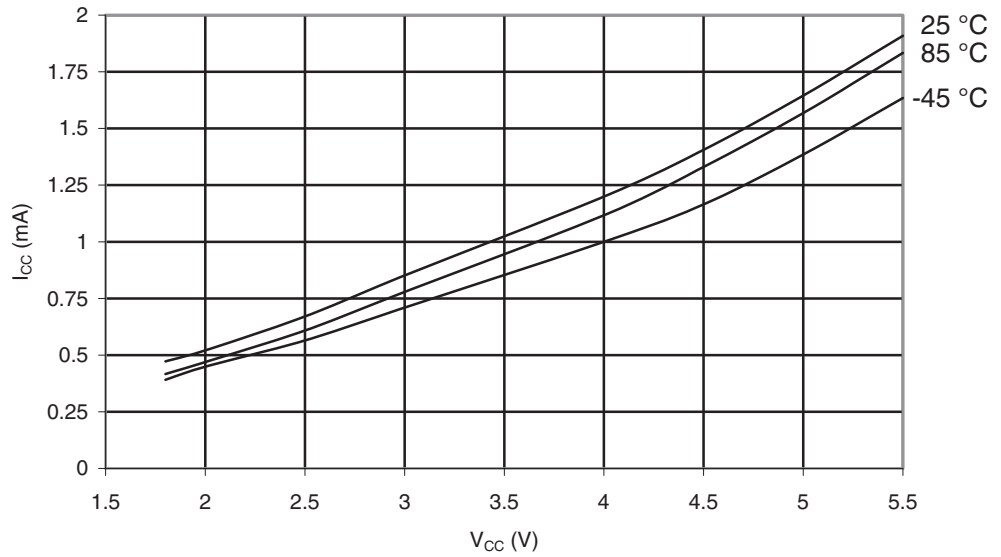
Figure 30-8. ATmega169A: Idle Supply Current vs. V_{CC} (Internal RC Oscillator, 8MHz)
