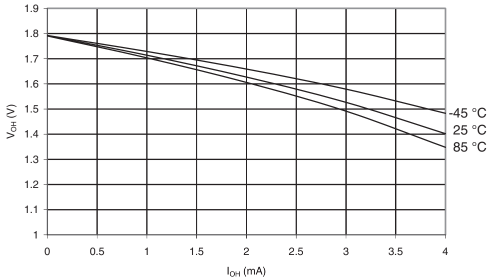
Figure 30-86. ATmega169PA: I/O Pin Output Voltage vs. Source Current, Ports A, C, D, E, F, G ( V_{CC} = 1.8V )
