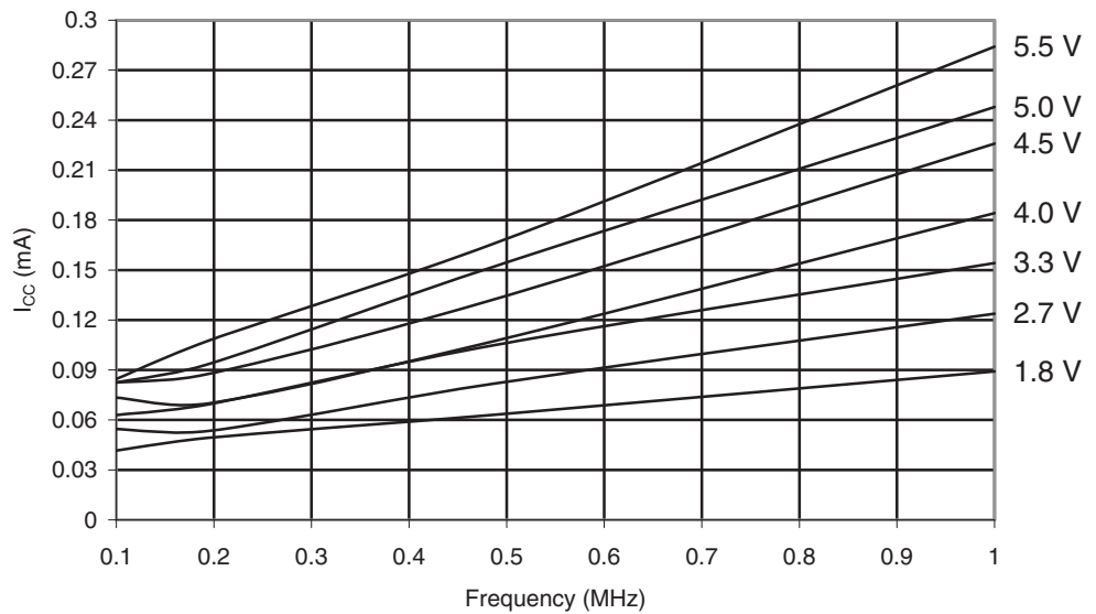
Figure 30-553. ATmega6490P: Idle Supply Current vs. Low Frequency (0.1 - 1.0MHz)
