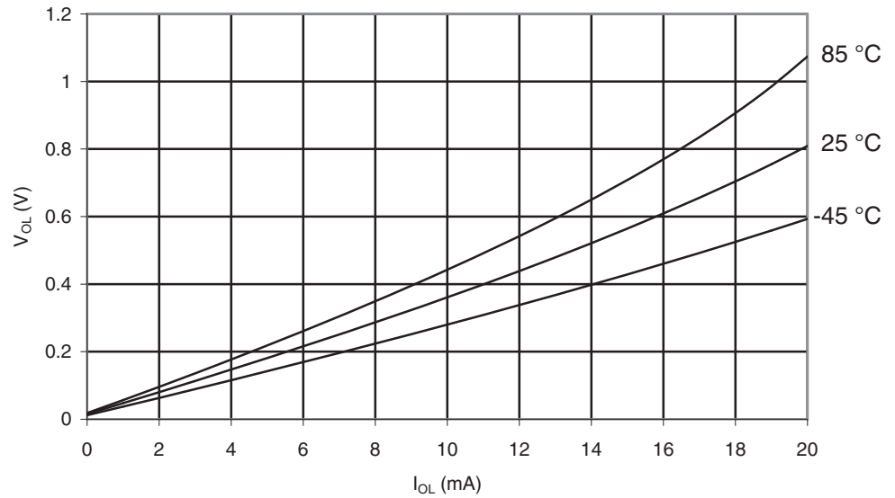
Figure 30-32. ATmega169A: I/O Pin Output Voltage vs. Sink Current, Port B ( V_{CC} = 2.7V )
