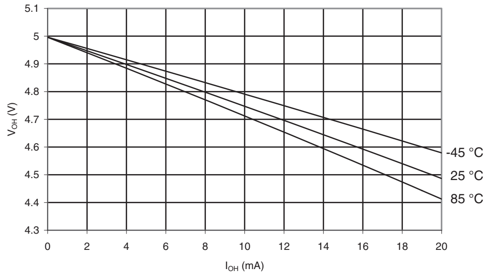
Figure 30-87. ATmega169PA: I/O Pin Output Voltage vs. Source Current, Port B ( V_{CC} = 5V )
