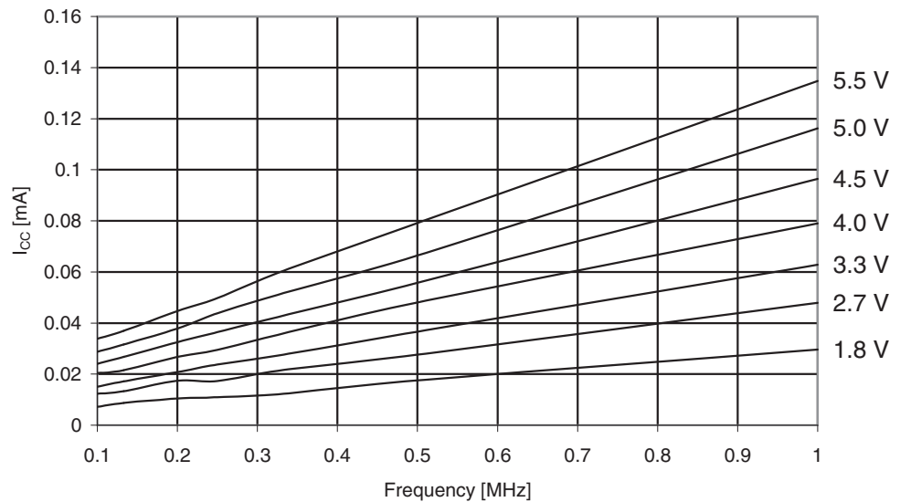
Figure 30-302. ATmega3290A: Reset Supply Current vs. V_{CC} (0.1 - 1.0MHz, Excluding Current Through The Reset Pull-up)
