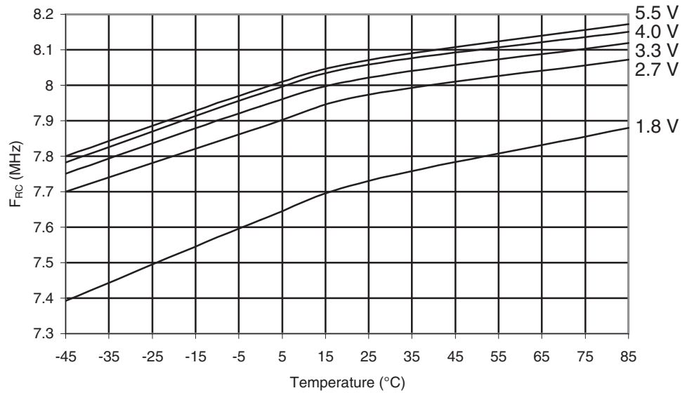
Figure 30-473. ATmega649P: Calibrated 8MHz RC Oscillator Frequency vs. Temperature
