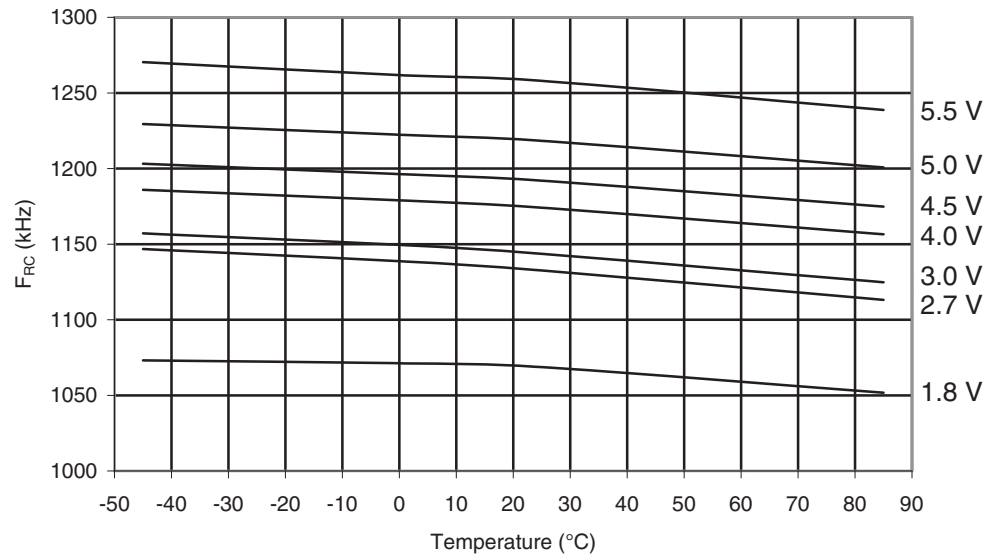
Figure 30-110. ATmega169PA: Watchdog Oscillator Frequency vs. Temperature
