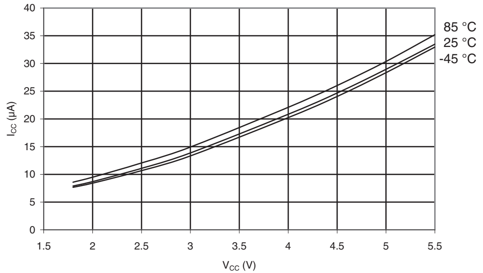
Figure 30-5. ATmega169A: Active Supply Current vs. V_{CC} (32kHz Watch Crystal)
