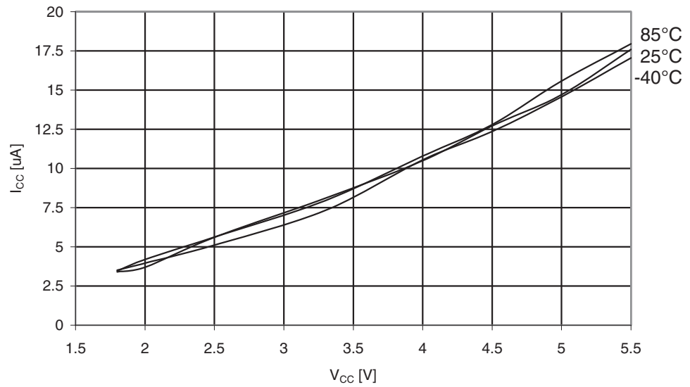
Figure 30-359. ATmega3290PA: Watchdog Timer Current vs. V_{CC}
