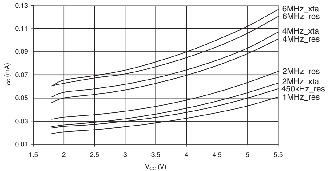
Figure 30-199. ATmega329PA Standby Supply Current vs. V_{CC} (Xtall and Resonator, Watchdog Timer Disabled)
