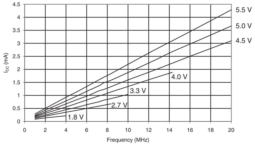
Figure 30-493. ATmega6490A: Idle Supply Current vs. Frequency (1 - 20MHz)
