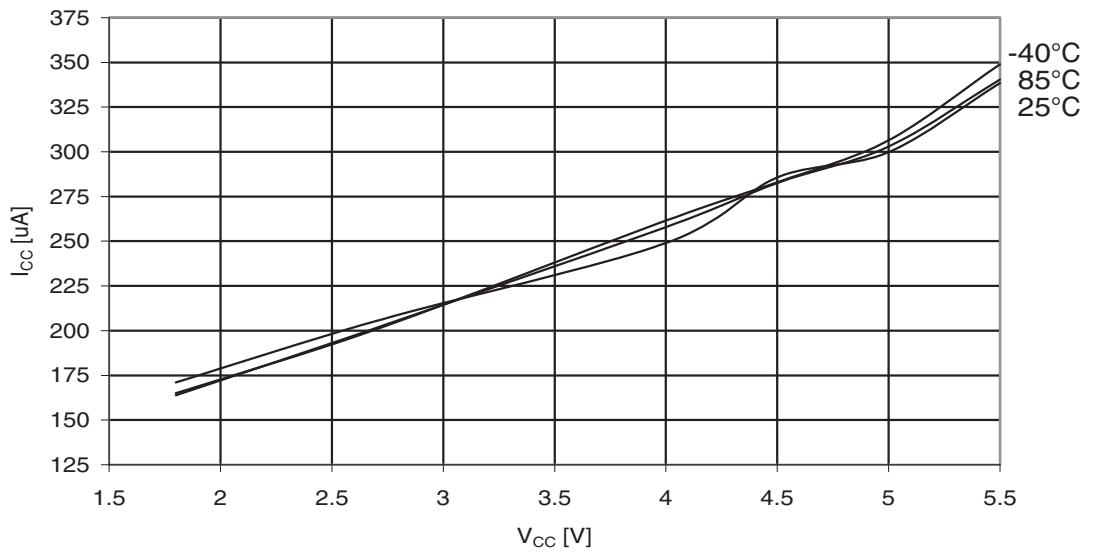
Figure 30-177. ATmega329A: Active Supply Current with ADC at 1MHz vs. V_{CC}
