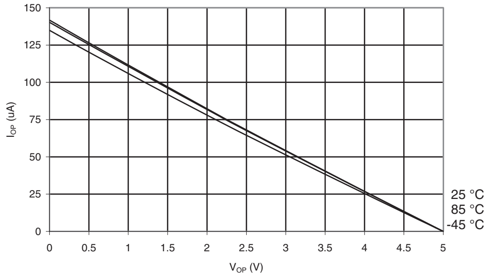
Figure 30-78. ATmega169PA: I/O Pin Pull-up Resistor Current vs. Input Voltage ( V_{CC} = 5V )
