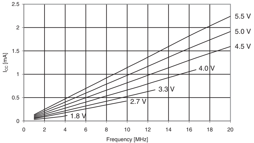
Figure 30-243. ATmega329PA: Reset Supply Current vs. V_{CC} (1 - 20MHz, Excluding Current Through The Reset Pull-up)
