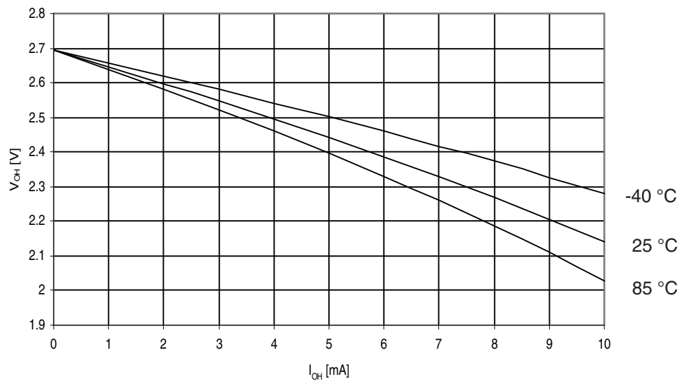
Figure 30-207. ATmega329PA: I/O Pin Output Voltage vs. Source Current, Ports A, C, D, E, F, G ( V_{CC} = 2.7V )
