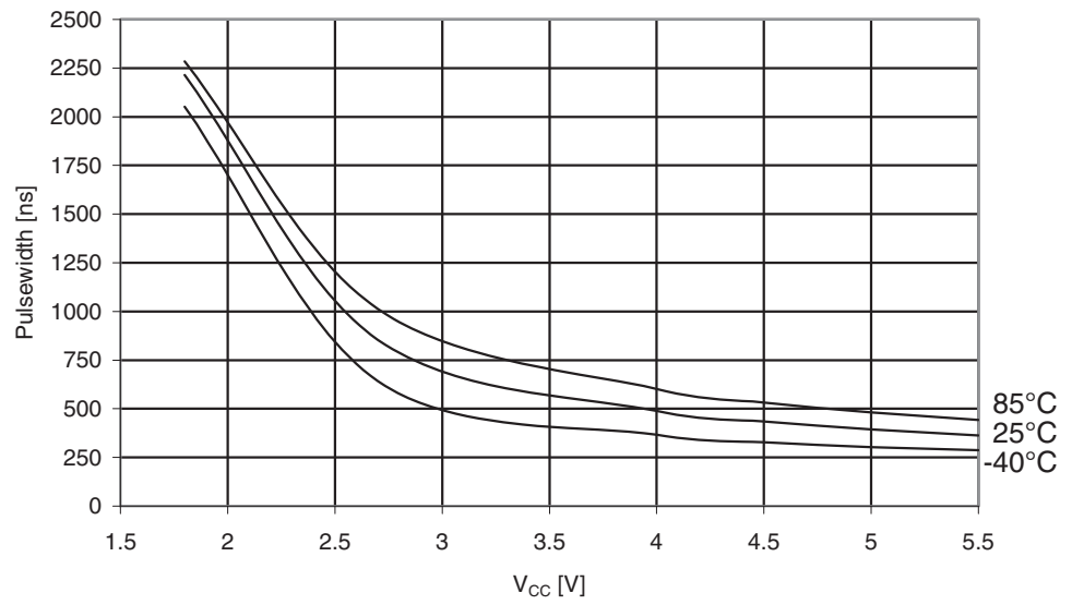
Figure 30-364. ATmega3290PA: Minimum Reset Pulse Width vs. V_{CC}
