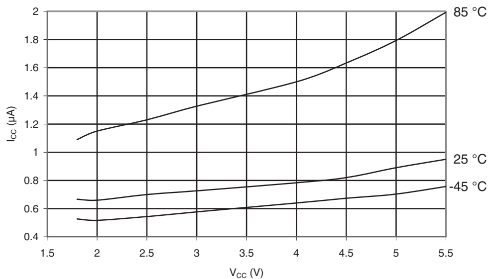
Figure 30-76. ATmega169PA: Standby Supply Current vs. V_{CC} (32kHz Watch Crystal, Watchdog Timer Disabled)
