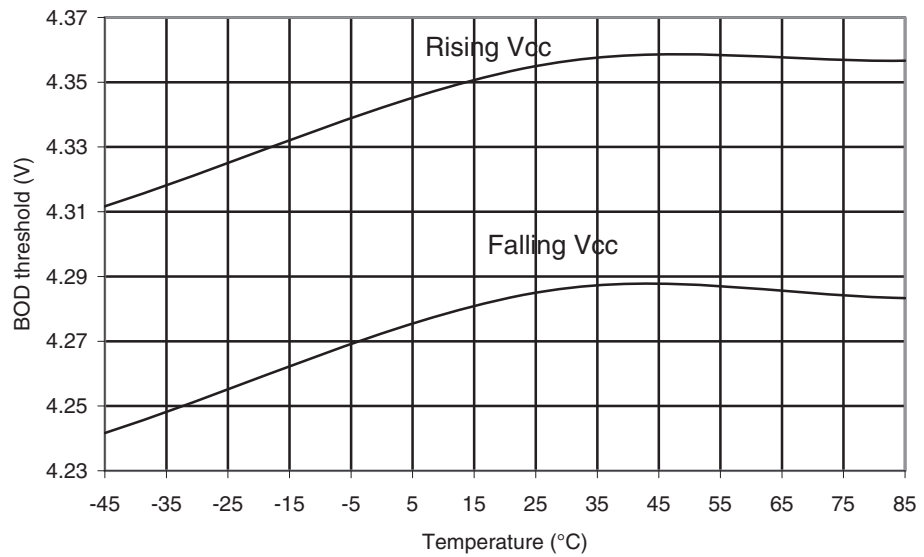
Figure 30-40. ATmega169A: BOD Thresholds vs. Temperature (BOD Level is 4.3V)
