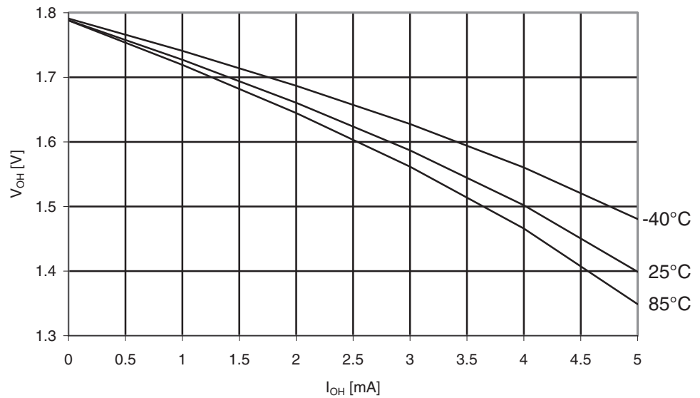
Figure 30-151. ATmega329A: I/O Pin Output Voltage vs. Source Current, Port B ( V_{CC} = 1.8V )
