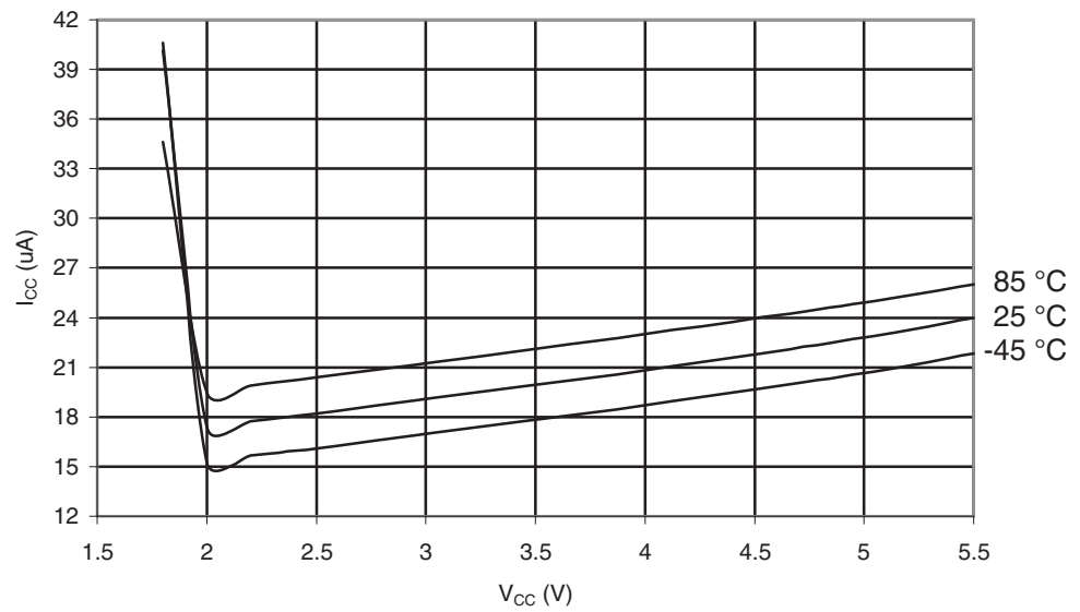
Figure 30-598. ATmega6490P: Brownout Detector Current vs. V_{CC}
