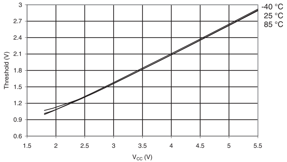
Figure 30-218. ATmega329PA: I/O Pin Input Threshold Voltage vs. V_{CC} ( V_{IH} , I/O Pin Read as "1")
