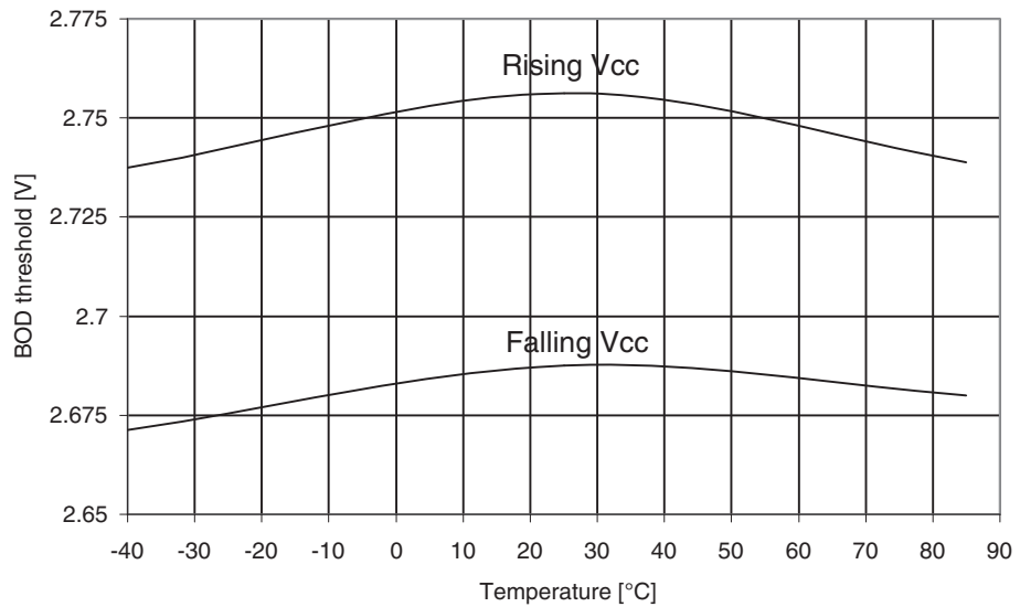
Figure 30-345. ATmega3290PA: BOD Thresholds vs. Temperature (BOD Level is 2.7V)
