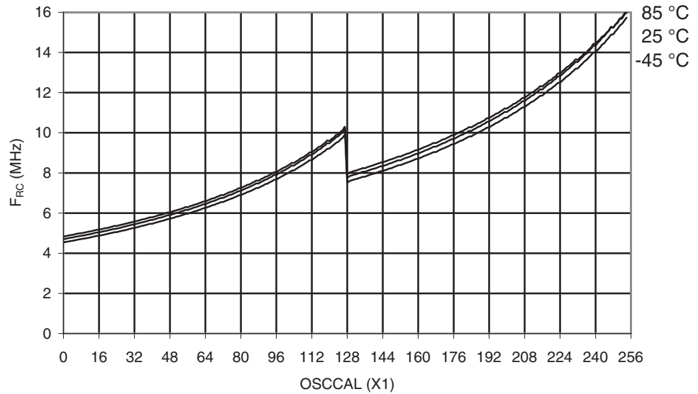
Figure 30-51. ATmega169A: Calibrated 8MHz RC Oscillator Frequency vs. Oscal Value
