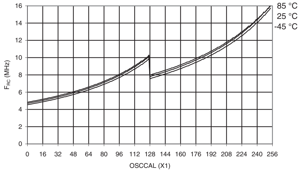
Figure 30-113. ATmega169PA: Calibrated 8MHz RC Oscillator Frequency vs. Oscscal Value
