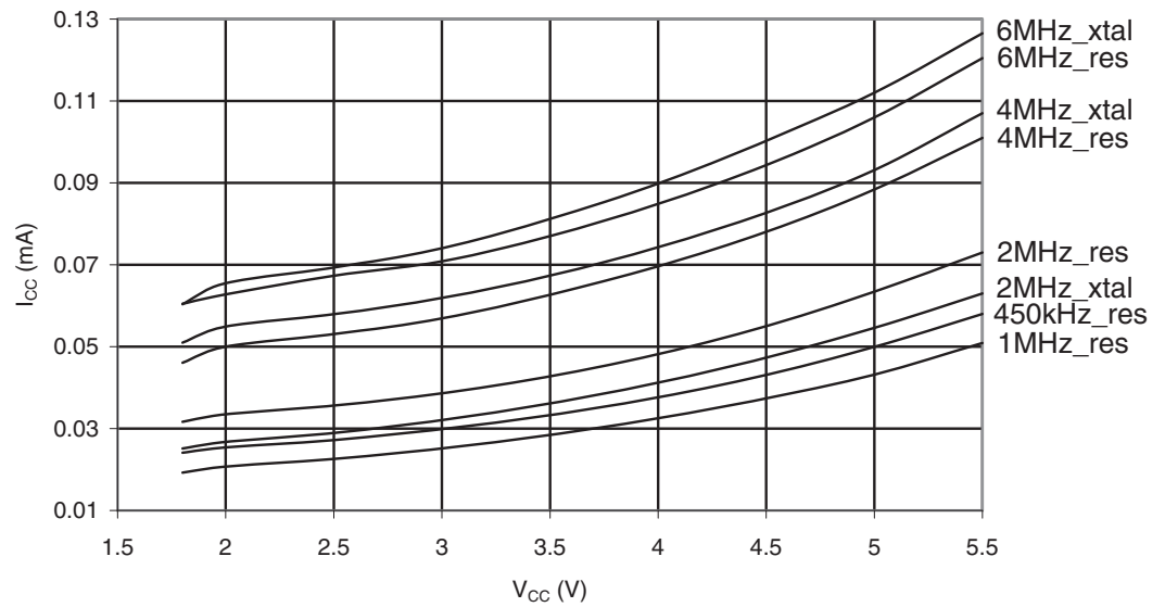
Figure 30-319. ATmega3290PA: Standby Supply Current vs. V_{CC} (Xtall and Resonator, Watchdog Timer Disabled)
