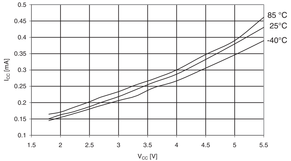
Figure 30-133. ATmega329A: Idle Supply Current vs. V_{CC} (Internal RC Oscillator, 1MHz)
