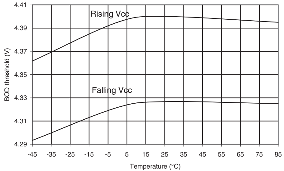
Figure 30-588. ATmega6490P: BOD Thresholds vs. Temperature (BOD Level is 4.3V)
