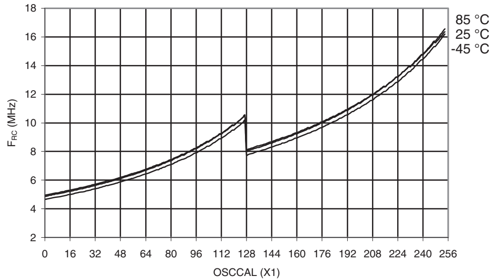
Figure 30-475. ATmega649P: Calibrated 8MHz RC Oscillator Frequency vs. OSCCAL Value
