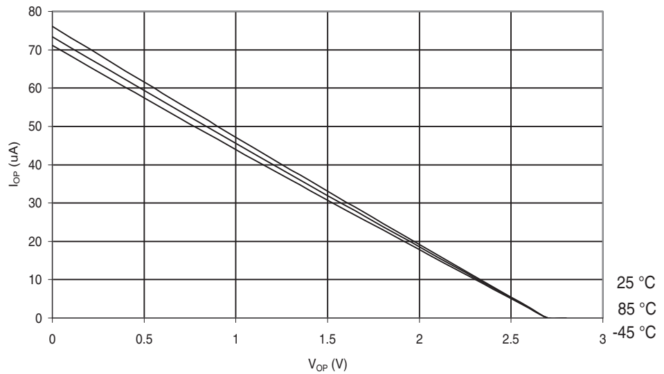
Figure 30-443. ATmega649P: I/O Pin Pull-up Resistor Current vs. Input Voltage ( V_{CC} = 2.7V )
