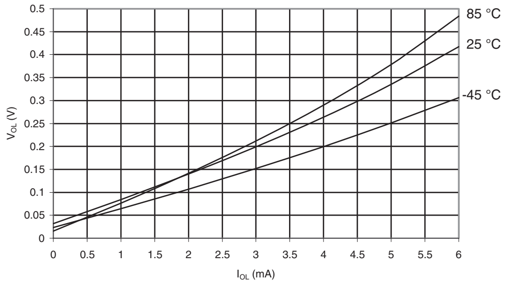
Figure 30-459. ATmega649P: I/O Pin Output Voltage vs. Sink Current, Port B ( V_{CC} = 1.8V )
