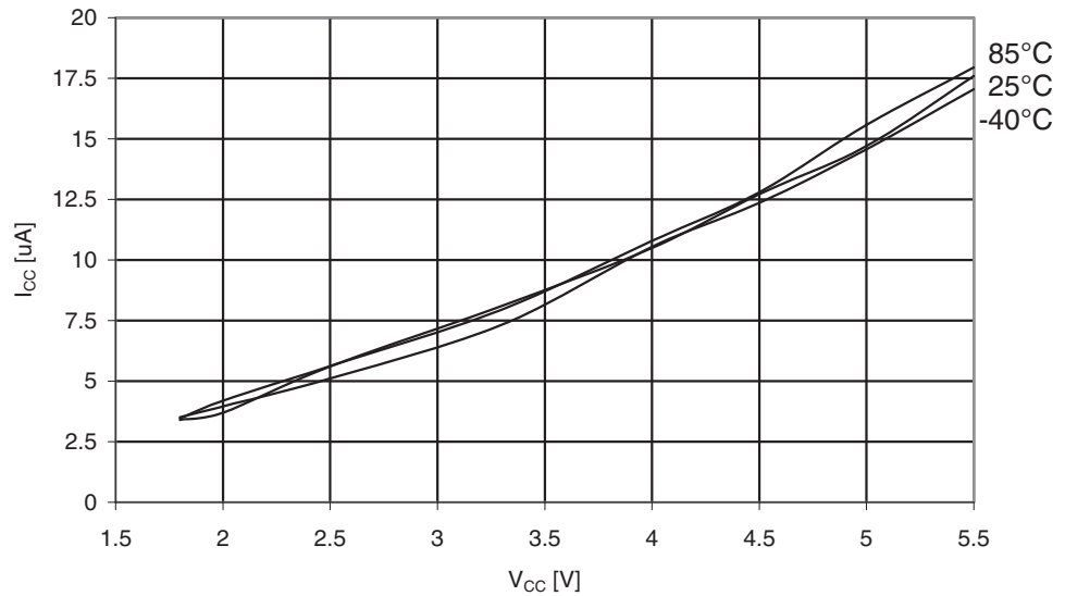
Figure 30-179. ATmega329A: Watchdog Timer Current vs. V_{CC}
