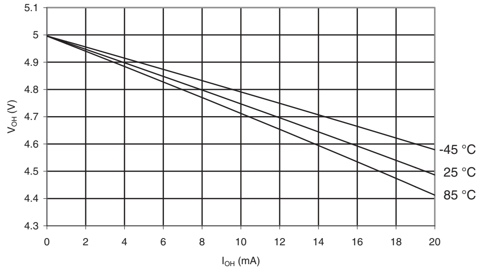
Figure 30-25. ATmega169A: I/O Pin Output Voltage vs. Source Current, Port B ( V_{CC} = 5V )
