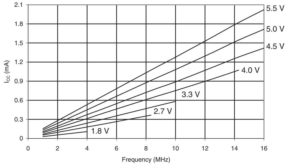
Figure 30-123. ATmega169PA: Reset Supply Current vs. V_{CC} (1 - 16MHz, Excluding Current Through The Reset Pull-up)
