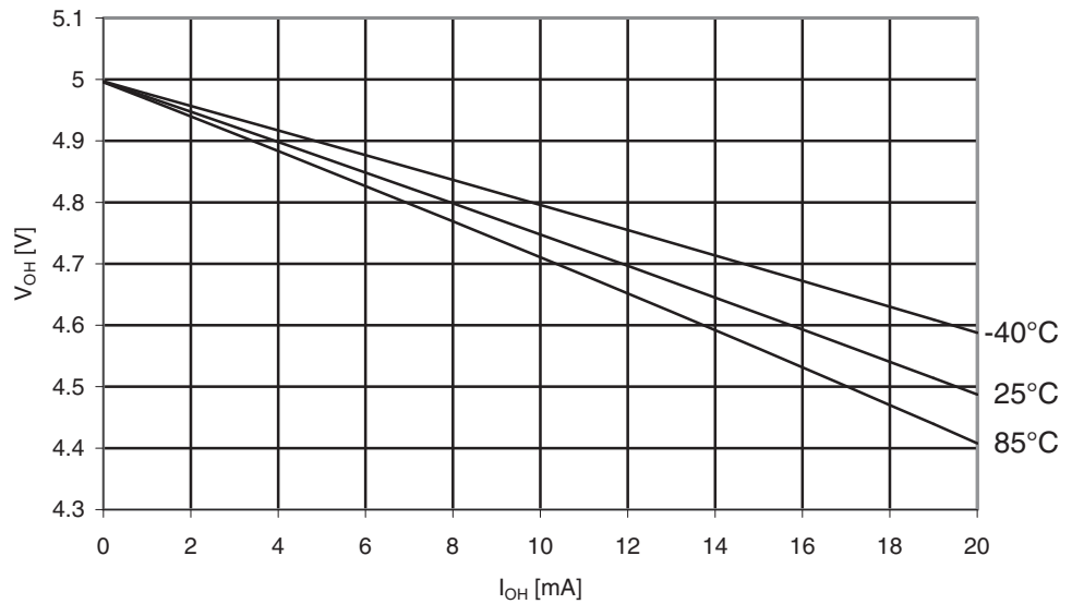
Figure 30-149. ATmega329A: I/O Pin Output Voltage vs. Source Current, Port B ( V_{CC} = 5V )
