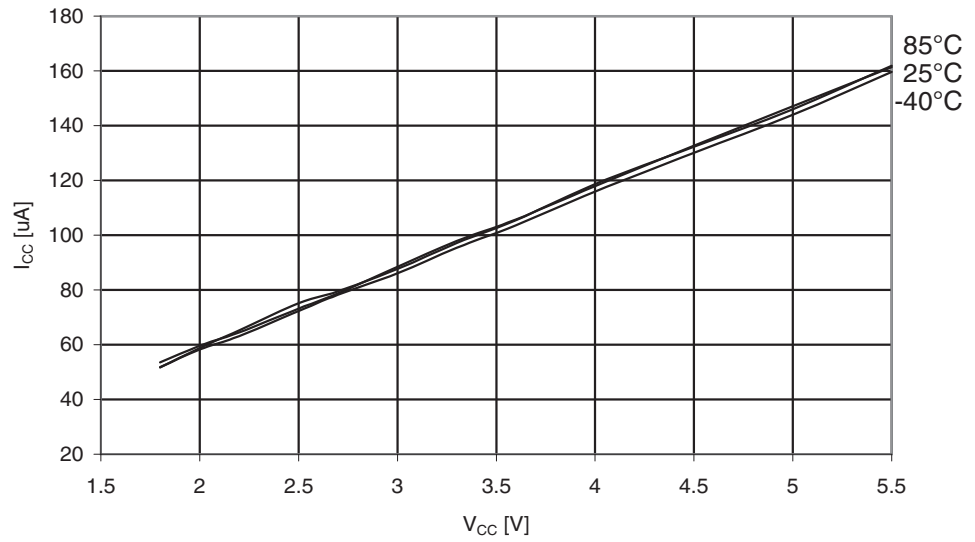
Figure 30-358. ATmega3290PA: AREF External Reference Current vs. V_{CC}
