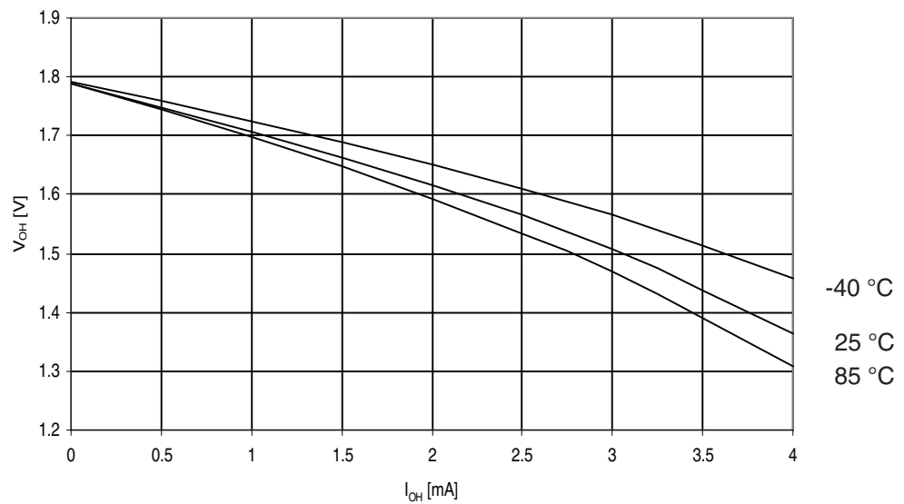
Figure 30-268. ATmega3290A: I/O Pin Output Voltage vs. Source Current, Ports A, C, D, E, F, G ( V_{CC} = 1.8V )
