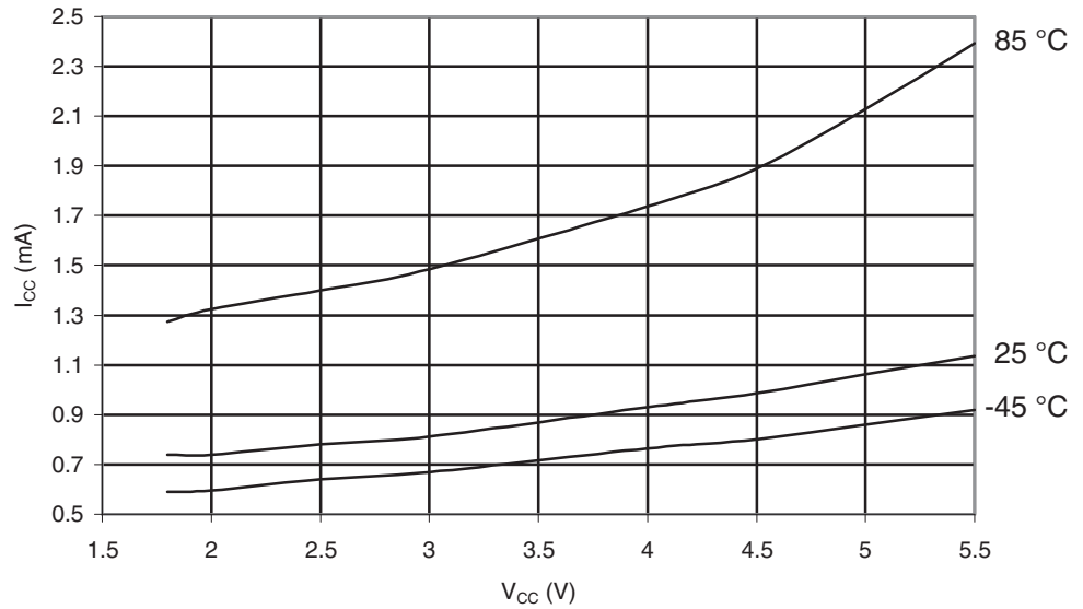
Figure 30-378. ATmega649A: Power-save Supply Current vs. V_{CC} (Watchdog Timer Disabled and 32kHz Crystal Oscillator Running)
