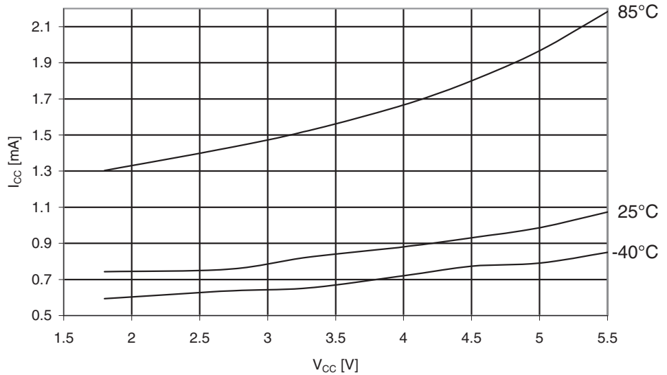
Figure 30-258. ATmega3290A: Standby Supply Current vs. V_{CC} (32kHz Watch Crystal, Watchdog Timer Disabled)
