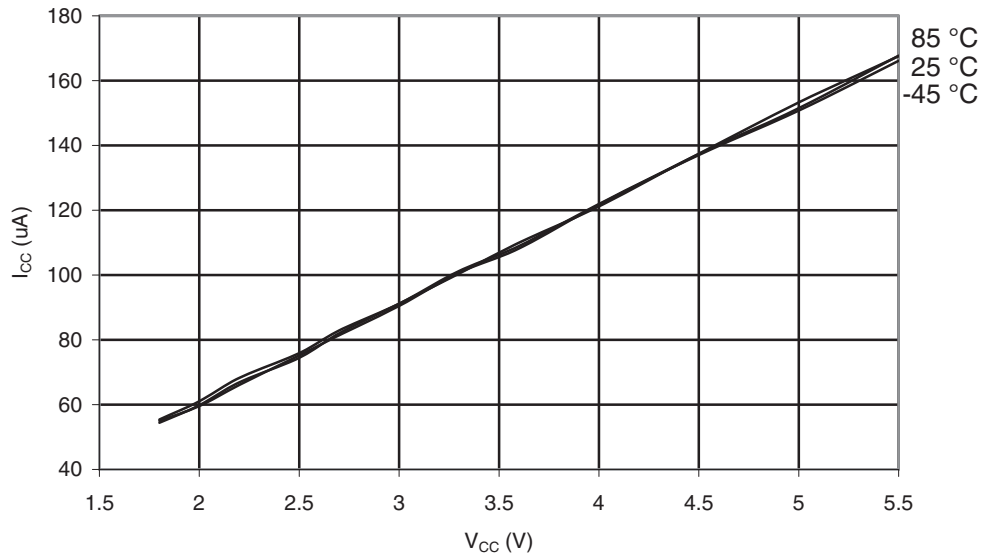
Figure 30-118. ATmega169PA: AREF External Reference Current vs. V_{CC}
