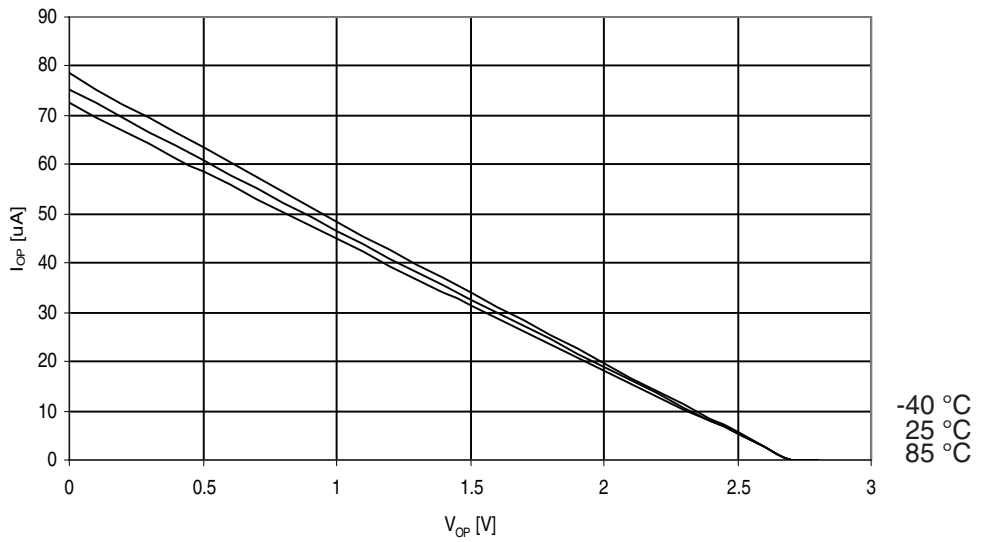
Figure 30-321. ATmega3290PA: I/O Pin Pull-up Resistor Current vs. Input Voltage ( V_{CC} = 2.7V )
