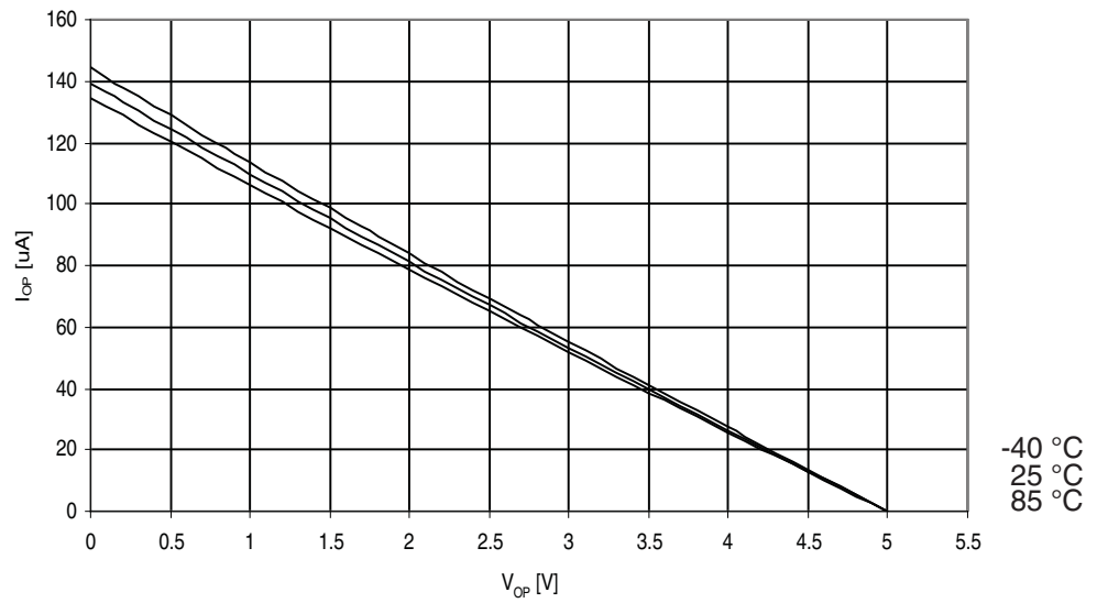
Figure 30-200. ATmega329PA: I/O Pin Pull-up Resistor Current vs. Input Voltage ( V_{CC} = 5V )
