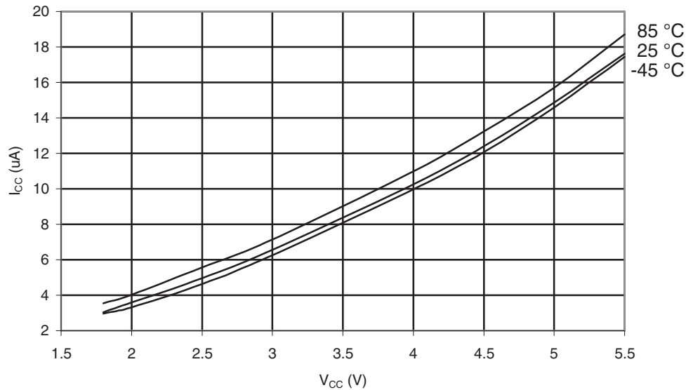
Figure 30-559. ATmega6490P: Power-down Supply Current vs. V_{CC} (Watchdog Timer Enabled)
