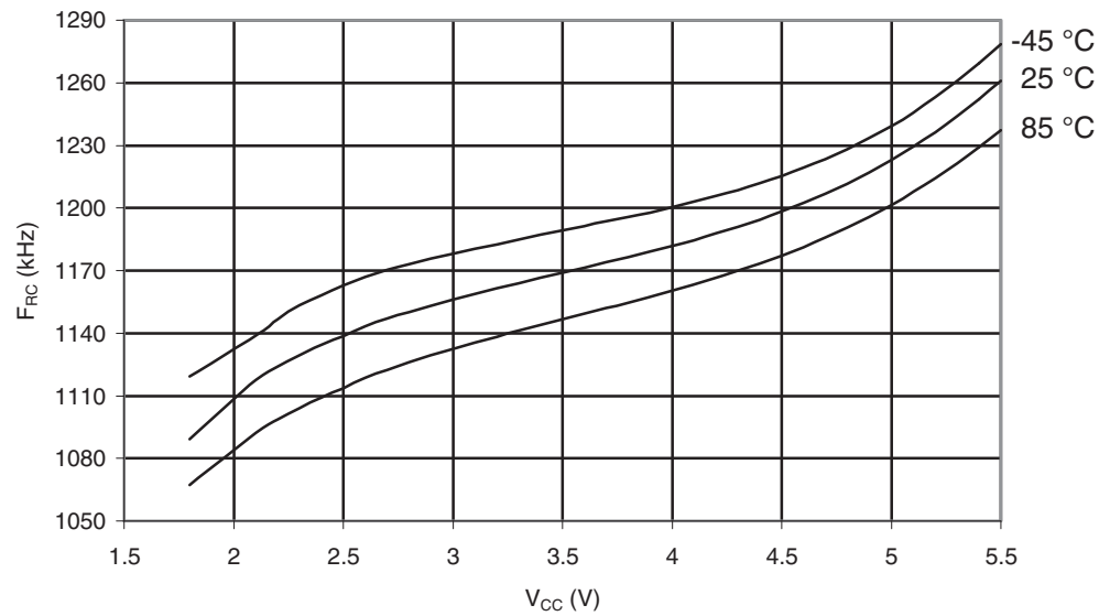
Figure 30-410. ATmega649A: Watchdog Oscillator Frequency vs. V_{CC}
