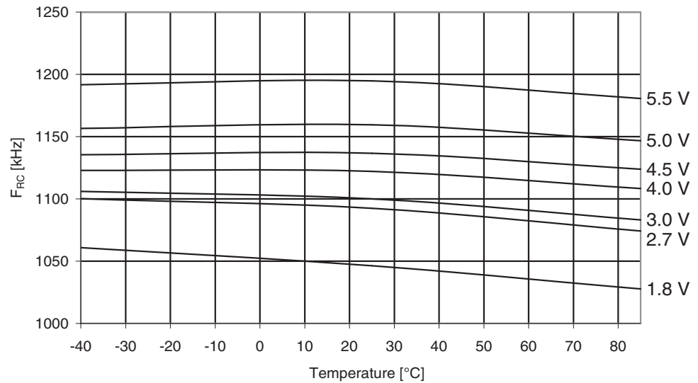
Figure 30-290. ATmega3290A: Watchdog Oscillator Frequency vs. Temperature
