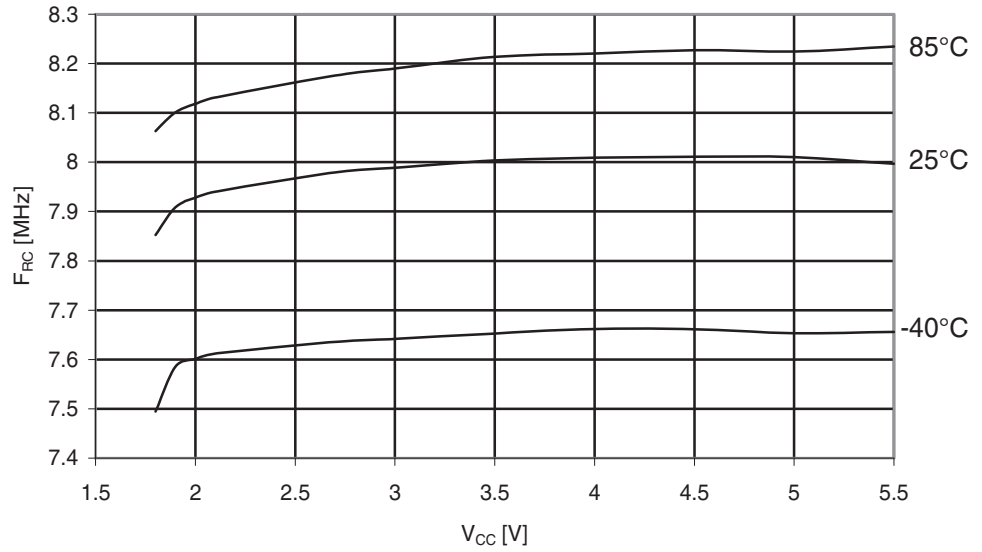
Figure 30-172. ATmega329A: Calibrated 8MHz RC Oscillator Frequency vs. V_{CC}
