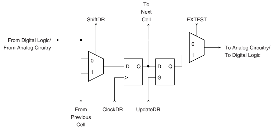
Figure 26-7. General Boundary-scan cell Used for Signals for Comparator and ADC
