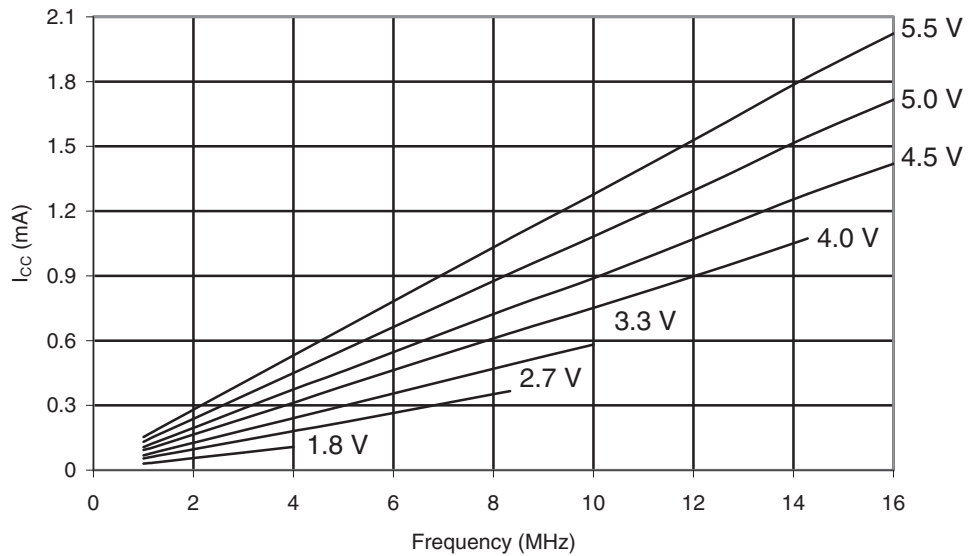
Figure 30-61. ATmega169A: Reset Supply Current vs. V_{CC} (1 - 16MHz, Excluding Current Through The Reset Pull-up)
