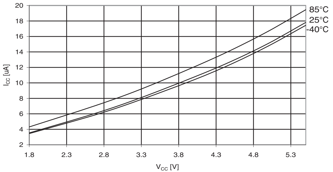
Figure 30-316. ATmega3290PA: Power-down Supply Current vs. V_{CC} (Watchdog Timer Enabled)
