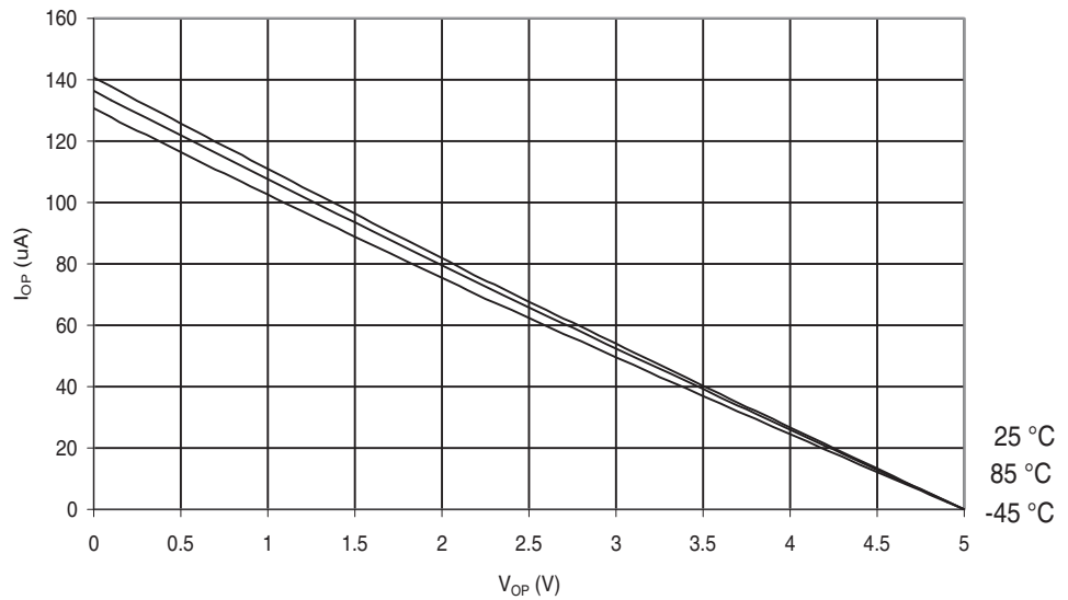
Figure 30-564. ATmega6490P: I/O Pin Pull-up Resistor Current vs. Input Voltage ( V_{CC} = 5V )
