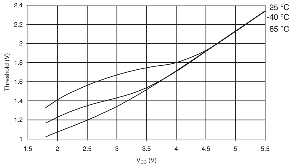
Figure 30-221. ATmega329PA: Reset Input Threshold Voltage vs. V_{CC} ( V_{IH} , Reset Pin Read as "1")
