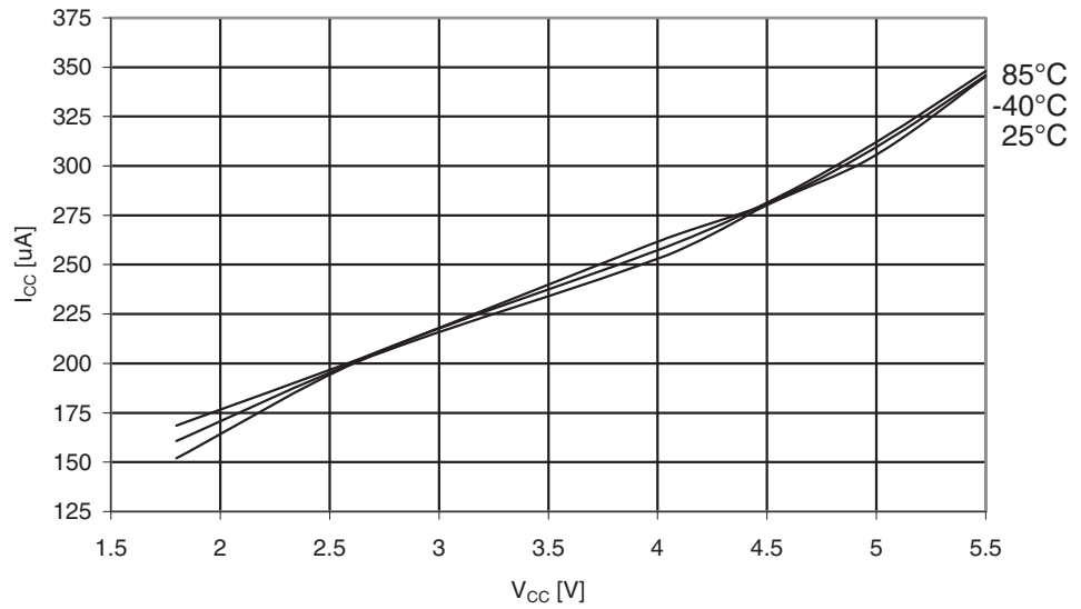
Figure 30-176. ATmega329A: Active Supply Current with ADC at 200kHz vs. V_{CC}
