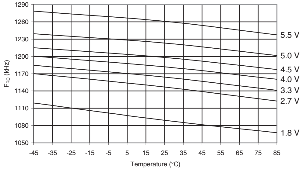
Figure 30-472. ATmega649P: Watchdog Oscillator Frequency vs. Temperature
