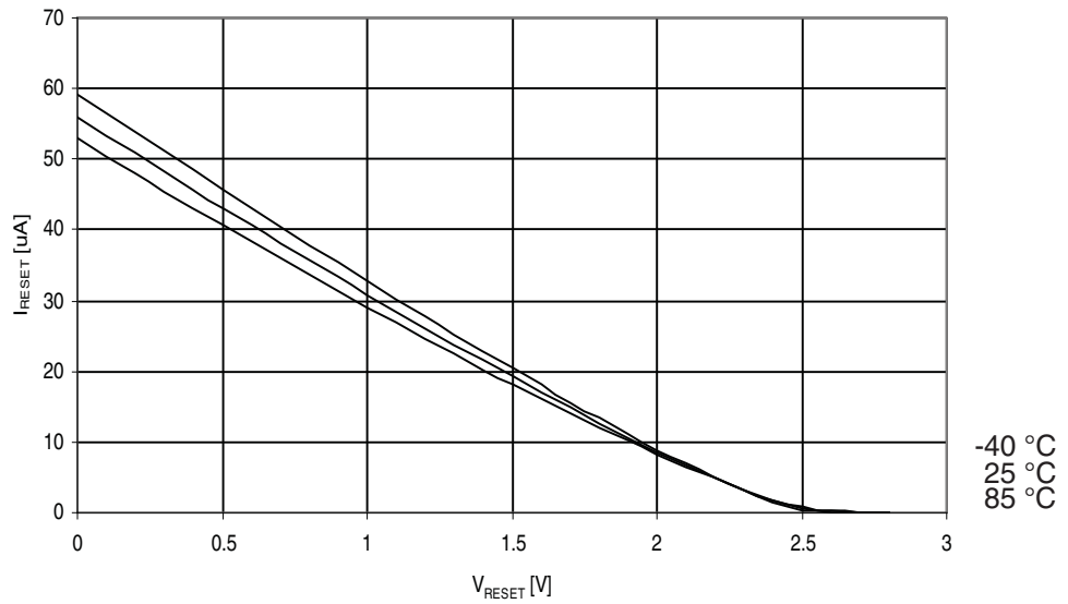
Figure 30-144. ATmega329A: Reset Pull-up Resistor Current vs. Reset Pin Voltage ( V_{CC} = 2.7V )
