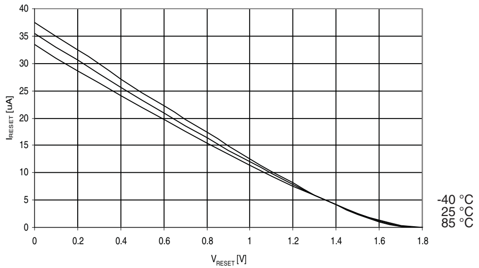
Figure 30-145. ATmega329A: Reset Pull-up Resistor Current vs. Reset Pin Voltage ( V_{CC} = 1.8V )
