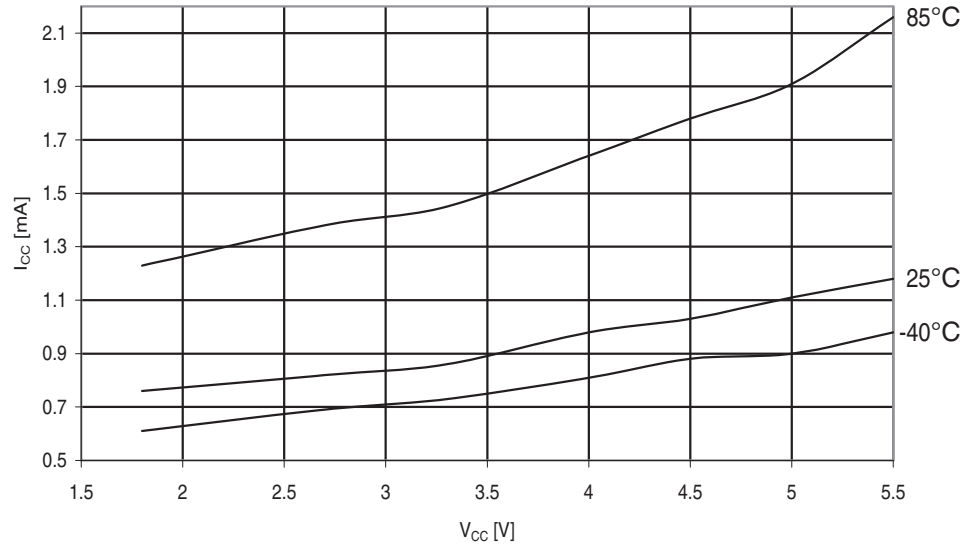
Figure 30-137. ATmega329A: Power-save Supply Current vs. V_{CC} (Watchdog Timer Disabled and 32kHz Crystal Oscillator Running)
