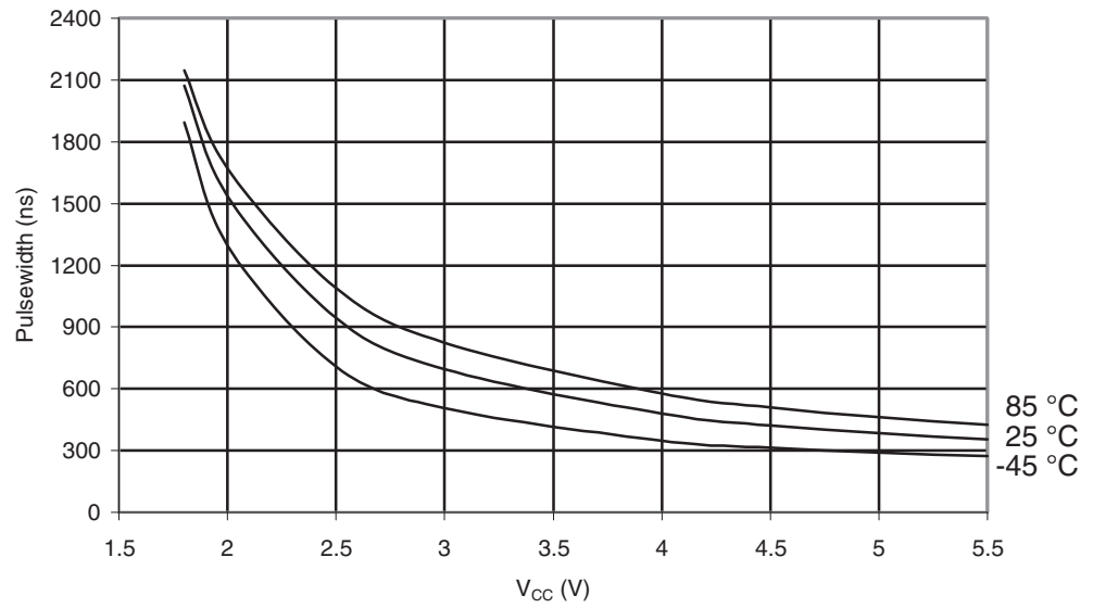
Figure 30-547. ATmega6490A: Minimum Reset Pulse Width vs. V_{CC}
