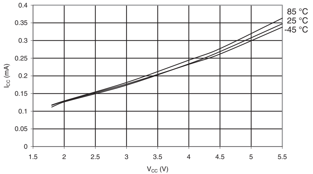
Figure 30-9. ATmega169A: Idle Supply Current vs. V_{CC} (Internal RC Oscillator, 1MHz)
