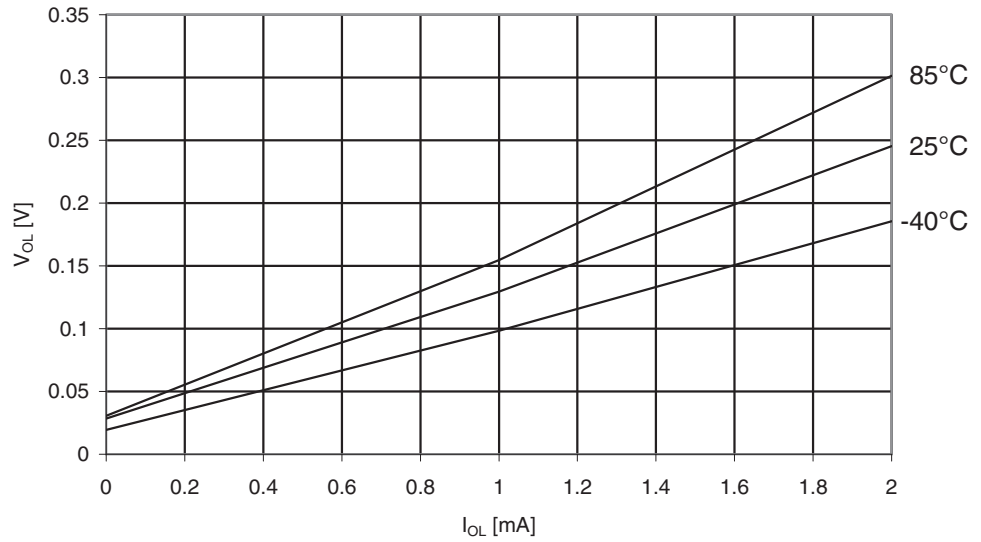
Figure 30-154. ATmega329A: I/O Pin Output Voltage vs. Sink Current, Ports A, C, D, E, F, G ( V_{CC} = 1.8V )
