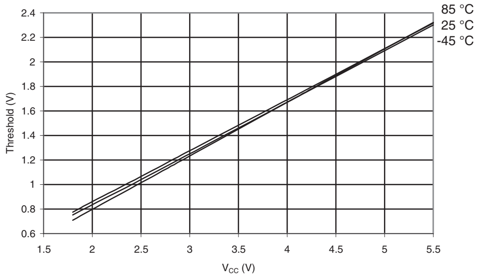
Figure 30-464. ATmega649P: Reset Input Threshold Voltage vs. V_{CC} ( V_{IL} , Reset Pin Read as "0")
