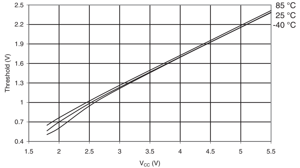
Figure 30-159. ATmega329A: I/O Pin Input Threshold Voltage vs. V_{CC} ( V_{IL} , I/O Pin Read as “0”)
