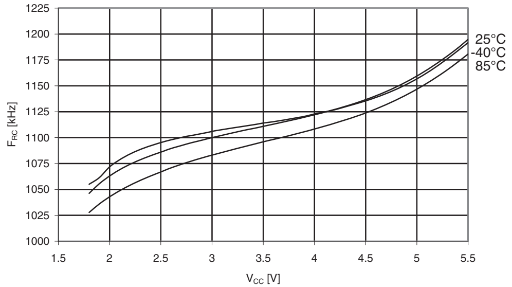
Figure 30-349. ATmega3290PA: Watchdog Oscillator Frequency vs. V_{CC}
