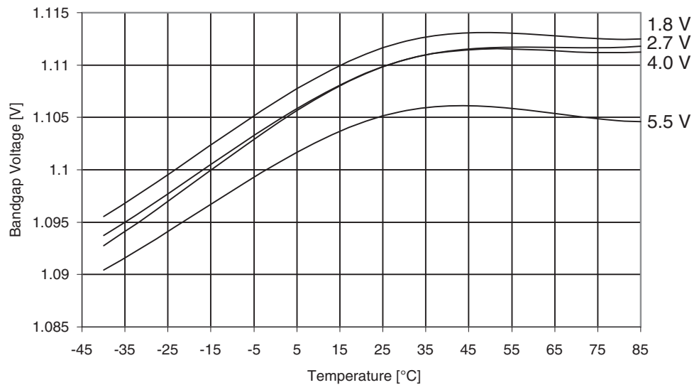
Figure 30-288. ATmega3290A: Bandgap Voltage vs. Temperature
