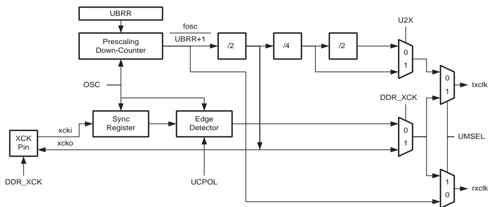
Figure 20-2. Clock Generation Logic, Block Diagram
