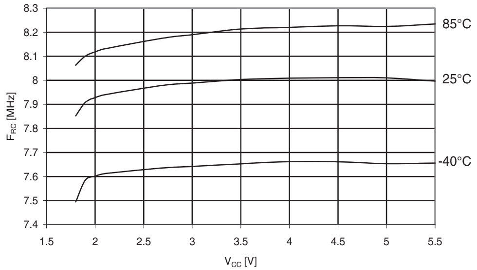
Figure 30-352. ATmega3290PA: Calibrated 8MHz RC Oscillator Frequency vs. V_{CC}
