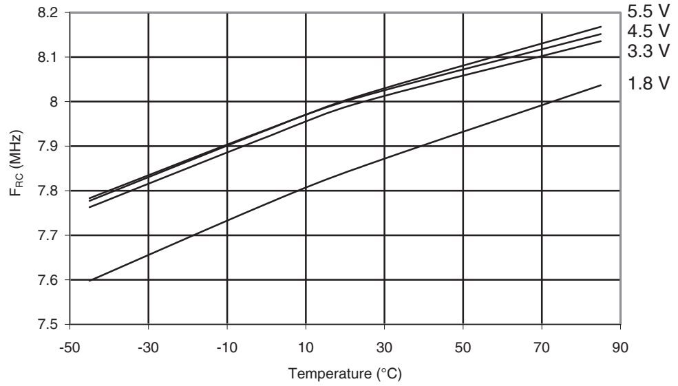
Figure 30-111. ATmega169PA: Calibrated 8MHz RC Oscillator Frequency vs. Temperature
