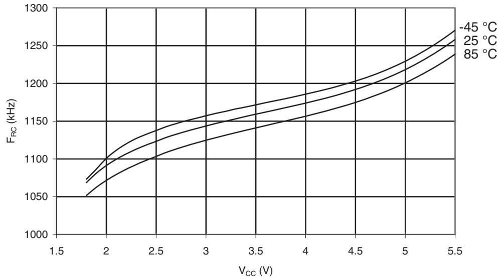
Figure 30-109. ATmega169PA: Watchdog Oscillator Frequency vs. V_{CC}
