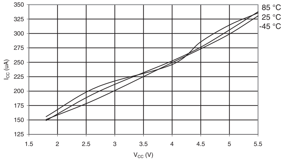
Figure 30-117. ATmega169PA: Active Supply Current with ADC at 1MHz vs. V_{CC}
