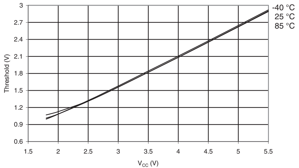
Figure 30-278. ATmega3290A: I/O Pin Input Threshold Voltage vs. V_{CC} ( V_{IH} , I/O Pin Read as "1")
