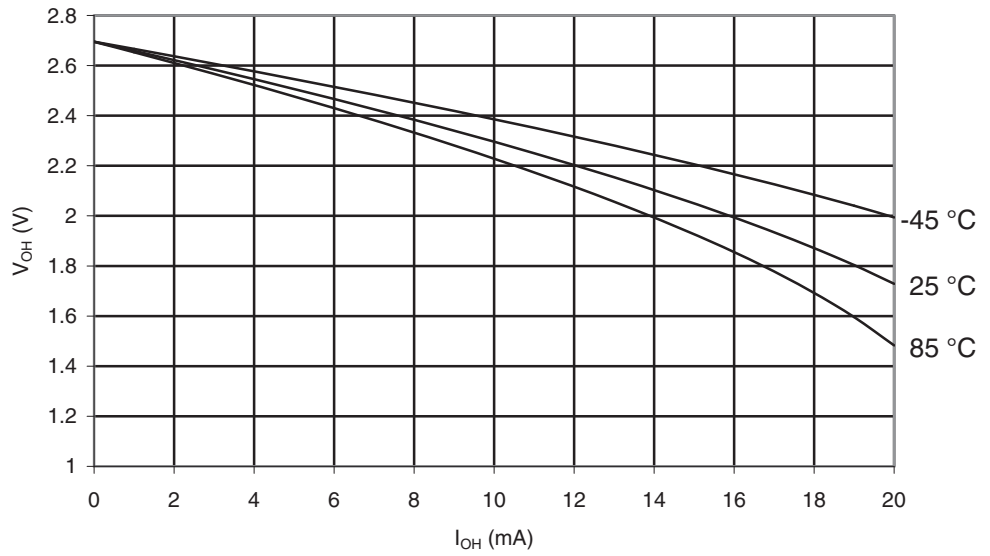
Figure 30-26. ATmega169A: I/O Pin Output Voltage vs. Source Current, Port B ( V_{CC} = 2.7V )
