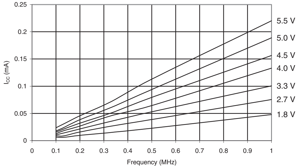
Figure 30-6. ATmega169A: Idle Supply Current vs.Low Frequency (0.1 - 1.0MHz)
