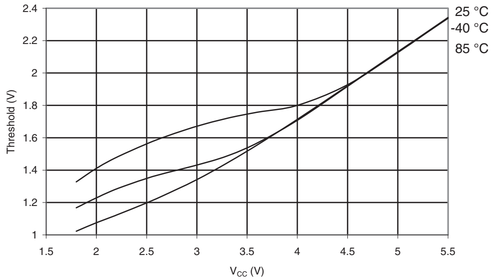
Figure 30-341. ATmega3290PA: Reset Input Threshold Voltage vs. V_{CC} ( V_{IH,Reset} Pin Read as "1")
