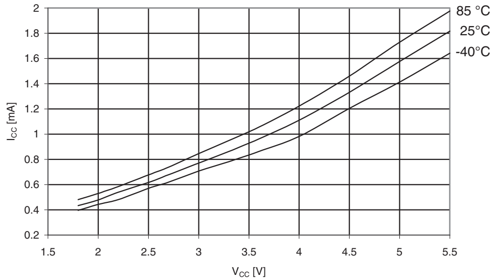
Figure 30-312. ATmega3290PA: Idle Supply Current vs. V_{CC} (Internal RC Oscillator, 8MHz)
