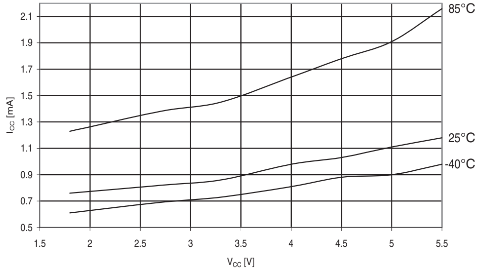
Figure 30-257. ATmega3290A: Power-save Supply Current vs. V_{CC} (Watchdog Timer Disabled and 32kHz Crystal Oscillator Running)
