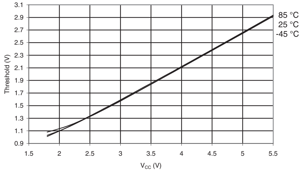
Figure 30-34. ATmega169A: I/O Pin Input Threshold Voltage vs. V_{CC} ( V_{IH} , I/O Pin Read as “1”)
