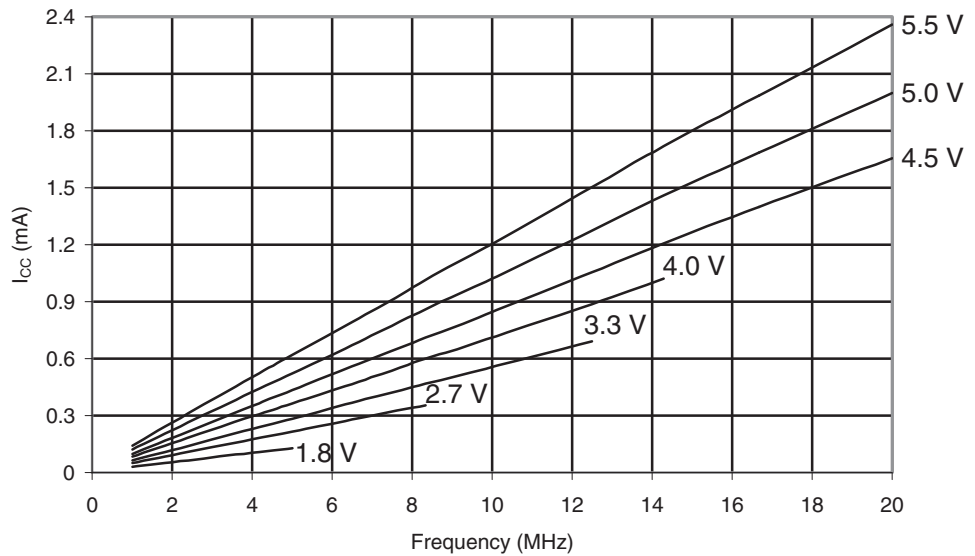
Figure 30-424. ATmega649A: Reset Supply Current vs. V_{CC} (1 - 20MHz, Excluding Current Through The Reset Pull-up)
