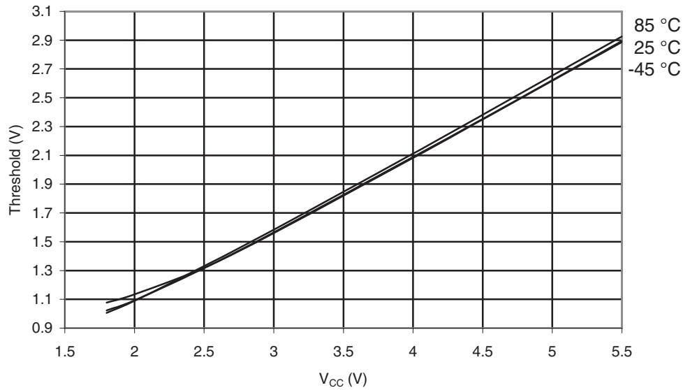
Figure 30-582. ATmega6490P: I/O Pin Input Threshold Voltage vs. V_{CC} ( V_{IH} , I/O Pin Read as "1")
