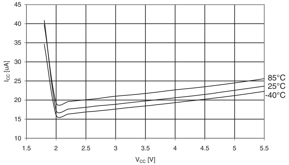
Figure 30-234. ATmega329PA: Brownout Detector Current vs. V_{CC}
