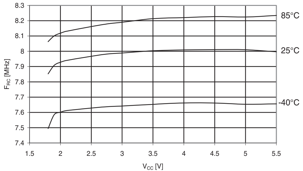
Figure 30-292. ATmega3290A: Calibrated 8MHz RC Oscillator Frequency vs. V CC
