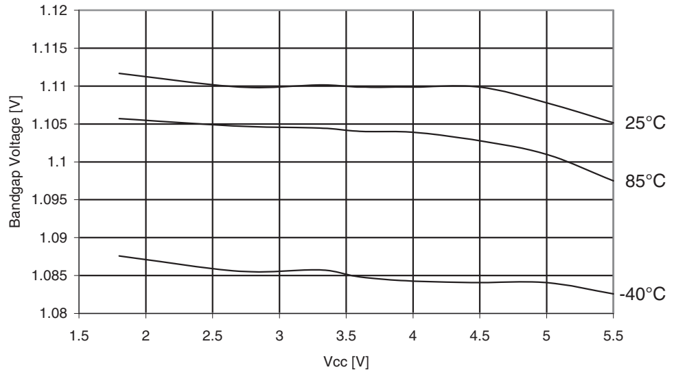
Figure 30-287. ATmega3290A: Bandgap Voltage vs. V_{CC}
