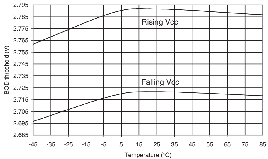
Figure 30-406. ATmega649A: BOD Thresholds vs. Temperature (BOD Level is 2.7V)
