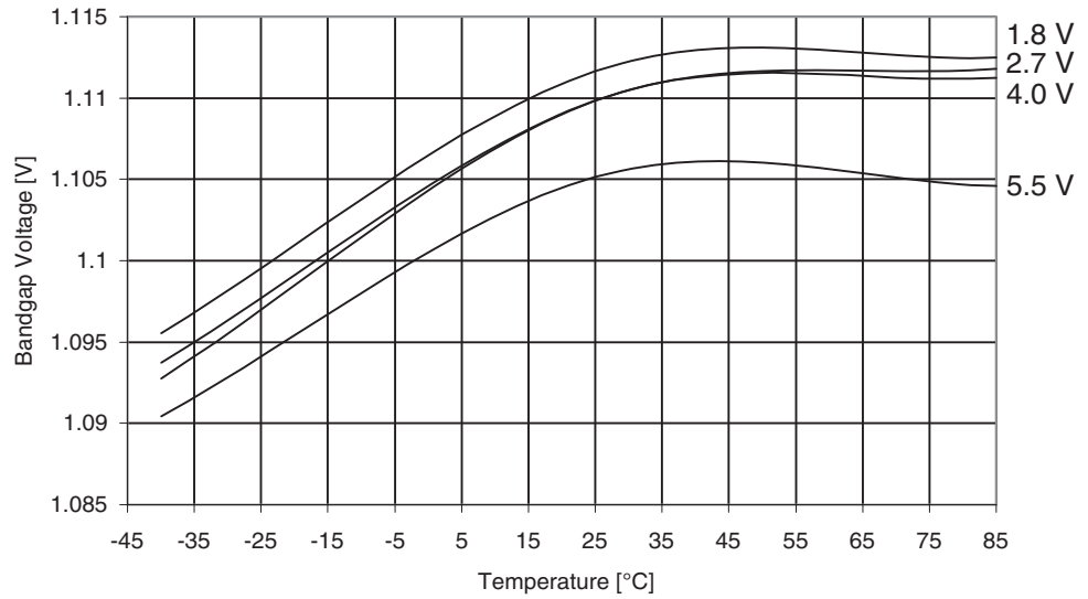
Figure 30-168. ATmega329A: Bandgap Voltage vs. Temperature
