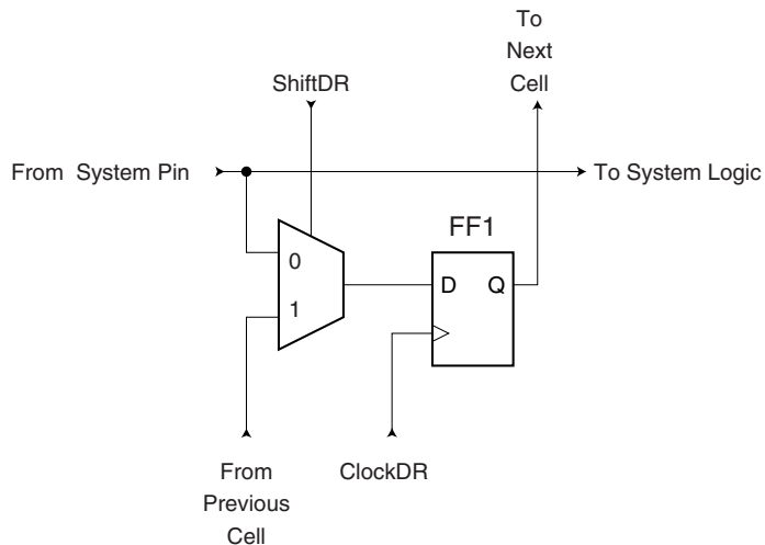
Figure 26-4. Observe-only Cell
