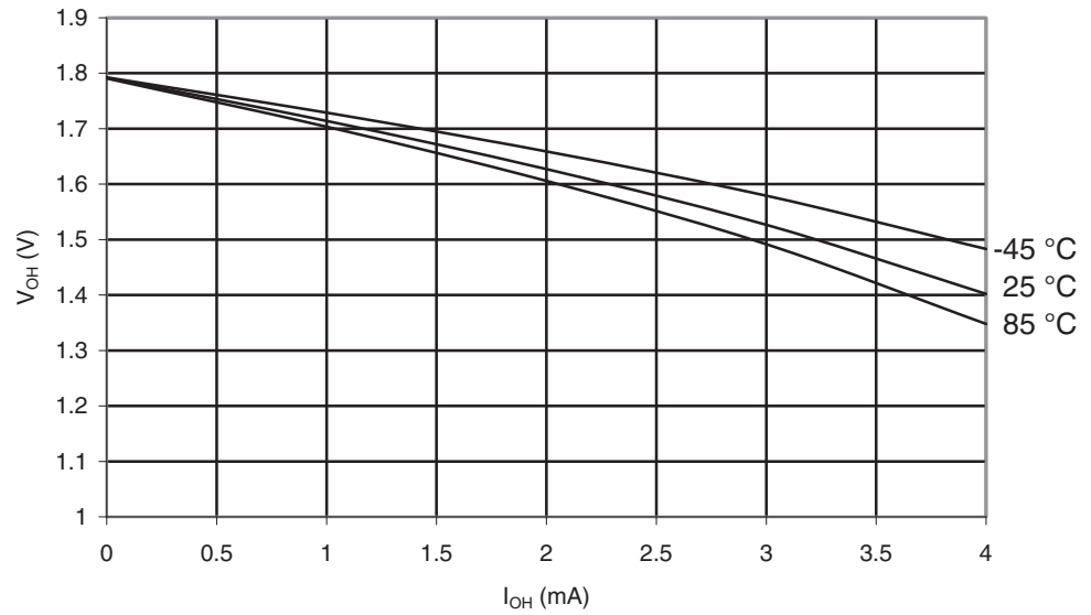
Figure 30-24. ATmega169A: I/O Pin Output Voltage vs. Source Current, Ports A, C, D, E, F, G ( V_{CC} = 1.8V )
