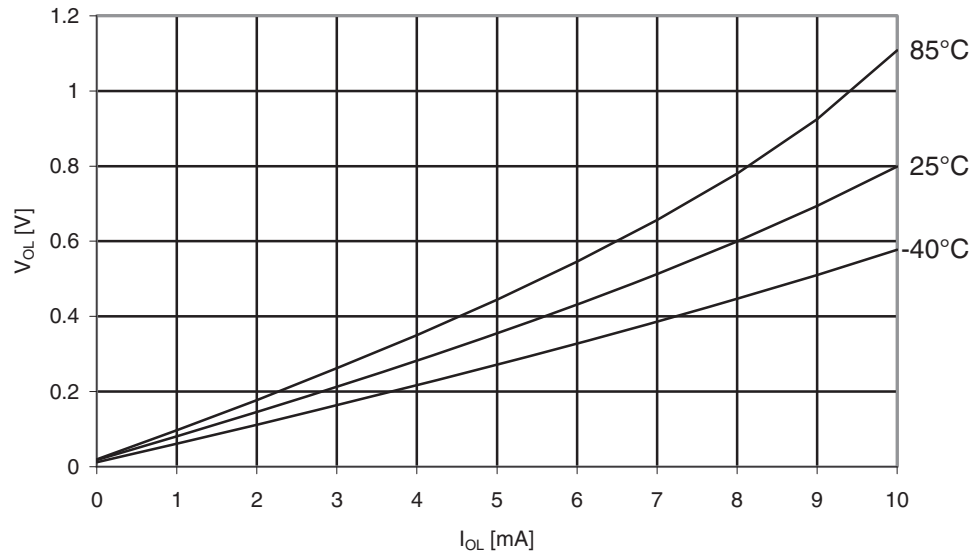
Figure 30-213. ATmega329PA: I/O Pin Output Voltage vs. Sink Current, Ports A, C, D, E, F, G ( V_{CC} = 2.7V )
