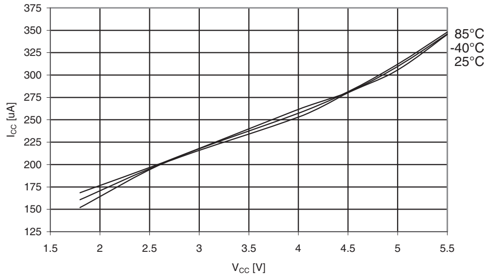
Figure 30-296. ATmega3290A: Active Supply Current with ADC at 200kHz vs. V_{CC}
