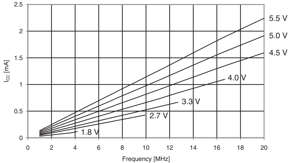
Figure 30-183. ATmega329A: Reset Supply Current vs. V_{CC} (1 - 20MHz, Excluding Current Through The Reset Pull-up)
