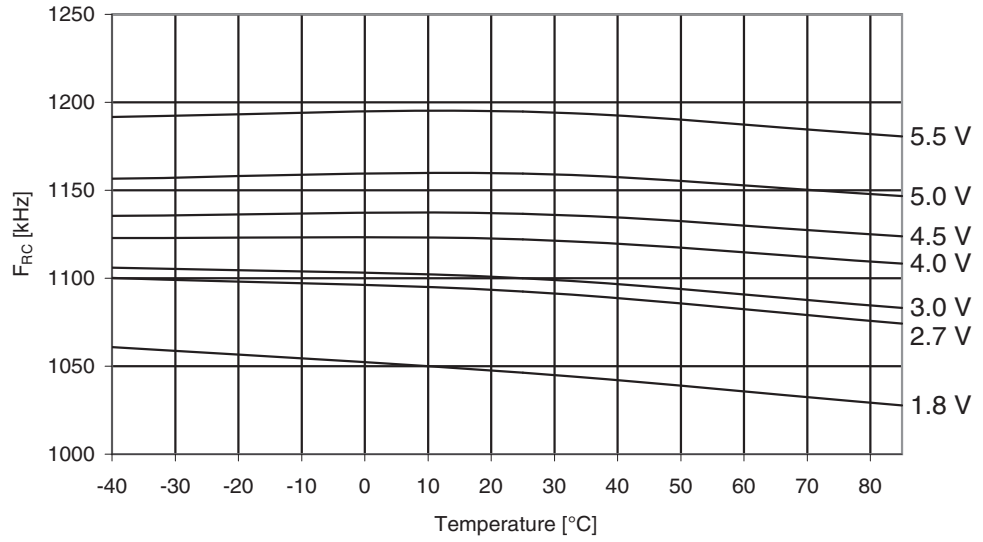
Figure 30-230. ATmega329PA: Watchdog Oscillator Frequency vs. Temperature
