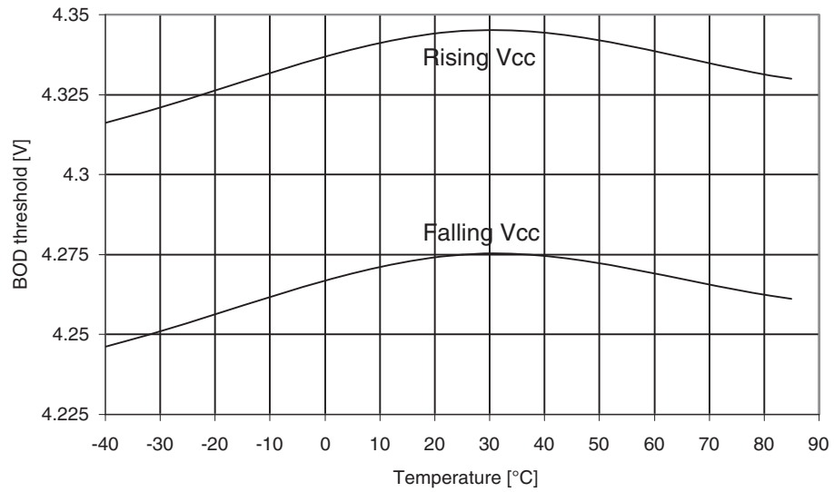
Figure 30-344. ATmega3290PA: BOD Thresholds vs. Temperature (BOD Level is 4.3V)
