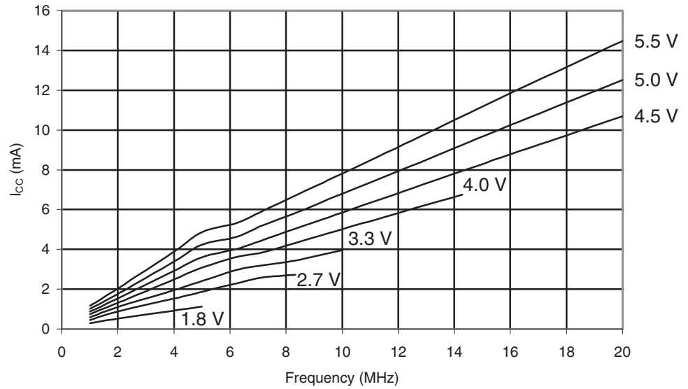
Figure 30-554. ATmega6490P: Idle Supply Current vs. Frequency (1 - 20MHz)
