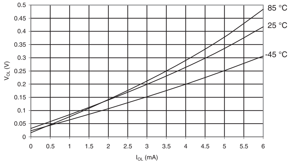
Figure 30-581. ATmega6490P: I/O Pin Output Voltage vs. Sink Current, Port B ( V_{CC} = 1.8V )
