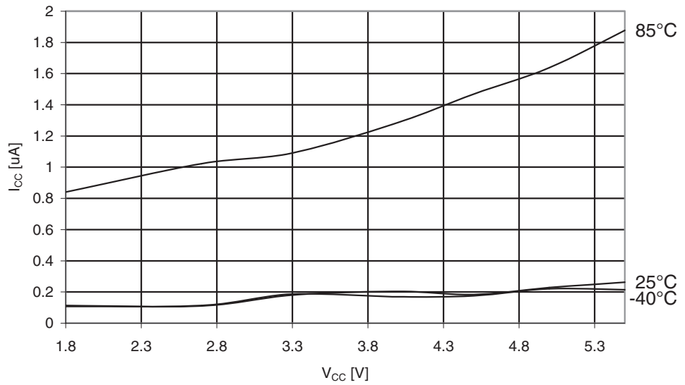
Figure 30-136. ATmega329A: Power-down Supply Current vs. V_{CC} (Watchdog Timer Enabled)
