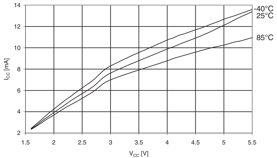
Figure 30-361. ATmega3290PA: Programming Current vs. V_{CC}
