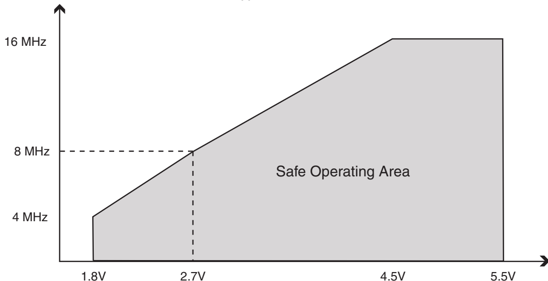
Figure 29-1. Maximum Frequency vs. V_{CC} : ATmega169A/169PA/ATmega649A/ATmega649P
