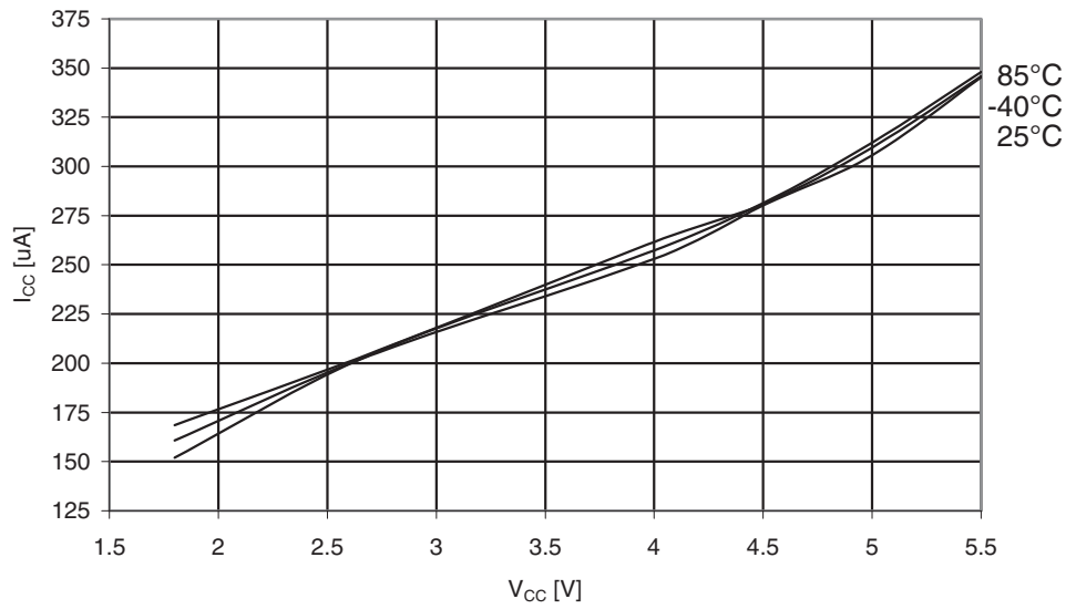
Figure 30-236. ATmega329PA: Active Supply Current with ADC at 200kHz vs. V_{CC}
