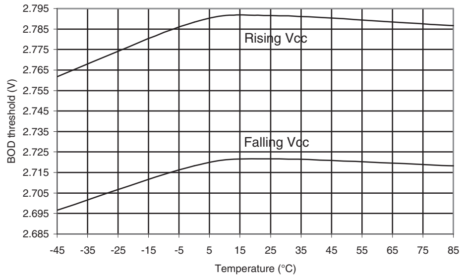
Figure 30-467. ATmega649P: BOD Thresholds vs. Temperature (BOD Level is 2.7V)
