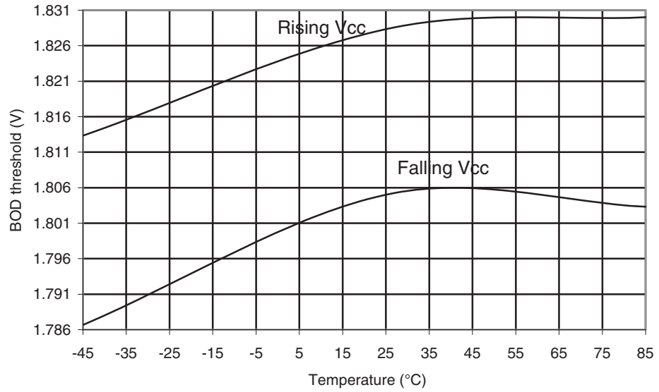
Figure 30-42. ATmega169A: BOD Thresholds vs. Temperature (BOD Level is 1.8V)
