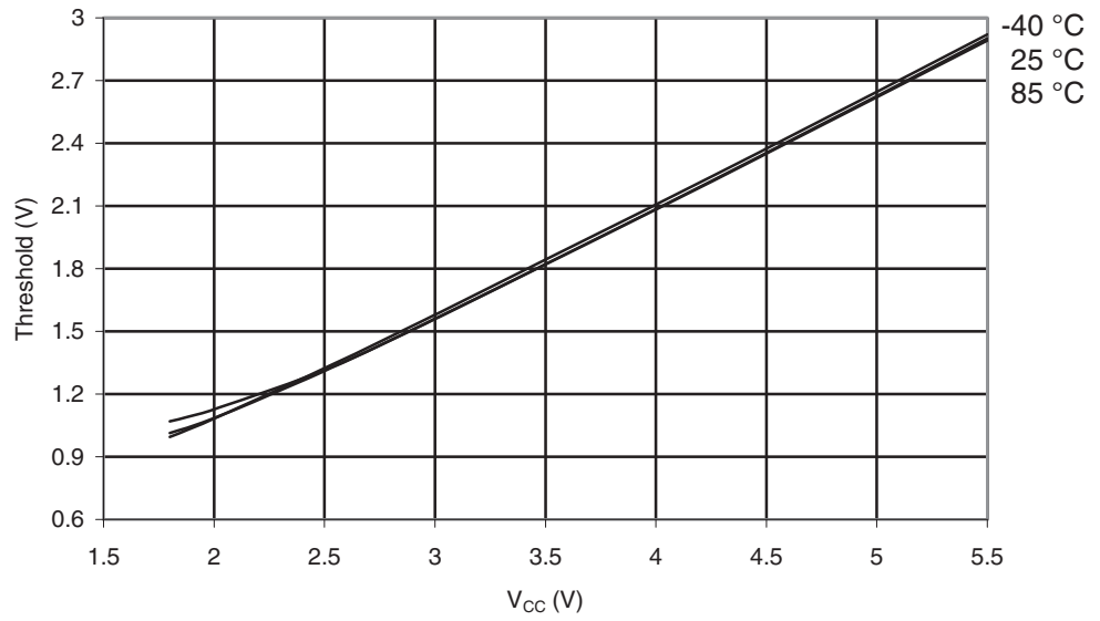
Figure 30-158. ATmega329A: I/O Pin Input Threshold Voltage vs. V_{CC} ( V_{IH} , I/O Pin Read as “1”)
