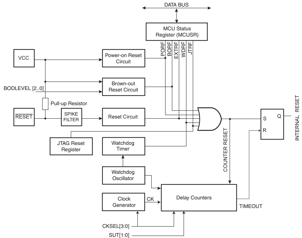
Figure 11-1. Reset Logic
