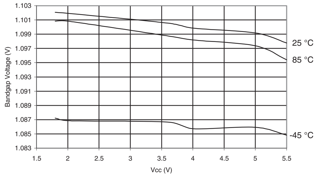
Figure 30-530. ATmega6490A: Bandgap Voltage vs. V_{CC}
