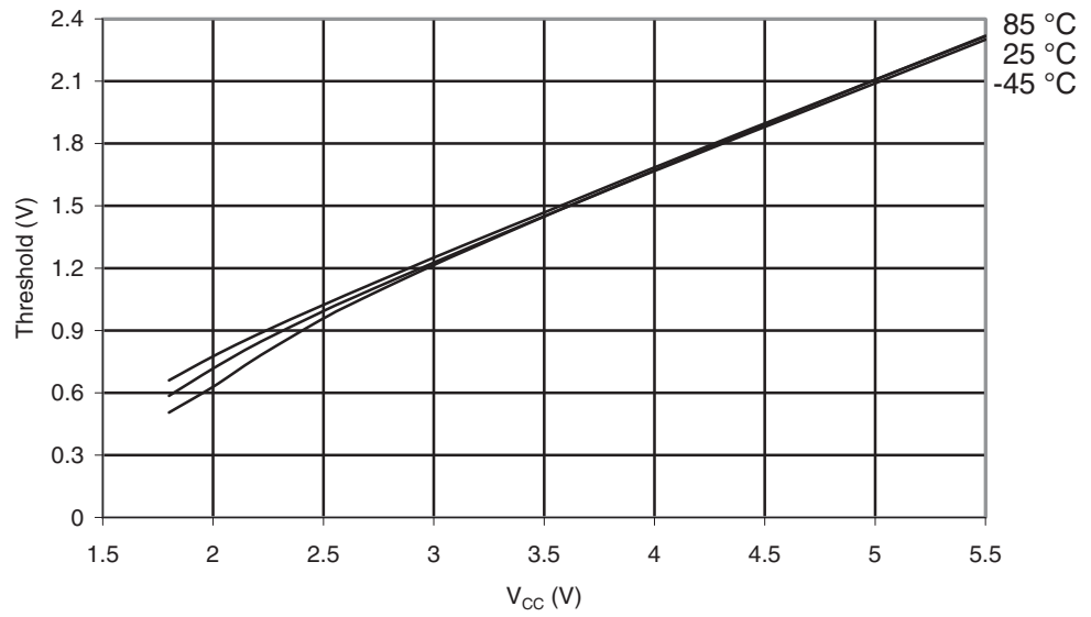
Figure 30-35. ATmega169A: I/O Pin Input Threshold Voltage vs. V_{CC} ( V_{IL} , I/O Pin Read as “0”)
