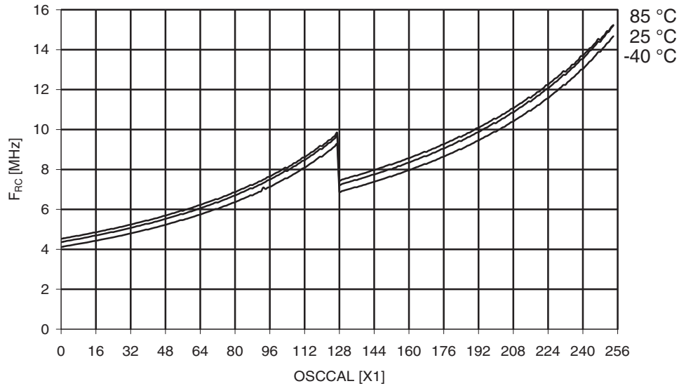
Figure 30-353. ATmega3290PA: Calibrated 8MHz RC Oscillator Frequency vs. Oscal Value
