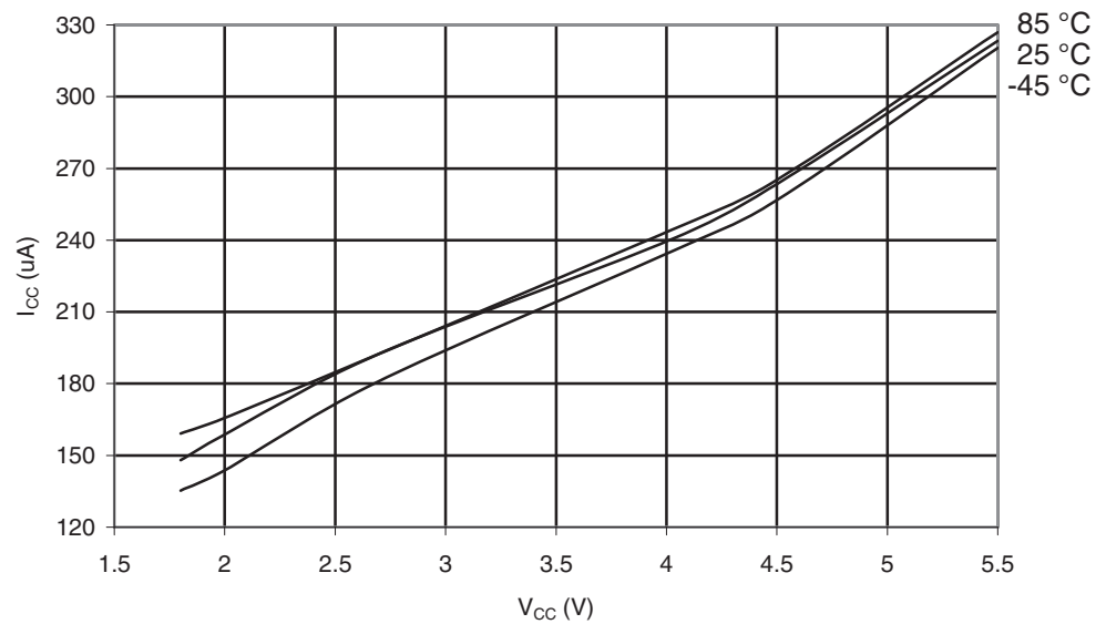
Figure 30-599. ATmega6490P: Active Supply Current with ADC at 50kHz vs. V_{CC}
