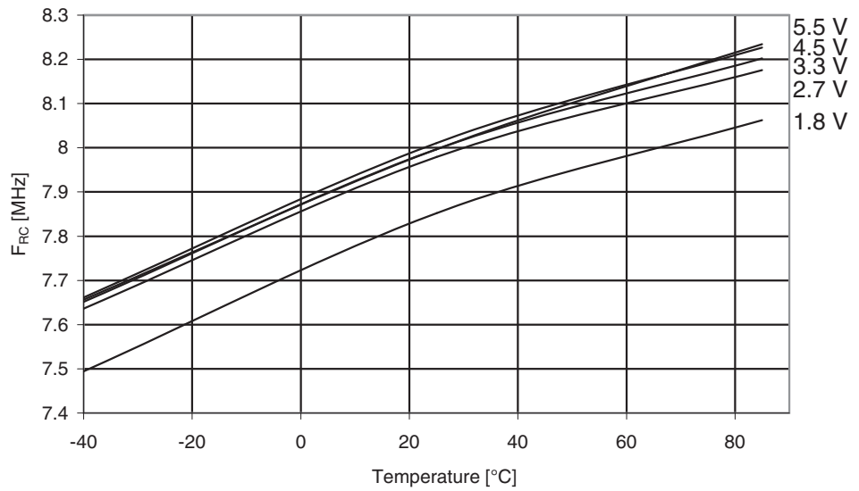
Figure 30-291. ATmega3290A: Calibrated 8MHz RC Oscillator Frequency vs. Temperature
