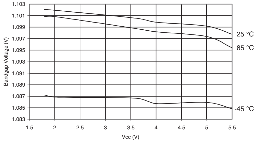
Figure 30-408. ATmega649A: Bandgap Voltage vs. V CC
