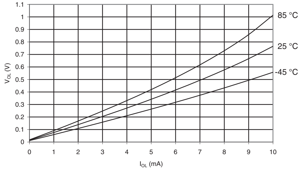
Figure 30-28. ATmega169A: I/O Pin Output Voltage vs. Sink Current, Ports A, C, D, E, F, G ( V_{CC} = 5V )
