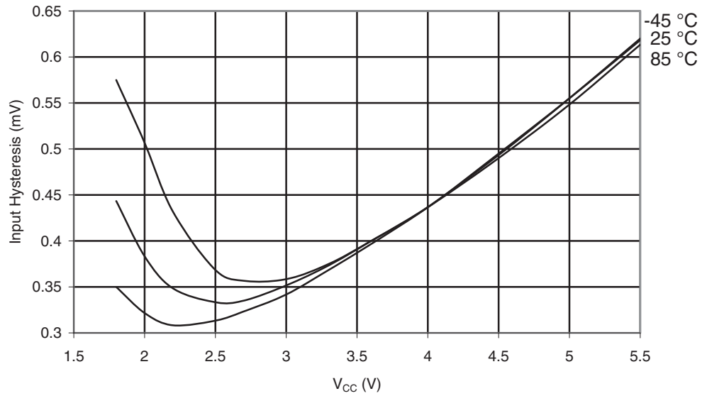
Figure 30-36. ATmega169A: I/O Pin Input Hysteresis vs. V_{CC}
