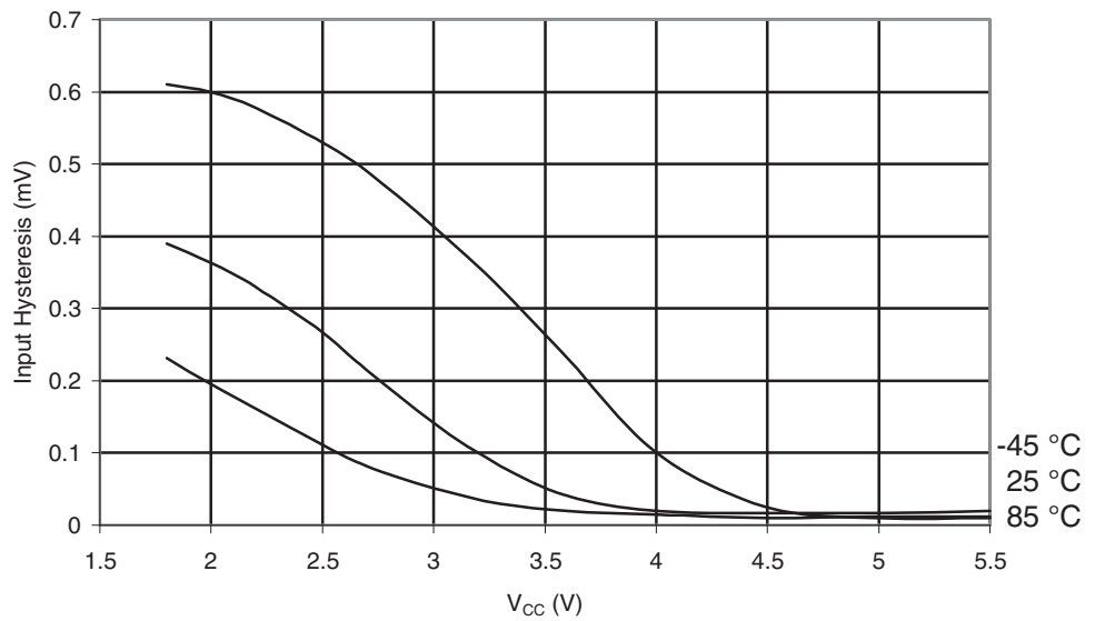
Figure 30-465. ATmega649P: Reset Input Pin Hysteresis vs. V_{CC}
