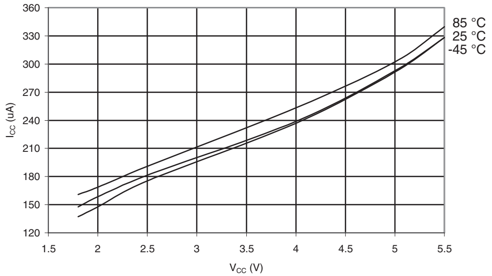
Figure 30-539. ATmega6490A: Active Supply Current with ADC at 200kHz vs. V_{CC}
