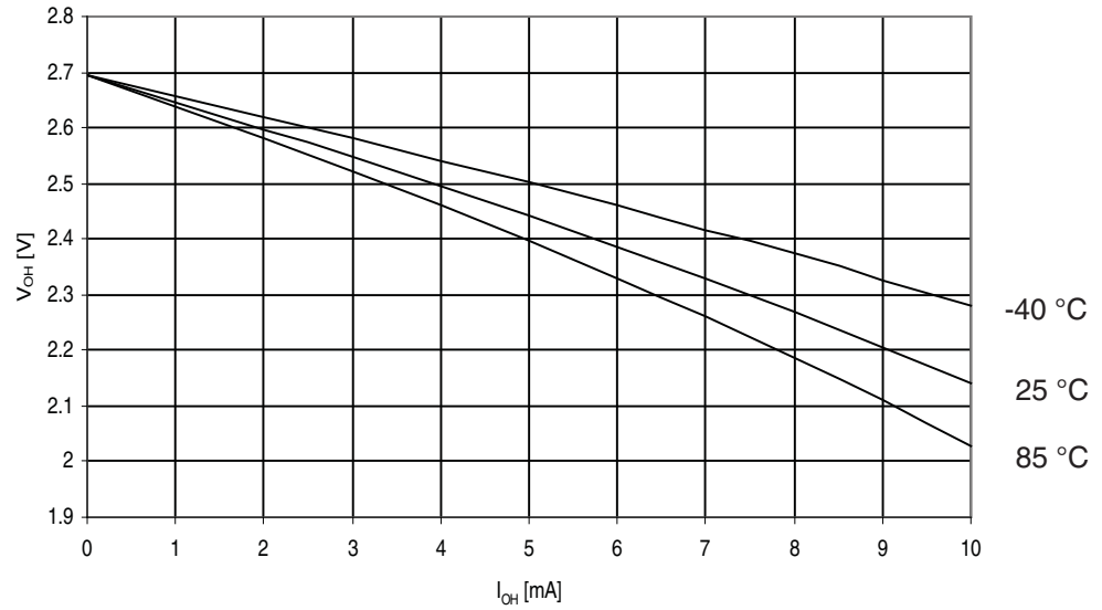
Figure 30-267. ATmega3290A: I/O Pin Output Voltage vs. Source Current, Ports A, C, D, E, F, G ( V_{CC} = 2.7V )
