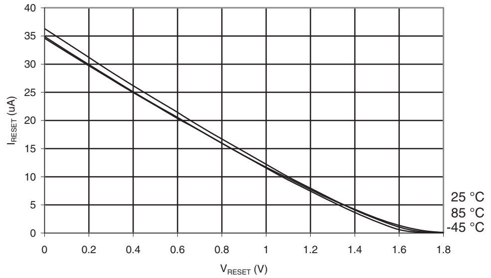
Figure 30-83. ATmega169PA: Reset Pull-up Resistor Current vs. Reset Pin Voltage ( V_{CC}=1.8V )
