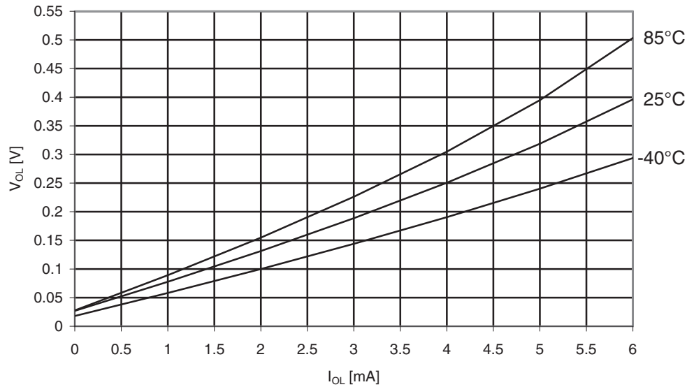
Figure 30-157. ATmega329A: I/O Pin Output Voltage vs. Sink Current, Port B ( V_{CC} = 1.8V )
