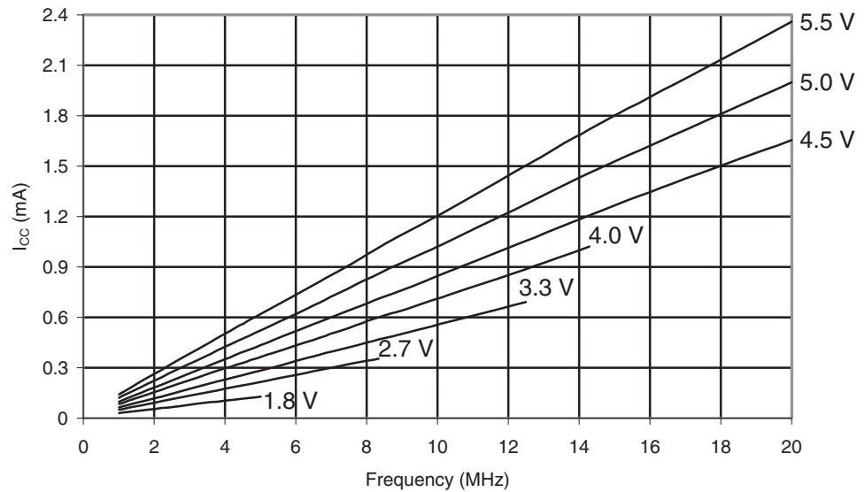
Figure 30-607. ATmega6490P: Reset Supply Current vs. V_{CC} (1 - 20MHz, Excluding Current Through The Reset Pull-up)
