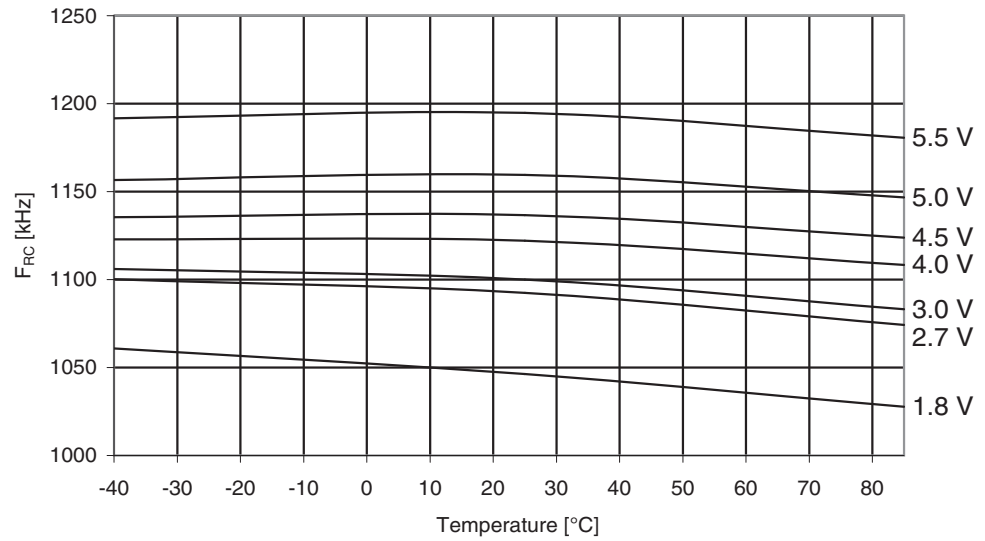
Figure 30-170. ATmega329A: Watchdog Oscillator Frequency vs. Temperature
