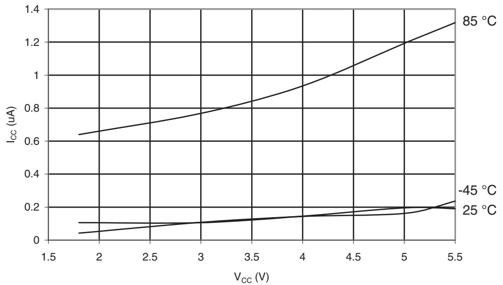
Figure 30-73. ATmega169PA: Power-down Supply Current vs. V_{CC} (Watchdog Timer Disabled)
