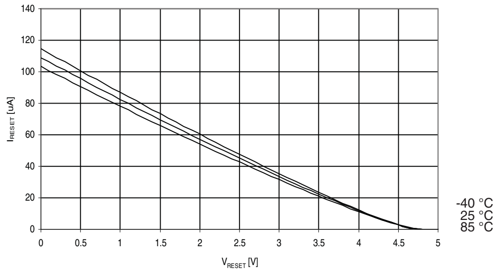
Figure 30-323. ATmega3290PA: Reset Pull-up Resistor Current vs. Reset Pin Voltage ( V_{CC}=5V )
