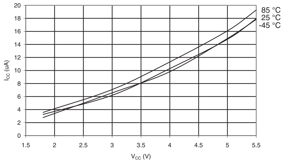
Figure 30-74. ATmega169PA: Power-down Supply Current vs. V_{CC} (Watchdog Timer Enabled)
