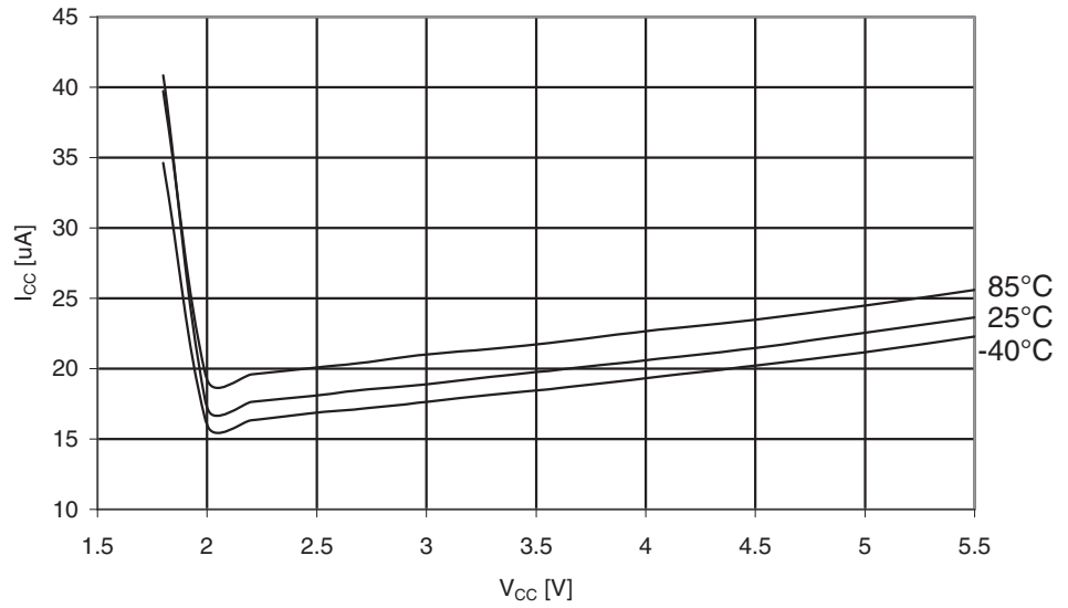
Figure 30-174. ATmega329A: Brownout Detector Current vs. V_{CC}
