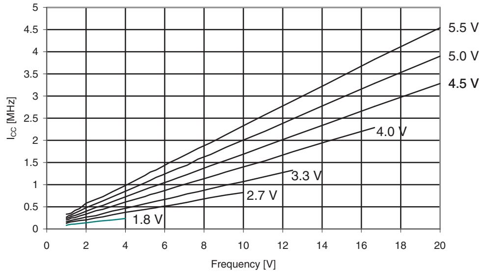
Figure 30-311. ATmega3290PA: Idle Supply Current vs. Frequency (1 - 20MHz)
