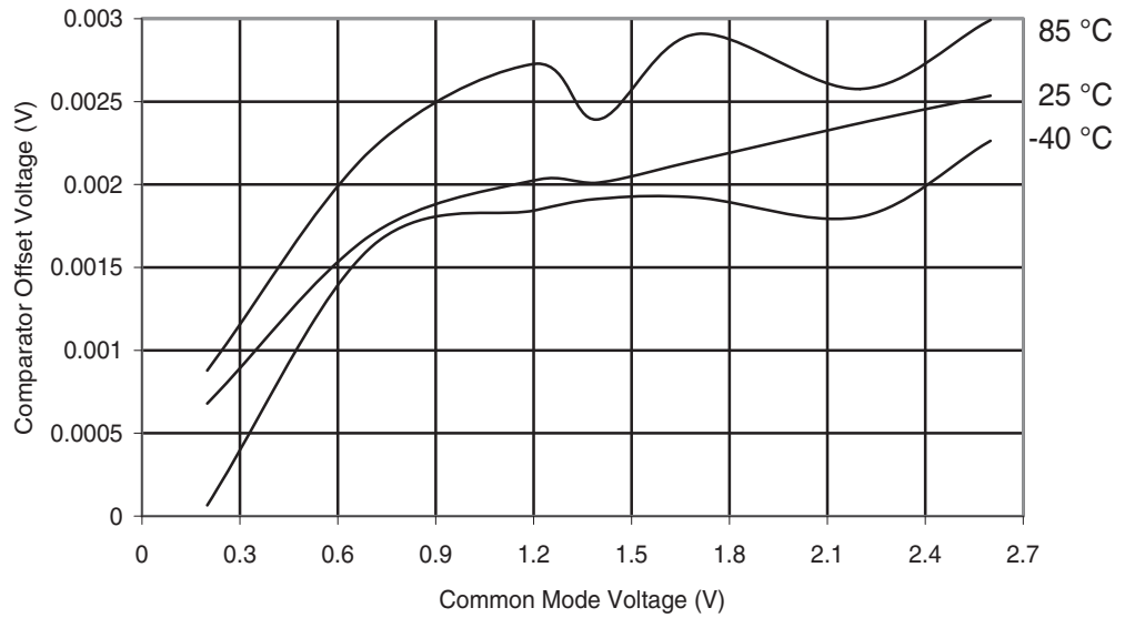
Figure 30-108. ATmega169PA: Analog Comparator Offset Voltage vs. Common Mode Voltage ( V_{CC} = 2.7V )
