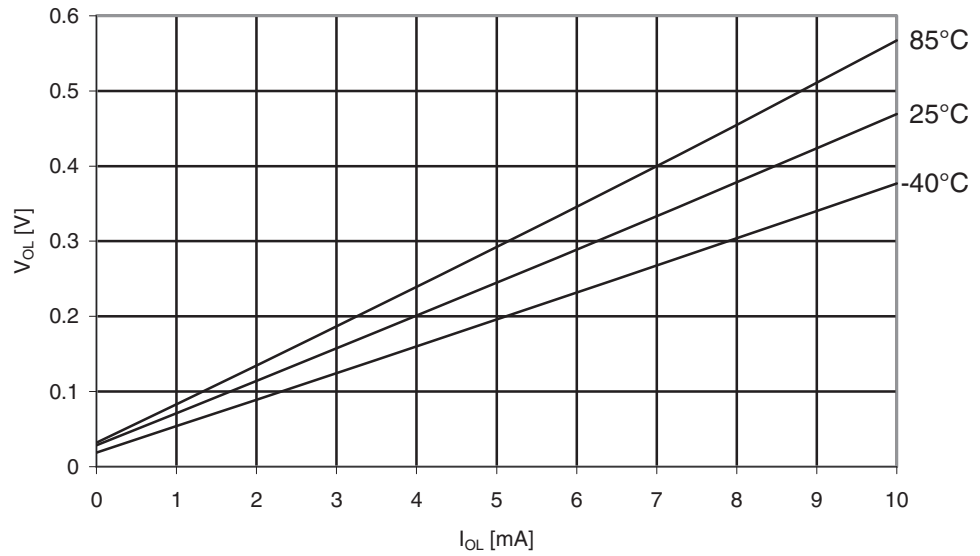
Figure 30-152. ATmega329A: I/O Pin Output Voltage vs. Sink Current, Ports A, C, D, E, F, G ( V_{CC} = 5V )
