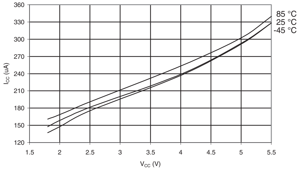
Figure 30-478. ATmega649P: Active Supply Current with ADC at 200kHz vs. V_{CC}
