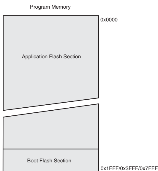
Figure 8-1. Program Memory Map
