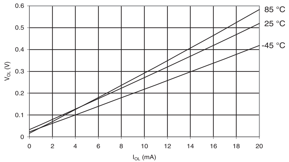
Figure 30-518. ATmega6490A: I/O Pin Output Voltage vs. Sink Current, Port B ( V_{CC} = 5V )
