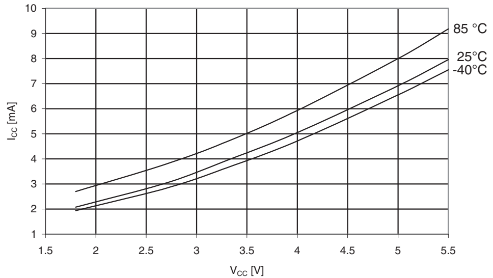
Figure 30-314. ATmega3290PA: Idle Supply Current vs. V_{CC} (32kHz Watch Crystal)
