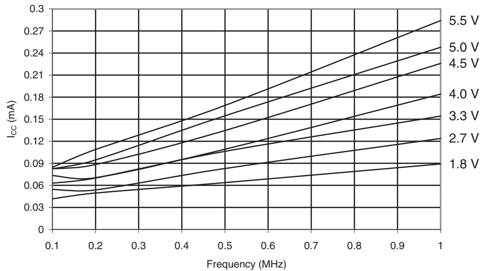
Figure 30-370. ATmega649A: Idle Supply Current vs. Low Frequency (0.1 - 1.0MHz)
