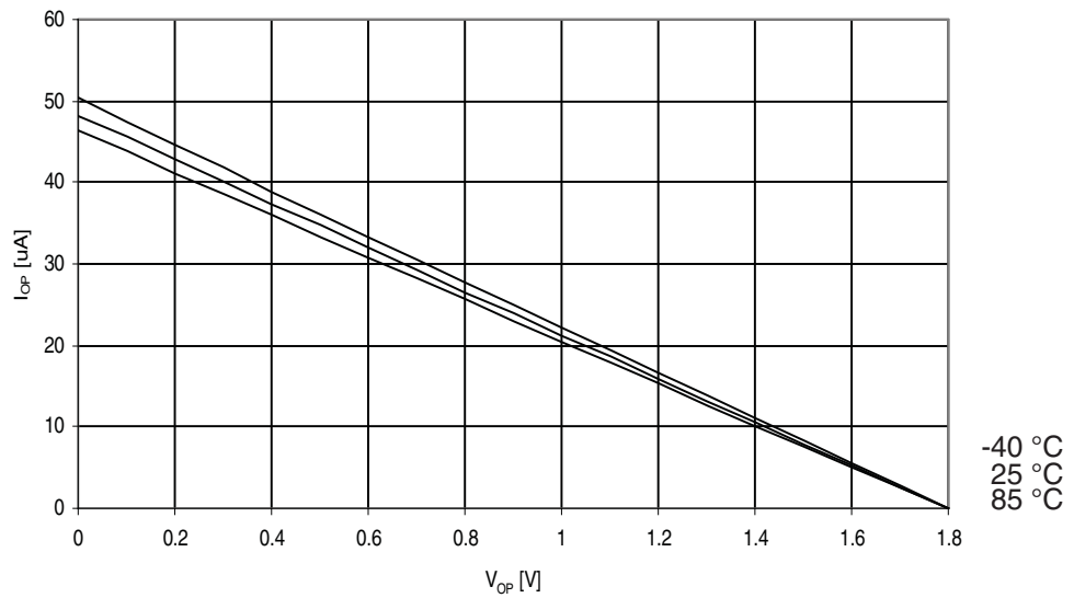
Figure 30-262. ATmega3290A: I/O Pin Pull-up Resistor Current vs. Input Voltage ( V_{CC} = 1.8V )
