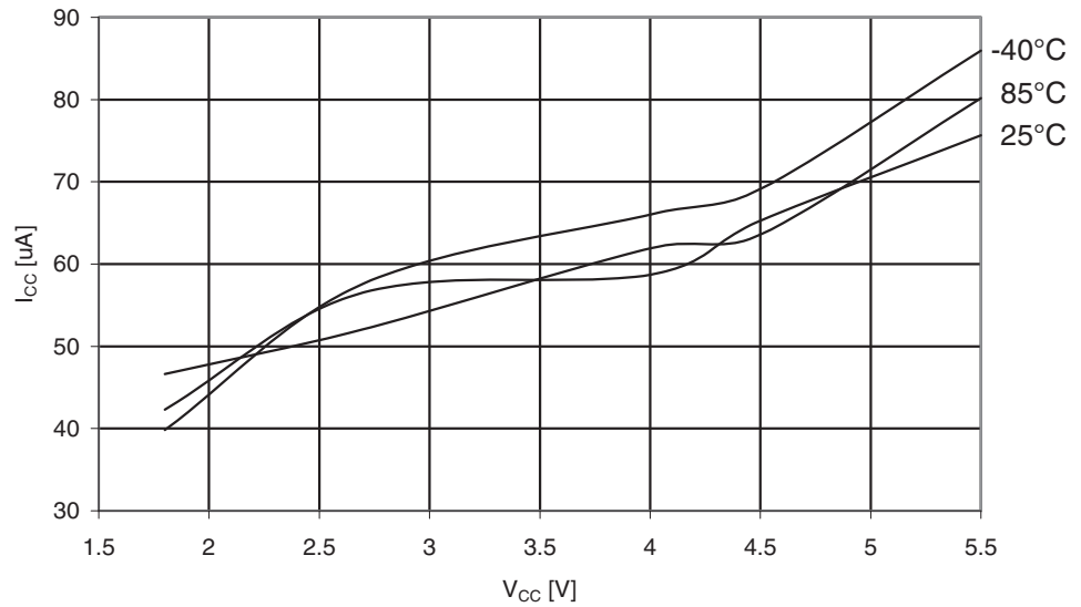
Figure 30-300. ATmega3290A: Analog Comparator Current vs. V_{CC}
