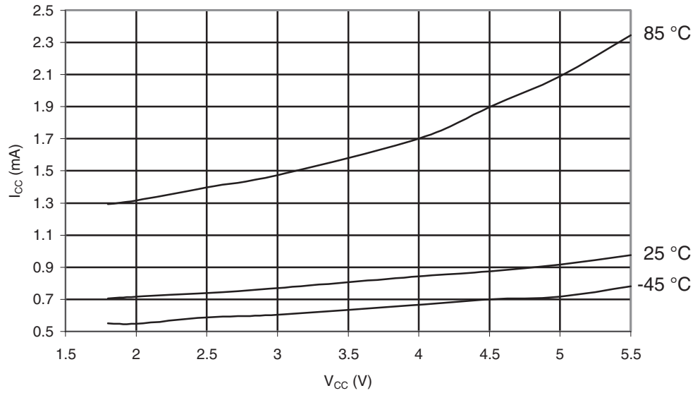
Figure 30-563. ATmega6490P: Standby Supply Current vs. V_{CC} (Xtall and Resonator, Watchdog Timer Disabled)
