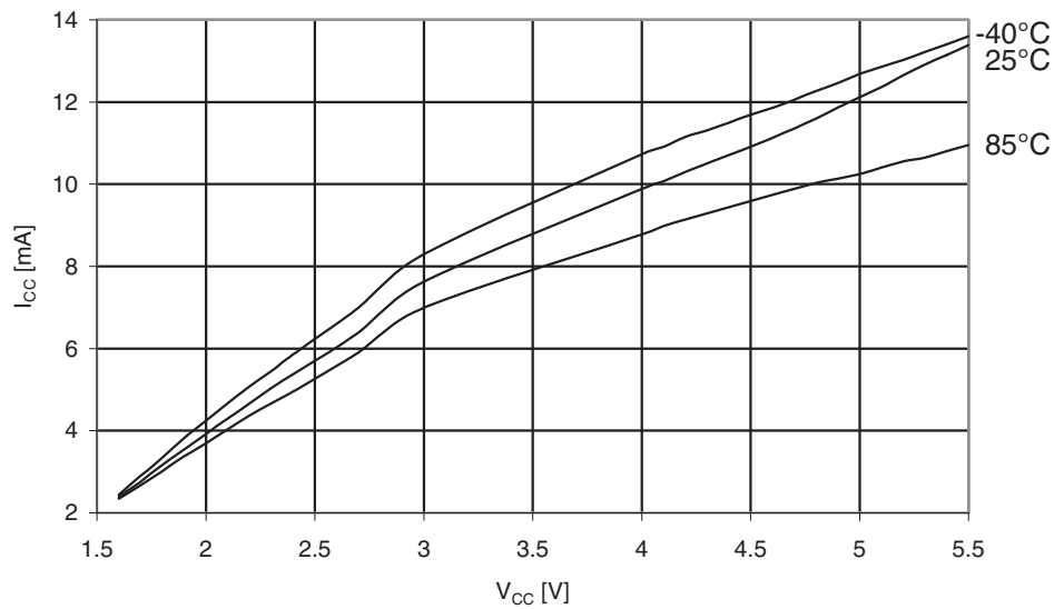
Figure 30-241. ATmega329PA: Programming Current vs. V_{CC}
