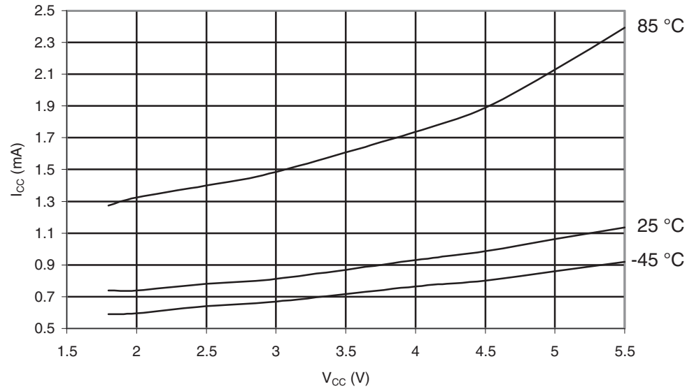
Figure 30-439. ATmega649P: Power-save Supply Current vs. V_{CC} (Watchdog Timer Disabled and 32kHz Crystal Oscillator Running)
