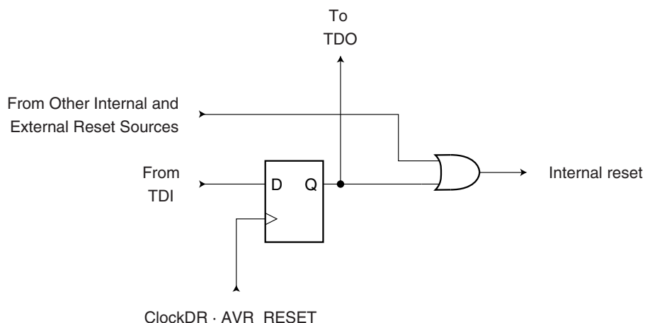
Figure 26-1. Reset Register
