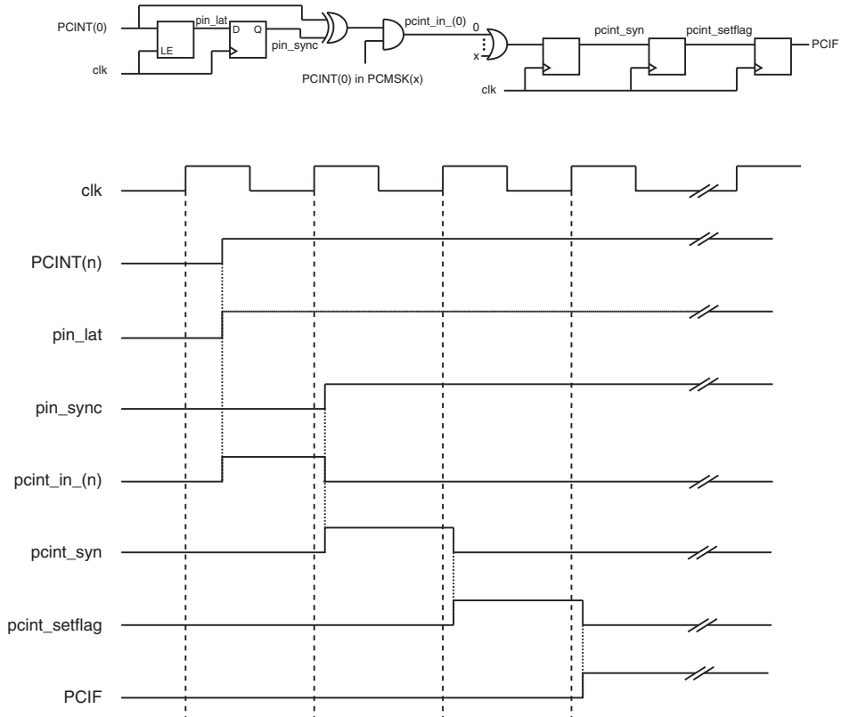
Figure 13-1. Pin Change Interrupt
