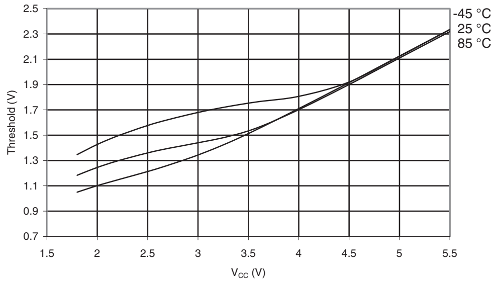
Figure 30-99. ATmega169PA: Reset Input Threshold Voltage vs. V_{CC} ( V_{IH} , Reset Pin Read as "1")
