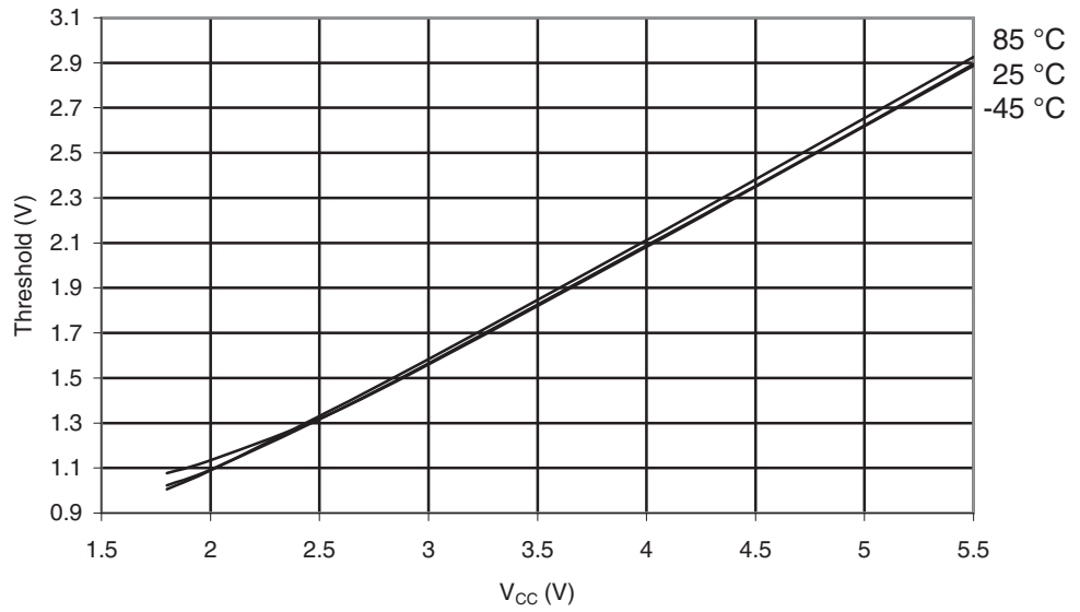
Figure 30-399. ATmega649A: I/O Pin Input Threshold Voltage vs. V_{CC} ( V_{IH} , I/O Pin Read as "1")
