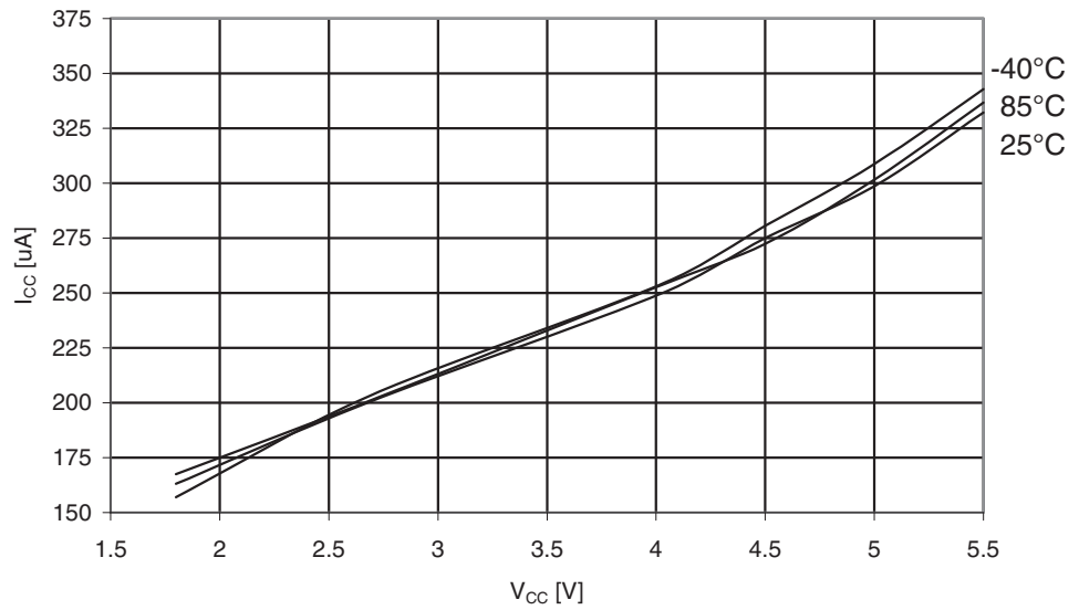
Figure 30-175. ATmega329A: Active Supply Current with ADC at 50kHz vs. V_{CC}
