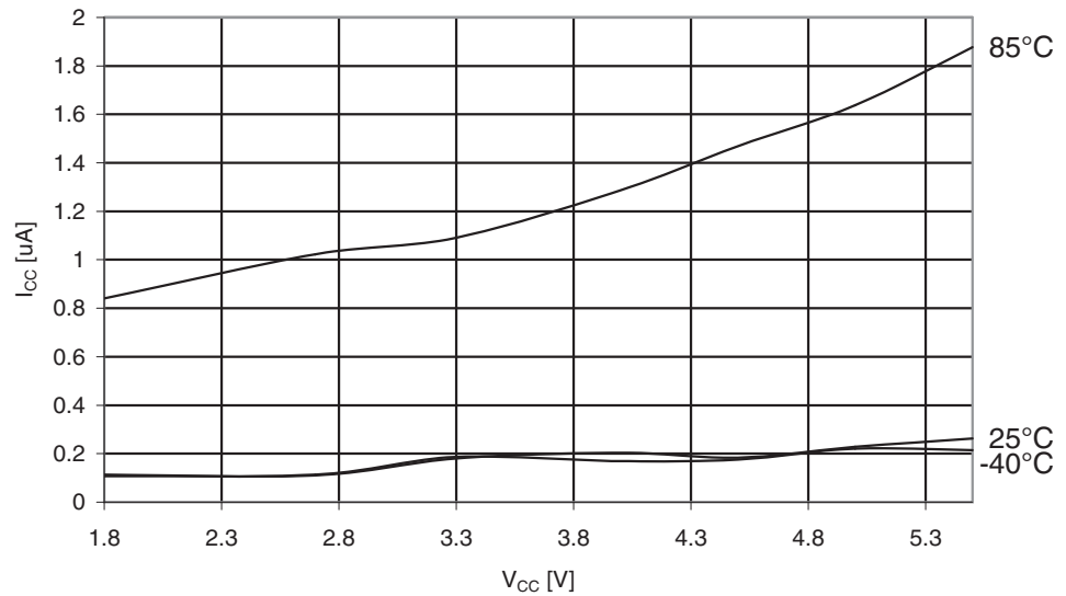
Figure 30-256. ATmega3290A: Power-down Supply Current vs. V_{CC} (Watchdog Timer Enabled)
