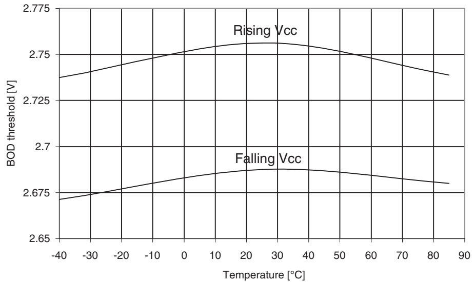
Figure 30-165. ATmega329A: BOD Thresholds vs. Temperature (BOD Level is 2.7V)
