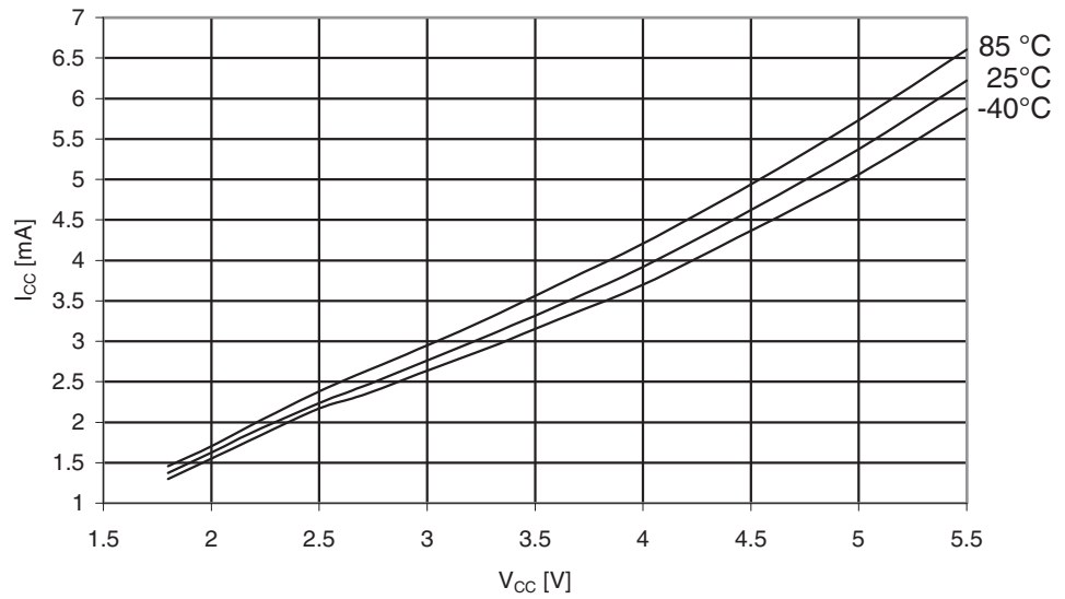
Figure 30-187. ATmega329PA: Active Supply Current vs. V_{CC} (Internal RC Oscillator, 8MHz)
