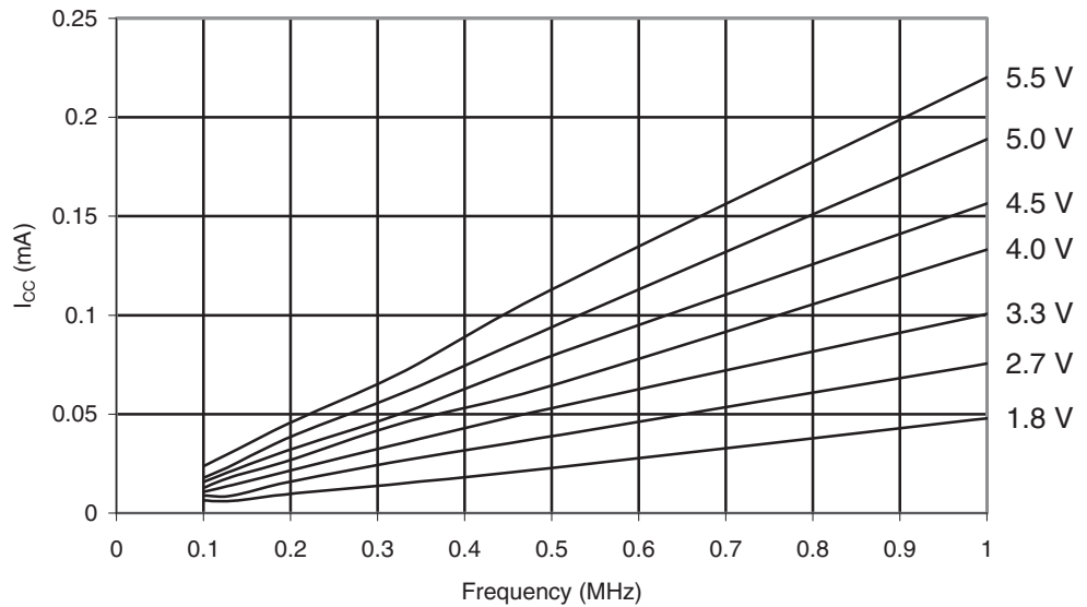
Figure 30-68. ATmega169PA: Idle Supply Current vs. Frequency (0.1 - 1.0MHz)
