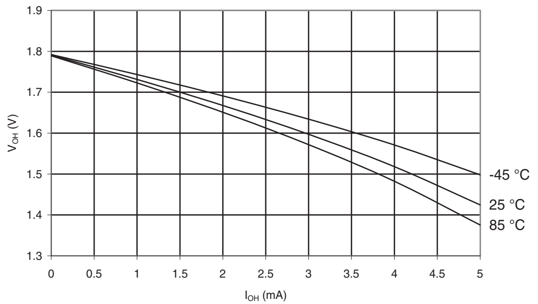
Figure 30-27. ATmega169A: I/O Pin Output Voltage vs. Source Current, Port B ( V_{CC} = 1.8V )
