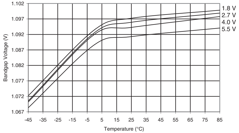
Figure 30-44. ATmega169A: Bandgap Voltage vs. Temperature
