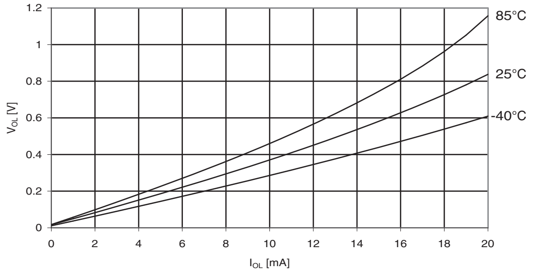
Figure 30-156. ATmega329A: I/O Pin Output Voltage vs. Sink Current, Port B ( V_{CC} = 2.7V )
