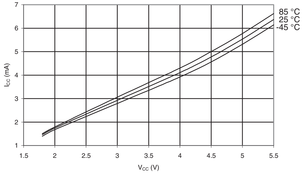
Figure 30-489. ATmega6490A: Active Supply Current vs. V_{CC} (Internal RC Oscillator, 8MHz)
