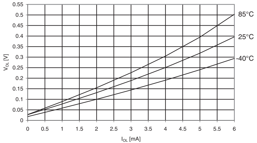
Figure 30-277. ATmega3290A: I/O Pin Output Voltage vs. Sink Current, Port B ( V_{CC} = 1.8V )
