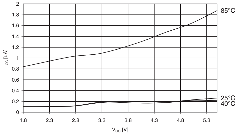
Figure 30-315. ATmega3290PA Power-down Supply Current vs. V_{CC} (Watchdog Timer Disabled)
