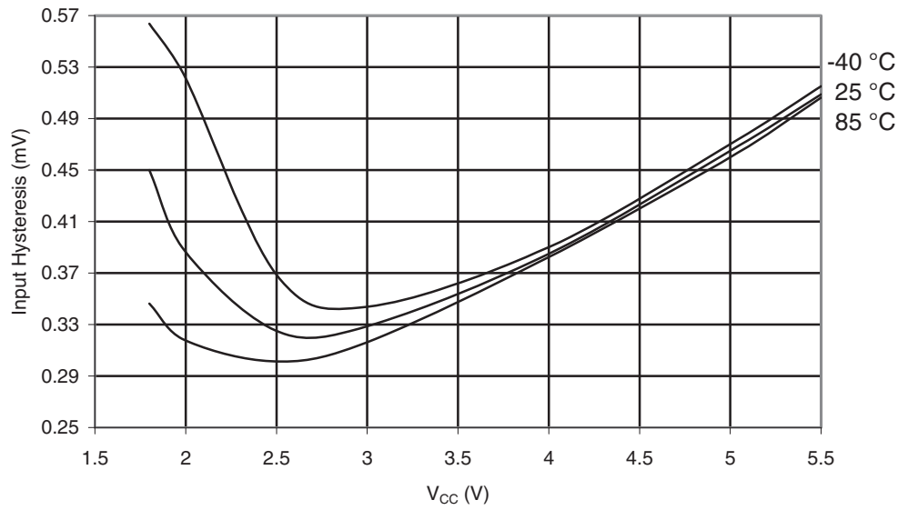
Figure 30-220. ATmega329PA: I/O Pin Input Hysteresis vs. V_{CC}
