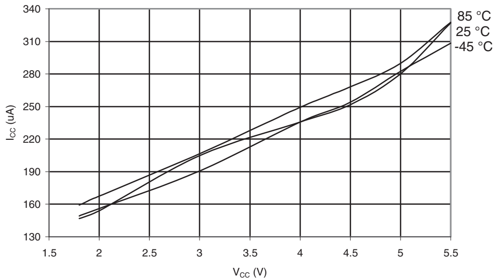
Figure 30-540. ATmega6490A: Active Supply Current with ADC at 1MHz vs. V_{CC}
