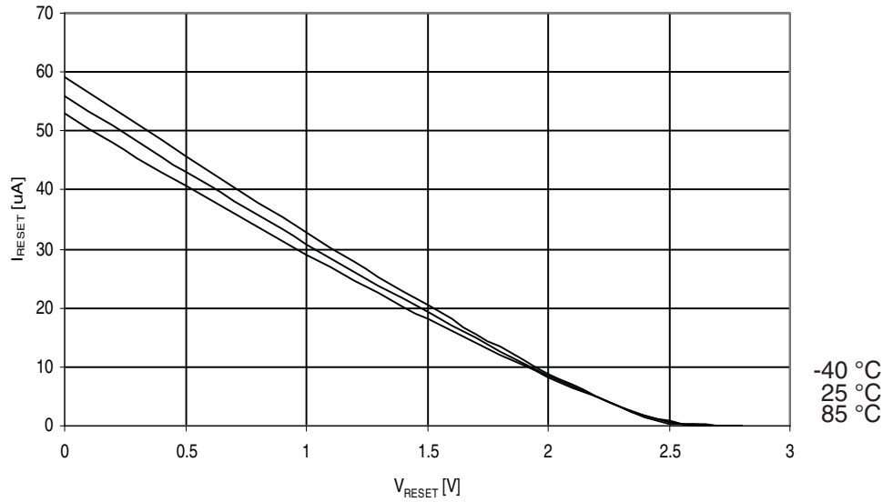
Figure 30-324. ATmega3290PA: Reset Pull-up Resistor Current vs. Reset Pin Voltage ( V_{CC}=2.7V )
