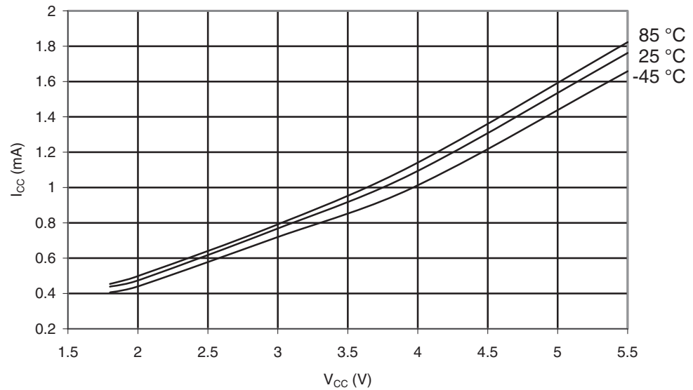
Figure 30-433. ATmega649P: Idle Supply Current vs. V_{CC} (Internal RC Oscillator, 8MHz)
