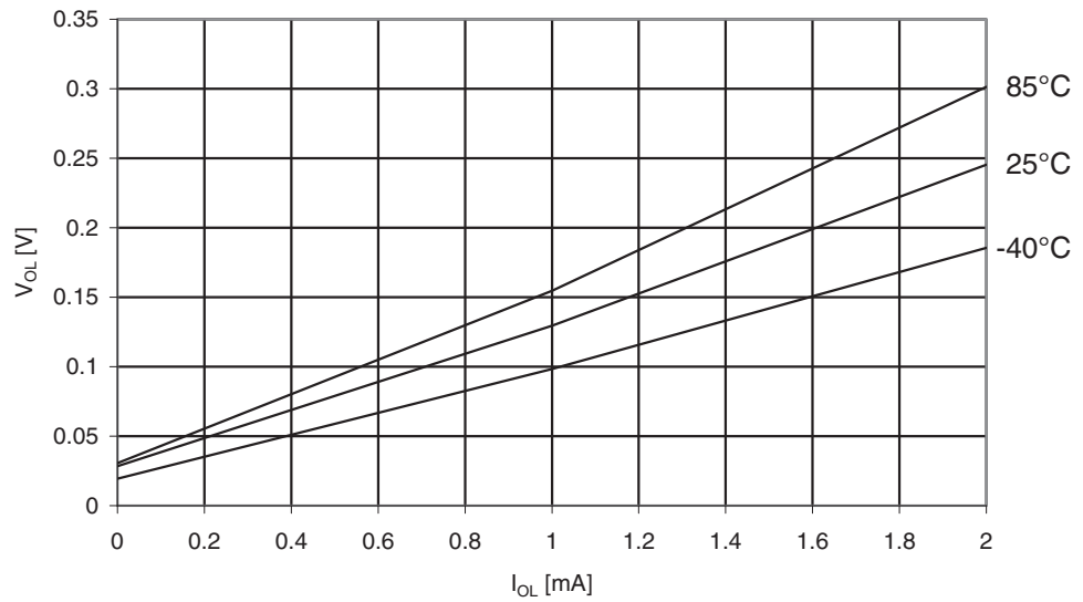
Figure 30-274. ATmega3290A: I/O Pin Output Voltage vs. Sink Current, Ports A, C, D, E, F, G ( V_{CC} = 1.8V )
