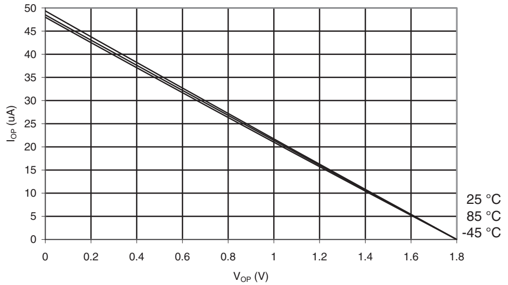
Figure 30-18. ATmega169A: I/O Pin Pull-up Resistor Current vs. Input Voltage ( V_{CC} = 1.8V )
