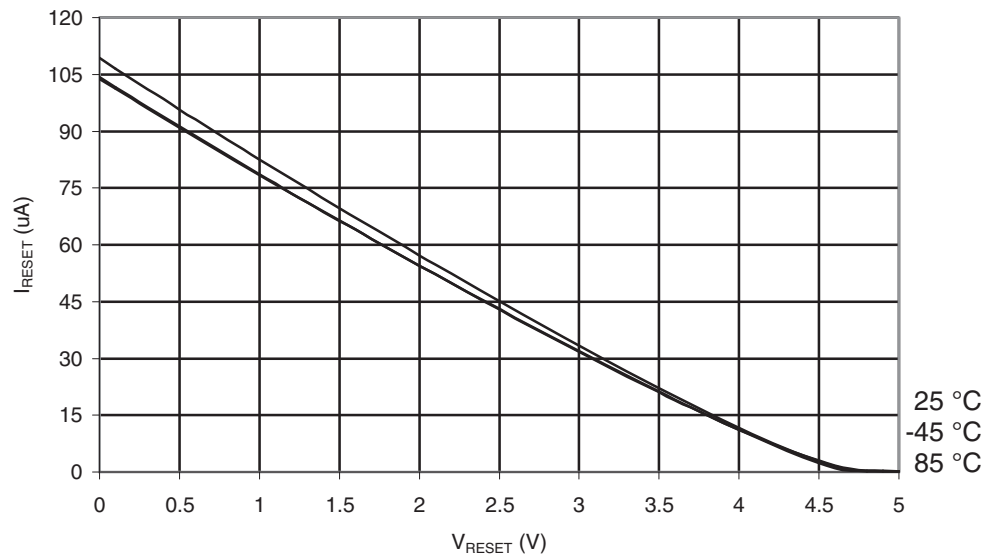
Figure 30-506. ATmega6490A: Reset Pull-up Resistor Current vs. Reset Pin Voltage ( V_{CC} = 5V )
