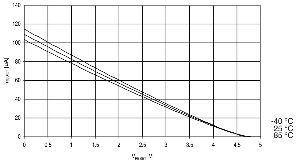
Figure 30-203. ATmega329PA: Reset Pull-up Resistor Current vs. Reset Pin Voltage ( V_{CC} = 5V )
