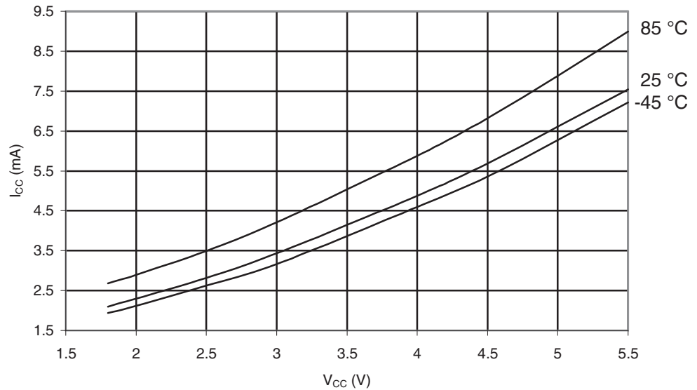
Figure 30-435. ATmega649P: Idle Supply Current vs. V_{CC} (32kHz Watch Crystal)
