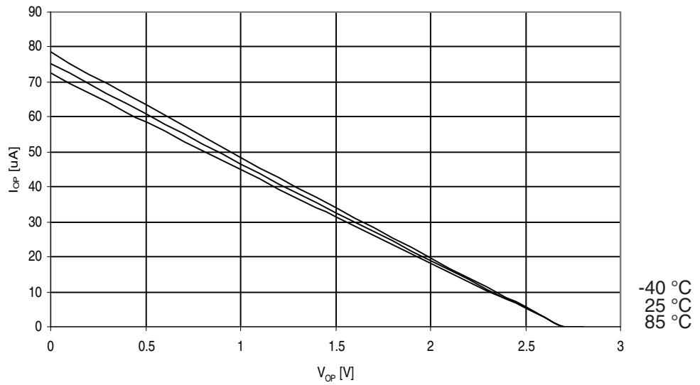
Figure 30-201. ATmega329PA: I/O Pin Pull-up Resistor Current vs. Input Voltage ( V_{CC} = 2.7V )
