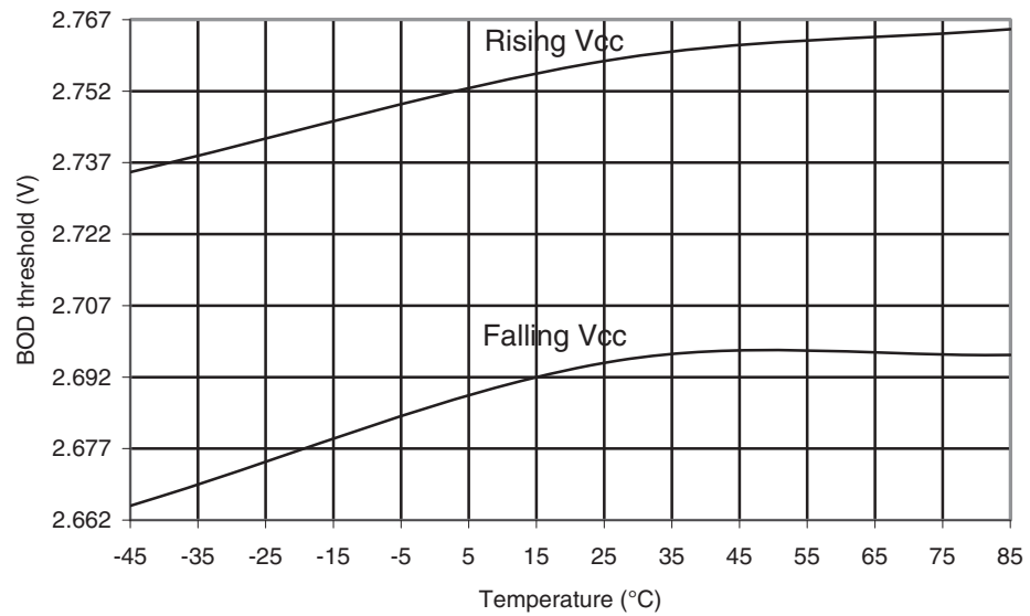
Figure 30-41. ATmega169A: BOD Thresholds vs. Temperature (BOD Level is 2.7V)
