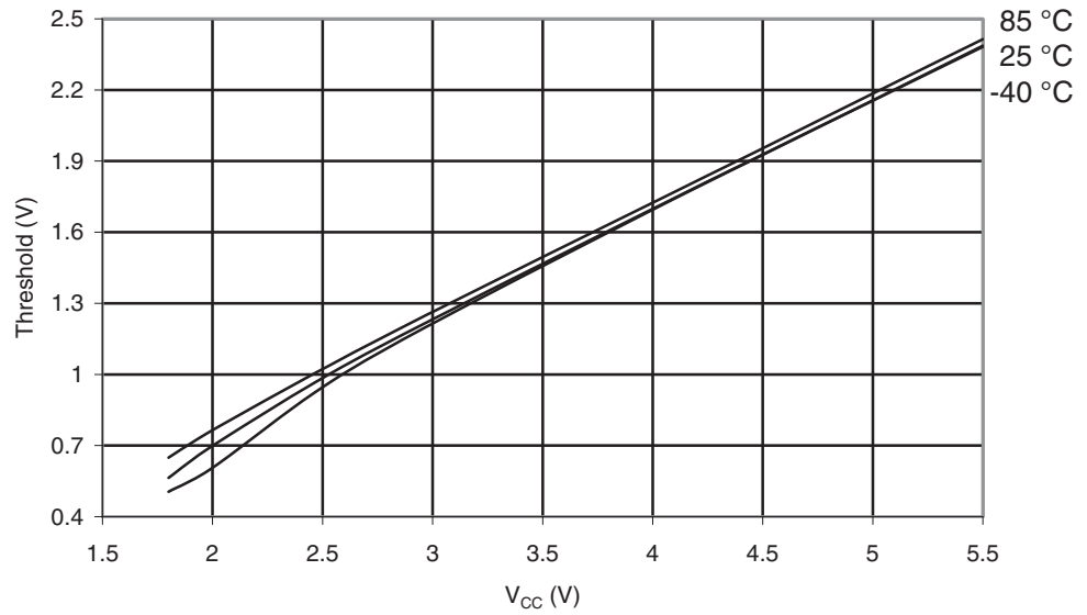
Figure 30-339. ATmega3290PA: I/O Pin Input Threshold Voltage vs. V_{CC} ( V_{IL} , I/O Pin Read as "0")
