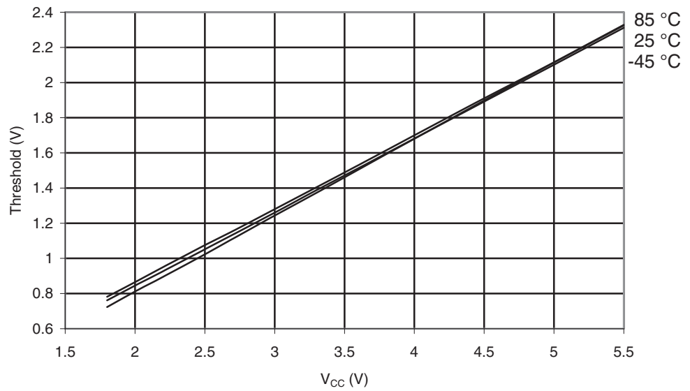
Figure 30-100. ATmega169PA: Reset Input Threshold Voltage vs. V_{CC} ( V_{IL} , Reset Pin Read as "0")
