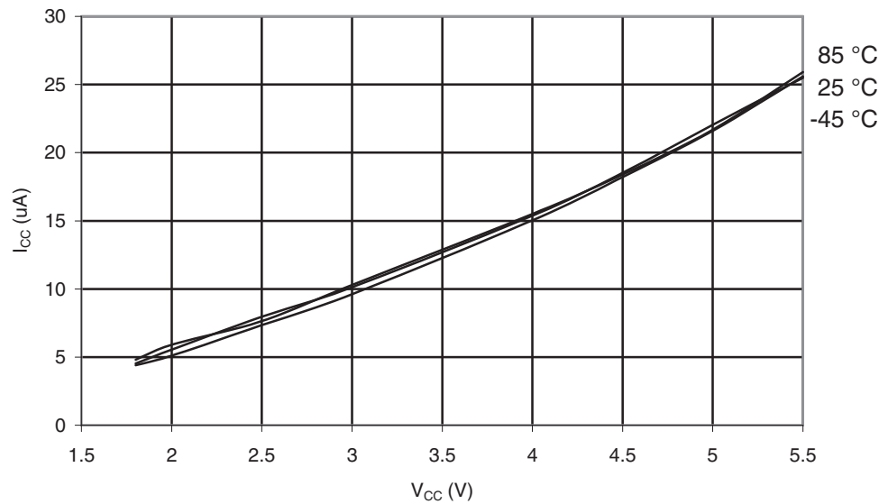
Figure 30-57. ATmega169A: Watchdog Timer Current vs. V_{CC}
