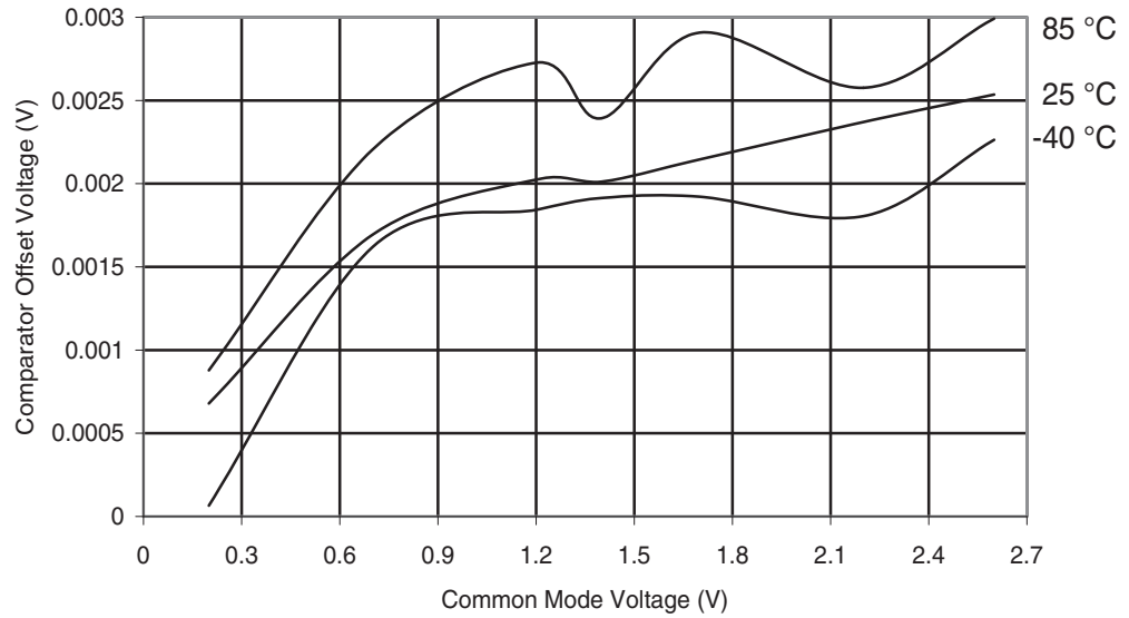
Figure 30-46. ATmega169A: Analog Comparator Offset Voltage vs. Common Mode Voltage ( V_{CC} = 2.7V )
