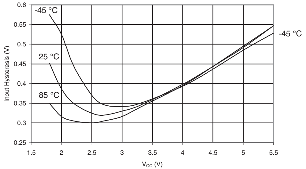
Figure 30-523. ATmega6490A: I/O Pin Input Hysteresis vs. V_{CC}
