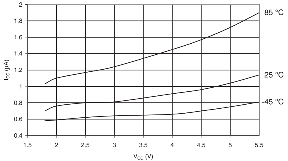
Figure 30-13. ATmega169A: Power-save Supply Current vs. V_{CC} (Watchdog Timer Disabled and 32kHz Crystal Oscillator Running)
