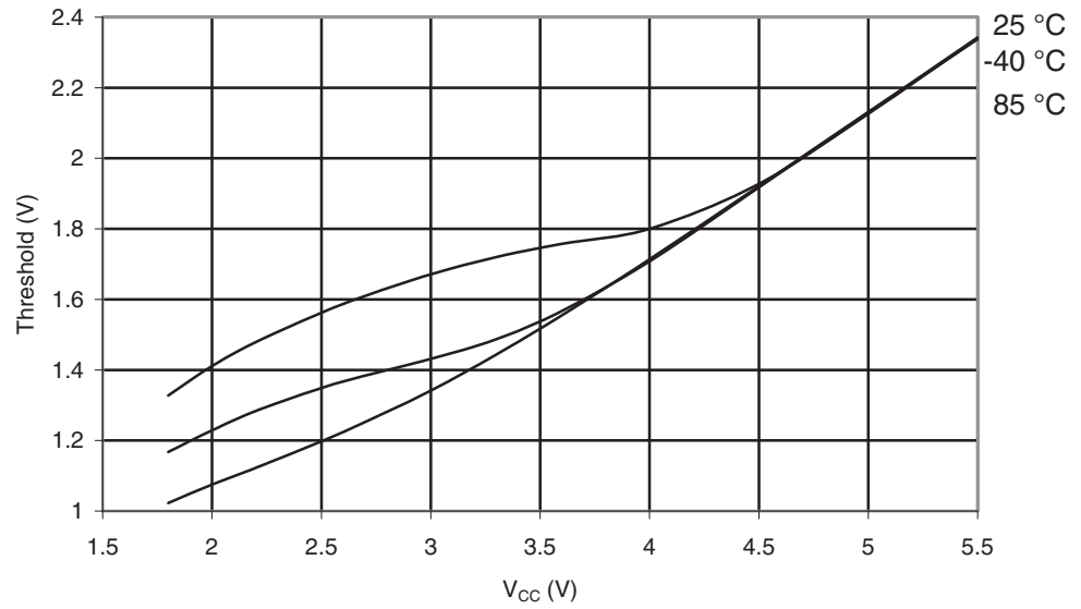
Figure 30-281. ATmega3290A: Reset Input Threshold Voltage vs. V_{CC} ( V_{IH} , Reset Pin Read as "1")
