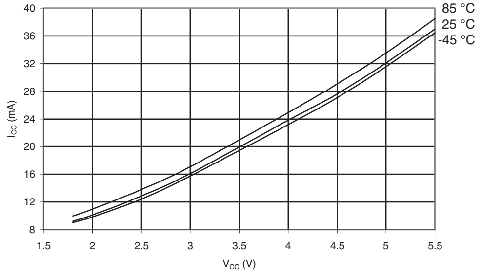
Figure 30-430. ATmega649P: Active Supply Current vs. V_{CC} (32kHz Watch Crystal)
