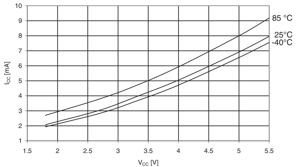
Figure 30-134. ATmega329A: Idle Supply Current vs. V_{CC} (32kHz Watch Crystal)
