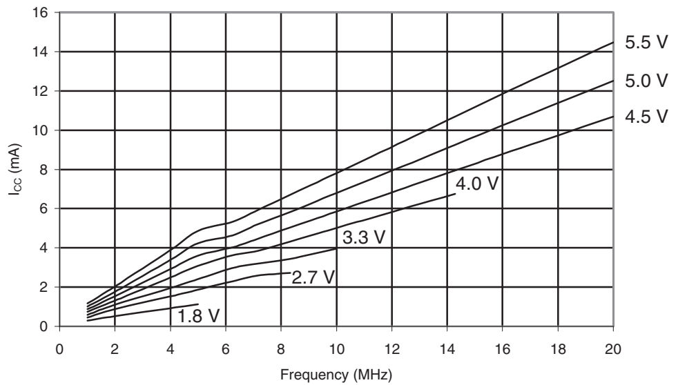
Figure 30-427. ATmega649P: Active Supply Current vs. Frequency (1 - 20MHz)
