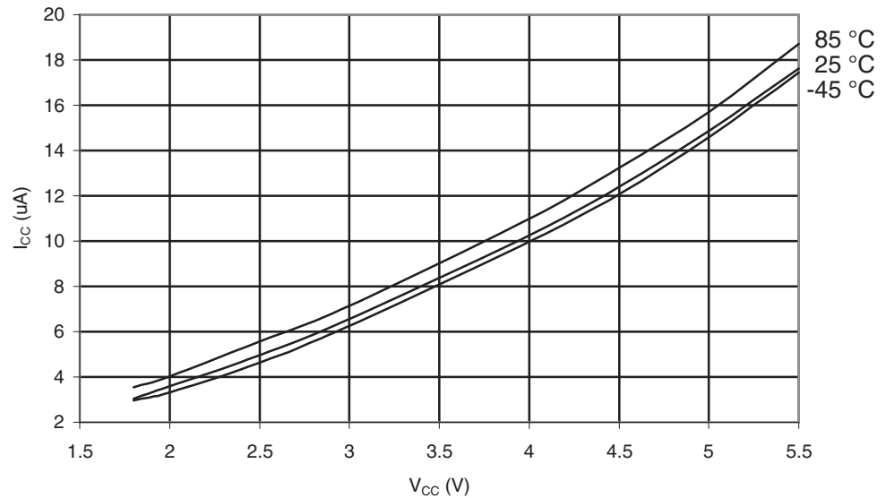
Figure 30-376. ATmega649A: Power-down Supply Current vs. V_{CC} (Watchdog Timer Enabled)
