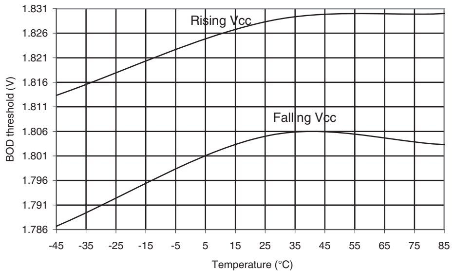
Figure 30-104. ATmega169PA: BOD Thresholds vs. Temperature (BOD Level is 1.8V)
