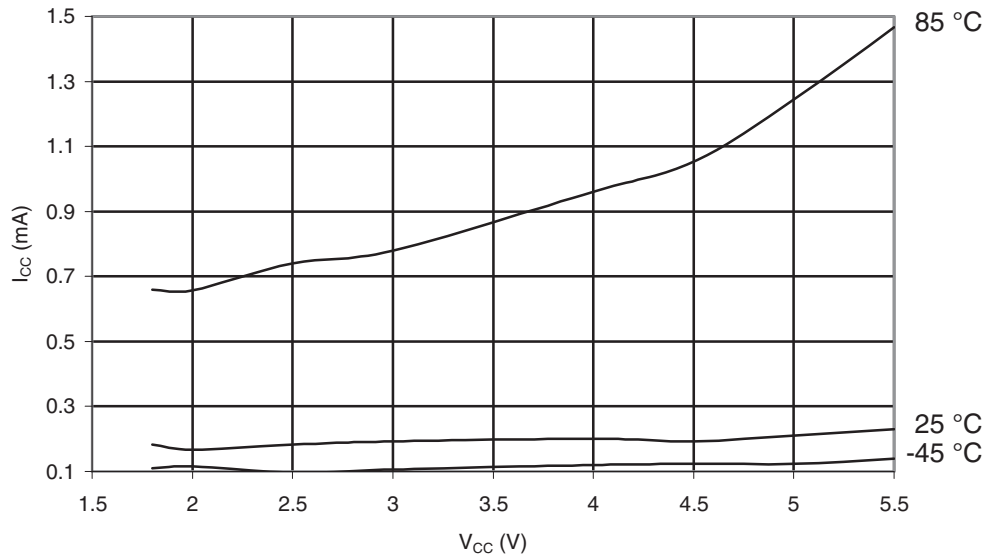
Figure 30-560. ATmega649A: Power-down Supply Current vs. V_{CC} (32kHz Watch Crystal)
