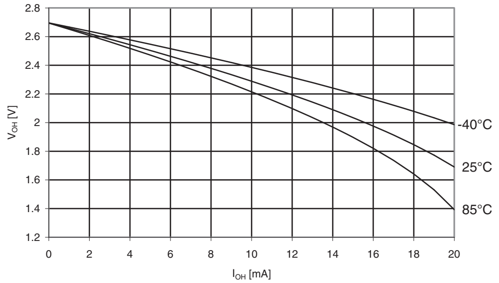
Figure 30-210. ATmega329PA: I/O Pin Output Voltage vs. Source Current, Port B ( V_{CC} = 2.7V )
