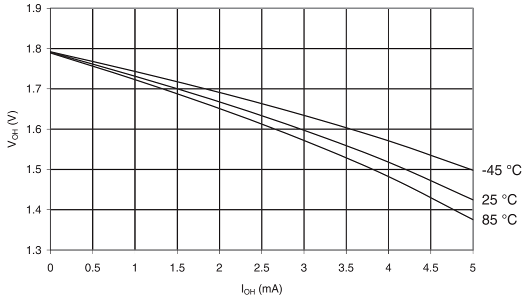
Figure 30-89. ATmega169PA: I/O Pin Output Voltage vs. Source Current, Port B ( V_{CC} = 1.8V )
