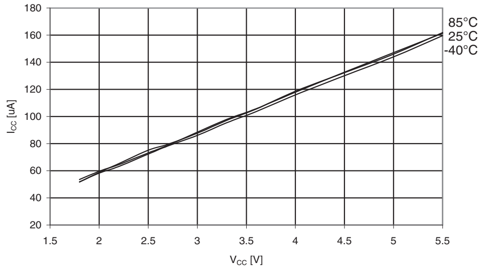
Figure 30-238. ATmega329PA: AREF External Reference Current vs. V_{CC}
