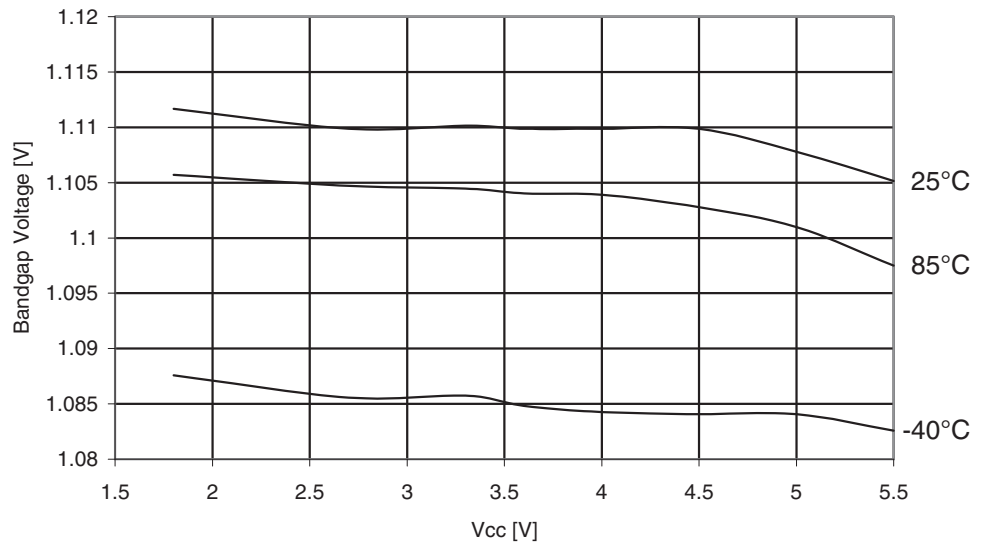
Figure 30-167. ATmega329A: Bandgap Voltage vs. V CC
