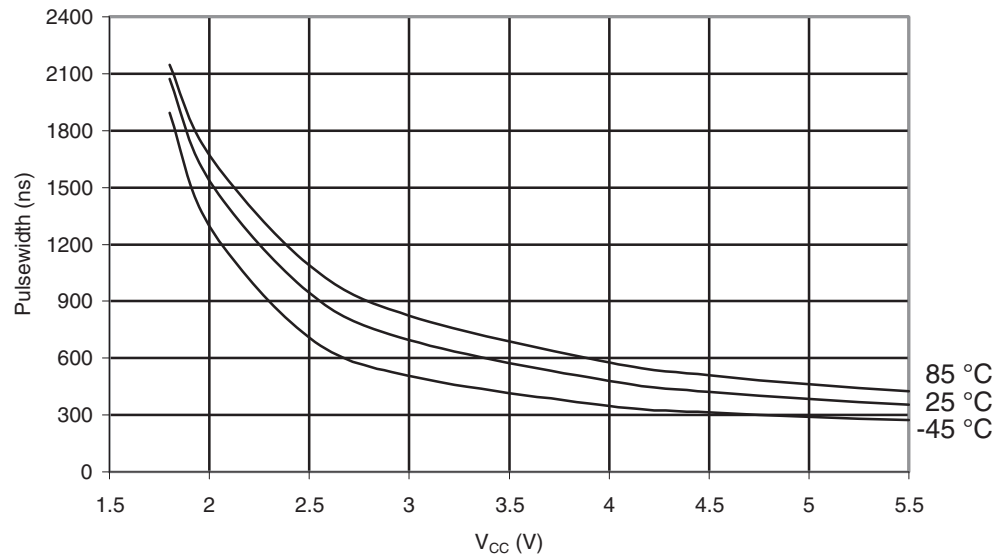
Figure 30-608. ATmega6490P: Minimum Reset Pulse Width vs. V_{CC}
