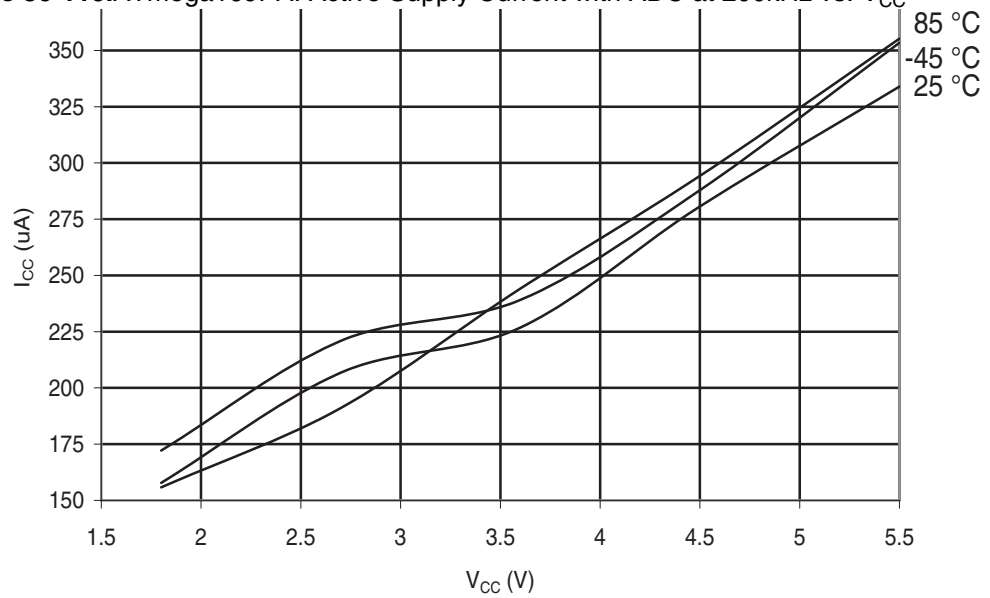
Figure 30-116. ATmega169PA: Active Supply Current with ADC at 200kHz vs. V_{CC}
