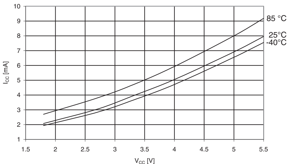
Figure 30-254. ATmega3290A: Idle Supply Current vs. V_{CC} (32kHz Watch Crystal)
