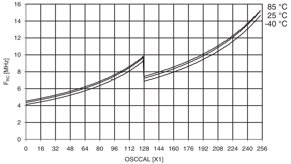
Figure 30-293. ATmega3290A: Calibrated 8MHz RC Oscillator Frequency vs. Oscal Value
