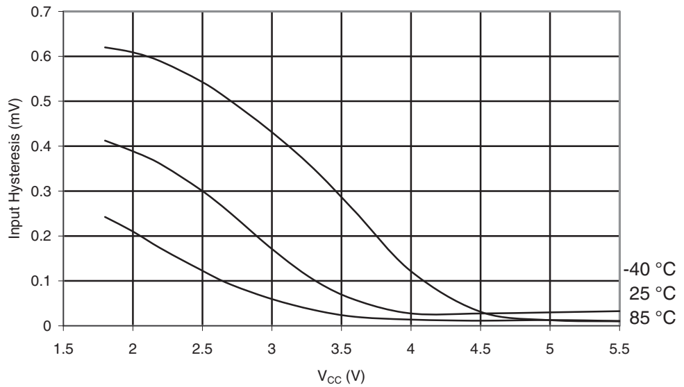
Figure 30-283. ATmega3290A: Reset Input Pin Hysteresis vs. V_{CC}
