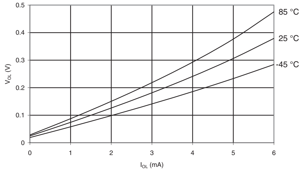
Figure 30-33. ATmega169A: I/O Pin Output Voltage vs. Sink Current, Port B ( V_{CC} = 1.8V )
