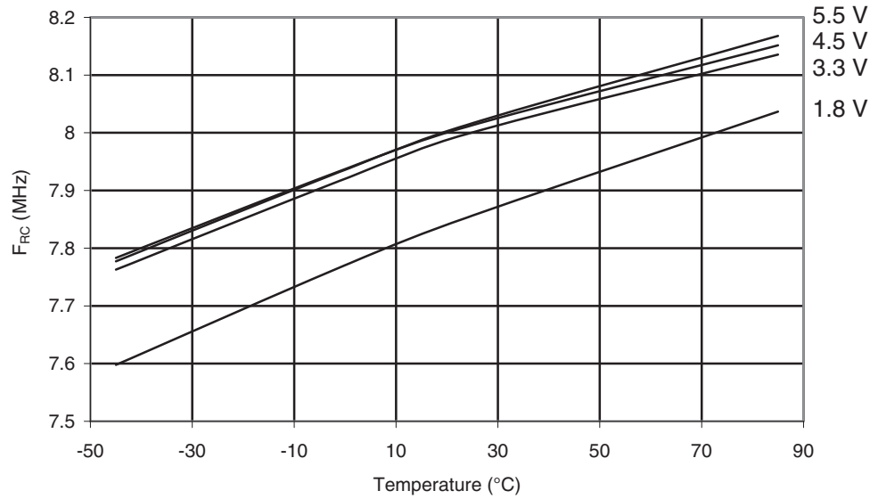
Figure 30-49. ATmega169A: Calibrated 8MHz RC Oscillator Frequency vs. Temperature
