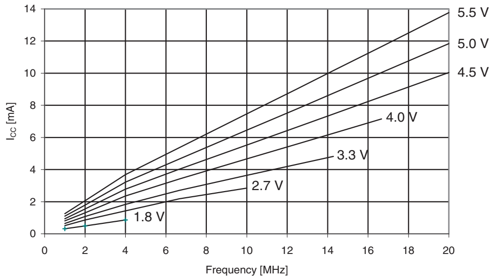
Figure 30-246. ATmega3290A: Active Supply Current vs. Frequency (1 - 20MHz)
