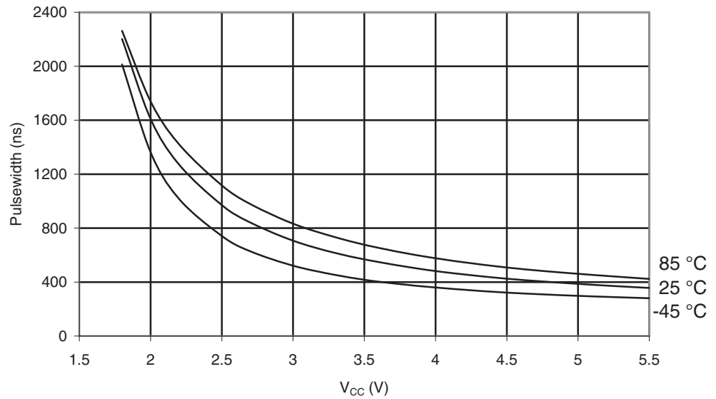
Figure 30-124. ATmega169PA: Minimum Reset Pulse Width vs. V_{CC}
