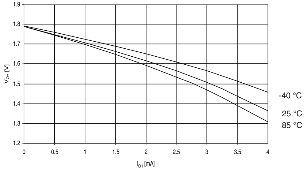
Figure 30-208. ATmega329PA: I/O Pin Output Voltage vs. Source Current, Ports A, C, D, E, F, G ( V_{CC} = 1.8V )
