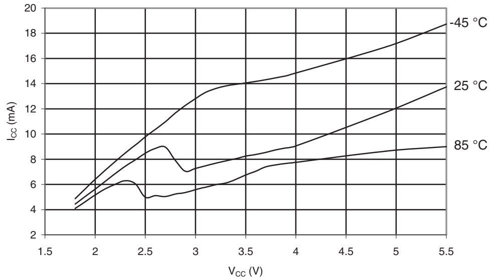
Figure 30-544. ATmega6490A: Programming Current vs. V_{CC}
