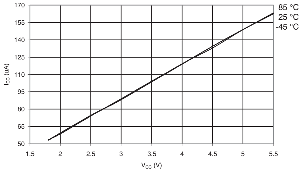
Figure 30-541. ATmega6490A: AREF External Reference Current vs. V_{CC}
