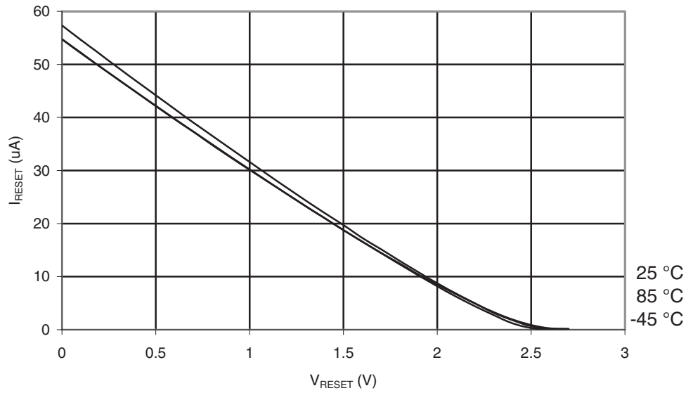
Figure 30-20. ATmega169A: Reset Pull-up Resistor Current vs. Reset Pin Voltage ( V_{CC} = 2.7V )
