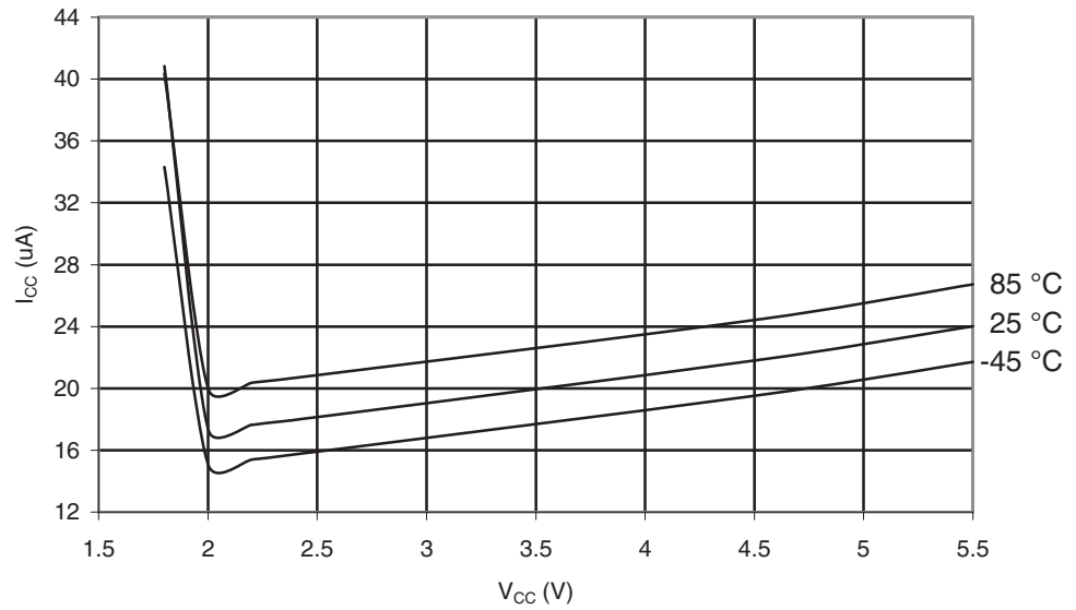
Figure 30-52. ATmega169A: Brownout Detector Current vs. V_{CC}
