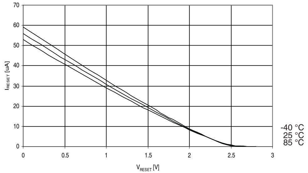
Figure 30-264. ATmega3290A: Reset Pull-up Resistor Current vs. Reset Pin Voltage ( V_{CC}=2.7V )
