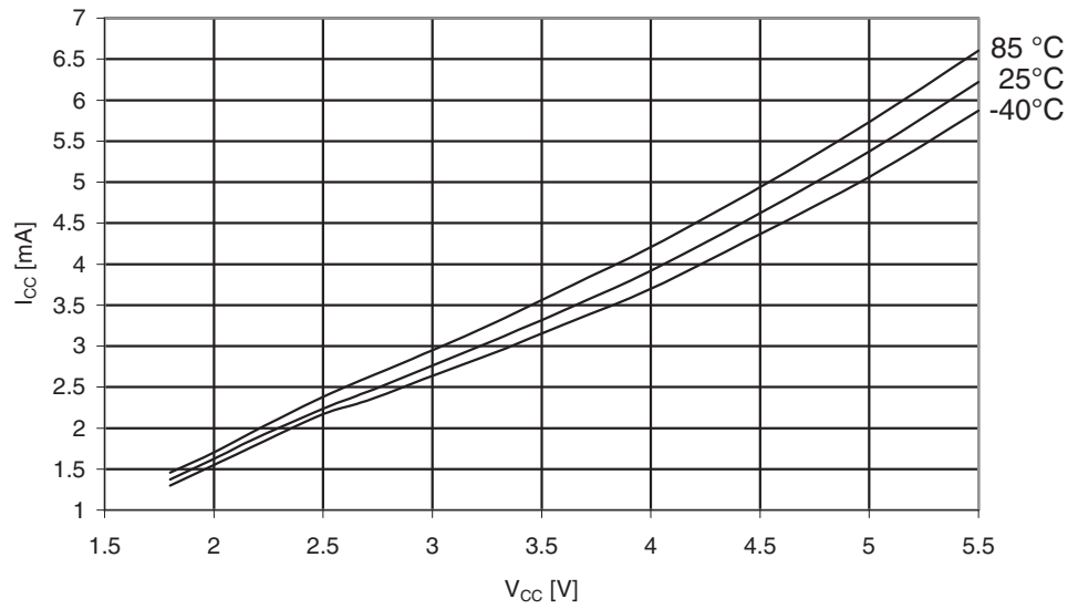
Figure 30-247. ATmega3290A: Active Supply Current vs. V_{CC} (Internal RC Oscillator, 8MHz)
