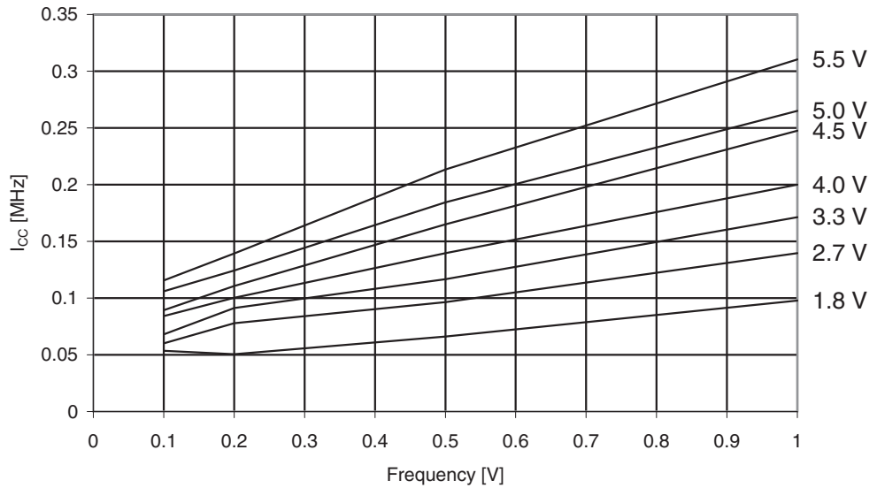
Figure 30-310. ATmega3290PA: Idle Supply Current vs. Low Frequency (0.1 - 1.0MHz)
