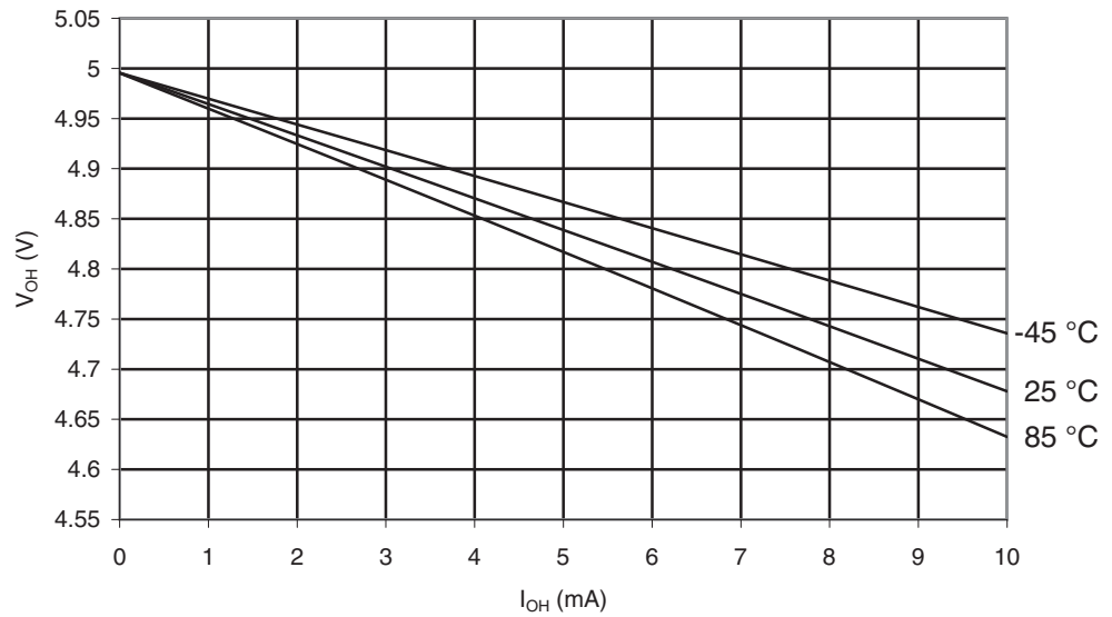
Figure 30-22. ATmega169A: I/O Pin Output Voltage vs. Source Current, Ports A, C, D, E, F, G ( V_{CC} = 5V )
