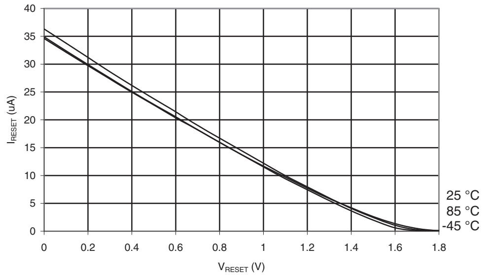
Figure 30-21. ATmega169A: Reset Pull-up Resistor Current vs. Reset Pin Voltage ( V_{CC} = 1.8V )
