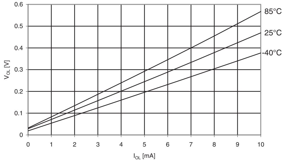
Figure 30-332. ATmega3290PA: I/O Pin Output Voltage vs. Sink Current, Ports A, C, D, E, F, G ( V_{CC} = 5V )
