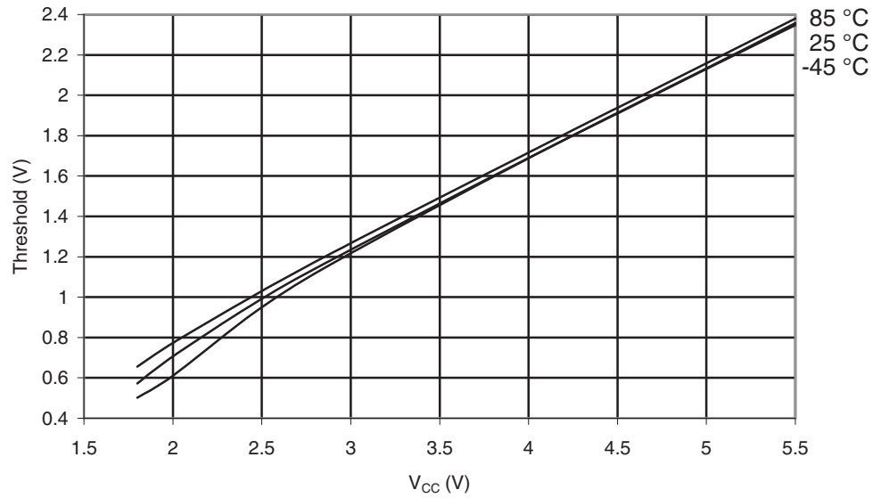
Figure 30-461. ATmega649P: I/O Pin Input Threshold Voltage vs. V_{CC} ( V_{IL} , I/O Pin Read as "0")
