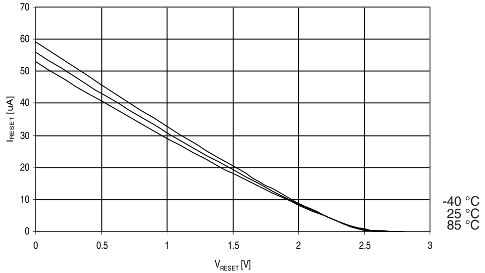
Figure 30-204. ATmega329PA: Reset Pull-up Resistor Current vs. Reset Pin Voltage ( V_{CC}=2.7V )
