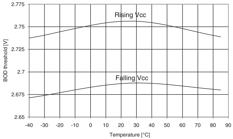
Figure 30-285. ATmega3290A: BOD Thresholds vs. Temperature (BOD Level is 2.7V)
