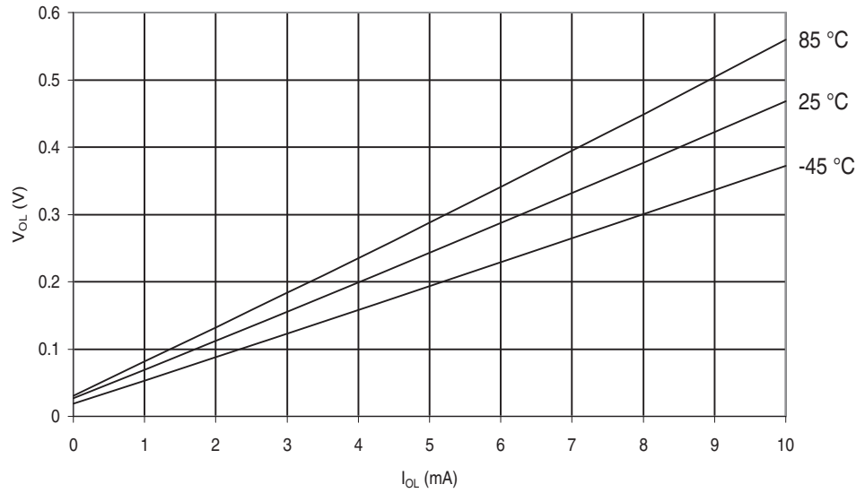
Figure 30-577. ATmega6490P: I/O Pin Output Voltage vs. Sink Current, Ports A, C, D, E, F, G ( V_{CC} = 2.7V )
