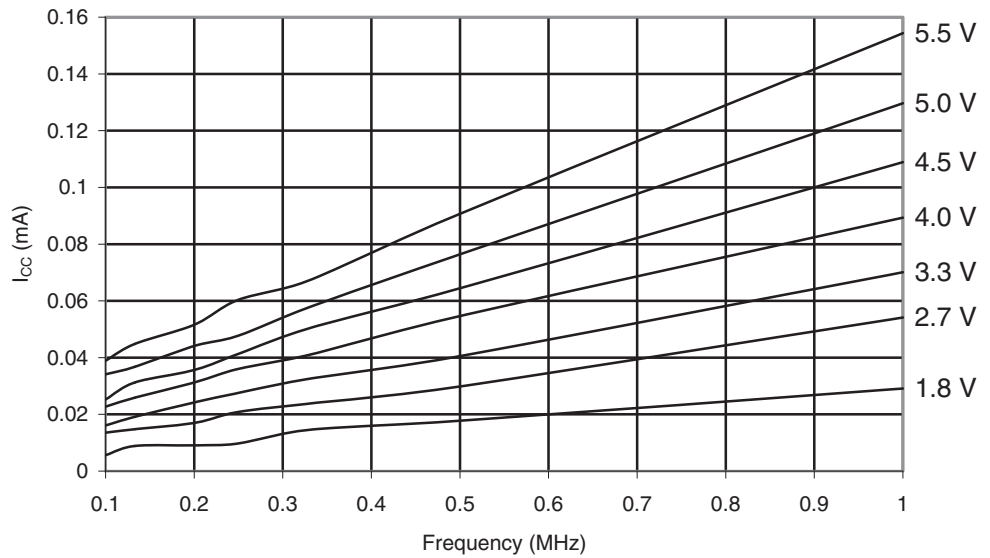
Figure 30-122. ATmega169PA: Reset Supply Current vs. V_{CC} (0.1 - 1.0MHz, Excluding Current Through The Reset Pull-up)
