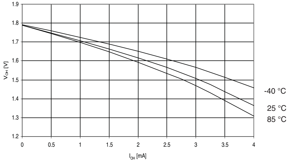
Figure 30-328. ATmega3290PA: I/O Pin Output Voltage vs. Source Current, Ports A, C, D, E, F, G ( V_{CC} = 1.8V )
