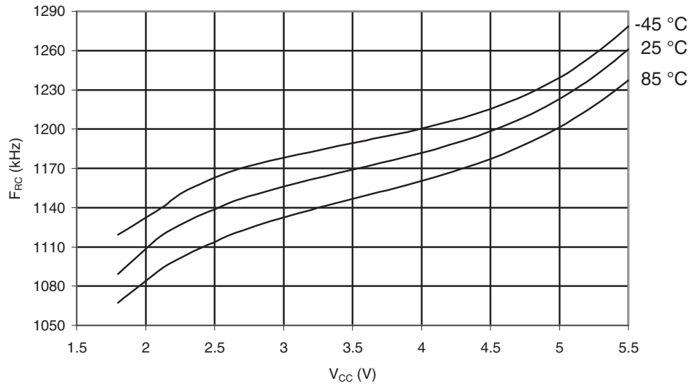
Figure 30-593. ATmega6490P: Watchdog Oscillator Frequency vs. V_{CC}
