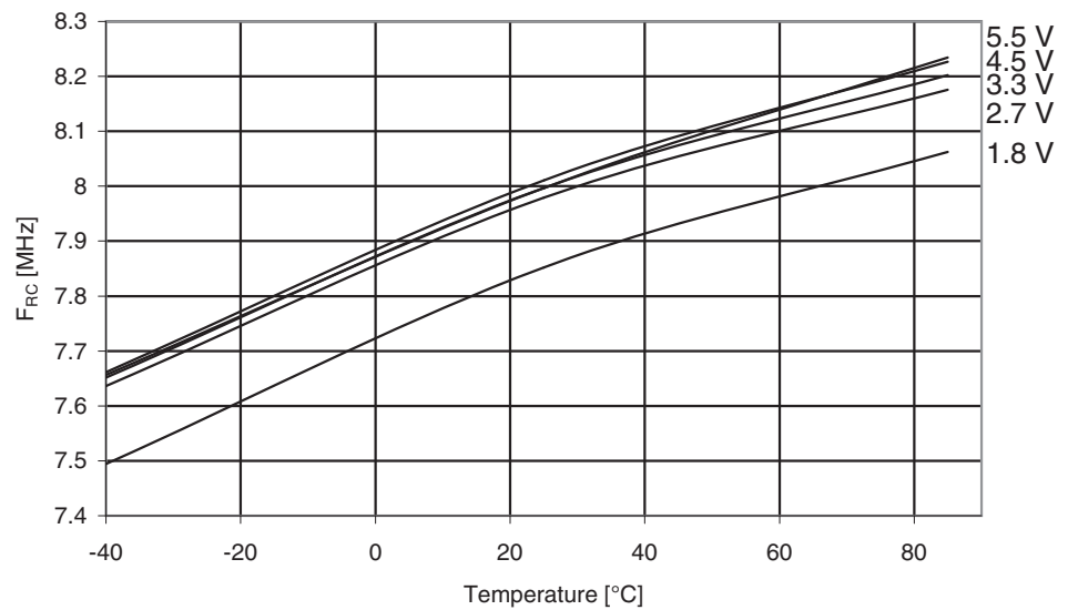
Figure 30-171. ATmega329A: Calibrated 8MHz RC Oscillator Frequency vs. Temperature
