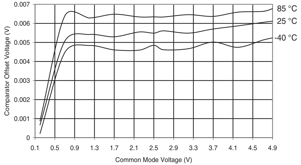
Figure 30-107. ATmega169PA: Analog Comparator Offset Voltage vs. Common Mode Voltage ( V_{CC} = 5V )
