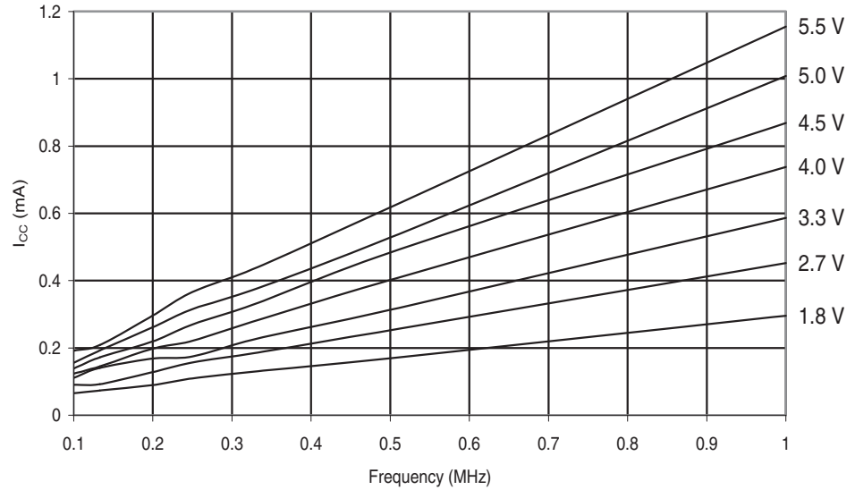
Figure 30-487. ATmega6490A: Active Supply Current vs. Low Frequency (0.1 - 1.0MHz)
