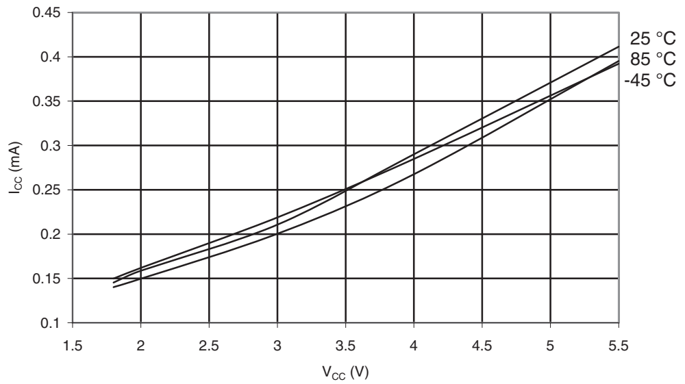
Figure 30-490. ATmega6490A: Active Supply Current vs. V_{CC} (Internal RC Oscillator, 1MHz)
