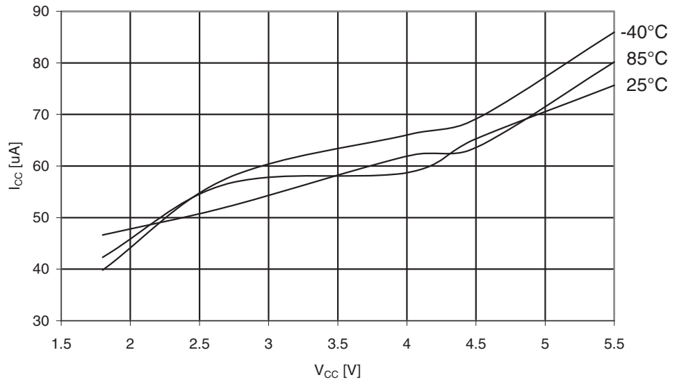
Figure 30-240. ATmega329PA: Analog Comparator Current vs. V_{CC}
