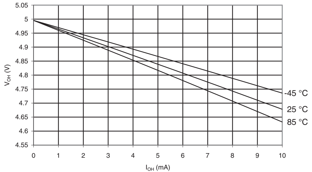
Figure 30-84. ATmega169PA: I/O Pin Output Voltage vs. Source Current, Ports A, C, D, E, F, G ( V_{CC} = 5V )
