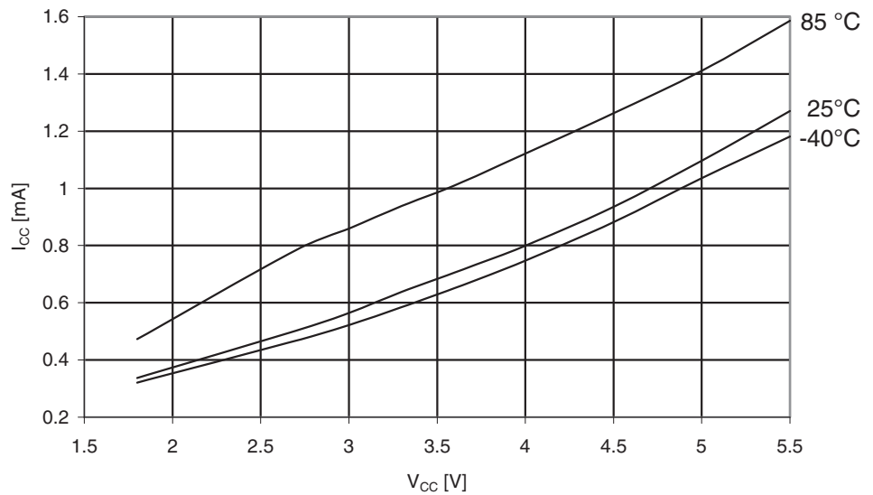
Figure 30-128. ATmega329A: Active Supply Current vs. V_{CC} (Internal RC Oscillator, 1MHz)
