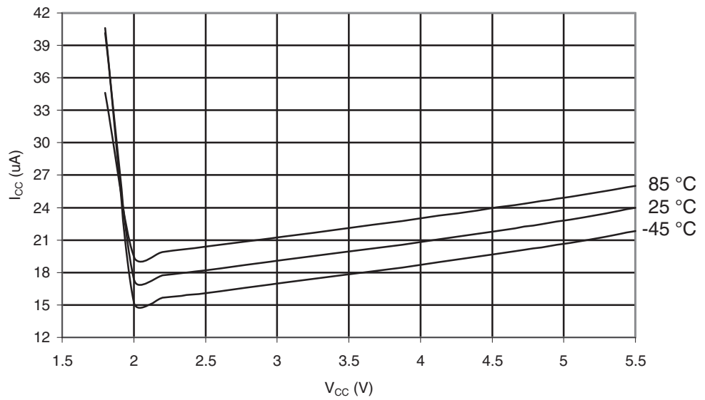
Figure 30-537. ATmega6490A: Brownout Detector Current vs. V_{CC}
