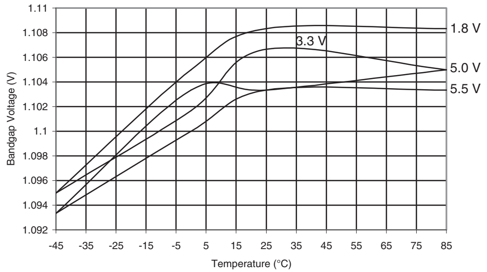
Figure 30-531. ATmega6490A: Bandgap Voltage vs. Temperature
