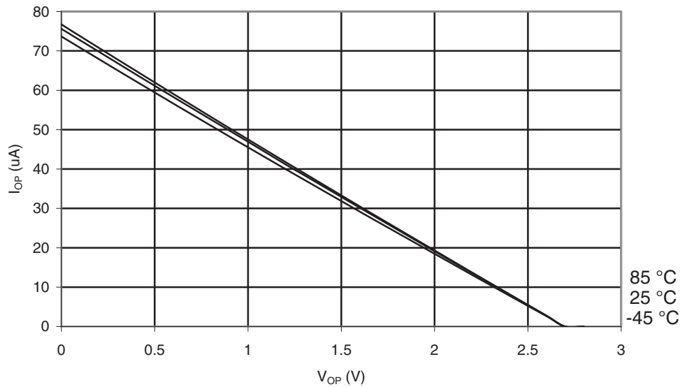
Figure 30-17. ATmega169A: I/O Pin Pull-up Resistor Current vs. Input Voltage ( V_{CC} = 2.7V )
