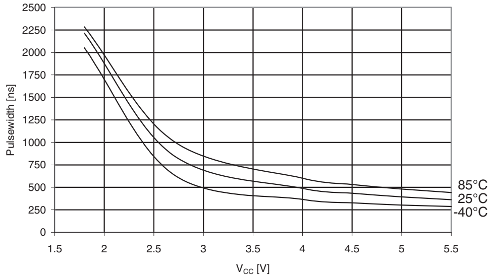
Figure 30-304. ATmega3290A: Minimum Reset Pulse Width vs. V_{CC}
