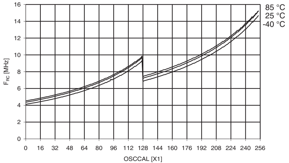
Figure 30-173. ATmega329A: Calibrated 8MHz RC Oscillator Frequency vs. Oscal Value
