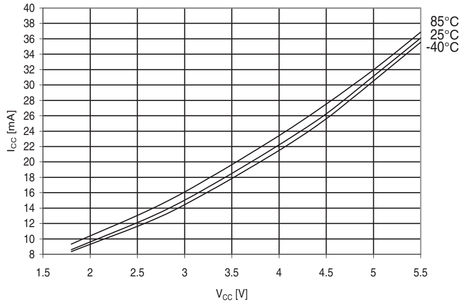
Figure 30-189. ATmega329PA: Active Supply Current vs. V_{CC} (32kHz Watch Crystal)
