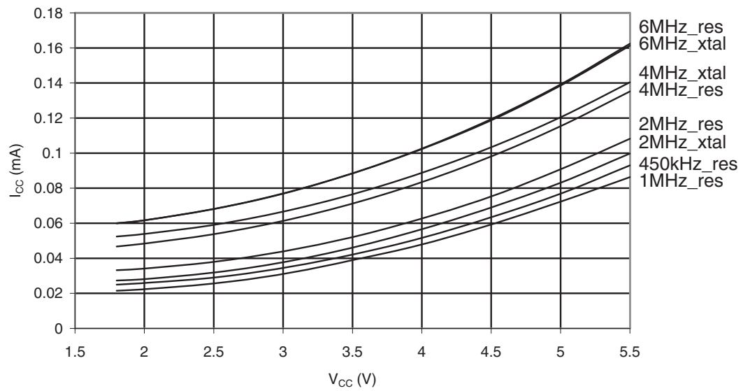
Figure 30-15. ATmega169A: Standby Supply Current vs. V_{CC} (Xtall and Resonator, Watchdog Timer Disabled)
