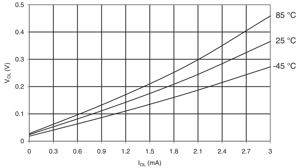
Figure 30-92. ATmega169PA: I/O Pin Output Voltage vs. Sink Current, Ports A, C, D, E, F, G ( V_{CC} = 1.8V )
