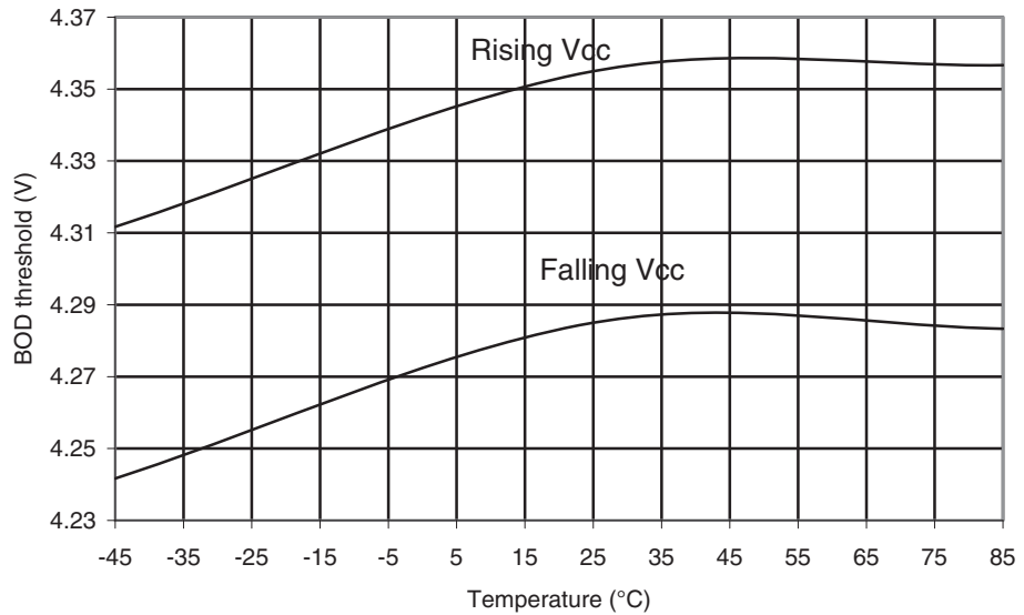
Figure 30-102. ATmega169PA: BOD Thresholds vs. Temperature (BOD Level is 4.3V)
