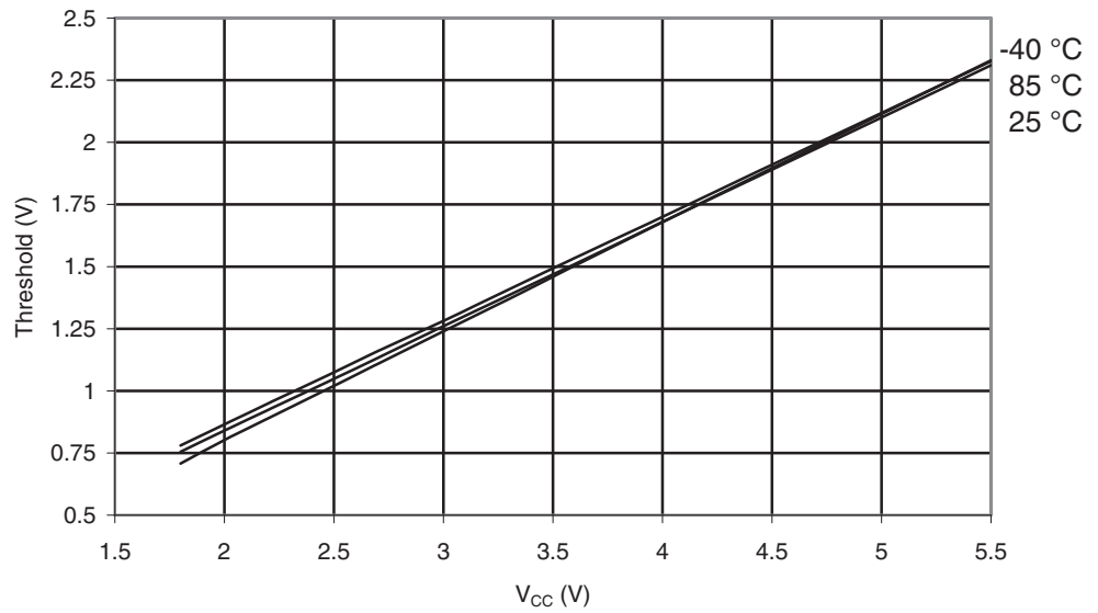
Figure 30-342. ATmega3290PA: Reset Input Threshold Voltage vs. V_{CC} ( V_{IL,Reset} Pin Read as "0")
