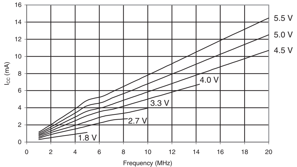
Figure 30-488. ATmega6490A: Active Supply Current vs. Frequency (1 - 20MHz)
