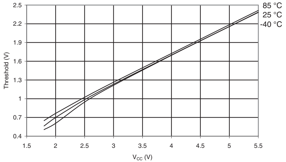
Figure 30-279. ATmega3290A: I/O Pin Input Threshold Voltage vs. V_{CC} ( V_{IL} , I/O Pin Read as "0")
