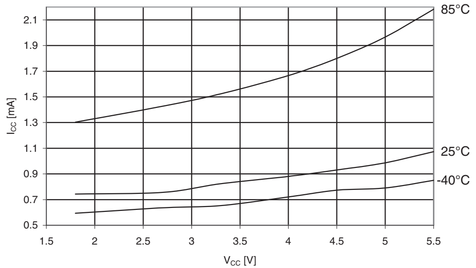
Figure 30-198. ATmega329PA Standby Supply Current vs. V_{CC} (32kHz Watch Crystal, Watchdog Timer Disabled)
