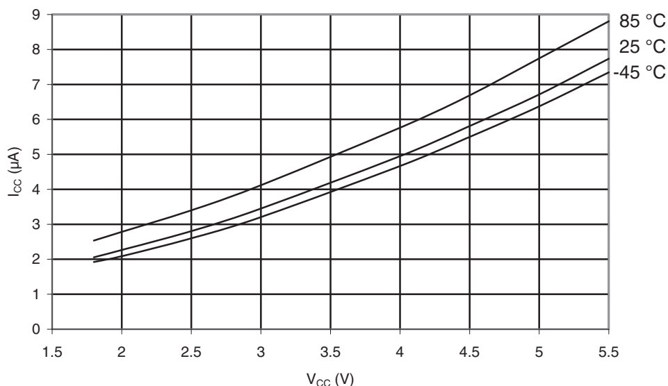
Figure 30-10. ATmega169A: Idle Supply Current vs. V_{CC} (32kHz Watch Crystal)
