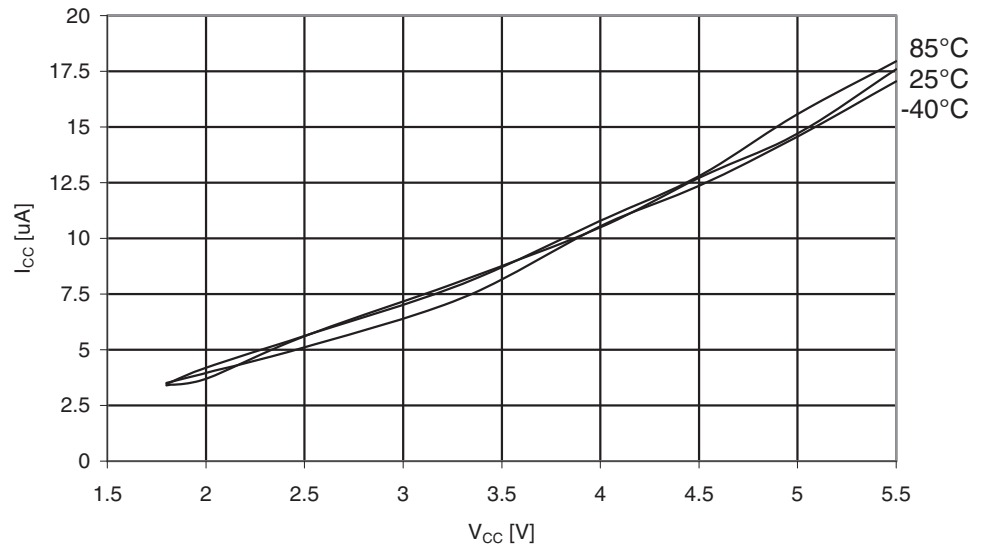
Figure 30-299. ATmega3290A: Watchdog Timer Current vs. V_{CC}
