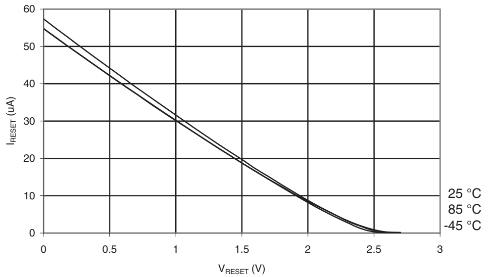
Figure 30-82. ATmega169PA: Reset Pull-up Resistor Current vs. Reset Pin Voltage ( V_{CC} = 2.7V )
