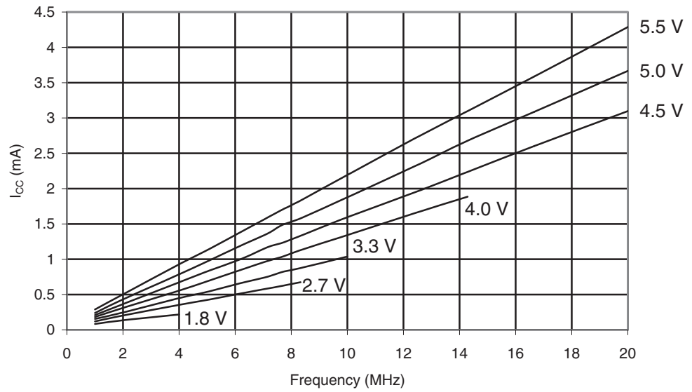
Figure 30-432. ATmega649P: Idle Supply Current vs. Frequency (1 - 20MHz)
