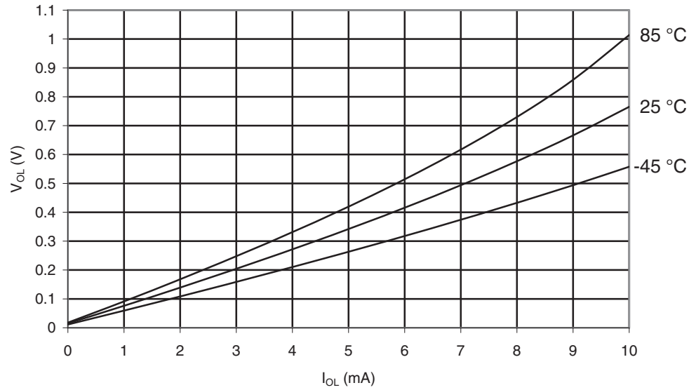
Figure 30-91. ATmega169PA. I/O Pin Output Voltage vs. Sink Current, Ports A, C, D, E, F, G ( V_{CC} = 2.7V )
