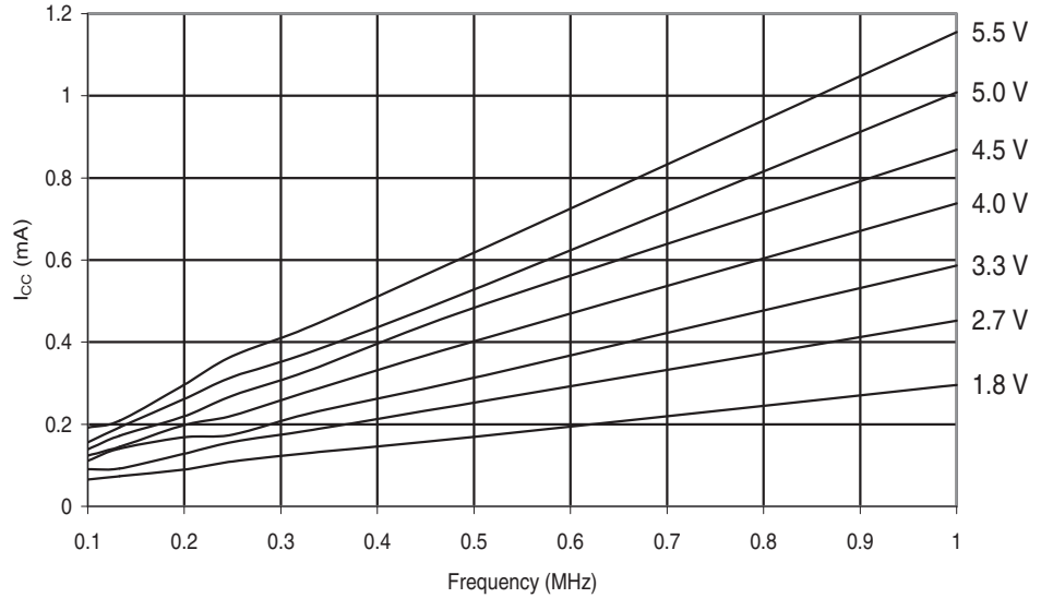
Figure 30-426. ATmega649P: Active Supply Current vs. Low Frequency (0.1 - 1.0MHz)
