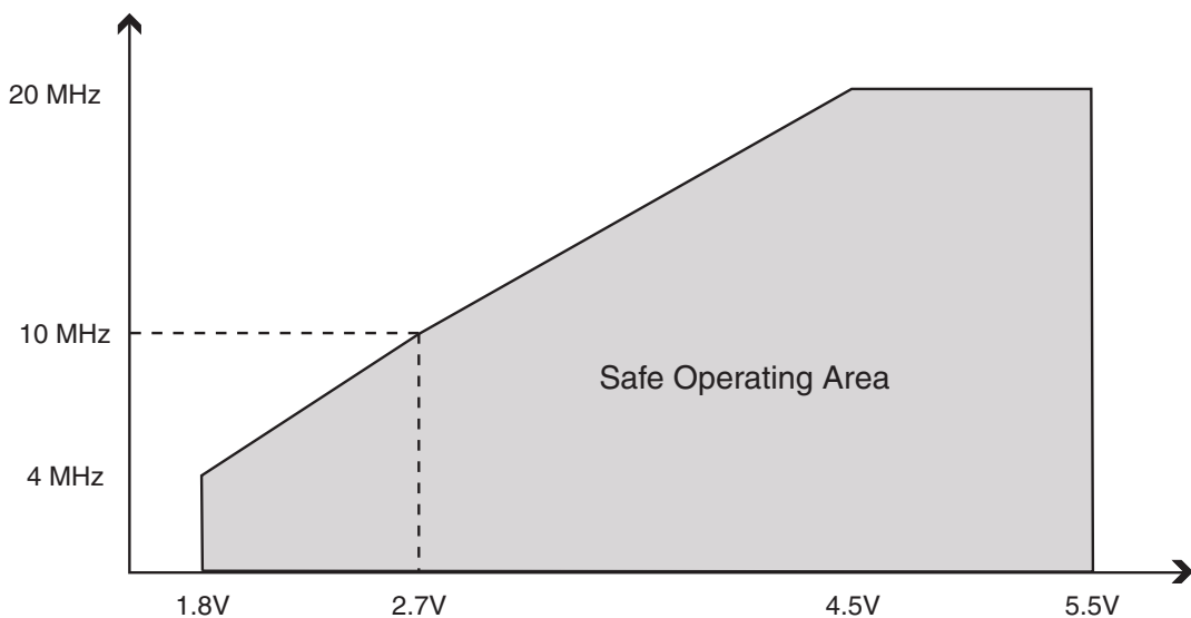
Figure 29-2. Maximum Frequency vs. V_{CC} (0 - 20MHz) ATmega329A/ATmega329PA/ATmega3290A/ATmega3290PA/ATmega6490A/ ATmega6490P
