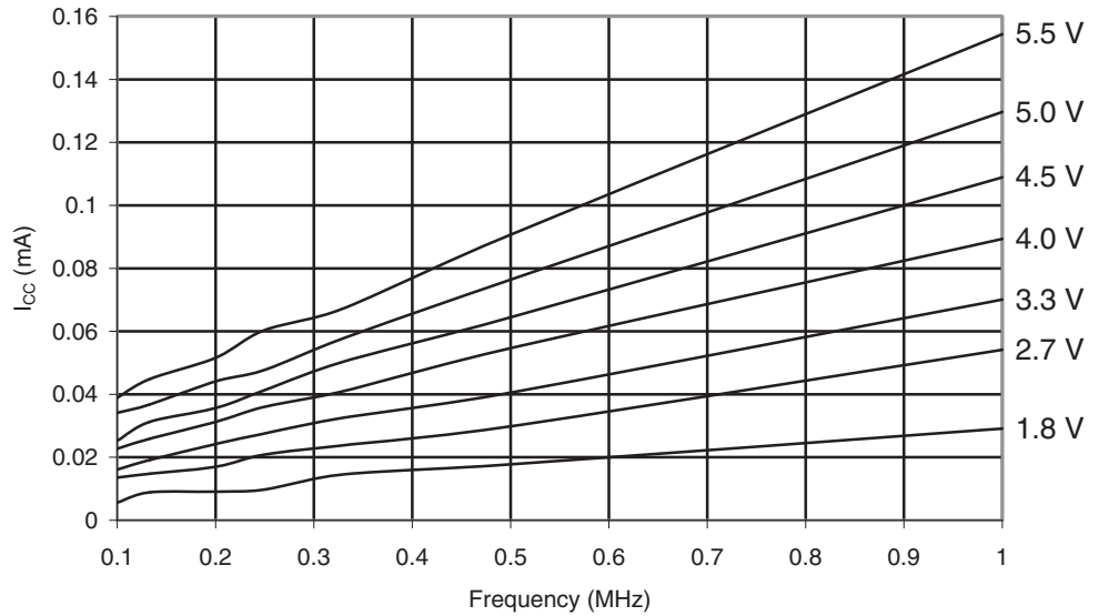
Figure 30-60. ATmega169A: Reset Supply Current vs. V_{CC} (0.1 - 1.0MHz, Excluding Current Through The Reset Pull-up)
