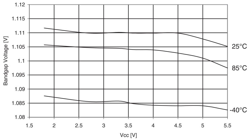
Figure 30-347. ATmega3290PA: Bandgap Voltage vs. V_{CC}
