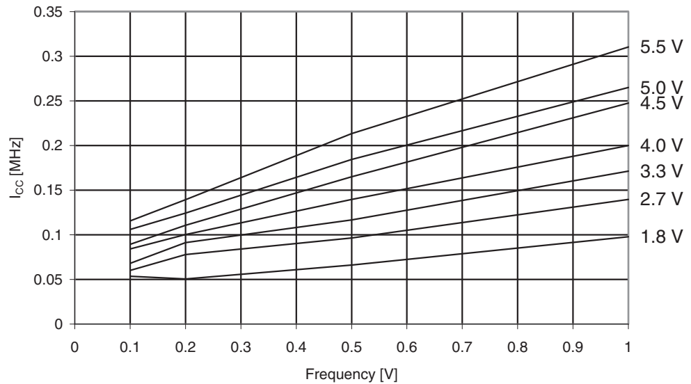
Figure 30-130. ATmega329A: Idle Supply Current vs. Low Frequency (0.1 - 1.0MHz)
