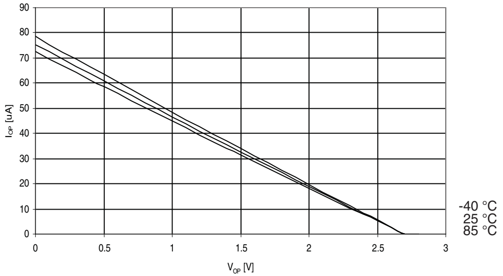
Figure 30-141. ATmega329A: I/O Pin Pull-up Resistor Current vs. Input Voltage ( V_{CC} = 2.7V )
