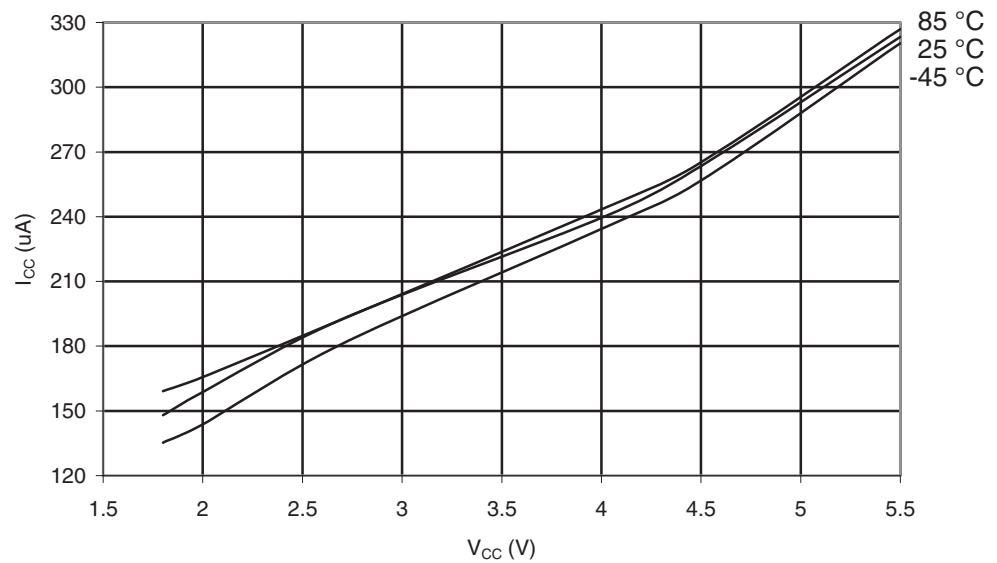
Figure 30-477. ATmega649P: Active Supply Current with ADC at 50kHz vs. V_{CC}
