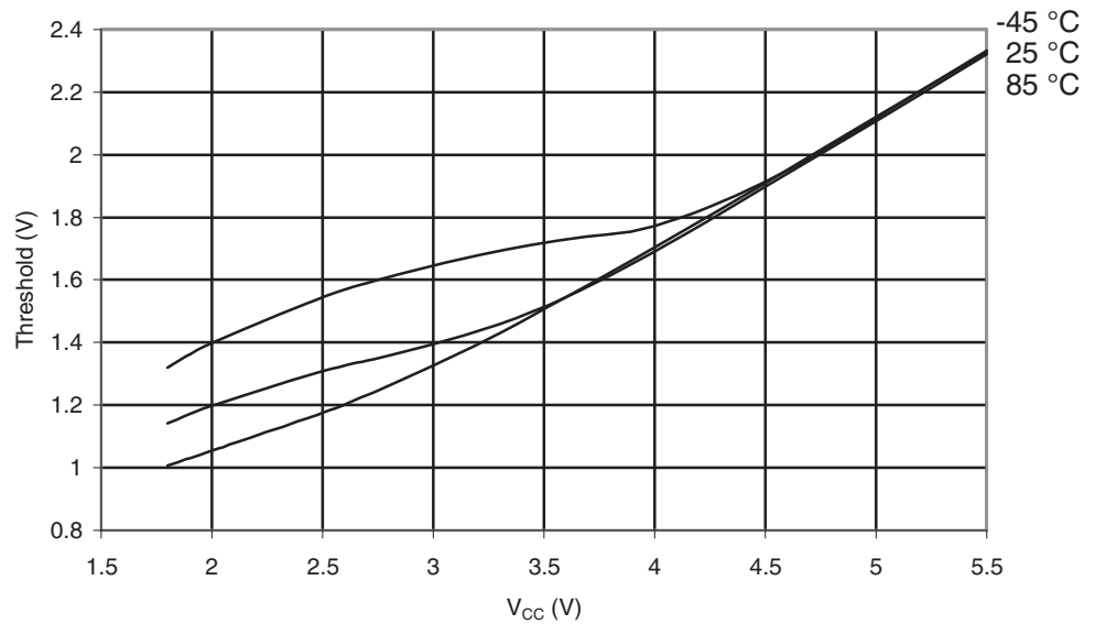
Figure 30-524. ATmega6490A: Reset Input Threshold Voltage vs. V_{CC} ( V_{IH,Reset} Pin Read as "1")
