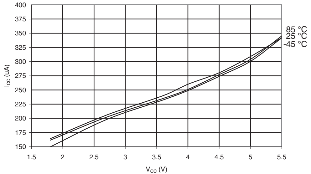
Figure 30-53. ATmega169A: Active Supply Current with ADC at 50kHz vs. V_{CC}
