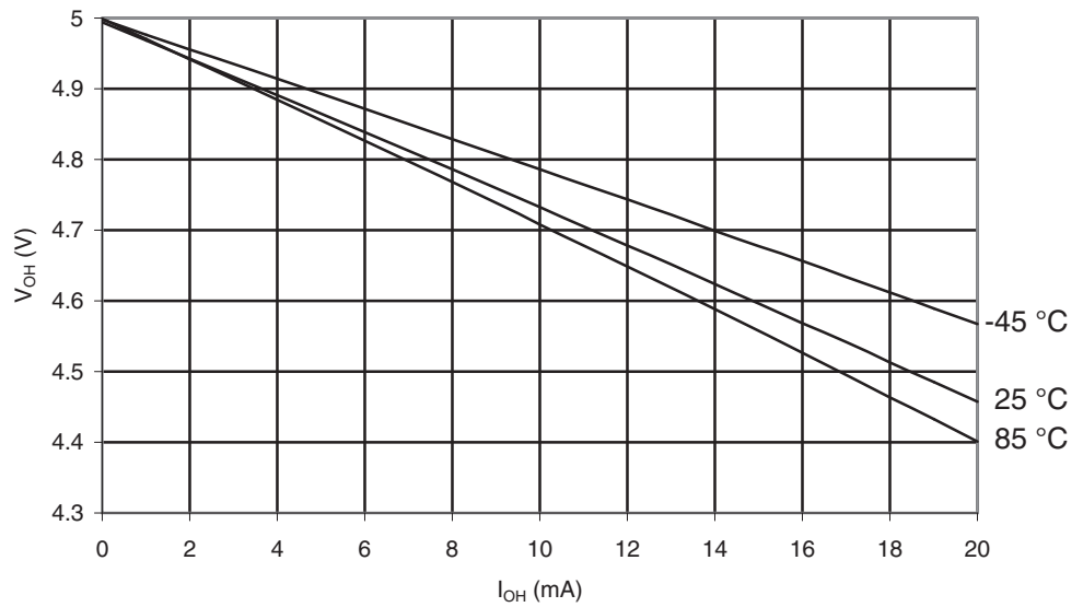
Figure 30-512. ATmega6490A: I/O Pin Output Voltage vs. Source Current, Port B ( V_{CC} = 5V )
