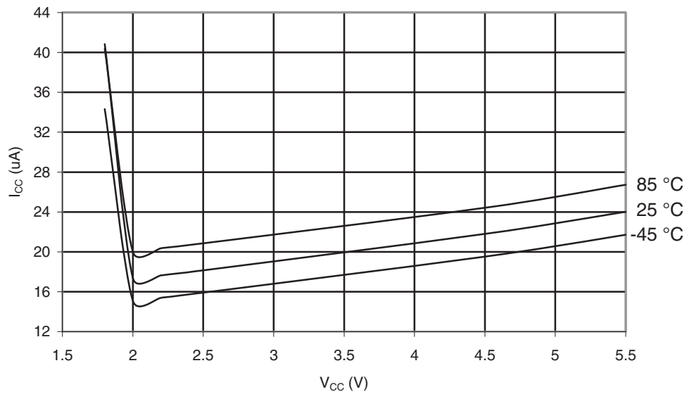
Figure 30-114. ATmega169PA: Brownout Detector Current vs. V_{CC}
