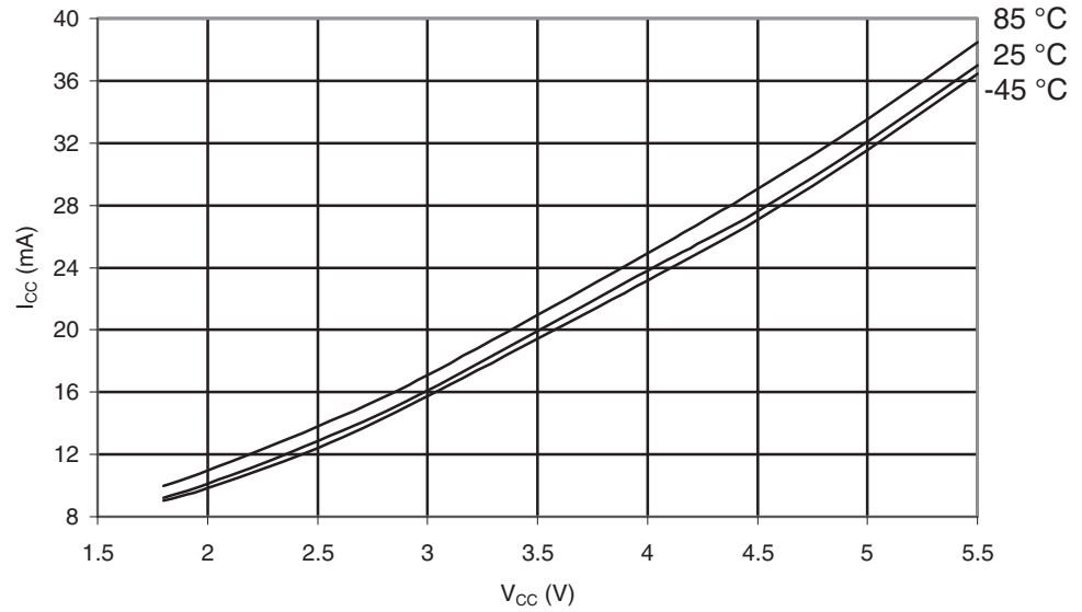
Figure 30-369. ATmega649A: Active Supply Current vs. V_{CC} (32kHz Watch Crystal)
