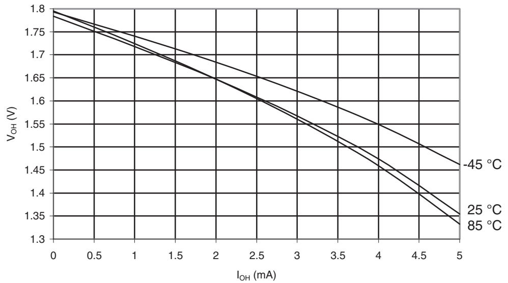
Figure 30-453. ATmega649P: I/O Pin Output Voltage vs. Source Current, Port B ( V_{CC} = 1.8V )
