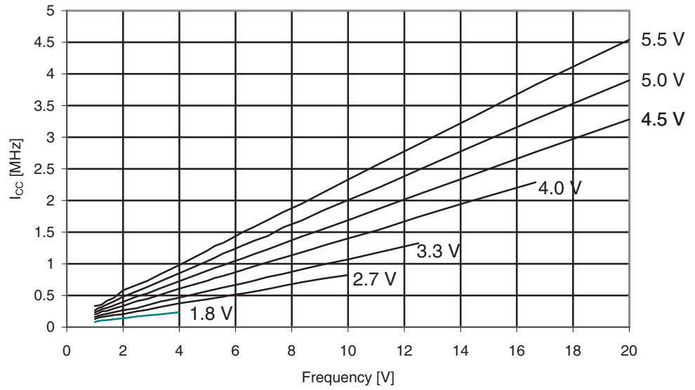
Figure 30-251. ATmega3290A: Idle Supply Current vs. Frequency (1 - 20MHz)
