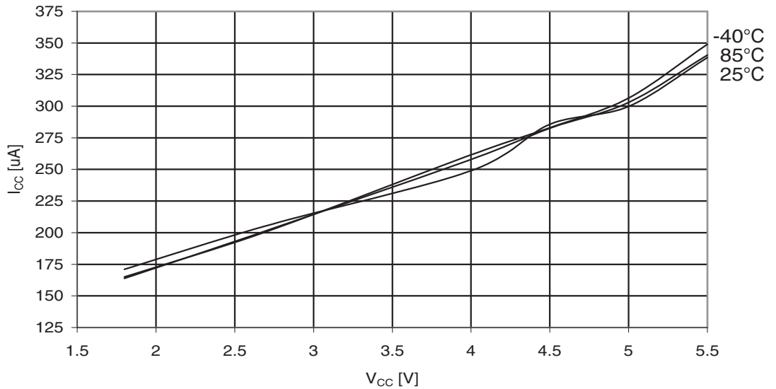
Figure 30-237. ATmega329PA: Active Supply Current with ADC at 1MHz vs. V_{CC}
