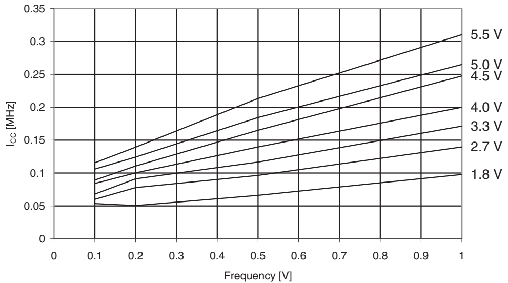
Figure 30-190. ATmega329PA: Idle Supply Current vs. Low Frequency (0.1 - 1.0MHz)
