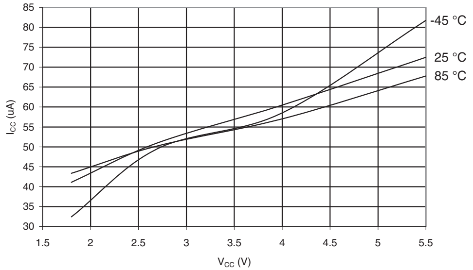
Figure 30-58. ATmega169A: Analog Comparator Current vs. V_{CC}
