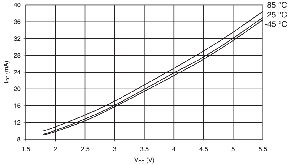
Figure 30-552. ATmega6490P: Active Supply Current vs. V_{CC} (32kHz Watch Crystal)
