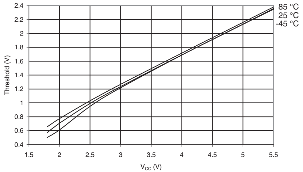
Figure 30-400. ATmega649A: I/O Pin Input Threshold Voltage vs. V_{CC} ( V_{IL} , I/O Pin Read as "0")
