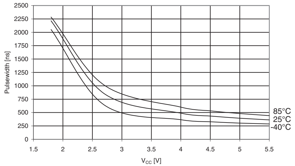
Figure 30-244. ATmega329PA: Minimum Reset Pulse Width vs. V_{CC}
