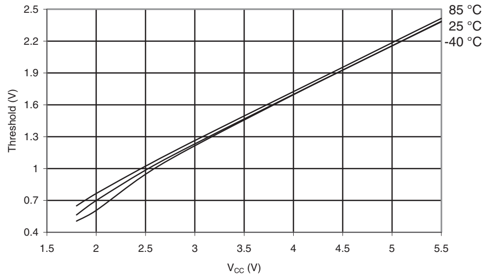
Figure 30-219. ATmega329PA: I/O Pin Input Threshold Voltage vs. V_{CC} ( V_{IL} , I/O Pin Read as "0")
