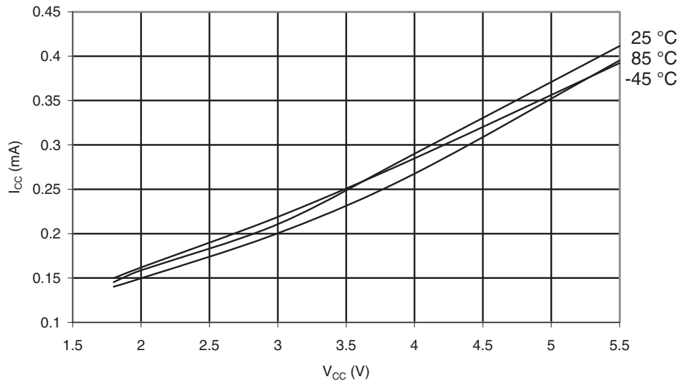
Figure 30-434. ATmega649P: Idle Supply Current vs. V_{CC} (Internal RC Oscillator, 1MHz)
