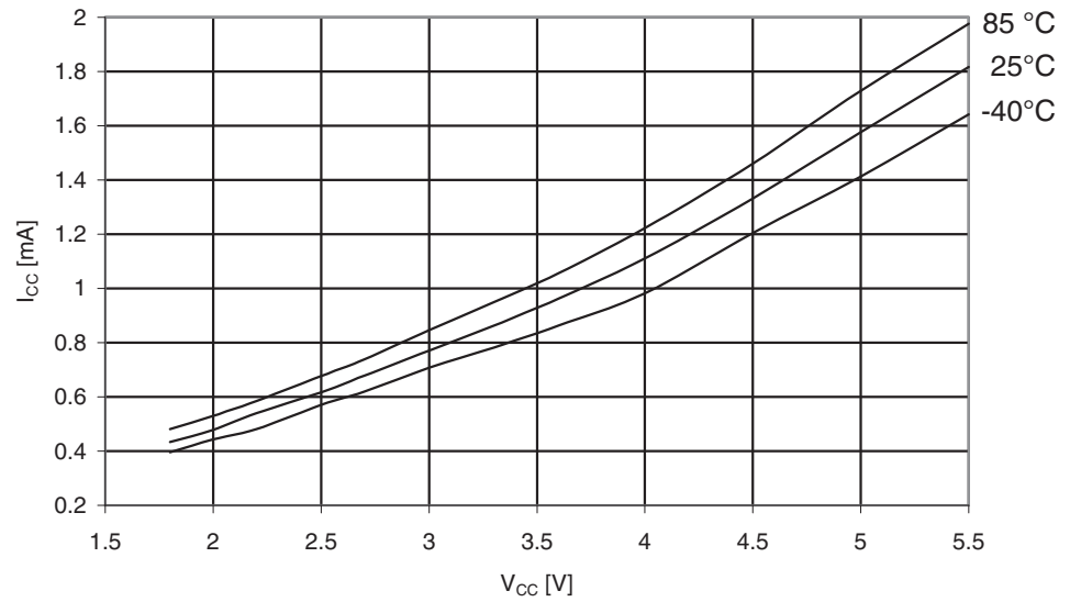
Figure 30-192. ATmega329PA: Idle Supply Current vs. V_{CC} (Internal RC Oscillator, 8MHz)
