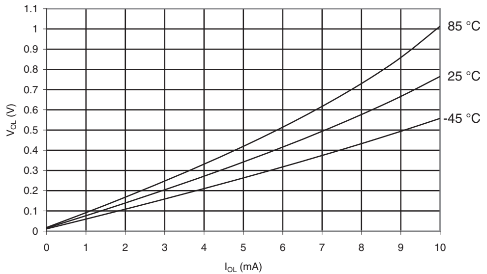
Figure 30-90. ATmega169PA: I/O Pin Output Voltage vs. Sink Current, Ports A, C, D, E, F, G ( V_{CC} = 5V )
