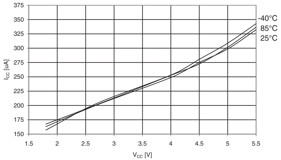
Figure 30-355. ATmega3290PA: Active Supply Current with ADC at 50kHz vs. V_{CC}
