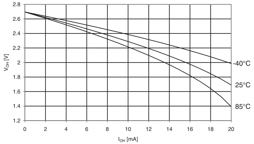
Figure 30-150. ATmega329A: I/O Pin Output Voltage vs. Source Current, Port B ( V_{CC} = 2.7V )
