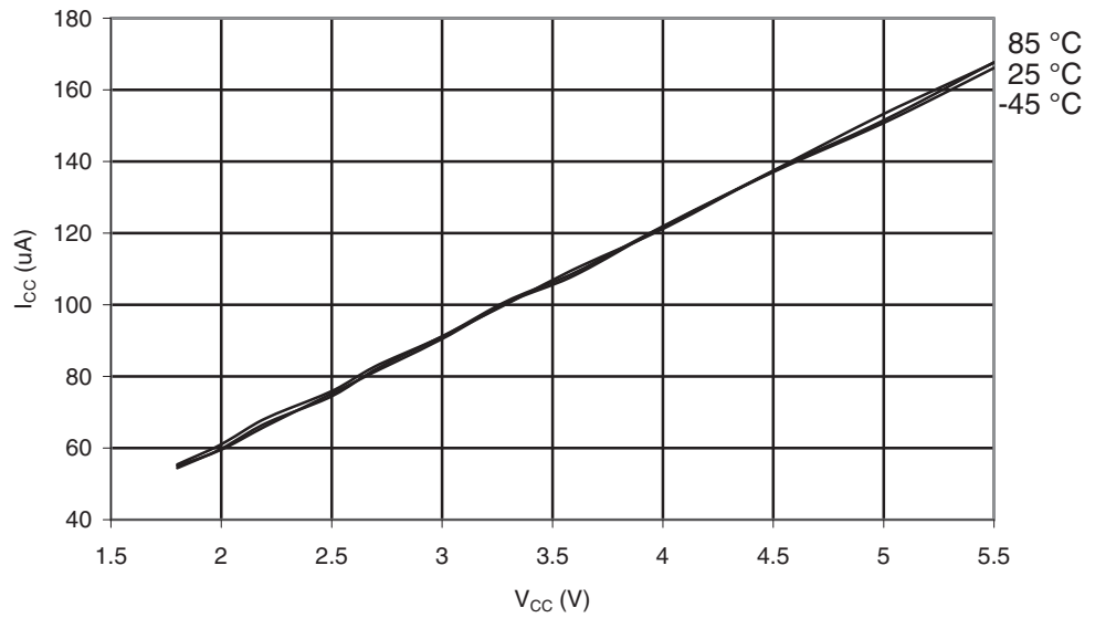
Figure 30-56. ATmega169A: AREF External Reference Current vs. V_{CC}
