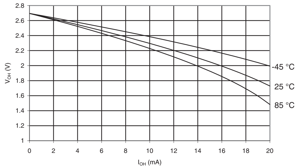
Figure 30-88. ATmega169PA: I/O Pin Output Voltage vs. Source Current, Port B ( V_{CC} = 2.7V )
