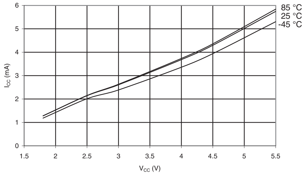
Figure 30-3. ATmega169A: Active Supply Current vs. V_{CC} (Internal RC Oscillator, 8MHz)
