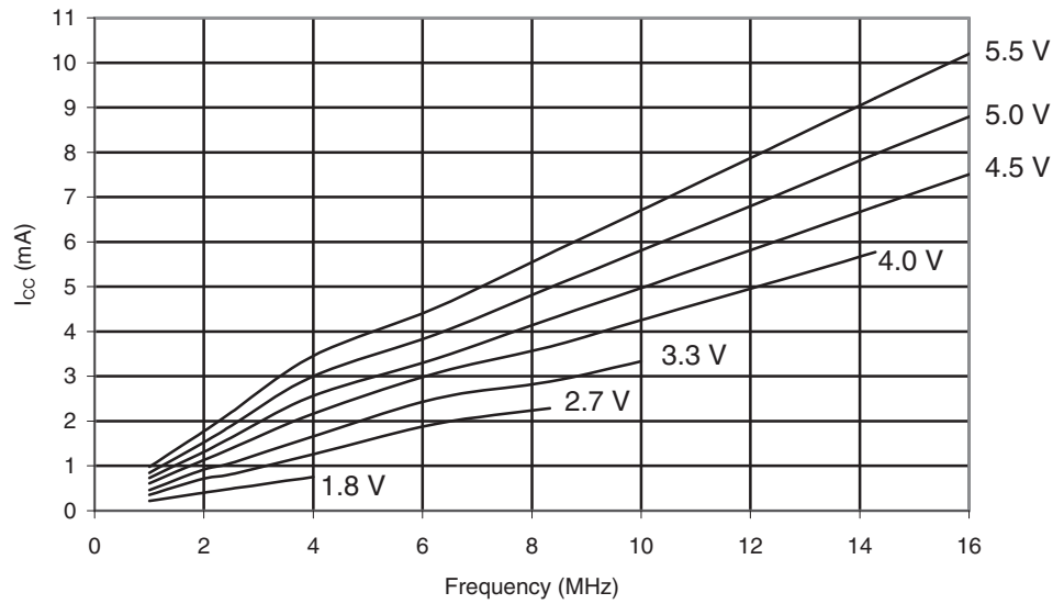
Figure 30-2. ATmega169A: Active Supply Current vs. Frequency (1 - 16MHz)
