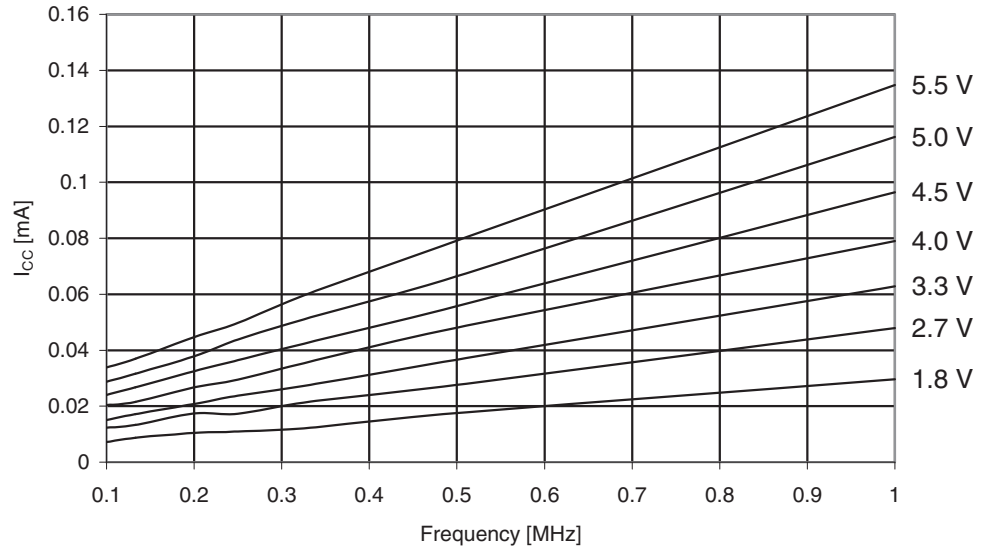
Figure 30-182. ATmega329A: Reset Supply Current vs. V_{CC} (0.1 - 1.0MHz, Excluding Current Through The Reset Pull-up)
