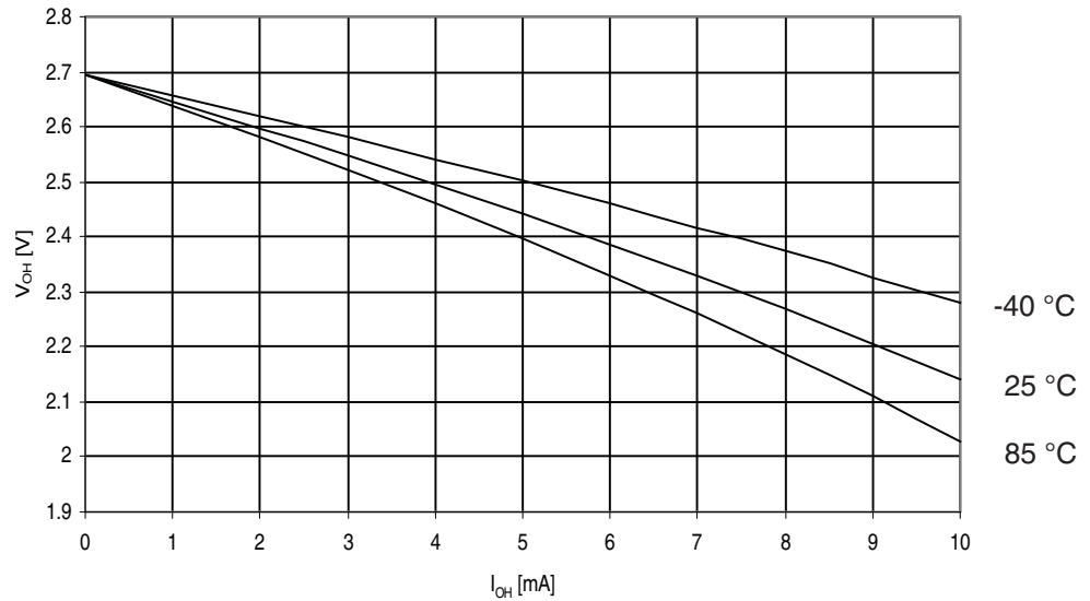
Figure 30-327. ATmega3290PA: I/O Pin Output Voltage vs. Source Current, Ports A, C, D, E, F, G ( V_{CC} = 2.7V )
