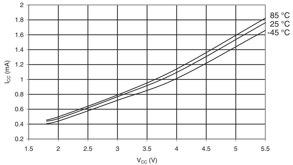
Figure 30-494. ATmega6490A: Idle Supply Current vs. V_{CC} (Internal RC Oscillator, 8MHz)
