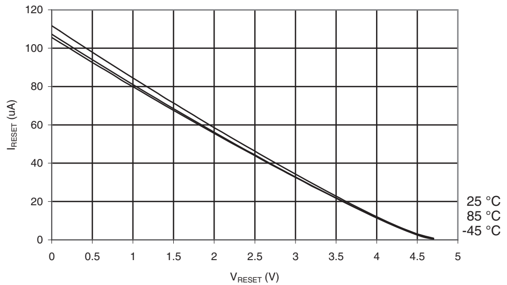
Figure 30-19. ATmega169A: Reset Pull-up Resistor Current vs. Reset Pin Voltage ( V_{CC} = 5V )
