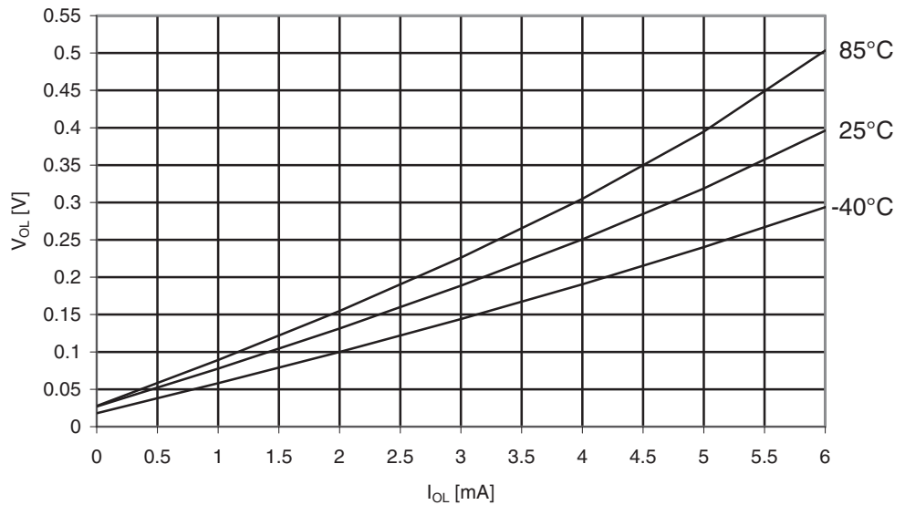
Figure 30-337. ATmega3290PA: I/O Pin Output Voltage vs. Sink Current, Port B ( V_{CC} = 1.8V )
