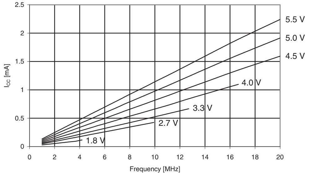
Figure 30-303. ATmega3290A: Reset Supply Current vs. V_{CC} (1 - 20MHz, Excluding Current Through The Reset Pull-up)
