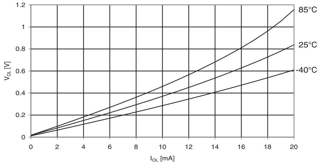
Figure 30-276. ATmega3290A: I/O Pin Output Voltage vs. Sink Current, Port B ( V_{CC} = 2.7V )
