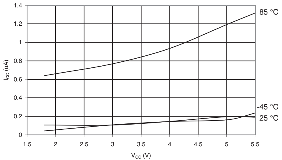
Figure 30-11. ATmega169A: Power-down Supply Current vs. V_{CC} (Watchdog Timer Disabled)
