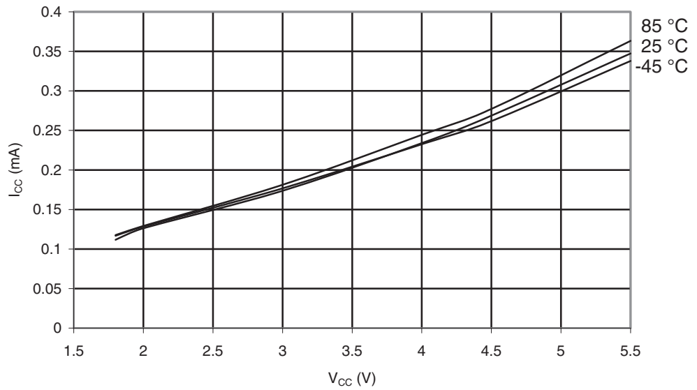
Figure 30-71. ATmega169PA: Idle Supply Current vs. V_{CC} (Internal RC Oscillator, 1MHz)
