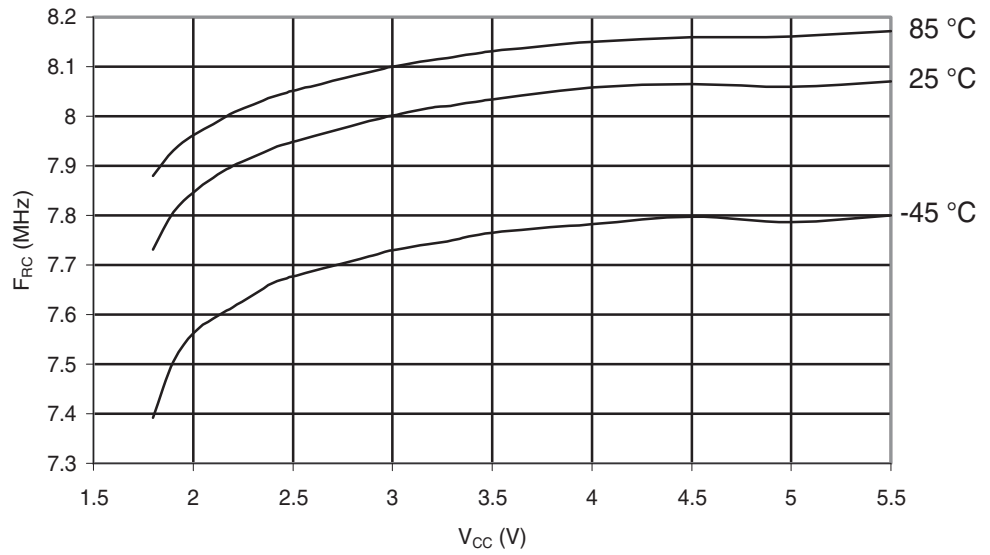
Figure 30-413. ATmega649A: Calibrated 8MHz RC Oscillator Frequency vs. V_{CC}
