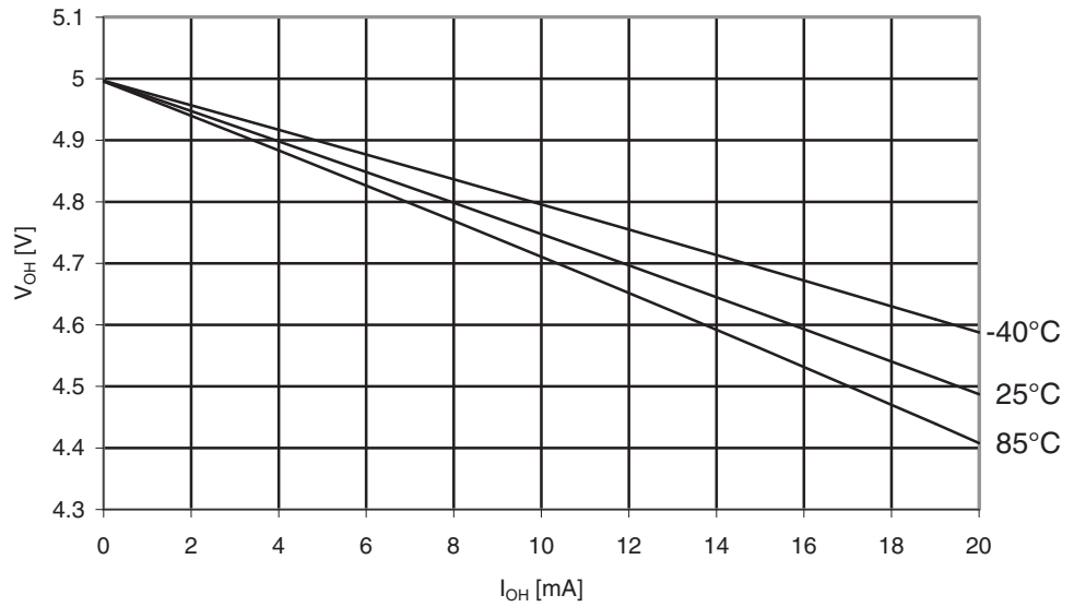
Figure 30-269. ATmega3290A: I/O Pin Output Voltage vs. Source Current, Port B ( V_{CC} = 5V )
