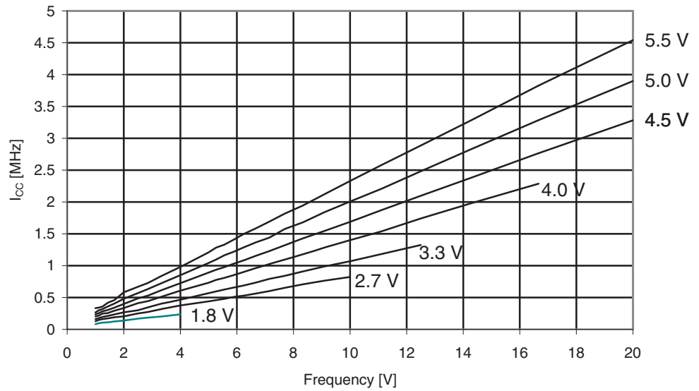
Figure 30-131. ATmega329A: Idle Supply Current vs. Frequency (1 - 20MHz)
