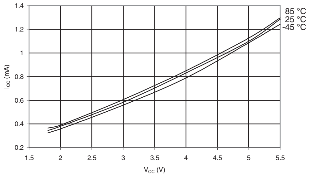
Figure 30-429. ATmega649P: Active Supply Current vs. V_{CC} (Internal RC Oscillator, 1MHz)
