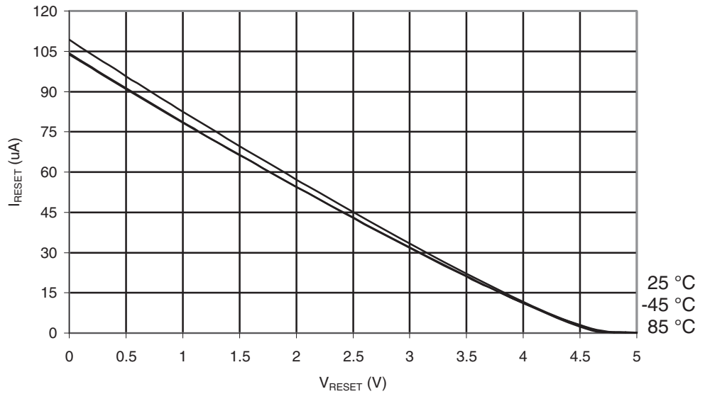
Figure 30-445. ATmega649P: Reset Pull-up Resistor Current vs. Reset Pin Voltage ( V_{CC} = 5V )
