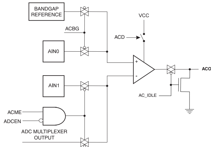
Figure 26-6. Analog Comparator
