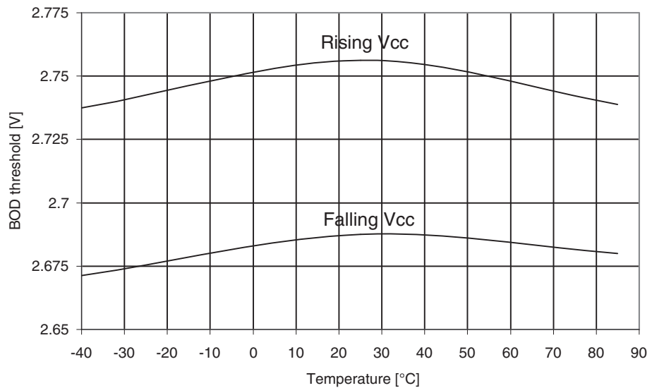
Figure 30-225. ATmega329PA: BOD Thresholds vs. Temperature (BOD Level is 2.7V)
