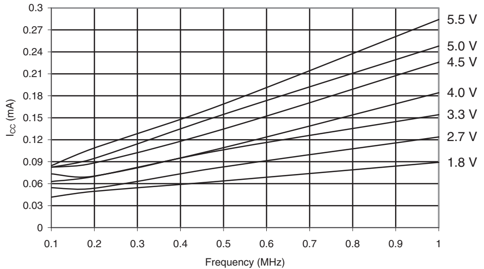
Figure 30-492. ATmega6490A: Idle Supply Current vs. Low Frequency (0.1 - 1.0MHz)
