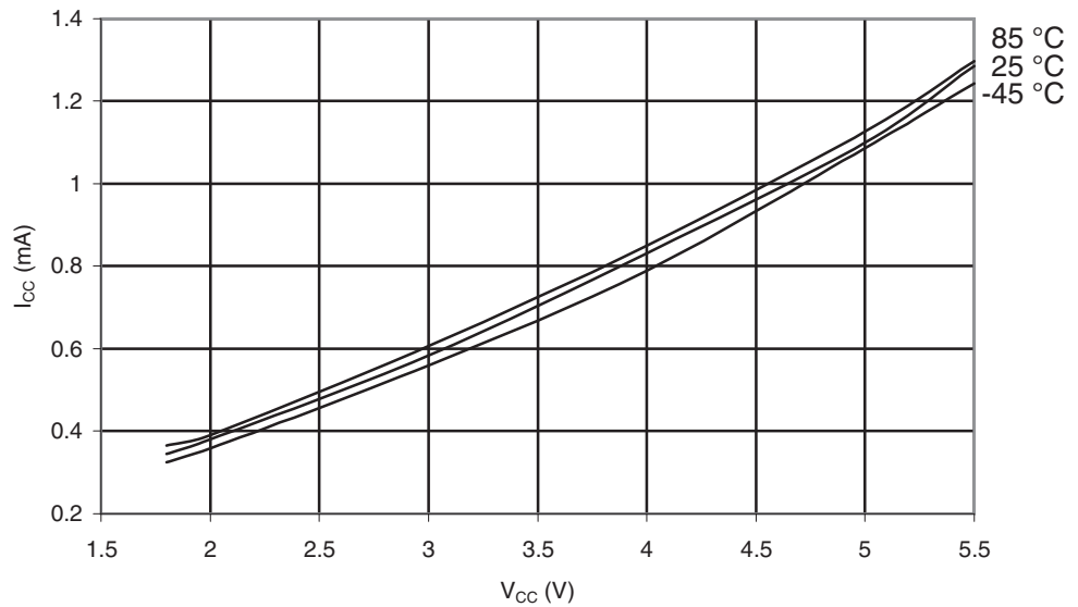
Figure 30-556. ATmega6490P: Idle Supply Current vs. V_{CC} (Internal RC Oscillator, 1MHz)
