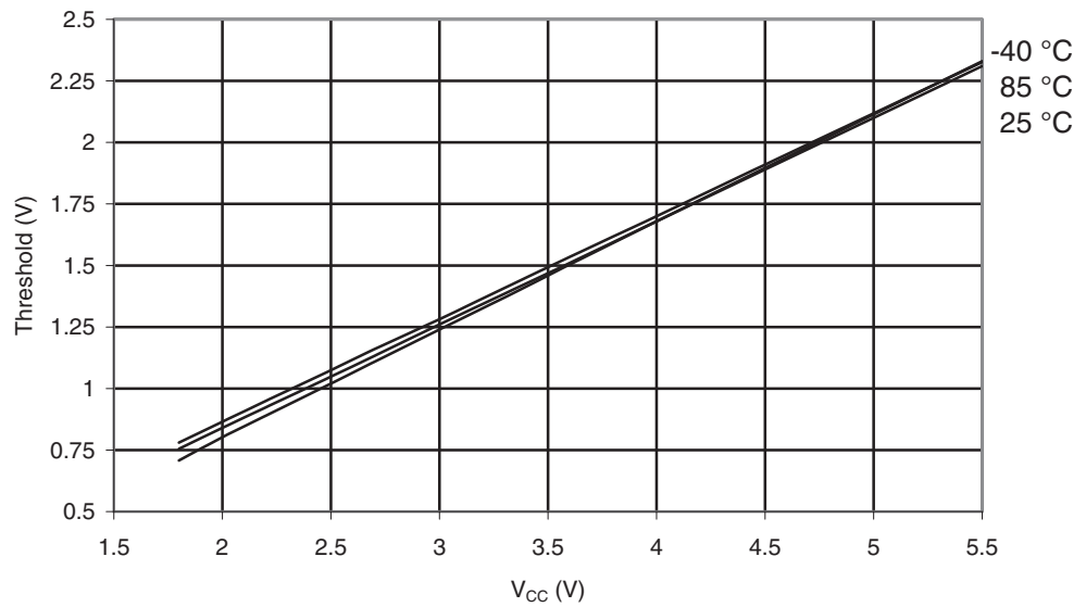
Figure 30-282. ATmega3290A: Reset Input Threshold Voltage vs. V_{CC} ( V_{IL} , Reset Pin Read as "0")
