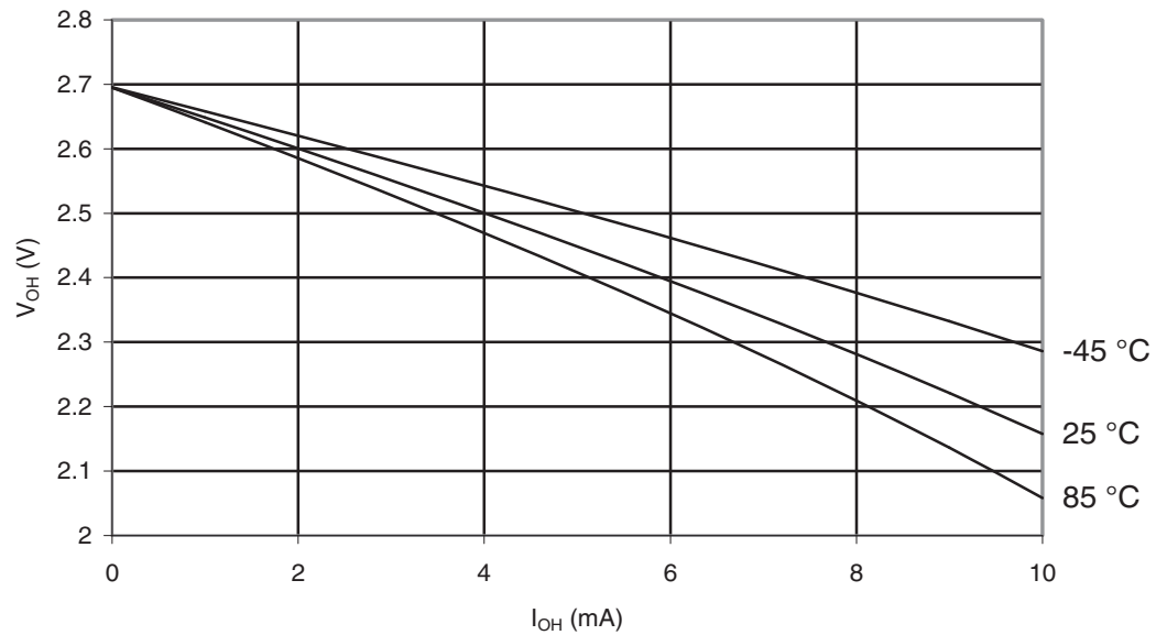
Figure 30-23. ATmega169A: I/O Pin Output Voltage vs. Source Current, Ports A, C, D, E, F, G ( V_{CC} = 2.7V )
