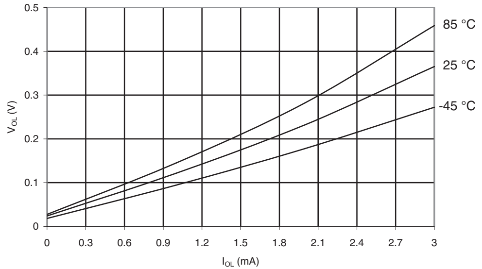
Figure 30-30. ATmega169A: I/O Pin Output Voltage vs. Sink Current, Ports A, C, D, E, F, G ( V_{CC} = 1.8V )
