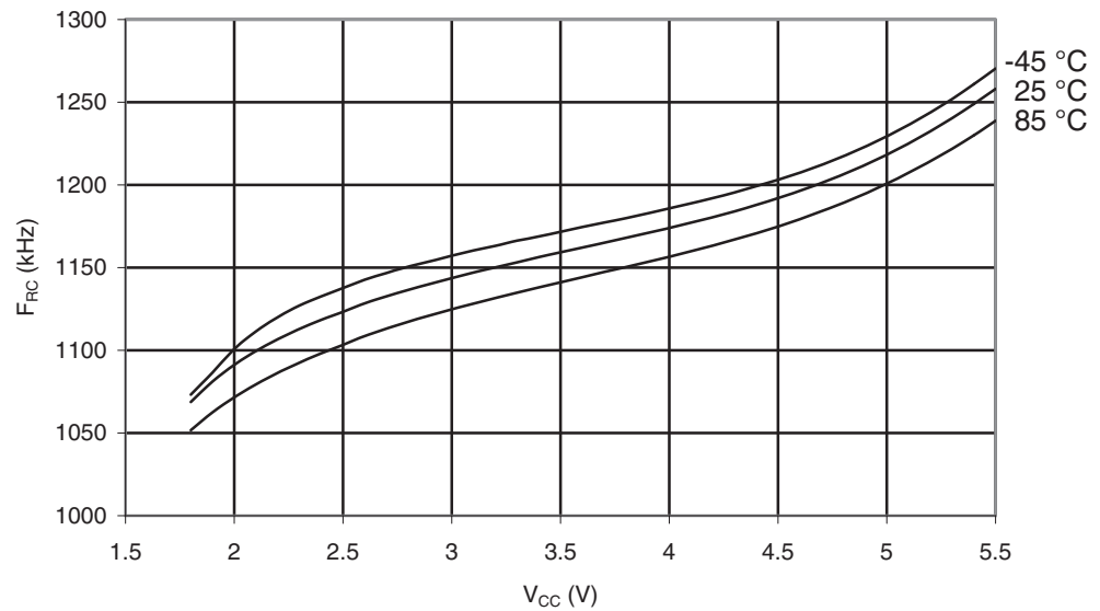
Figure 30-47. ATmega169A: Watchdog Oscillator Frequency vs. V_{CC}
