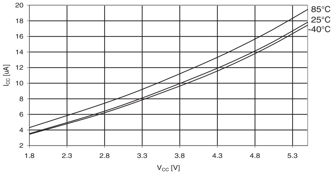
Figure 30-136. ATmega329A: Power-down Supply Current vs. V_{CC} (Watchdog Timer Enabled)
