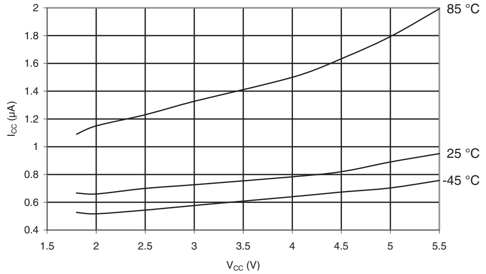
Figure 30-14. ATmega169A Standby Supply Current vs. V_{CC} (32kHz Watch Crystal, Watchdog Timer Disabled)
