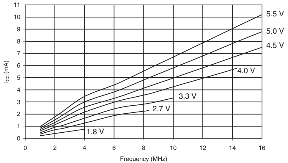
Figure 30-64. ATmega169PA: Active Supply Current vs. Frequency (1 - 16MHz)
