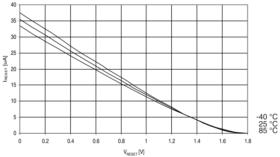
Figure 30-325. ATmega3290PA: Reset Pull-up Resistor Current vs. Reset Pin Voltage ( V_{CC}=1.8V )
