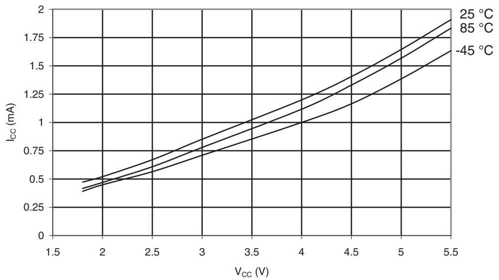
Figure 30-70. ATmega169PA: Idle Supply Current vs. V_{CC} (Internal RC Oscillator, 8MHz)
