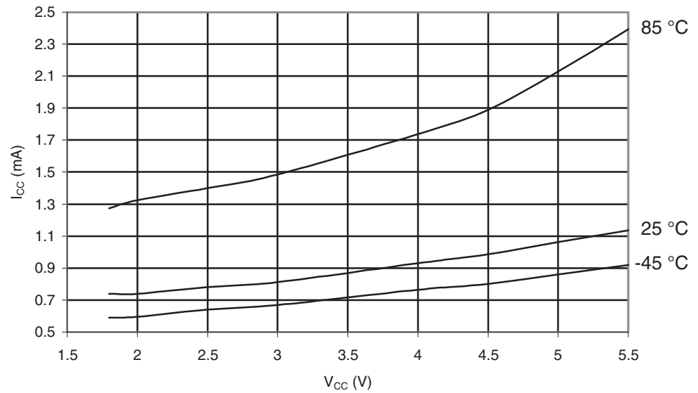
Figure 30-500. ATmega6490A: Power-save Supply Current vs. V_{CC} (Watchdog Timer Disabled and 32kHz Crystal Oscillator Running)
