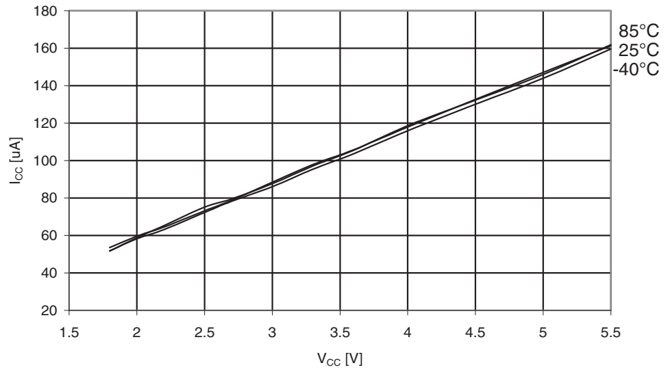
Figure 30-178. ATmega329A: AREF External Reference Current vs. V_{CC}
