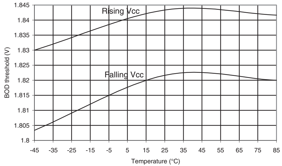
Figure 30-529. ATmega6490A: BOD Thresholds vs. Temperature (BOD Level is 1.8V)
