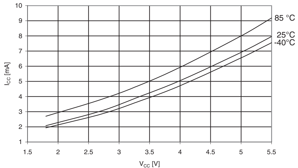
Figure 30-194. ATmega329PA: Idle Supply Current vs. V_{CC} (32kHz Watch Crystal)
