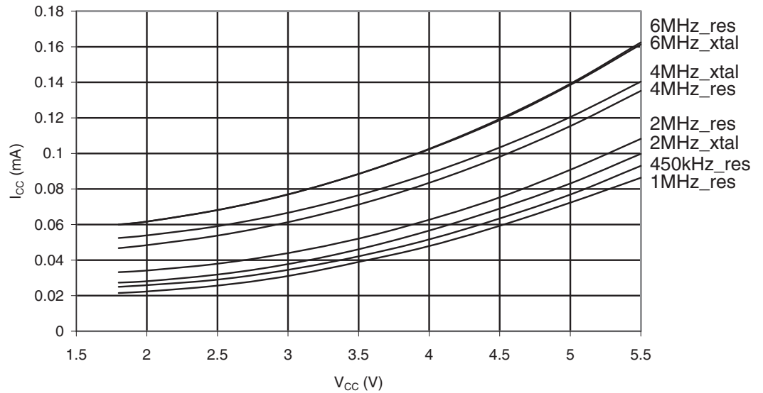
Figure 30-77. ATmega169PA: Standby Supply Current vs. V_{CC} (Xtall and Resonator, Watchdog Timer Disabled)
