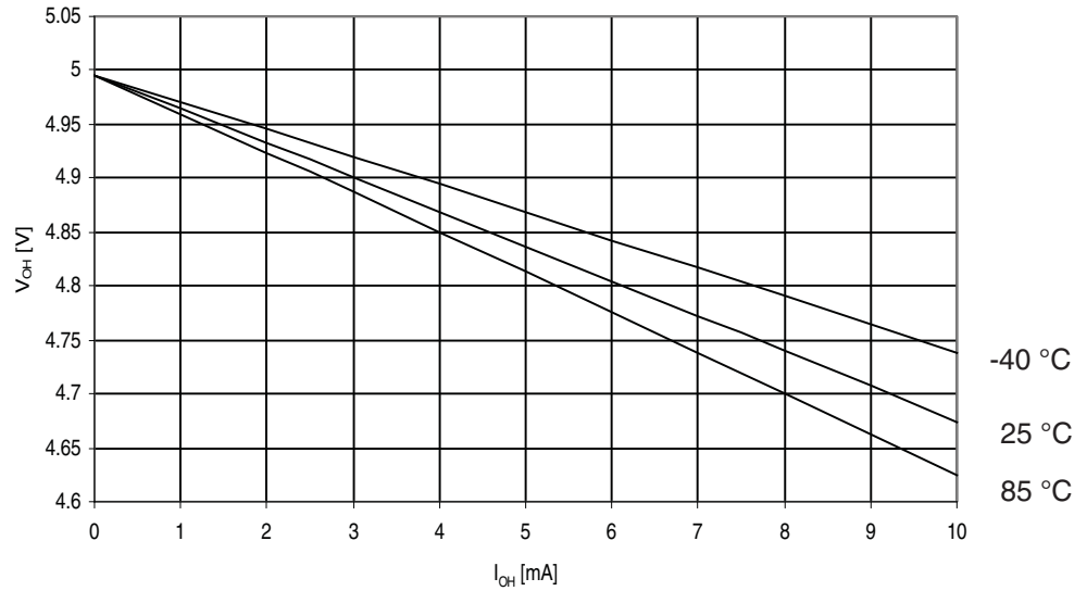
Figure 30-326. ATmega3290PA: I/O Pin Output Voltage vs. Source Current, Ports A, C, D, E, F, G ( V_{CC} = 5V )
