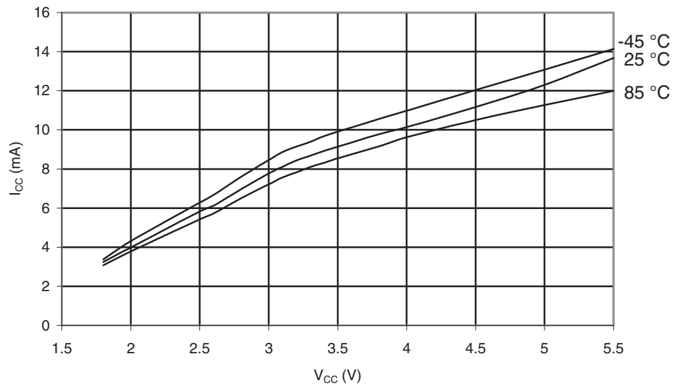
Figure 30-59. ATmega169A: Programming Current vs. V_{CC}
