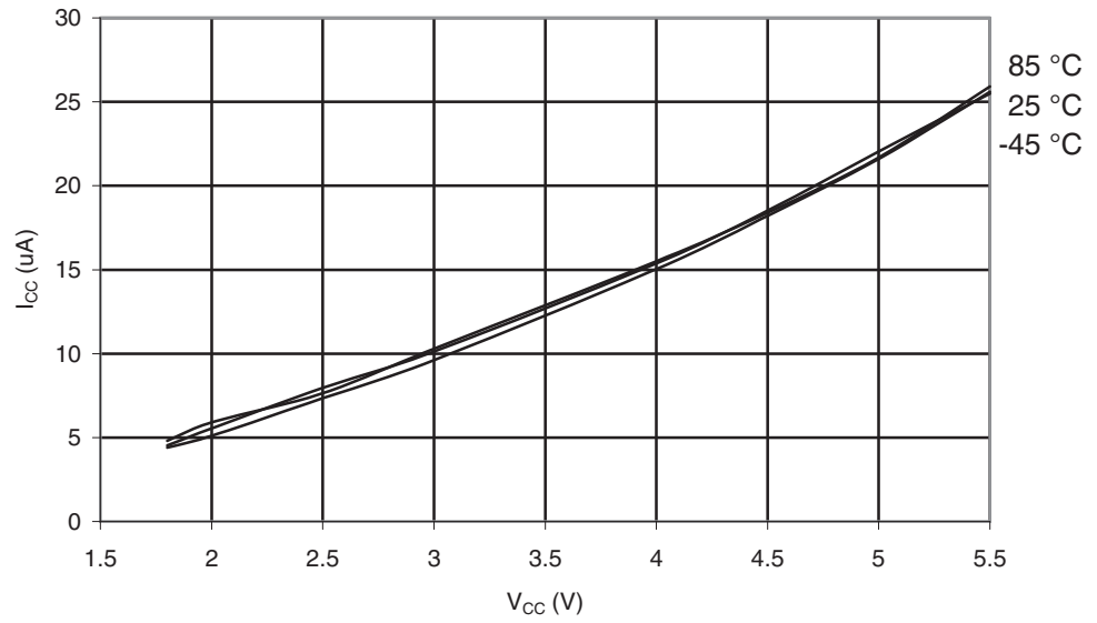
Figure 30-119. ATmega169PA: Watchdog Timer Current vs. V_{CC}
