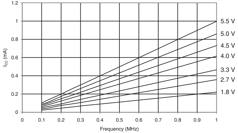
Figure 30-63. ATmega169PA: Active Supply Current vs. Frequency (0.1 - 1.0MHz)
