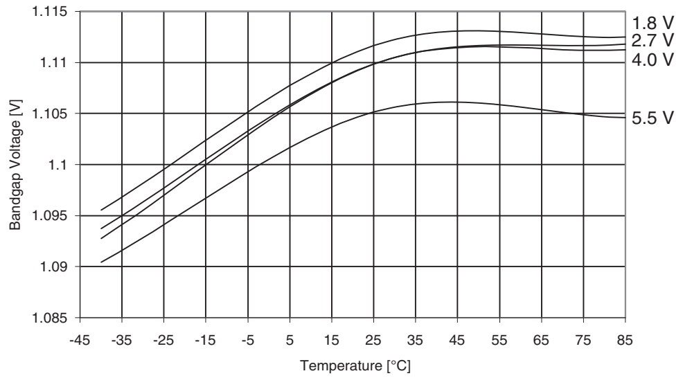
Figure 30-348. ATmega3290PA: Bandgap Voltage vs. Temperature
