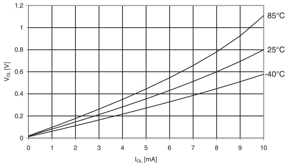
Figure 30-153. ATmega329A: I/O Pin Output Voltage vs. Sink Current, Ports A, C, D, E, F, G ( V_{CC} = 2.7V )
