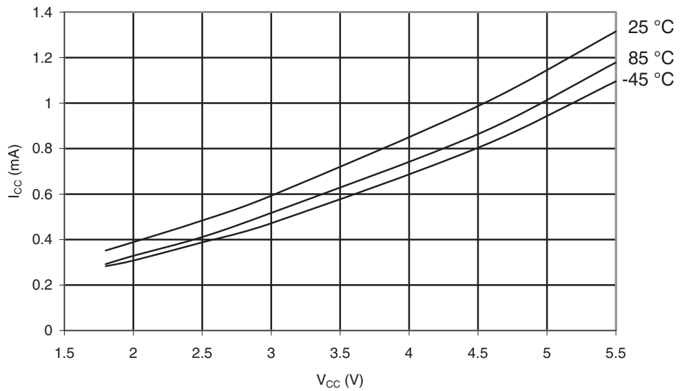
Figure 30-66. ATmega169PA: Active Supply Current vs. V_{CC} (Internal RC Oscillator, 1MHz)
