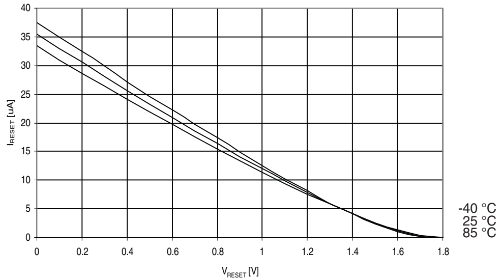
Figure 30-265. ATmega3290A: Reset Pull-up Resistor Current vs. Reset Pin Voltage ( V_{CC}=1.8V )
