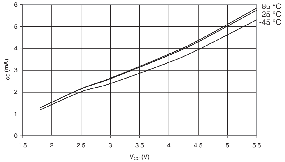
Figure 30-65. ATmega169PA: Active Supply Current vs. V_{CC} (Internal RC Oscillator, 8MHz)
