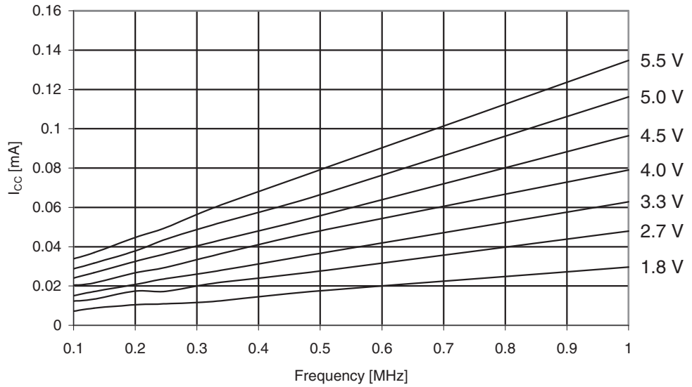
Figure 30-242. ATmega329PA: Reset Supply Current vs. V_{CC} (0.1 - 1.0MHz, Excluding Current Through The Reset Pull-up)
