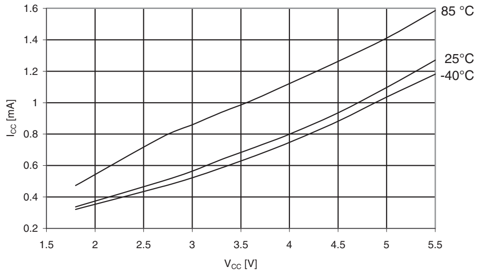
Figure 30-248. ATmega3290A: Active Supply Current vs. V_{CC} (Internal RC Oscillator, 1MHz)
