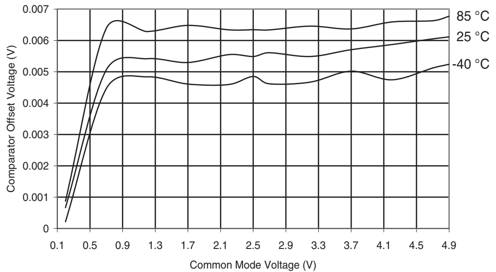
Figure 30-45. ATmega169A: Analog Comparator Offset Voltage vs. Common Mode Voltage ( V_{CC} = 5V )
