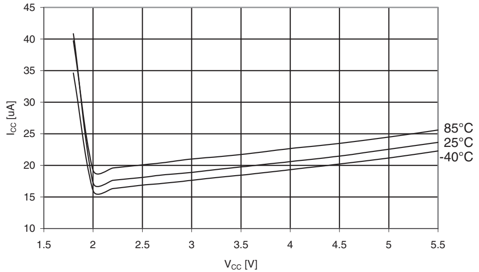
Figure 30-294. ATmega3290A: Brownout Detector Current vs. V_{CC}
