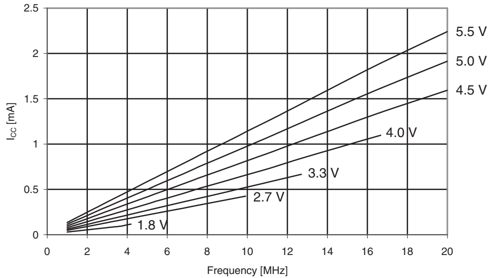
Figure 30-363. ATmega3290PA: Reset Supply Current vs. V_{CC} (1 - 20MHz, Excluding Current Through The Reset Pull-up)
