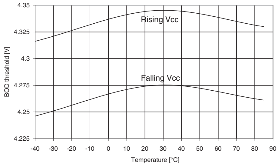
Figure 30-164. ATmega329A: BOD Thresholds vs. Temperature (BOD Level is 4.3V)
