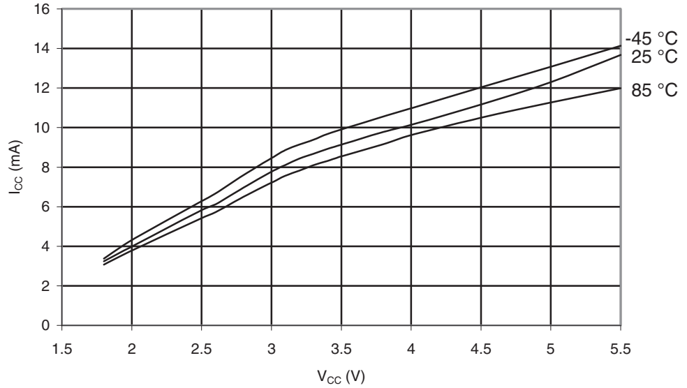
Figure 30-121. ATmega169PA: Programming Current vs. V_{CC}
