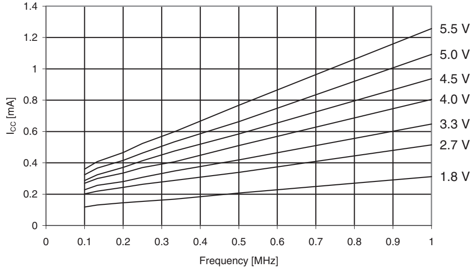
Figure 30-245. ATmega3290A: Active Supply Current vs. Low Frequency (0.1 - 1.0MHz)
