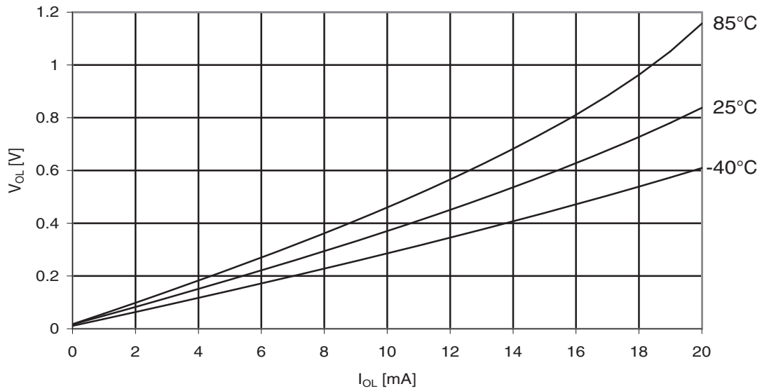
Figure 30-336. ATmega3290PA: I/O Pin Output Voltage vs. Sink Current, Port B ( V_{CC} = 2.7V )
