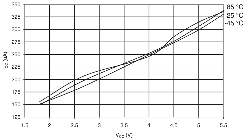
Figure 30-55. ATmega169A: Active Supply Current with ADC at 1MHz vs. V_{CC}
