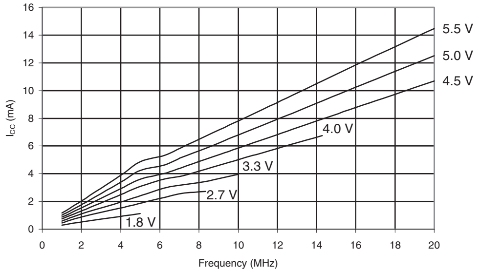
Figure 30-371. ATmega649A: Idle Supply Current vs. Frequency (1 - 20MHz)
