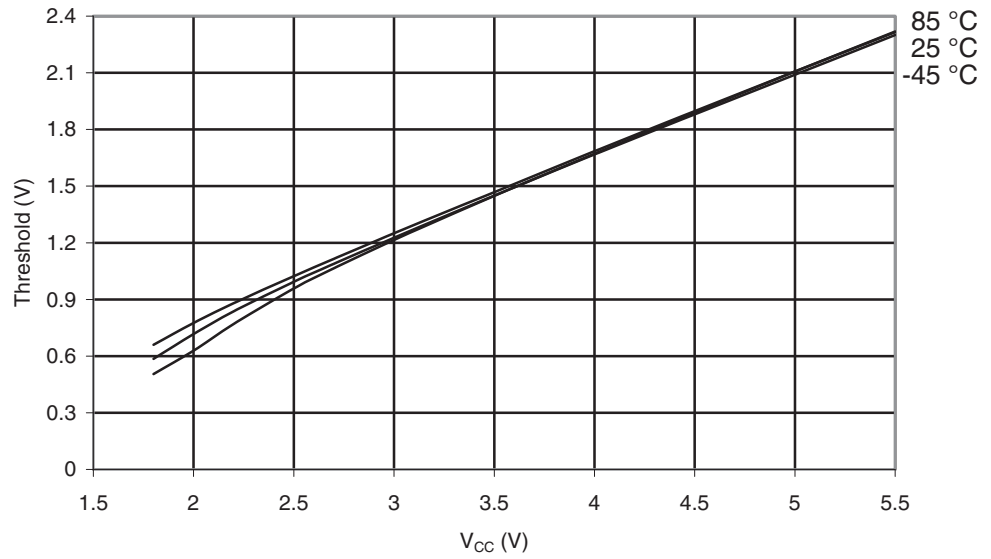
Figure 30-97. ATmega169PA. I/O Pin Input Threshold Voltage vs. V_{CC} ( V_{IL} , I/O Pin Read as "0")
