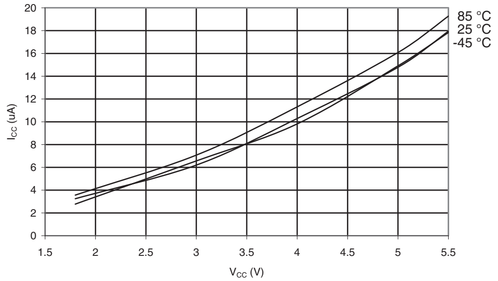
Figure 30-12. ATmega169A: Power-down Supply Current vs. V_{CC} (Watchdog Timer Enabled)
