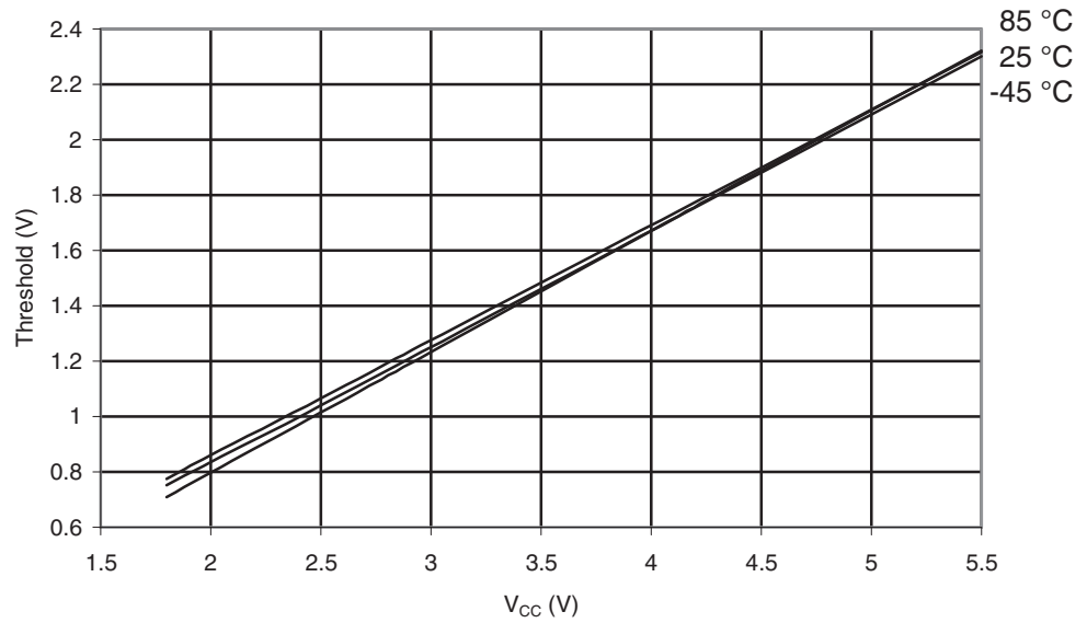
Figure 30-403. ATmega649A: Reset Input Threshold Voltage vs. V_{CC} ( V_{IL} , Reset Pin Read as "0")
