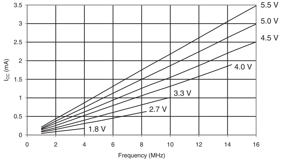
Figure 30-7. ATmega169A: Idle Supply Current vs. Frequency (1 - 16MHz)
