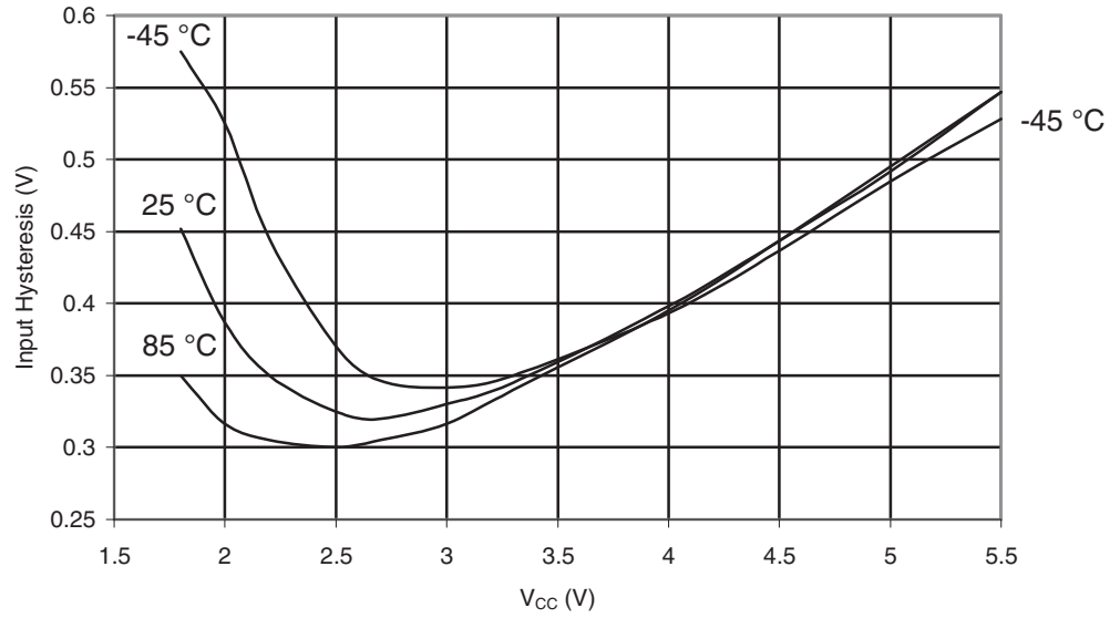
Figure 30-401. ATmega649A: I/O Pin Input Hysteresis vs. V_{CC}
