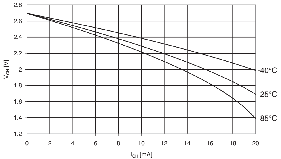
Figure 30-330. ATmega3290PA: I/O Pin Output Voltage vs. Source Current, Port B ( V_{CC} = 2.7V )
