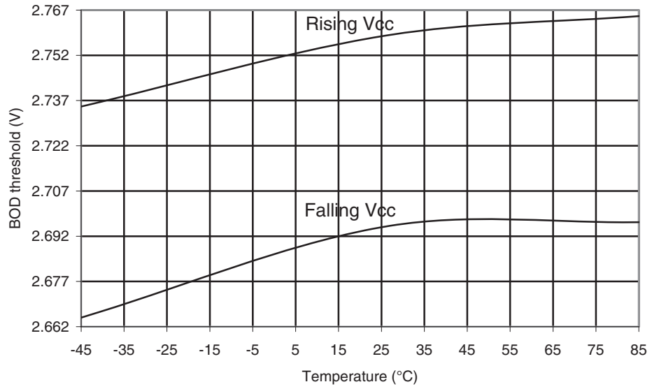
Figure 30-103. ATmega169PA: BOD Thresholds vs. Temperature (BOD Level is 2.7V)
