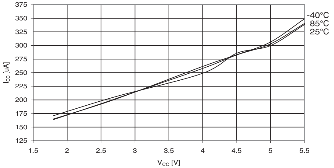
Figure 30-297. ATmega3290A: Active Supply Current with ADC at 1MHz vs. V_{CC}
