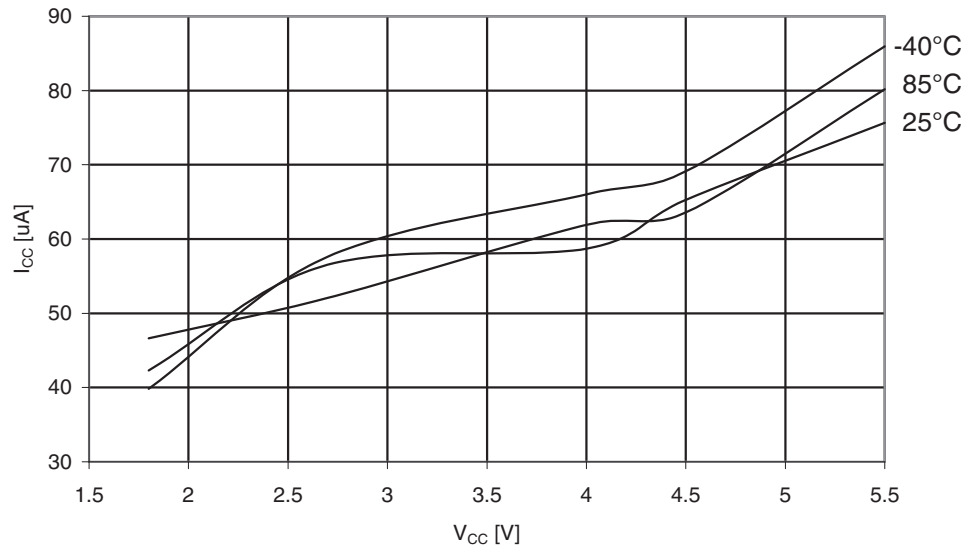
Figure 30-180. ATmega329A: Analog Comparator Current vs. V_{CC}
