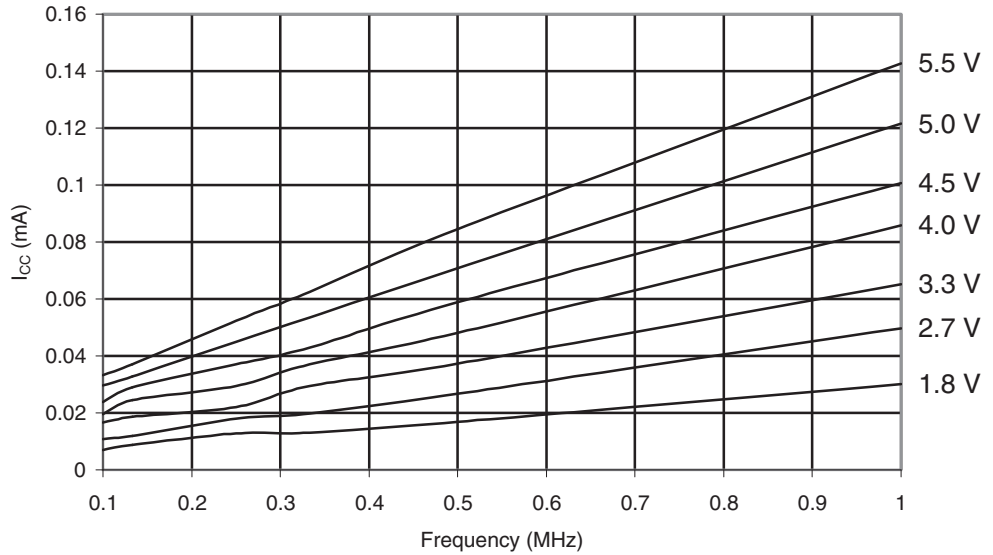
Figure 30-545. ATmega6490A: Reset Supply Current vs. V_{CC} (0.1 - 1.0MHz, Excluding Current Through The Reset Pull-up)
