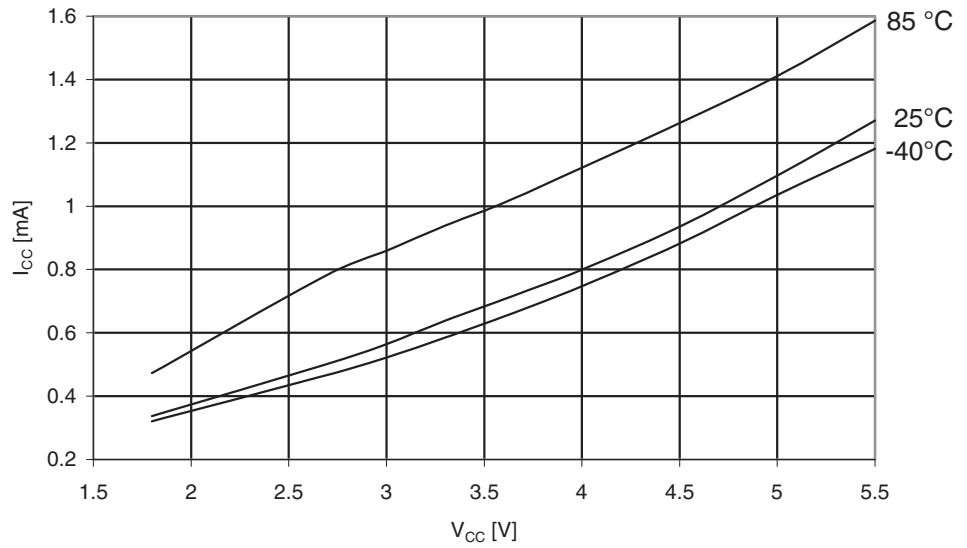
Figure 30-188. ATmega329PA: Active Supply Current vs. V_{CC} (Internal RC Oscillator, 1MHz)
