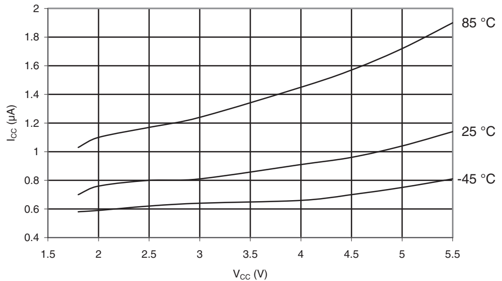
Figure 30-75. ATmega169PA: Power-save Supply Current vs. V_{CC} (Watchdog Timer Disabled)
