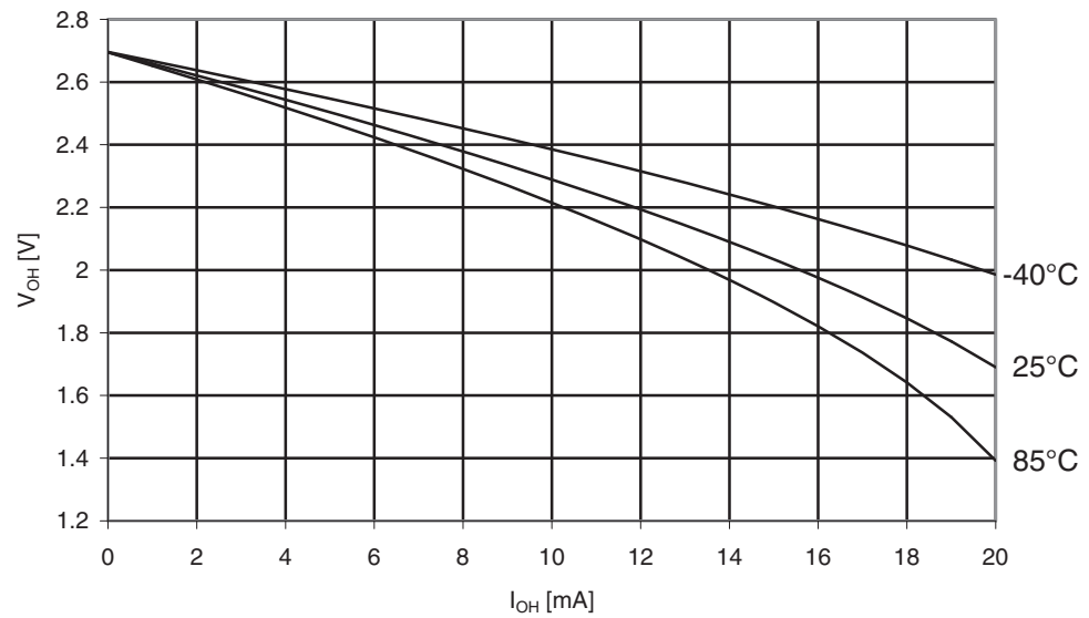
Figure 30-270. ATmega3290A: I/O Pin Output Voltage vs. Source Current, Port B ( V_{CC} = 2.7V )
