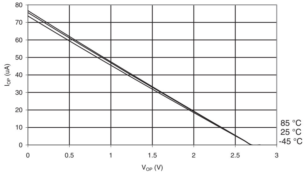
Figure 30-79. ATmega169PA: I/O Pin Pull-up Resistor Current vs. Input Voltage ( V_{CC} = 2.7V )
