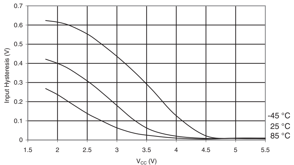
Figure 30-39. ATmega169A: Reset Input Pin Hysteresis vs. V_{CC}
