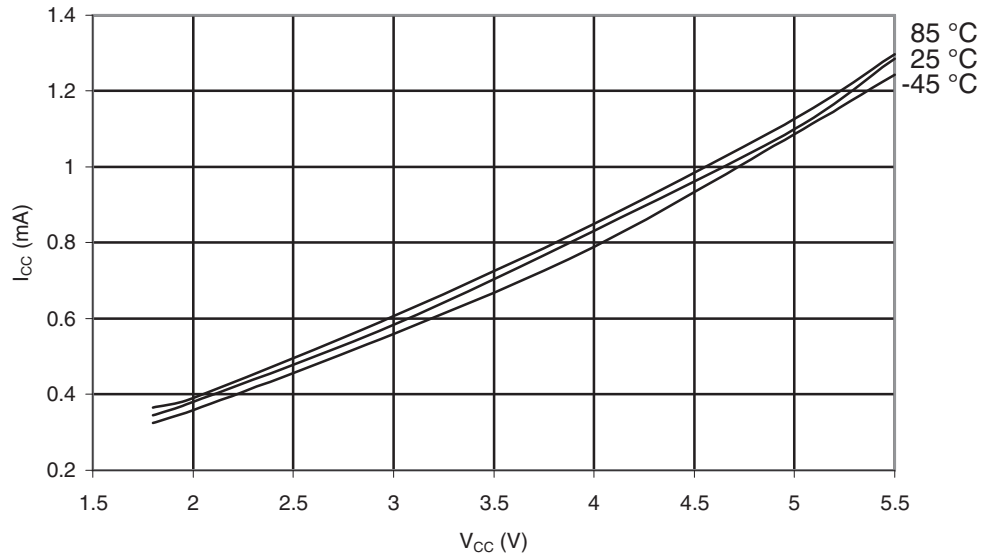
Figure 30-373. ATmega649A: Idle Supply Current vs. V_{CC} (Internal RC Oscillator, 1MHz)
