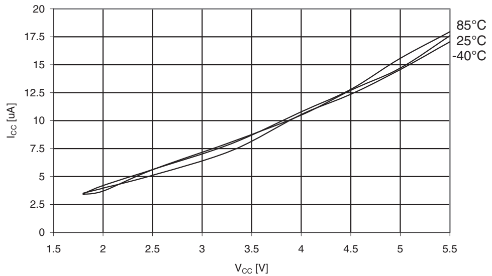
Figure 30-239. ATmega329PA: Watchdog Timer Current vs. V_{CC}
