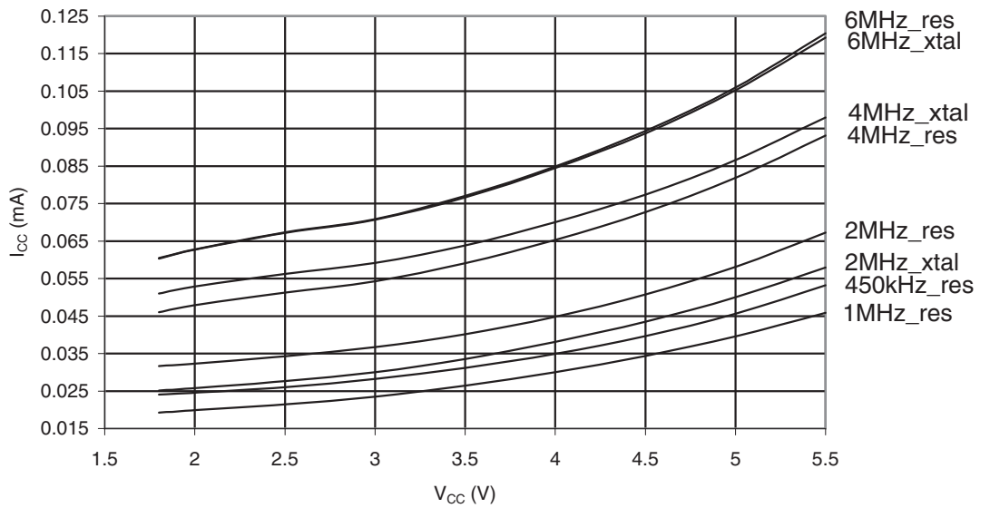
Figure 30-563. ATmega6490P: Standby Supply Current vs. V_{CC} (Xtall and Resonator, Watchdog Timer Disabled)
