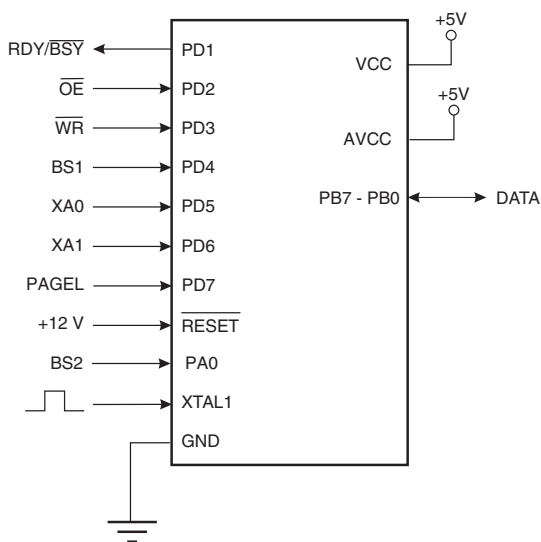
Figure 28-1. Parallel Programming
