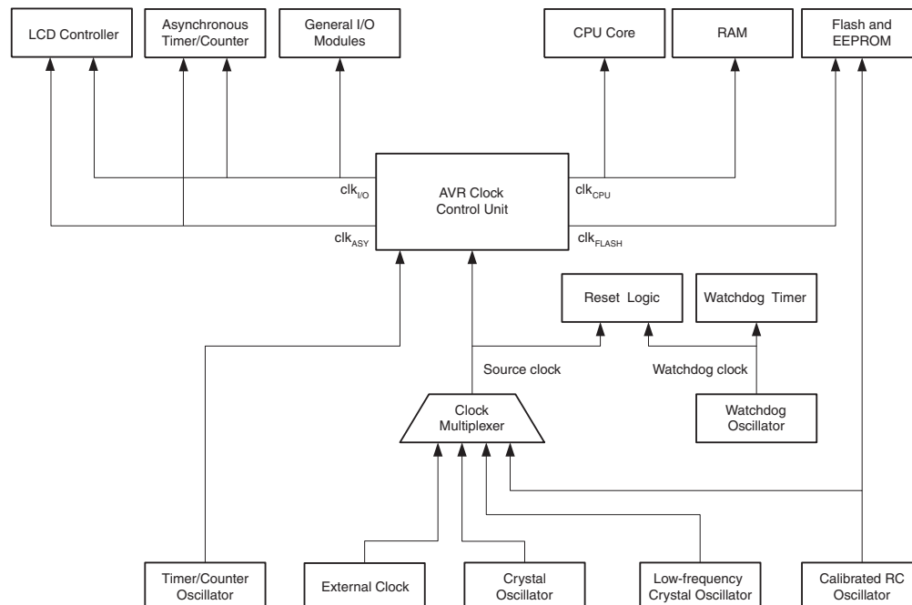
Figure 9-1. Clock Distribution
