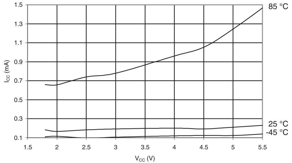
Figure 30-438. ATmega649P: Power-down Supply Current vs. V_{CC} (32kHz Watch Crystal)
