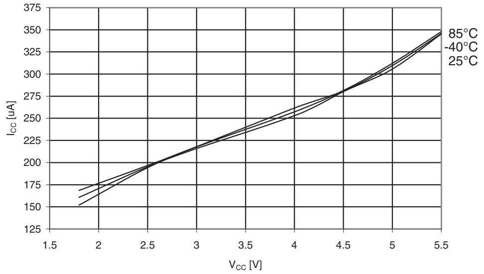
Figure 30-356. ATmega3290PA: Active Supply Current with ADC at 200kHz vs. V_{CC}
