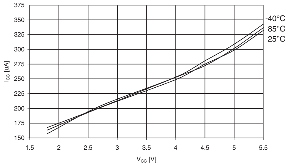
Figure 30-235. ATmega329PA: Active Supply Current with ADC at 50kHz vs. V_{CC}
