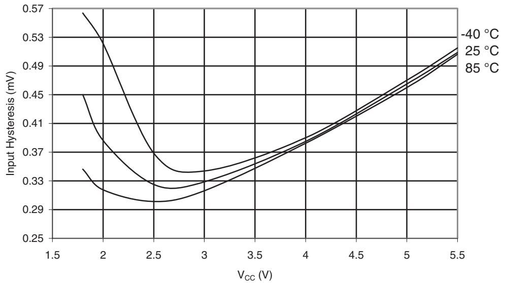
Figure 30-280. ATmega3290A: I/O Pin Input Hysteresis vs. V_{CC}
