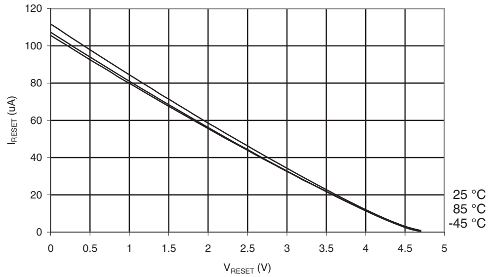
Figure 30-81. ATmega169PA: Reset Pull-up Resistor Current vs. Reset Pin Voltage ( V_{CC} = 5V )
