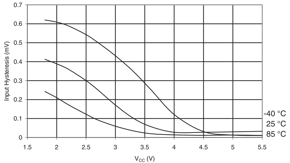
Figure 30-343. ATmega3290PA: Reset Input Pin Hysteresis vs. V_{CC}
