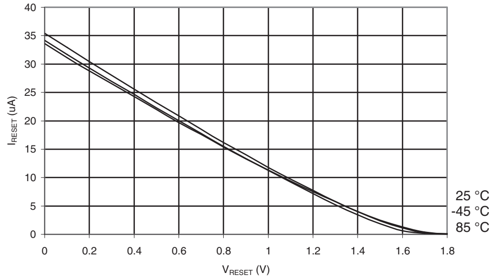
Figure 30-386. ATmega649A: Reset Pull-up Resistor Current vs. Reset Pin Voltage ( V_{CC} = 1.8V )
