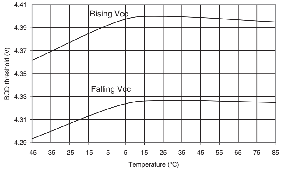
Figure 30-405. ATmega649A: BOD Thresholds vs. Temperature (BOD Level is 4.3V)
