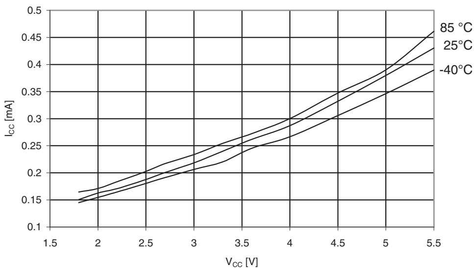
Figure 30-253. ATmega3290A: Idle Supply Current vs. V_{CC} (Internal RC Oscillator, 1MHz)
