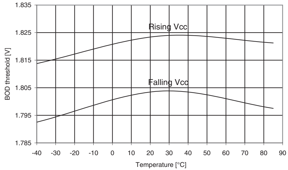
Figure 30-166. ATmega329A: BOD Thresholds vs. Temperature (BOD Level is 1.8V)
