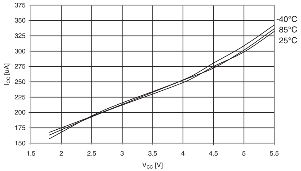
Figure 30-295. ATmega3290A: Active Supply Current with ADC at 50kHz vs. V_{CC}
