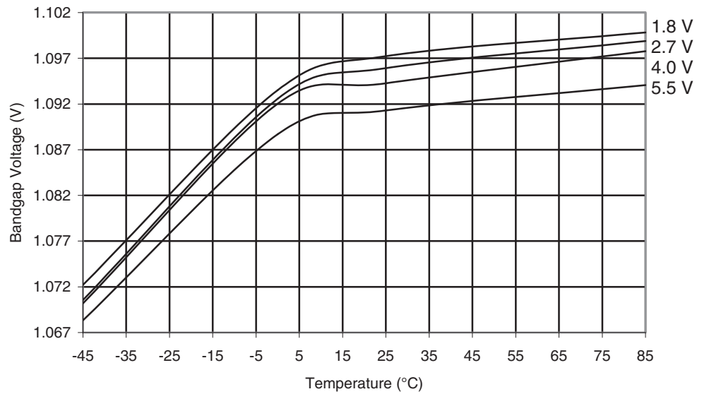
Figure 30-106. ATmega169PA: Bandgap Voltage vs. Temperature
