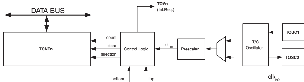
Figure 18-2. Counter Unit Block Diagram
