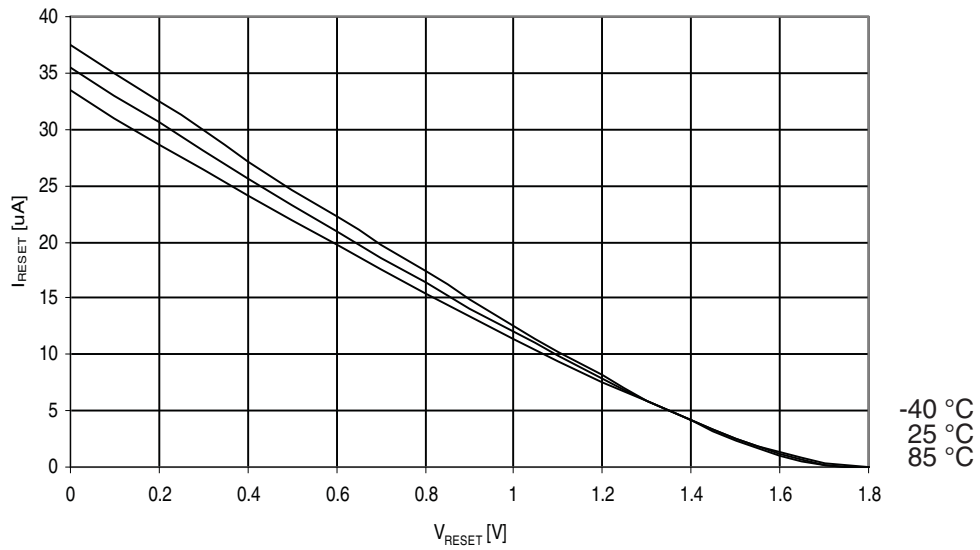
Figure 30-205. ATmega329PA: Reset Pull-up Resistor Current vs. Reset Pin Voltage ( V_{CC} = 1.8V )
