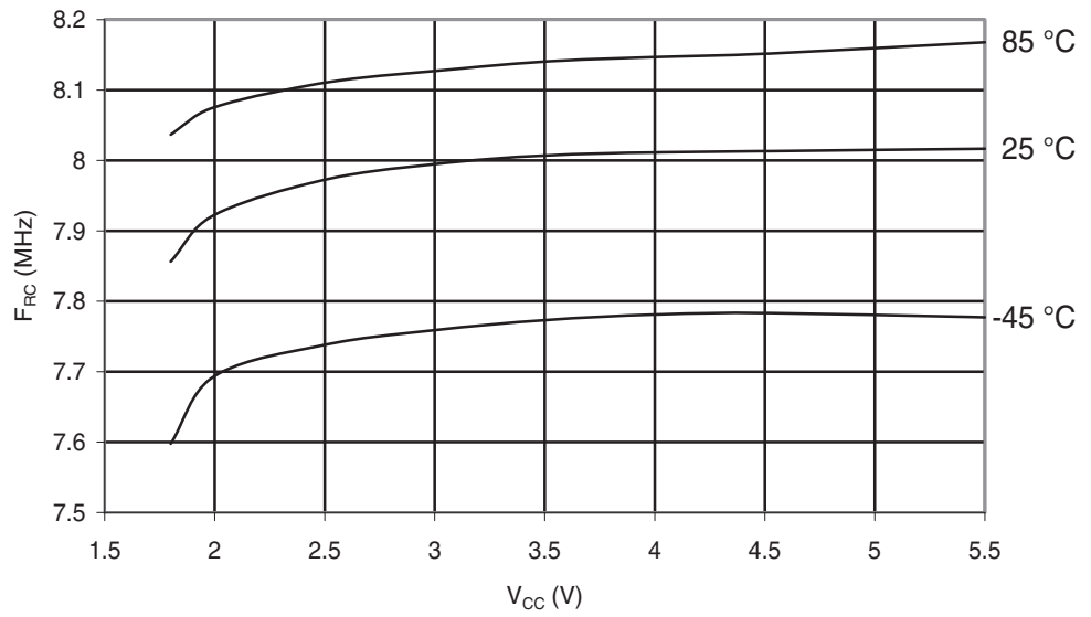
Figure 30-50. ATmega169A: Calibrated 8MHz RC Oscillator Frequency vs. V_{CC}
