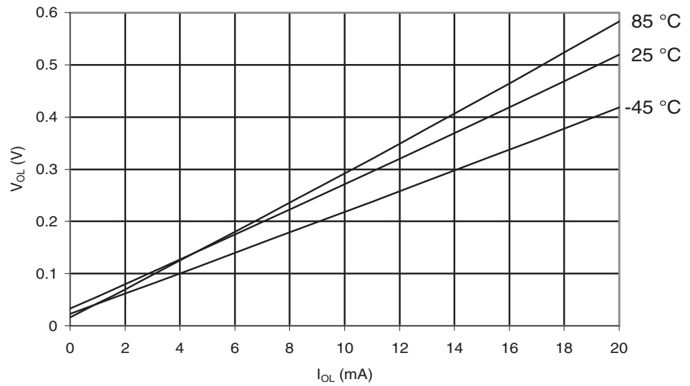
Figure 30-396. ATmega649A: I/O Pin Output Voltage vs. Sink Current, Port B ( V_{CC} = 5V )
