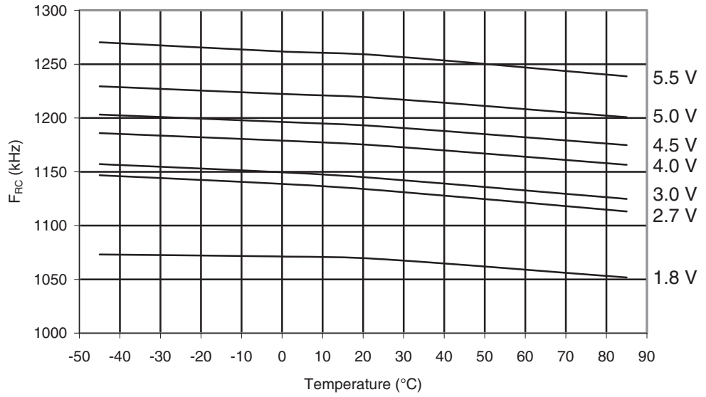
Figure 30-48. ATmega169A: Watchdog Oscillator Frequency vs. Temperature
