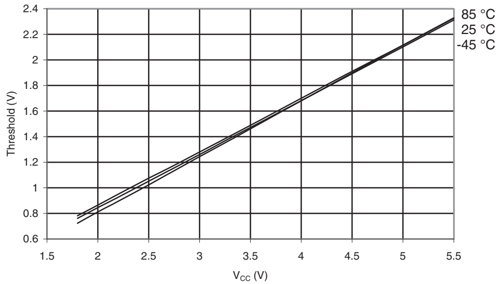
Figure 30-38. ATmega169A: Reset Input Threshold Voltage vs. V_{CC} ( V_{IL} , Reset Pin Read as "0")
