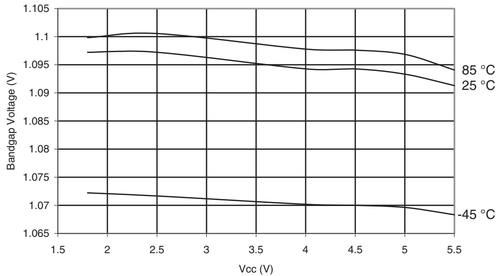
Figure 30-43. ATmega169A: Bandgap Voltage vs. V_{CC}
