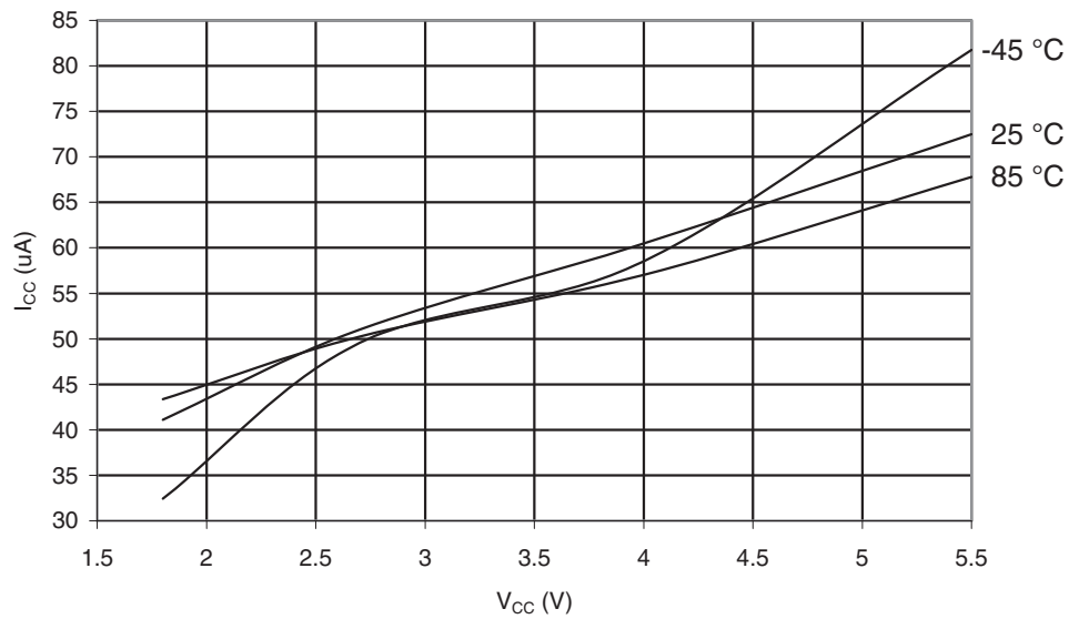
Figure 30-120. ATmega169PA: Analog Comparator Current vs. V_{CC}
