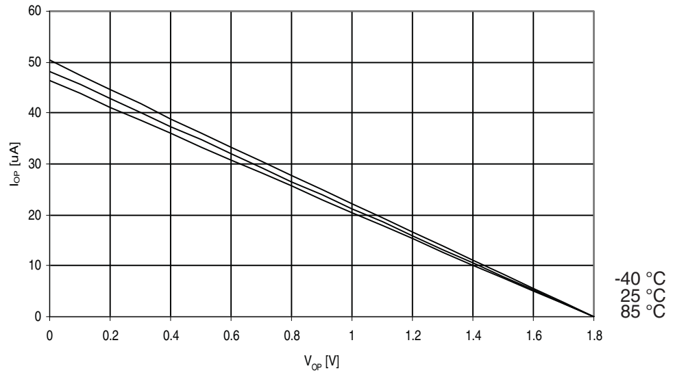
Figure 30-202. ATmega329PA: I/O Pin Pull-up Resistor Current vs. Input Voltage ( V_{CC} = 1.8V )
