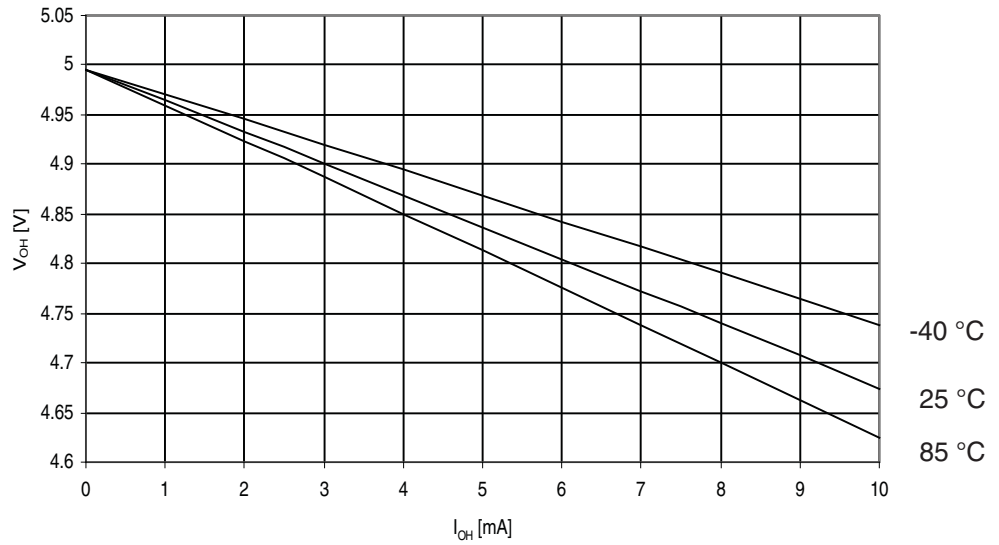
Figure 30-206. ATmega329PA: I/O Pin Output Voltage vs. Source Current, Ports A, C, D, E, F, G ( V_{CC} = 5V )
