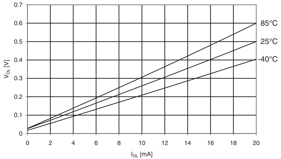
Figure 30-215. ATmega329PA: I/O Pin Output Voltage vs. Sink Current, Port B ( V_{CC} = 5V )
