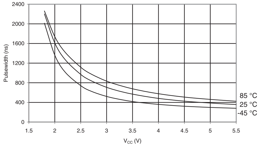
Figure 30-62. ATmega169A: Minimum Reset Pulse Width vs. V_{CC}
