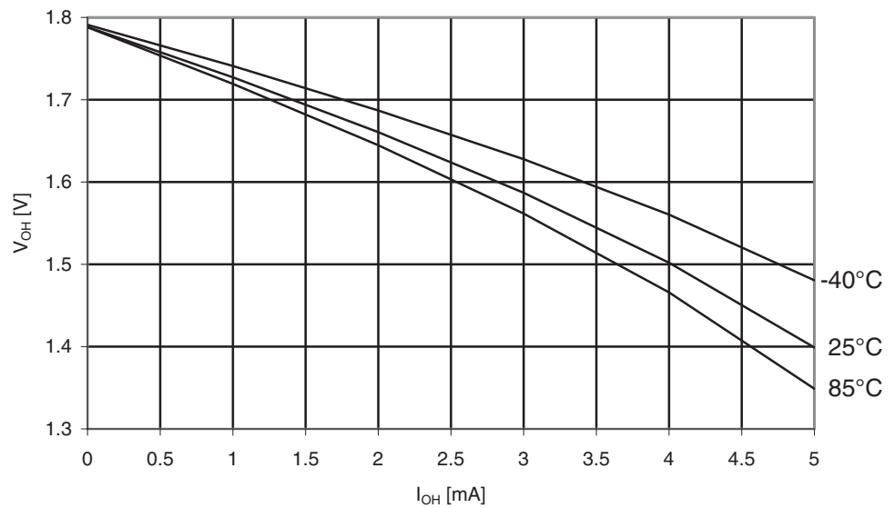
Figure 30-211. ATmega329PA: I/O Pin Output Voltage vs. Source Current, Port B ( V_{CC} = 1.8V )
