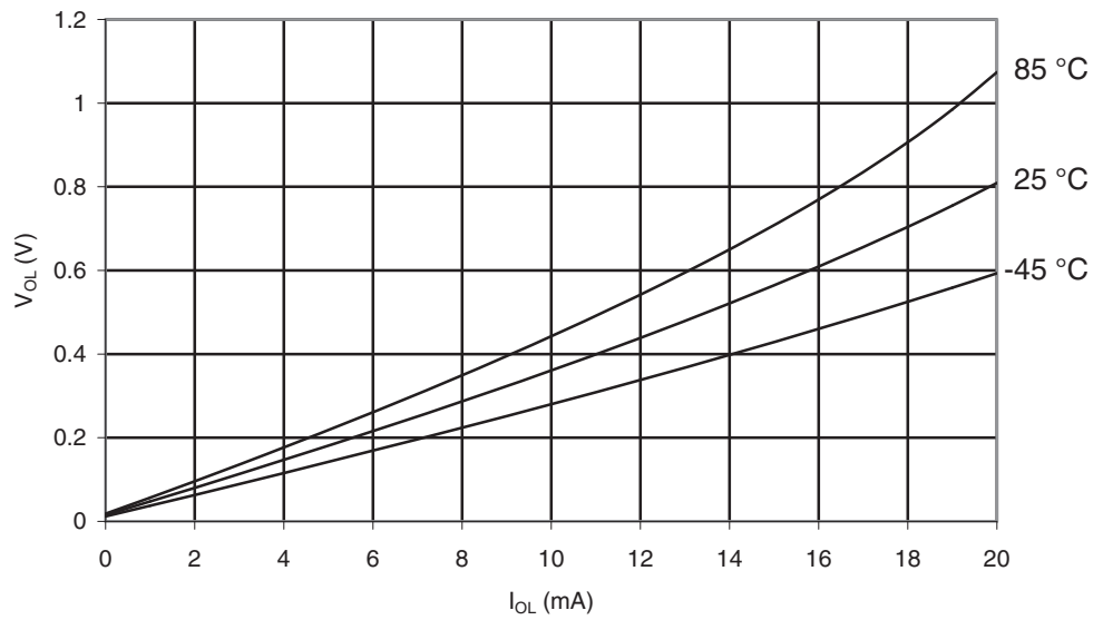
Figure 30-94. ATmega169PA: I/O Pin Output Voltage vs. Sink Current, Port B ( V_{CC} = 2.7V )
