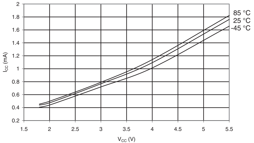
Figure 30-372. ATmega649A: Idle Supply Current vs. V_{CC} (Internal RC Oscillator, 8MHz)
