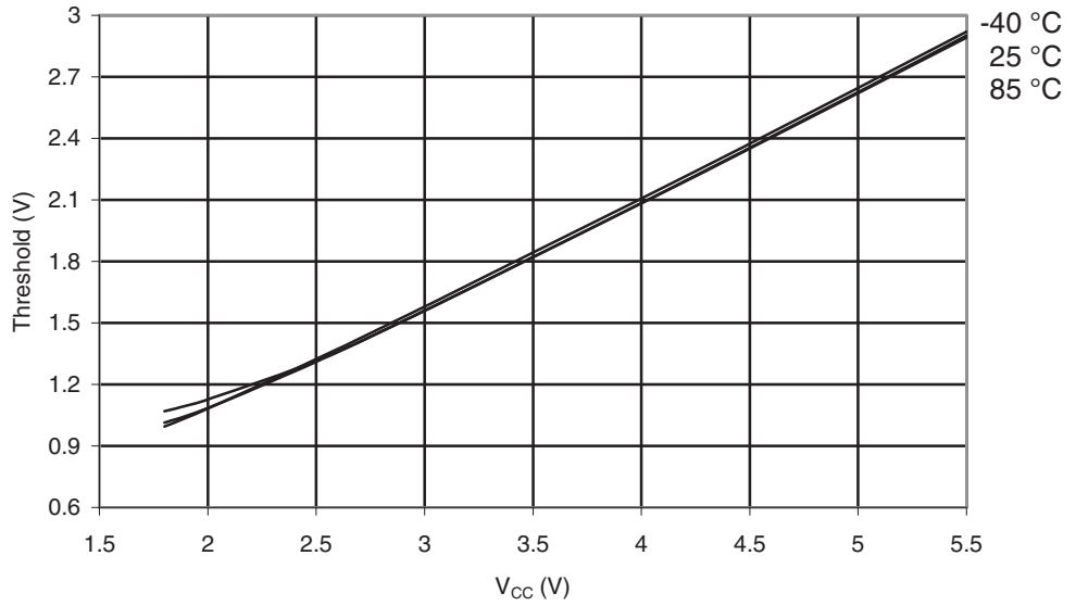
Figure 30-338. ATmega3290PA: I/O Pin Input Threshold Voltage vs. V_{CC} ( V_{IH} , I/O Pin Read as "1")
