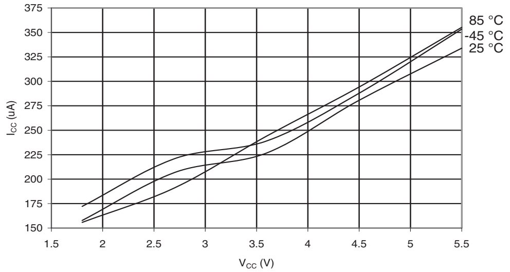
Figure 30-54. ATmega169A: Active Supply Current with ADC at 200kHz vs. V_{CC}
