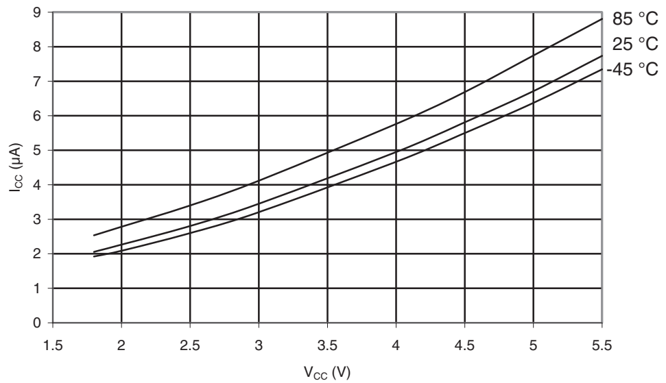
Figure 30-72. ATmega169PA: Idle Supply Current vs. V_{CC} (32kHz Watch Crystal)
