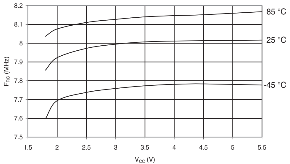
Figure 30-112. ATmega169PA: Calibrated 8MHz RC Oscillator Frequency vs. V_{CC}
