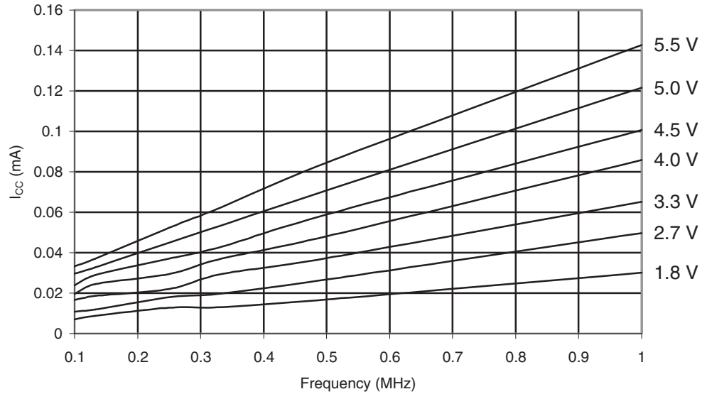
Figure 30-423. ATmega649A: Reset Supply Current vs. V_{CC} (0.1 - 1.0MHz, Excluding Current Through The Reset Pull-up)
