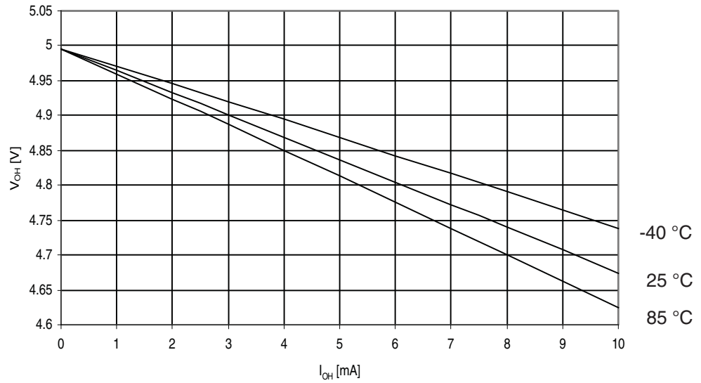
Figure 30-146. ATmega329A: I/O Pin Output Voltage vs. Source Current, Ports A, C, D, E, F, G ( V_{CC} = 5V )
