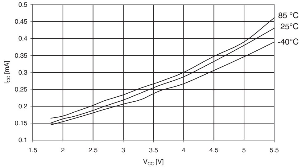
Figure 30-193. ATmega329PA: Idle Supply Current vs. V_{CC} (Internal RC Oscillator, 1MHz)
