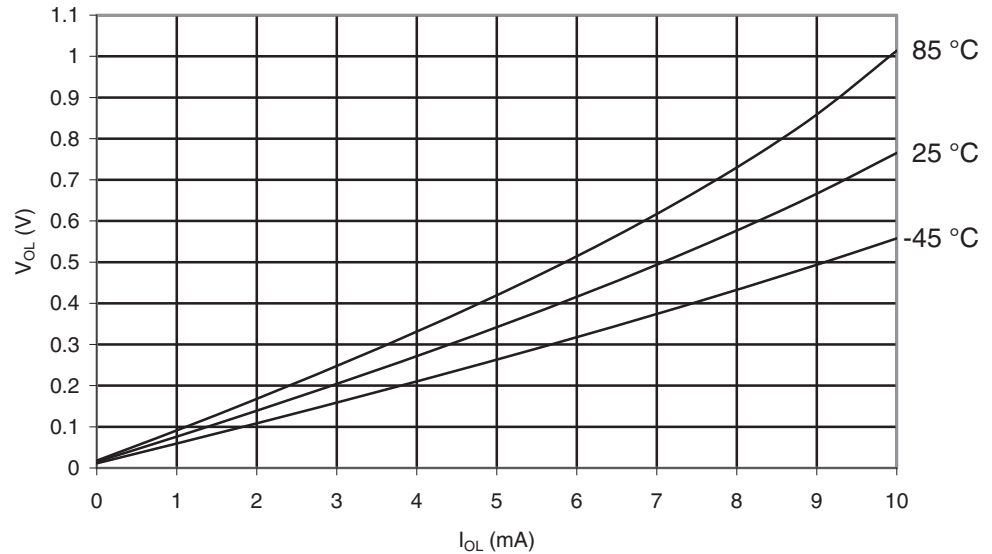
Figure 30-29. ATmega169A: I/O Pin Output Voltage vs. Sink Current, Ports A, C, D, E, F, G ( V_{CC} = 2.7V )
