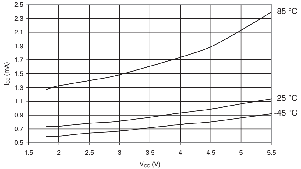
Figure 30-561. ATmega6490P: Power-save Supply Current vs. V_{CC} (Watchdog Timer Disabled and 32kHz Crystal Oscillator Running)
