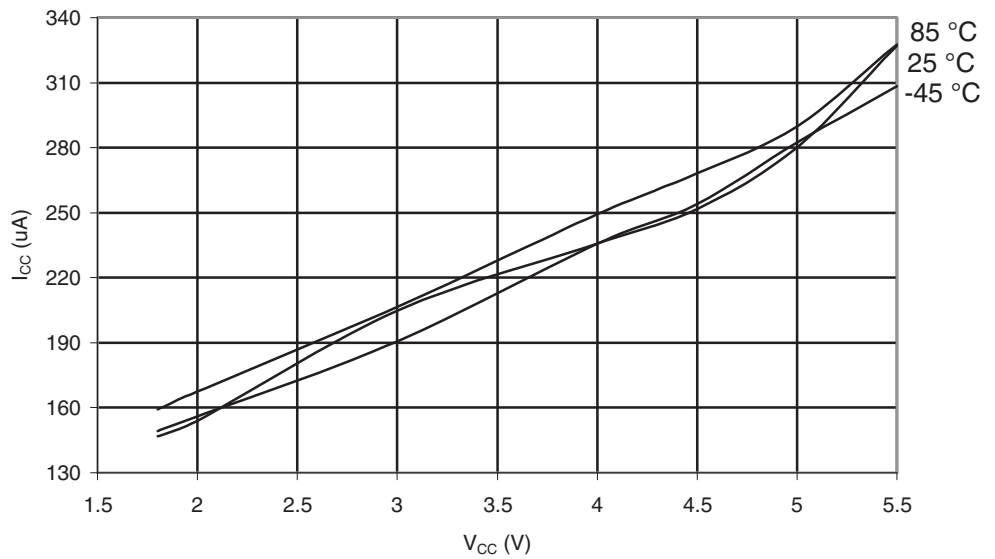
Figure 30-601. ATmega6490P: Active Supply Current with ADC at 1MHz vs. V_{CC}
