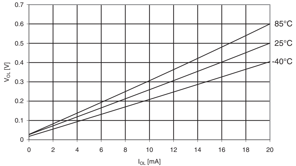
Figure 30-155. ATmega329A: I/O Pin Output Voltage vs. Sink Current, Port B ( V_{CC} = 5V )
