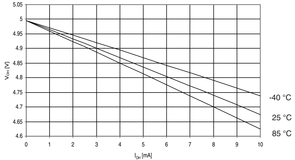
Figure 30-266. ATmega3290A: I/O Pin Output Voltage vs. Source Current, Ports A, C, D, E, F, G ( V_{CC} = 5V )
