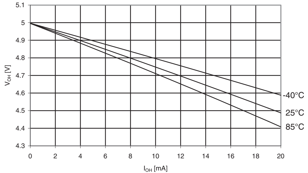
Figure 30-209. ATmega329PA: I/O Pin Output Voltage vs. Source Current, Port B ( V_{CC} = 5V )
