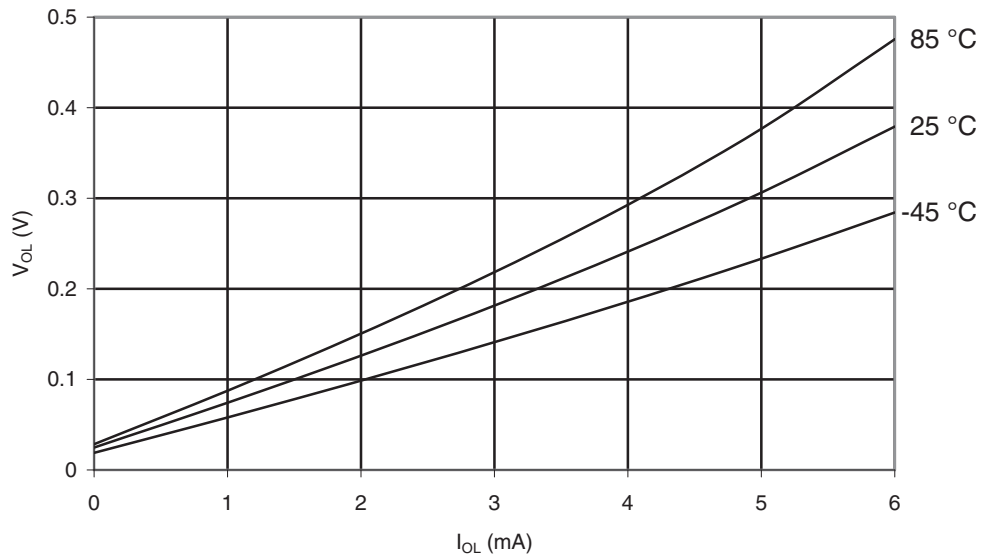
Figure 30-95. ATmega169PA: I/O Pin Output Voltage vs. Sink Current, Port B ( V_{CC} = 1.8V )
