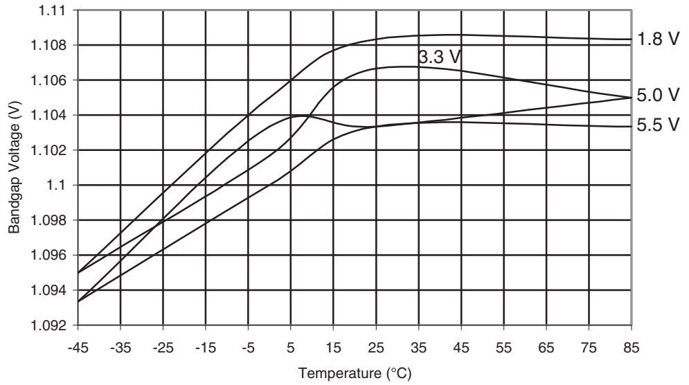
Figure 30-592. ATmega6490P: Bandgap Voltage vs. Temperature
