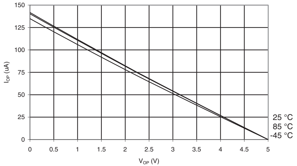
Figure 30-16. ATmega169A: I/O Pin Pull-up Resistor Current vs. Input Voltage ( V_{CC} = 5V )
