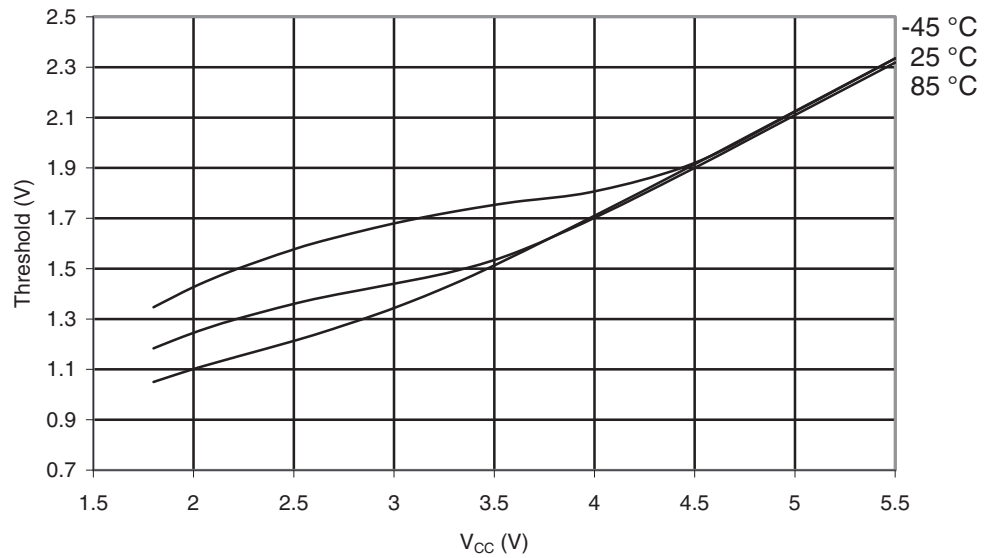
Figure 30-37. ATmega169A: Reset Input Threshold Voltage vs. V_{CC} ( V_{IH} , Reset Pin Read as "1")
