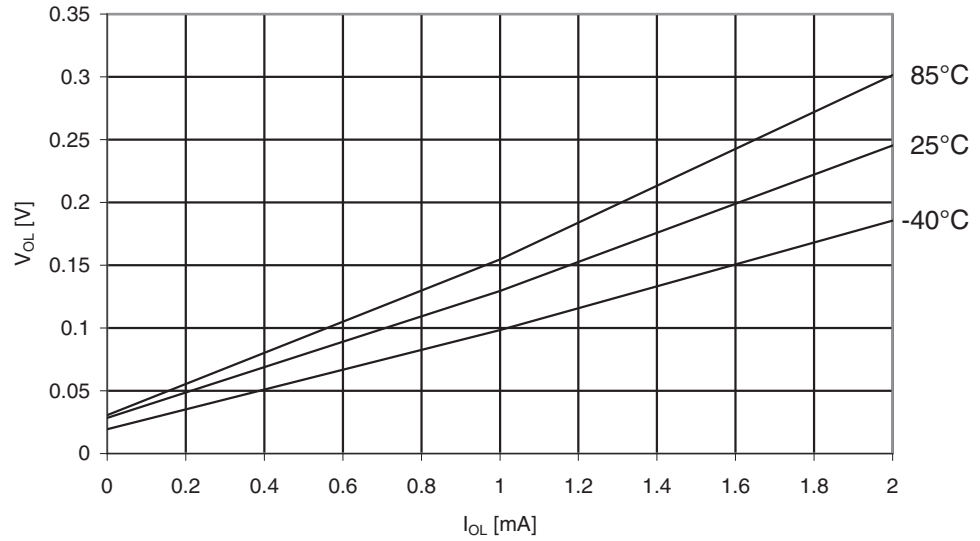
Figure 30-334. ATmega3290PA: I/O Pin Output Voltage vs. Sink Current, Ports A, C, D, E, F, G ( V_{CC} = 1.8V )
