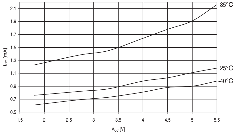
Figure 30-317. ATmega3290PA: Power-save Supply Current vs. V_{CC} (Watchdog Timer Disabled and 32kHz Crystal Oscillator Running)
