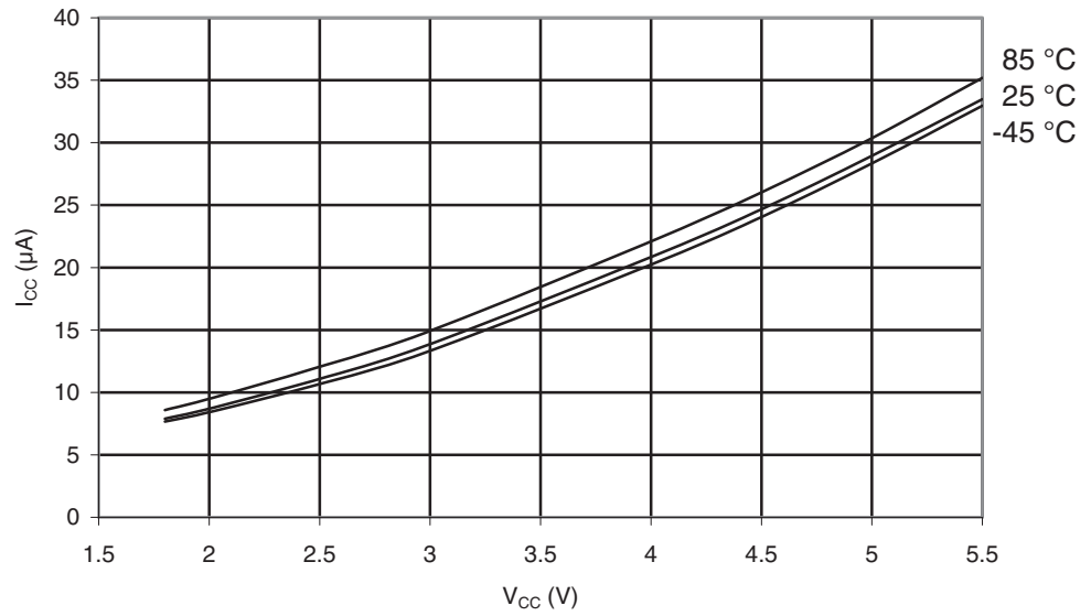
Figure 30-67. ATmega169PA: Active Supply Current vs. V_{CC} (32kHz Watch Crystal)
