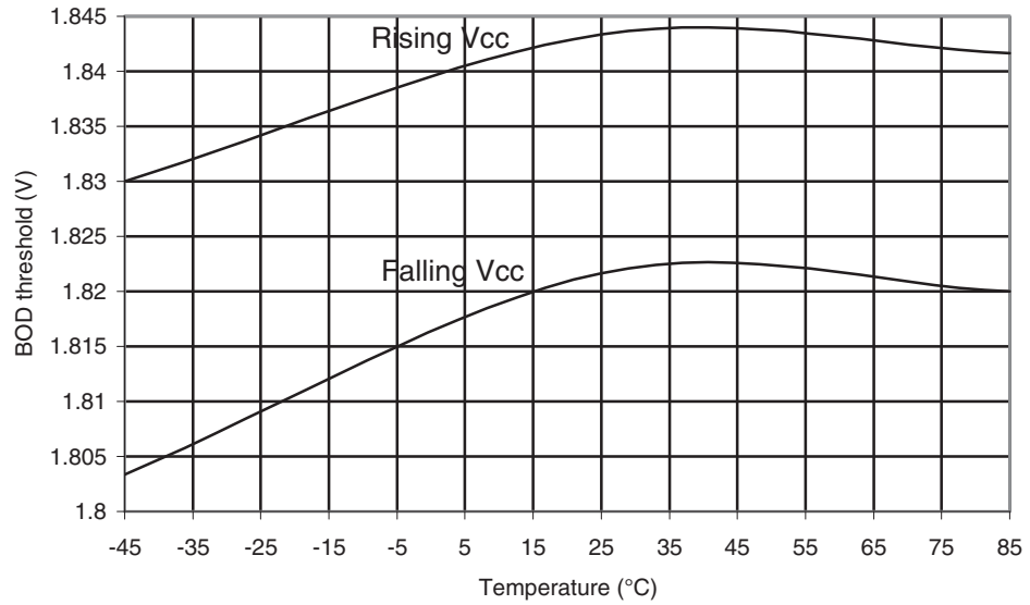
Figure 30-407. ATmega649A: BOD Thresholds vs. Temperature (BOD Level is 1.8V)
