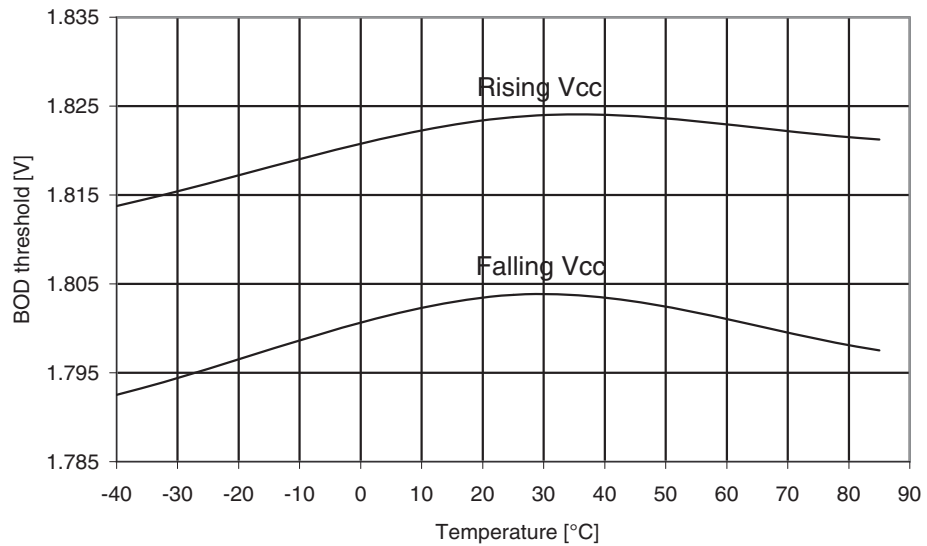
Figure 30-286. ATmega3290A: BOD Thresholds vs. Temperature (BOD Level is 1.8V)
