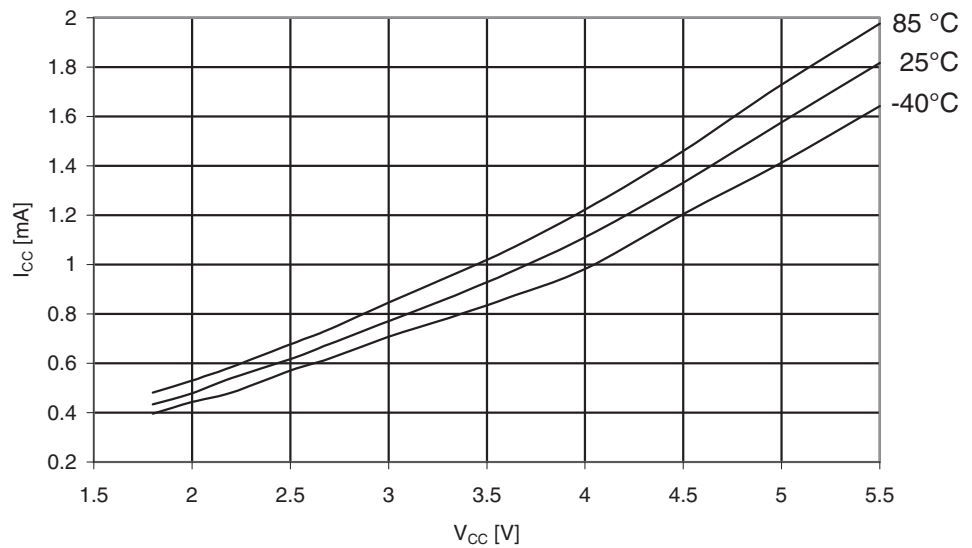
Figure 30-132. ATmega329A: Idle Supply Current vs. V_{CC} (Internal RC Oscillator, 8MHz)
