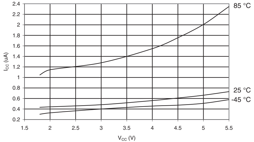
Figure 30-375. ATmega649A: Power-down Supply Current vs. V_{CC} (Watchdog Timer Disabled)
