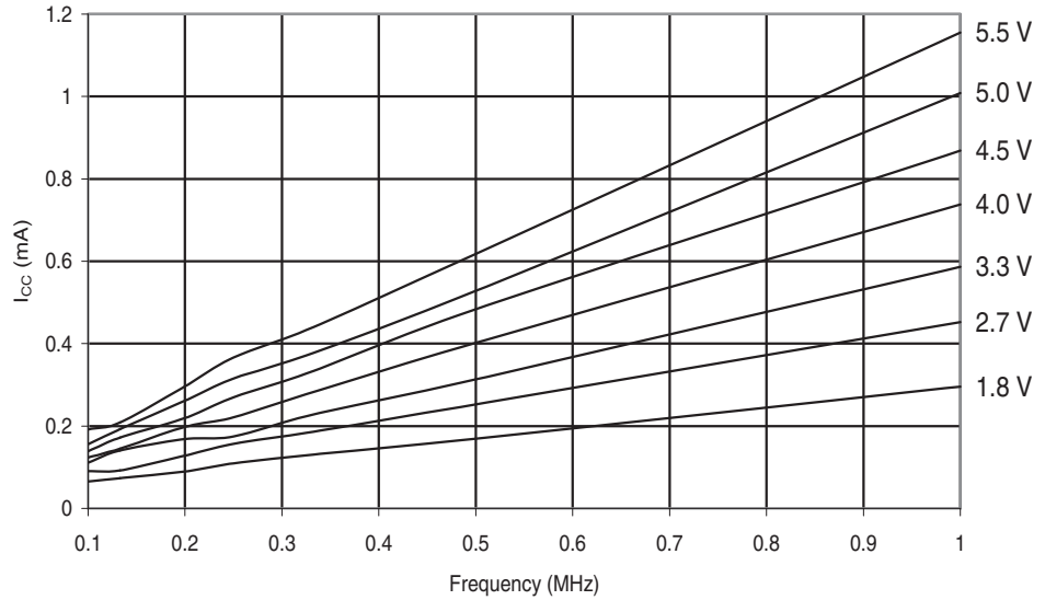
Figure 30-365. ATmega649A: Active Supply Current vs. Low Frequency (0.1 - 1.0MHz)
