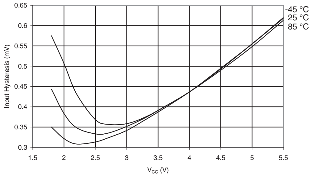
Figure 30-98. ATmega169PA: I/O Pin Input Hysteresis vs. V_{CC}
