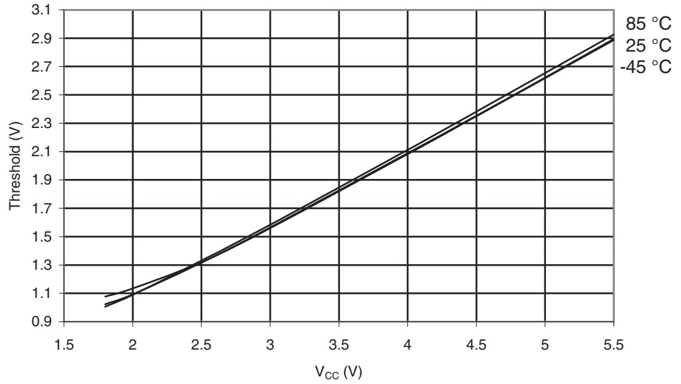
Figure 30-460. ATmega649P: I/O Pin Input Threshold Voltage vs. V_{CC} ( V_{IH} , I/O Pin Read as "1")
