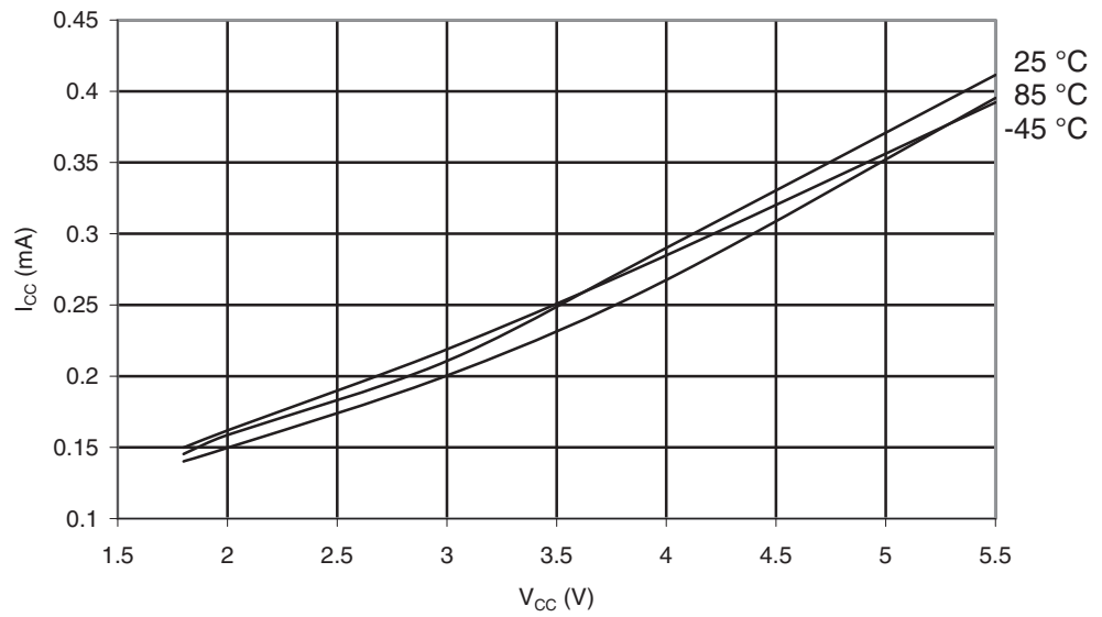
Figure 30-551. ATmega6490P: Active Supply Current vs. V_{CC} (Internal RC Oscillator, 1MHz)
