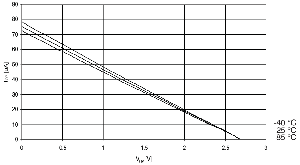
Figure 30-261. ATmega3290A: I/O Pin Pull-up Resistor Current vs. Input Voltage ( V_{CC} = 2.7V )
