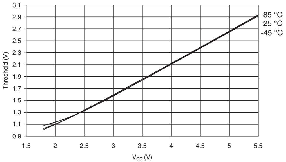
Figure 30-96. ATmega169PA: I/O Pin Input Threshold Voltage vs. V_{CC} ( V_{IH} , I/O Pin Read as "1")
