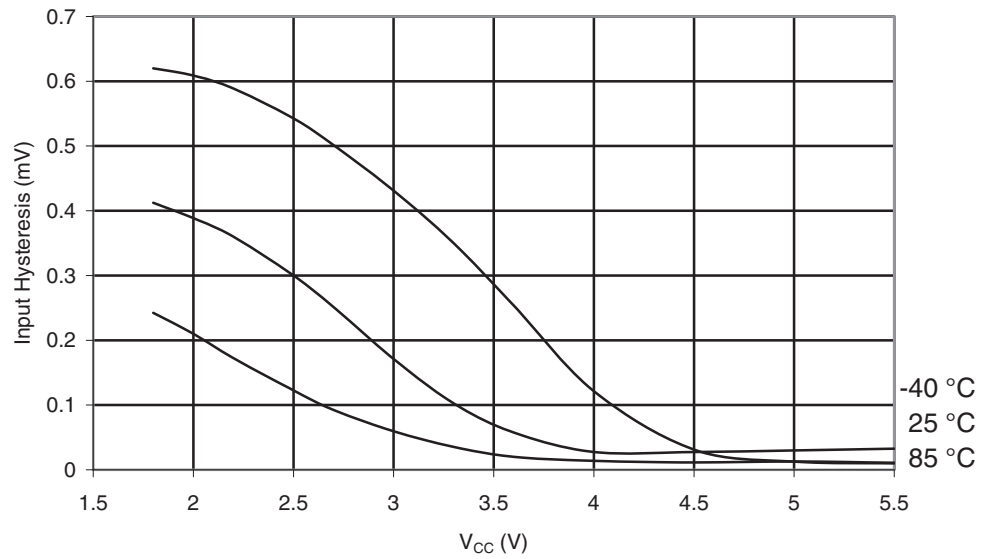
Figure 30-163. ATmega329A: Reset Pin Input Hysteresis vs. V_{CC}
