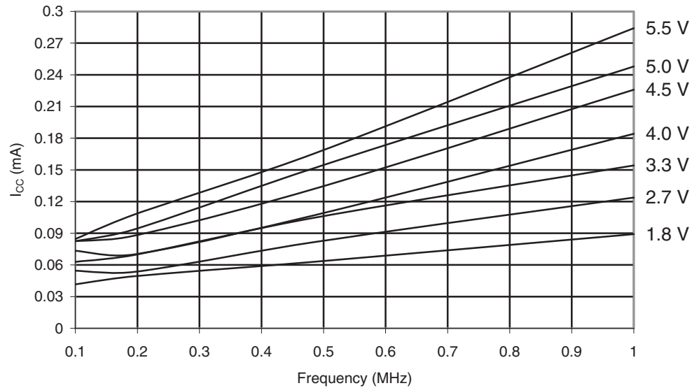
Figure 30-431. ATmega649P: Idle Supply Current vs. Low Frequency (0.1 - 1.0MHz)
