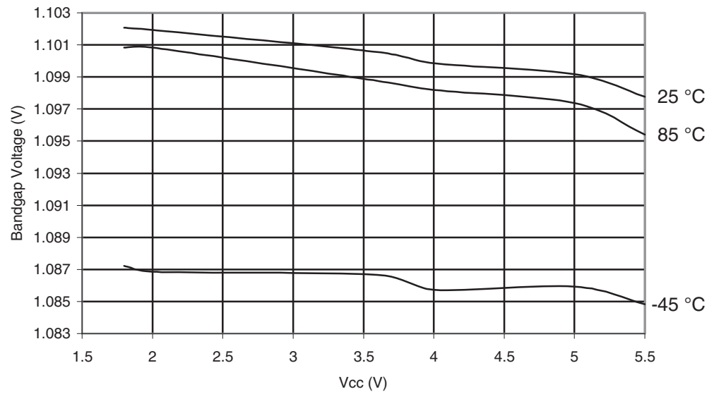
Figure 30-469. ATmega649P: Bandgap Voltage vs. V CC
