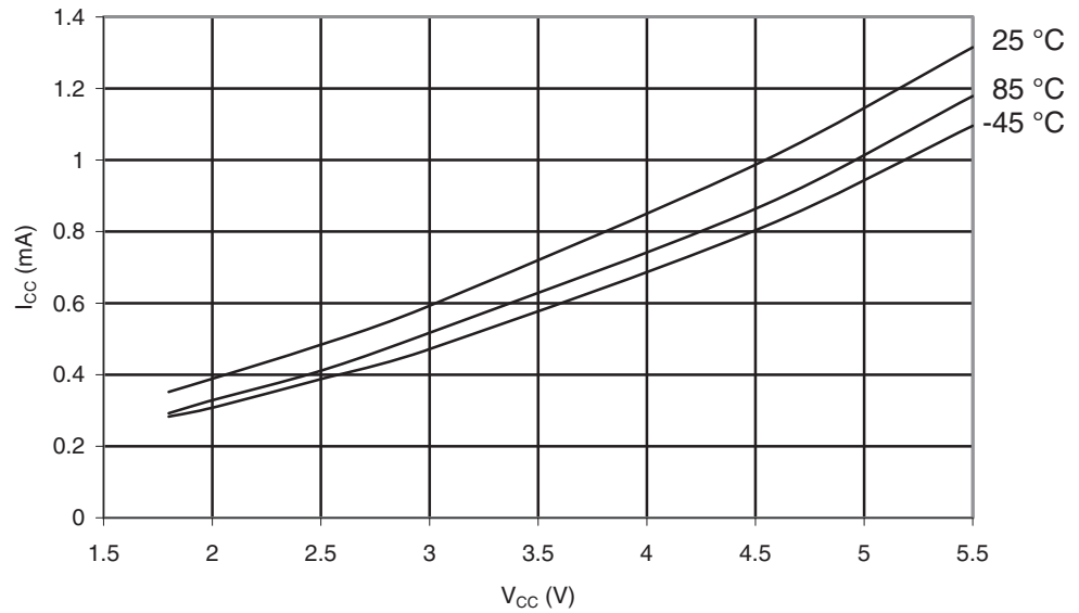
Figure 30-4. ATmega169A: Active Supply Current vs. V_{CC} (Internal RC Oscillator, 1MHz)
