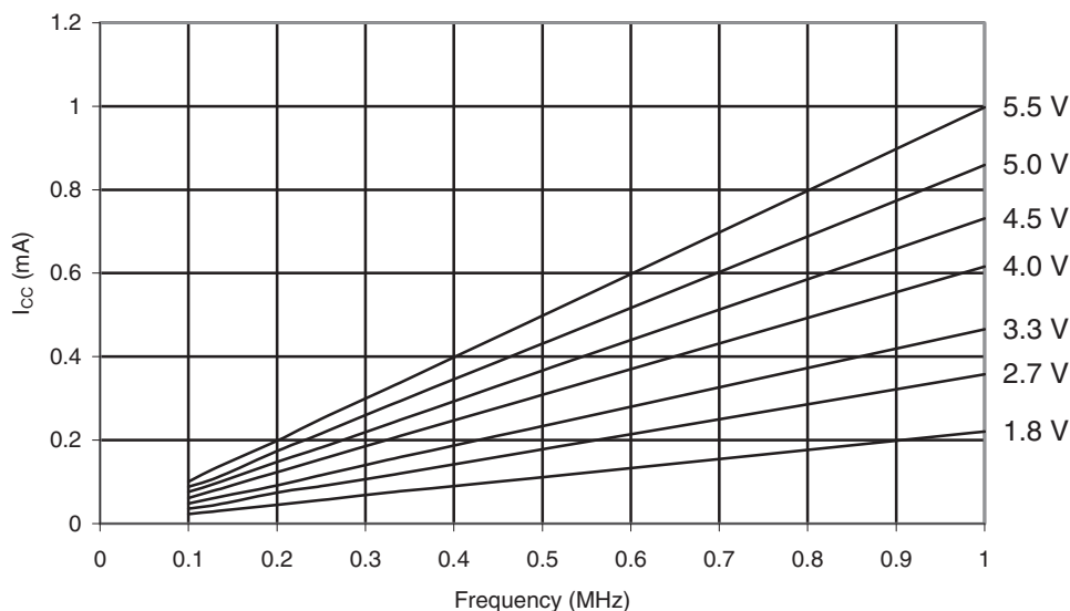
Figure 30-1. ATmega169A: Active Supply Current vs. Low Frequency (0.1 - 1.0MHz)
