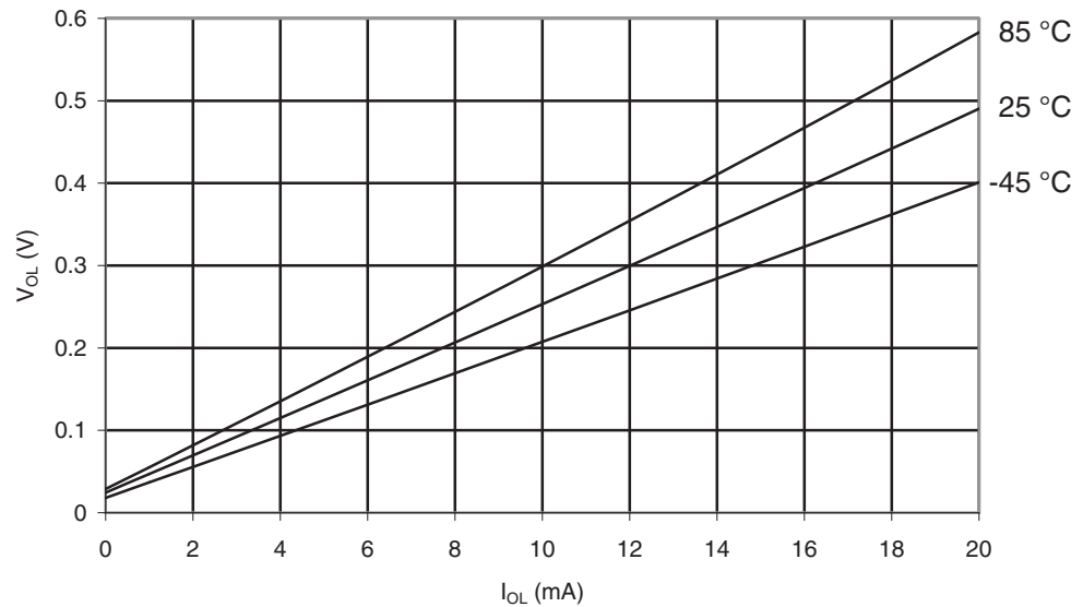
Figure 30-31. ATmega169A: I/O Pin Output Voltage vs. Sink Current, Port B ( V_{CC} = 5V )
