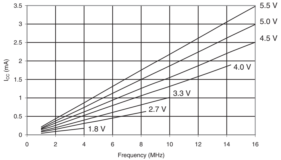
Figure 30-69. ATmega169PA: Idle Supply Current vs. Frequency (1 - 16MHz)
