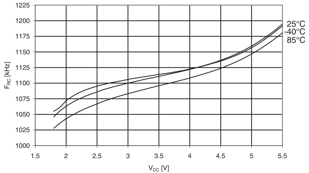
Figure 30-169. ATmega329A: Watchdog Oscillator Frequency vs. V_{CC}
