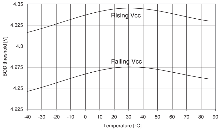
Figure 30-284. ATmega3290A: BOD Thresholds vs. Temperature (BOD Level is 4.3V)
