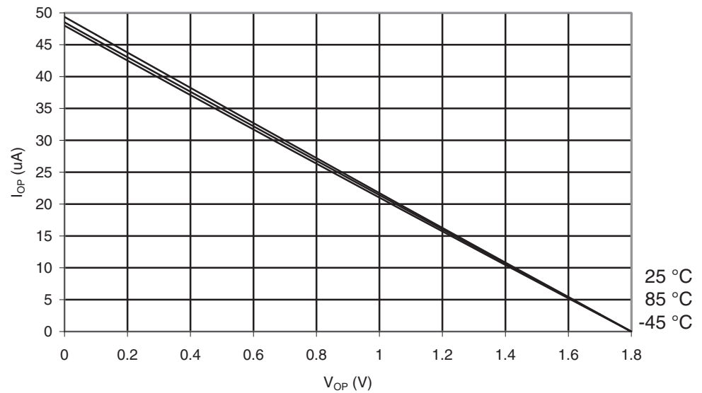
Figure 30-80. ATmega169PA: I/O Pin Pull-up Resistor Current vs. Input Voltage ( V_{CC} = 1.8V )
