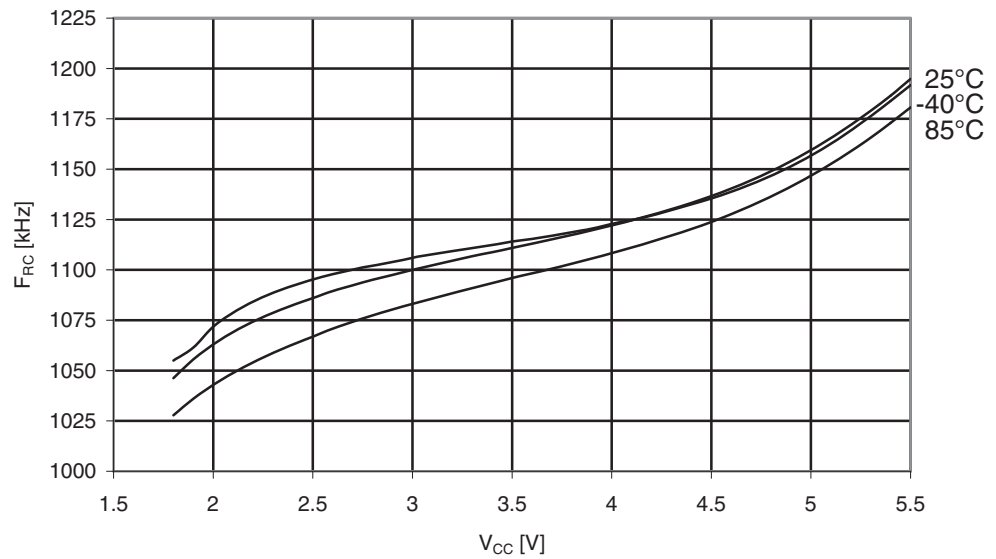
Figure 30-289. ATmega3290A: Watchdog Oscillator Frequency vs. V_{CC}
