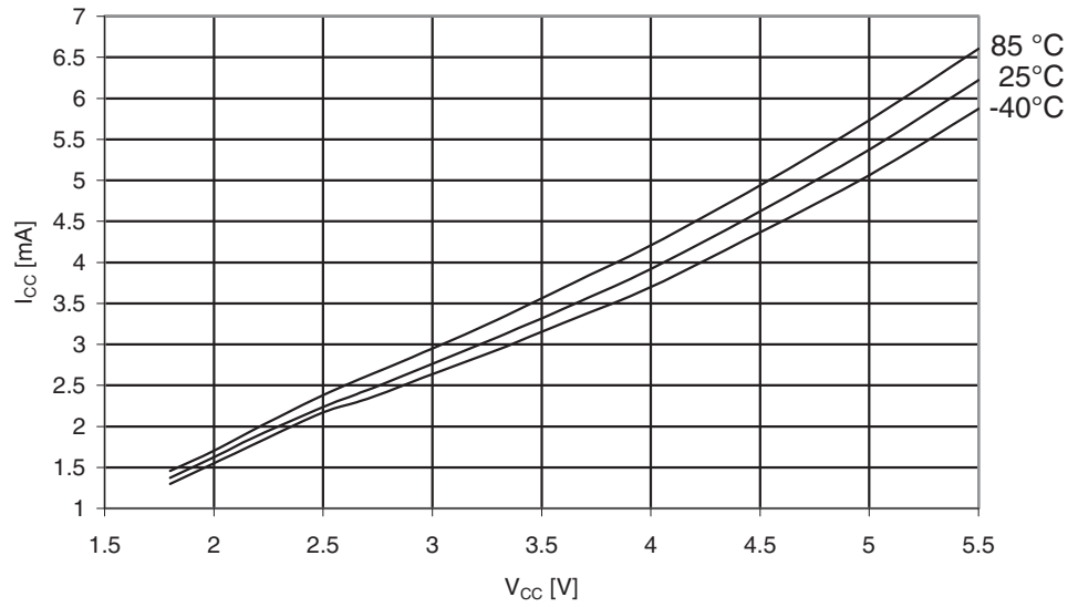
Figure 30-127. ATmega329A: Active Supply Current vs. V_{CC} (Internal RC Oscillator, 8MHz)
