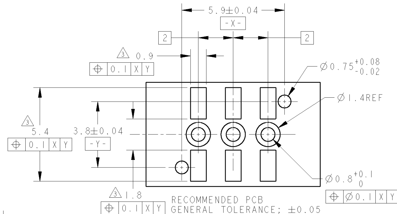
PLUG CONNECTOR
