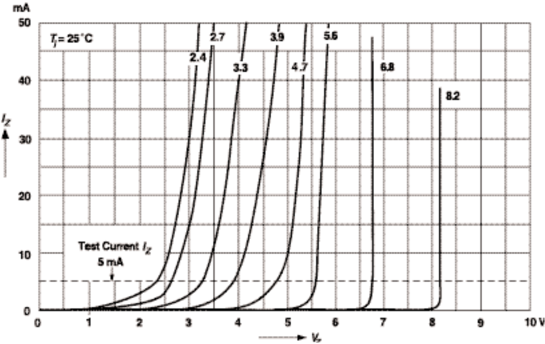
Breakdown characteristics
