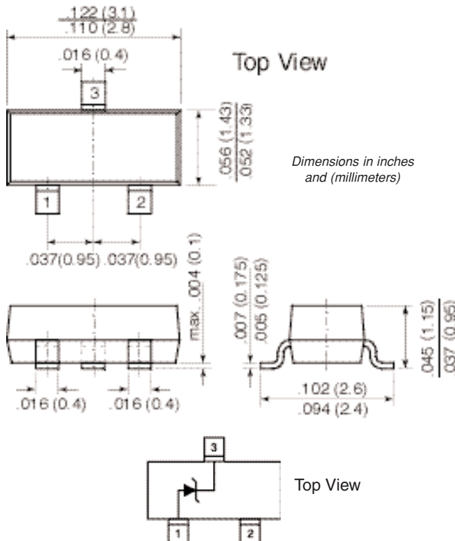
TO-236AB (SOT-23)
