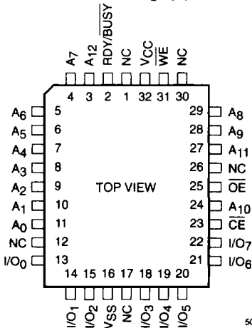
PLCC Package (N)
