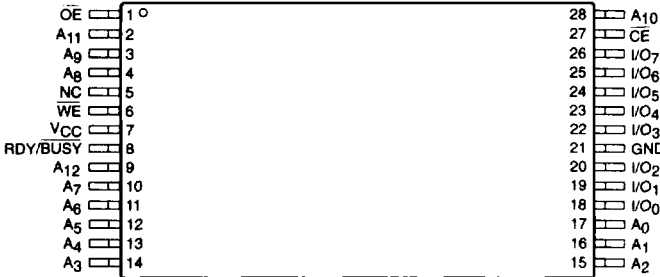
TSOP Package (8mm x 13.4mm) (T13)
