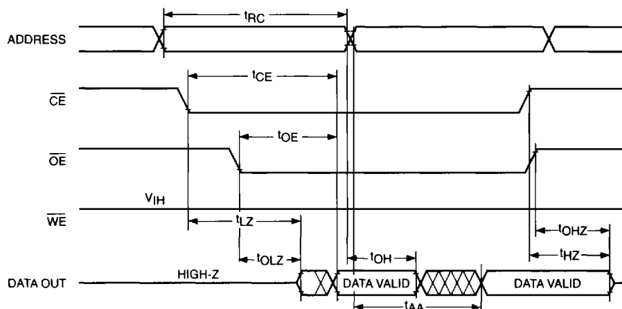
Figure 3. Read Cycle
