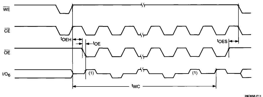
Figure 8. Toggle Bit
