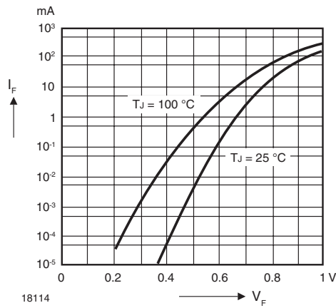
Figure 1. Forward characteristics
