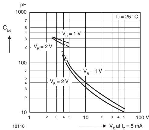
Figure 2. Capacitance vs. Zener Voltage
