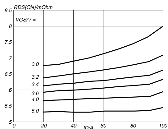
Fig.6. Typical on-state resistance, T_j = 25\ ^\circ C . R_{DS(ON)} = f(I_D)
