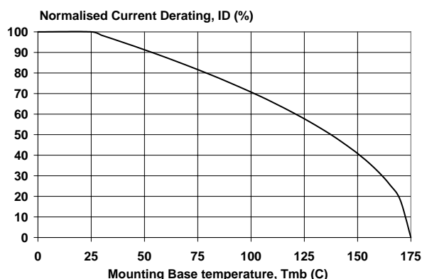
Fig.2. Normalised continuous drain current. ID\% = 100 \cdot I_D / I_{D\ 25\ ^\circ C} = f(T_{mb}) ; conditions: V_{GS} \geq 5\ V
