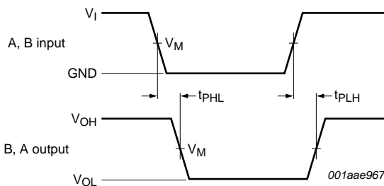
Measurement points are given in Table 14 . V_{OL} and V_{OH} are typical output voltage drops that occur with the output load.
