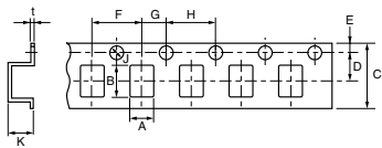
Dimensions of indented square hole plastic tape
