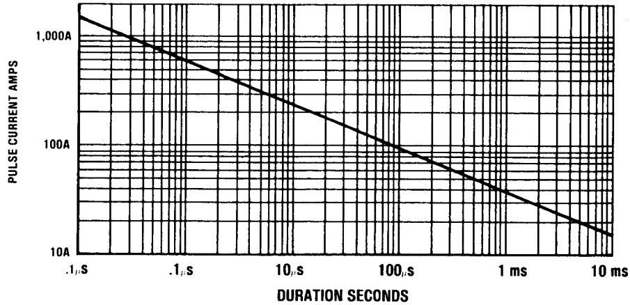
FIGURE 3 SURGE DURATION vs PULSE CURRENT Square Pulse Current vs Duration for Non-Repetitive Pulse
