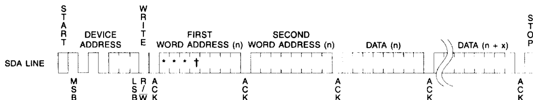
Figure 3. Page Write
