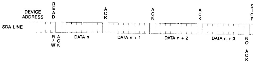
Figure 6. Sequential Read
