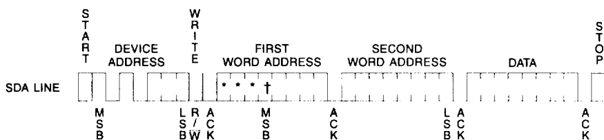
Figure 2. Byte Write
