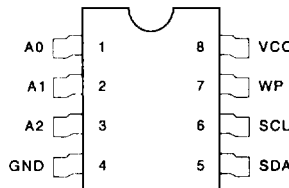
8-Pin SOIC
