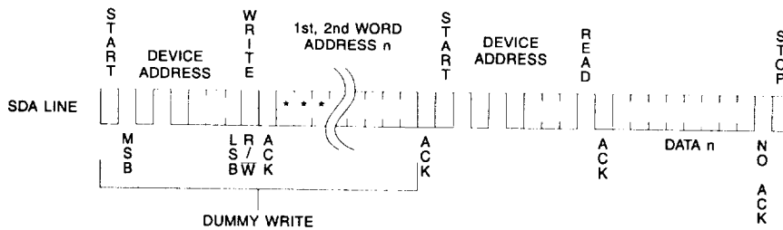
Figure 5. Random Read
