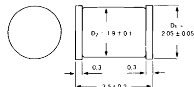
SOD-87
