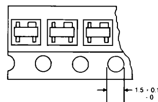
SOT-143 ORIENTATION
