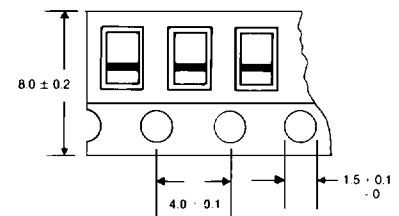
SOD-87 TAPE DIMENSIONS AND ORIENTATION
