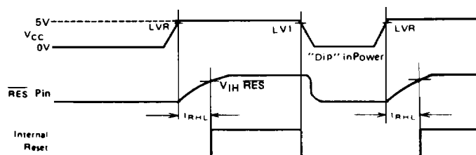
Figure 7 Power Up and \overline{\text{RES}} Timing
