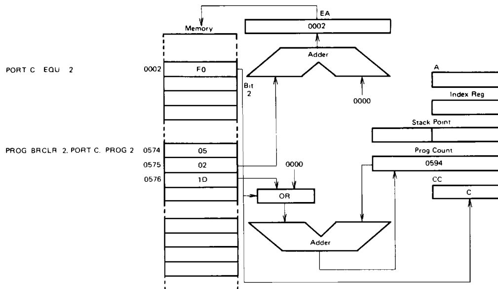
Figure 25 Bit Test and Branch Addressing Example
