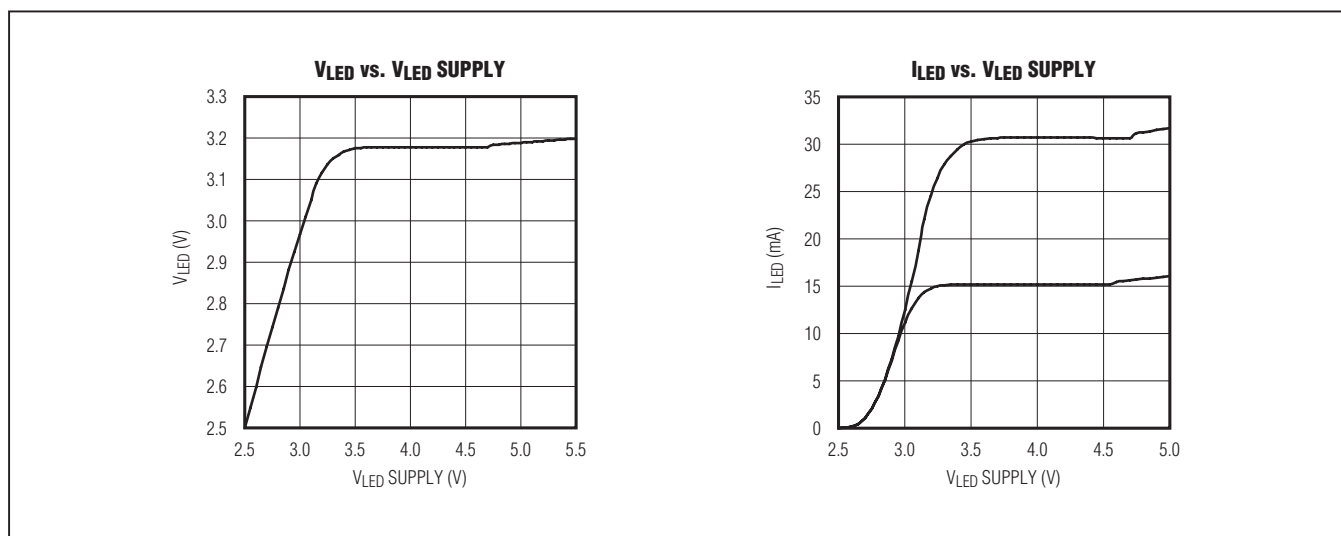
Figure 16. LED Brownout
