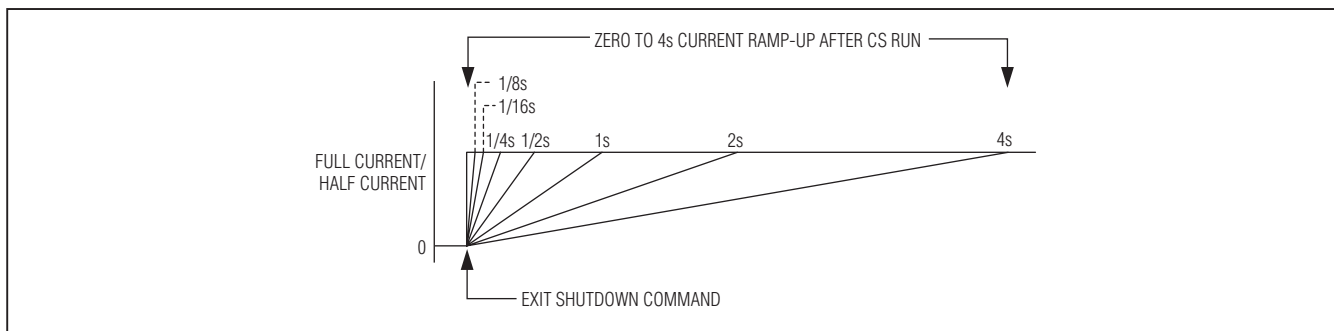
Figure 4. Ramp-Up Behavior
