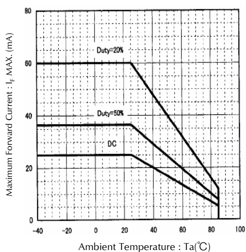
Derating Ambient Temperature vs. Maximum Forward Current Repetition Frequency : f \geq 100\text{Hz}
