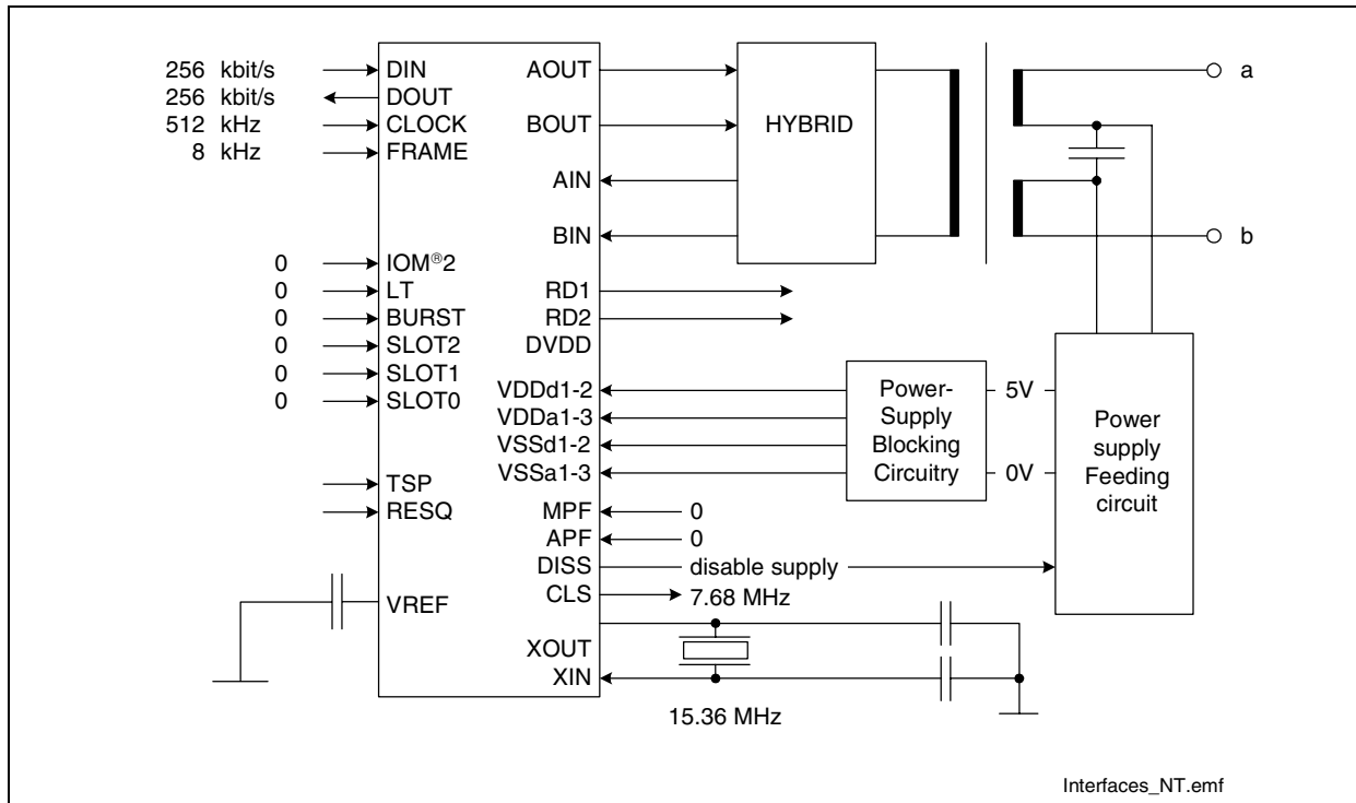
Figure 45 Interfaces of the NTC-T AM with IEC-T Functionality Selected in NT Mode
