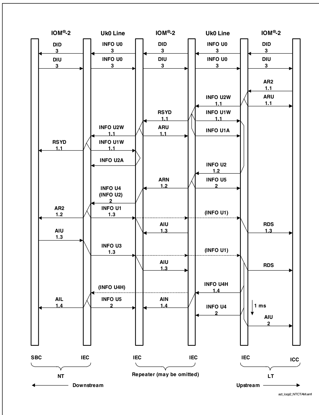
Figure 74 Activation of Loop 2 with NT
