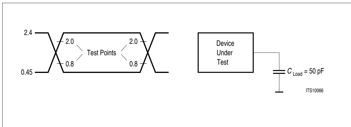
Figure 90 Input/Output Waveform for AC Tests
