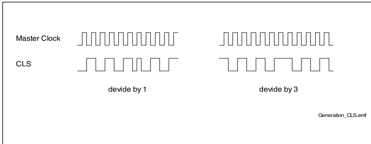
Figure 64 Generation of CLS from the Master Clock
