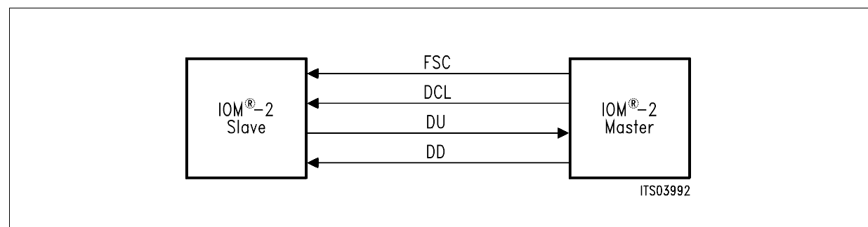
Figure 10 IOM ® -2 Clocks and Data Lines
