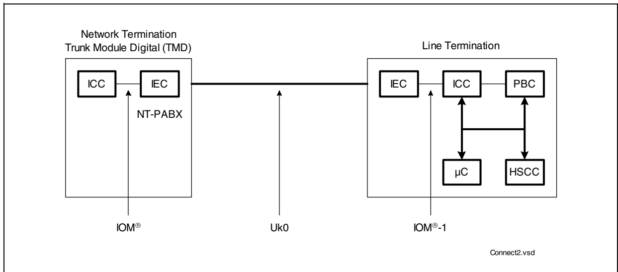
Figure 38 Connecting Private to Public Network
