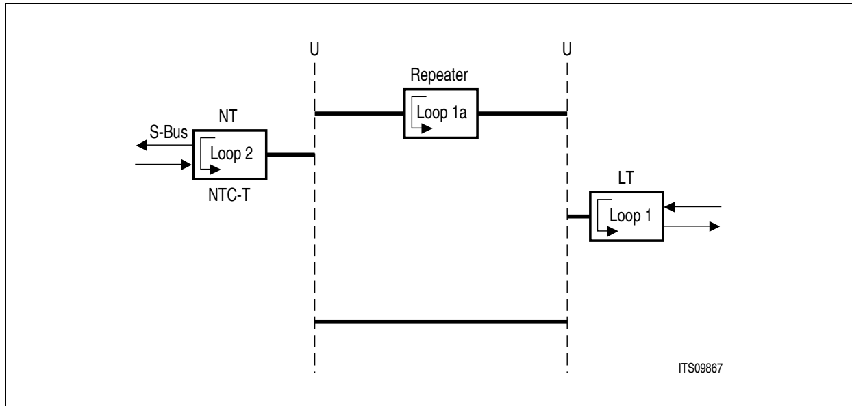
Figure 19 Test Loop-Backs
