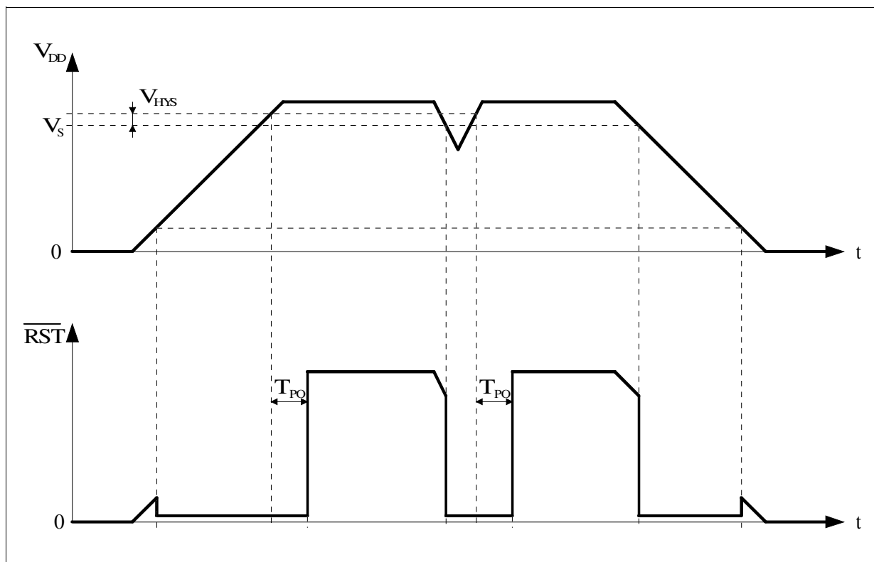
Figure 95 Undervoltage Detection
