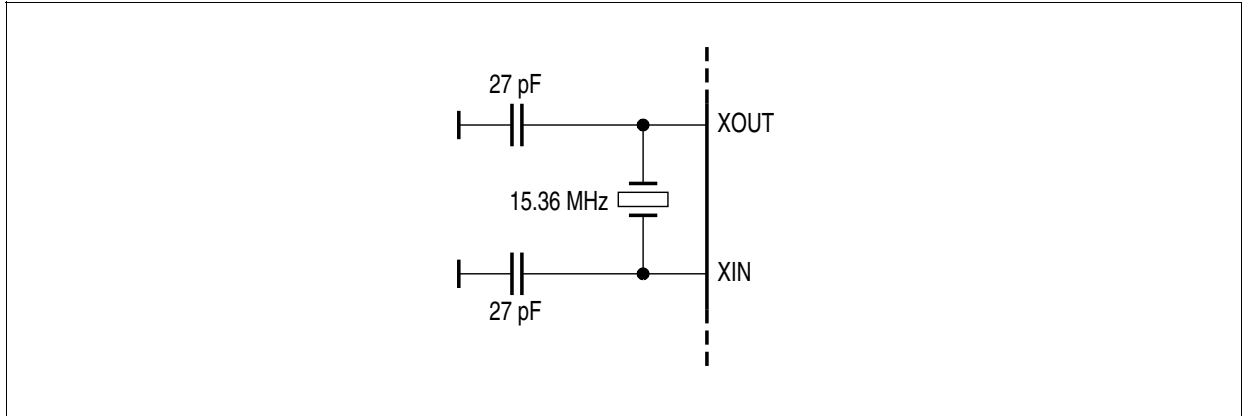
Figure 35 Crystal Oscillator
