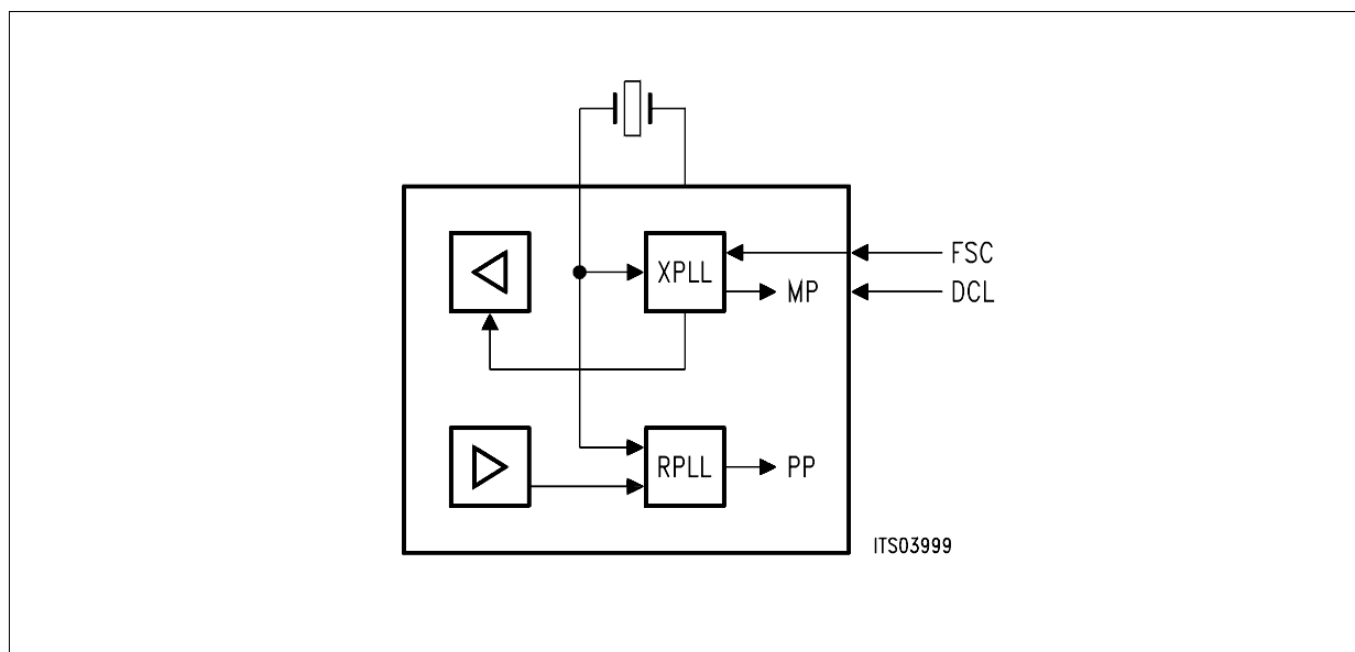
Figure 30 Clock System of the S-Transceiver
