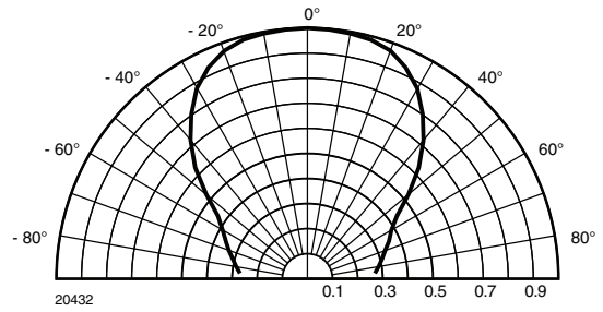
Fig. 12 - Directivity
