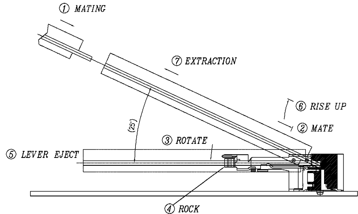
HOW TO MATE AND UNMATE
