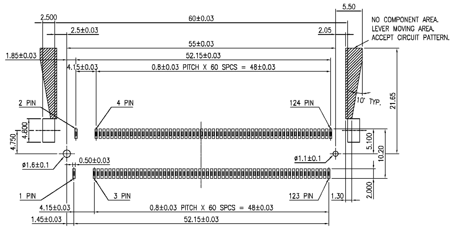
RECOMMENDED P.D. BOARD PATTERN LAYOUT (CONNECTOR MOUNTING SIDE)
