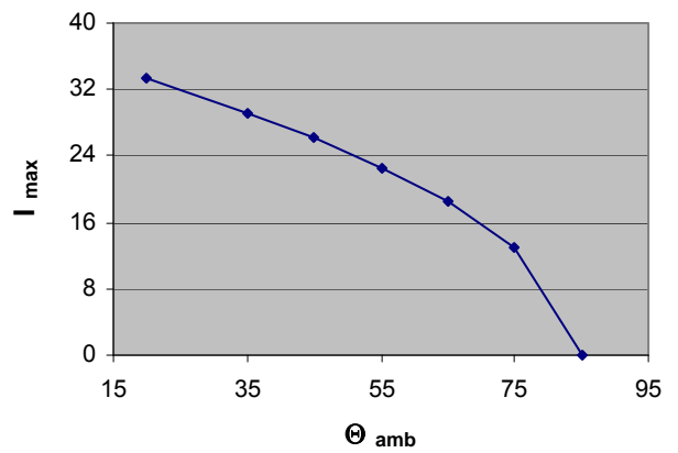
Max. allowable current (rms) at specific ambient Temp. B25667C2317A 175
