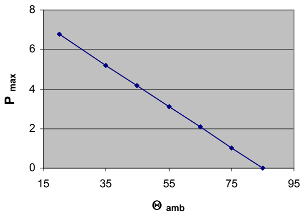
Max. allowable power loss at specific ambient Temp. B25667C2317A 175
