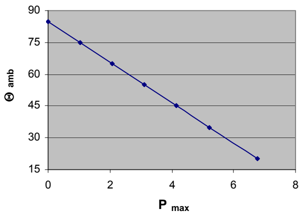
Max. allowable ambient Temp. at specific power loss B25667C2317A 175
