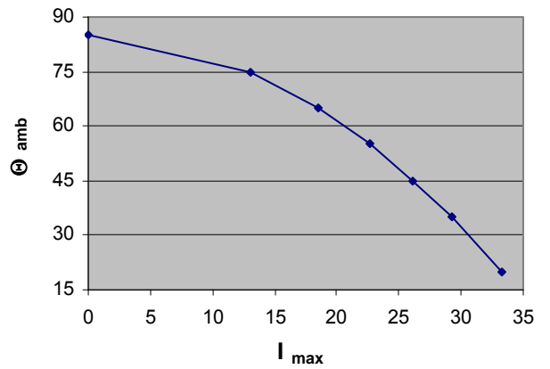
Max. allowable ambient Temp. at specific current (rms) B25667C2317A 175
